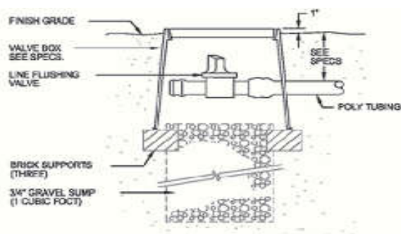
Figure 2.1 manual flushing
