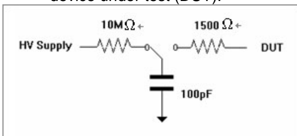
Fig 2.3: Human Body Model (HBM) test circuit
