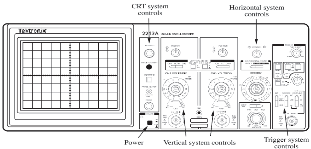
Fig. 2.2. Oscilloscope front panel with functional blocks marked.
