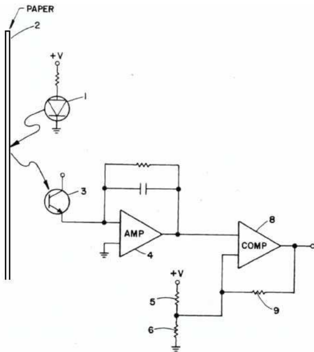
Figure 2.2 . paper sensor used in a laser printer
