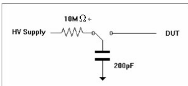
Fig 2.4 : Machine Model (MM) test circuit
