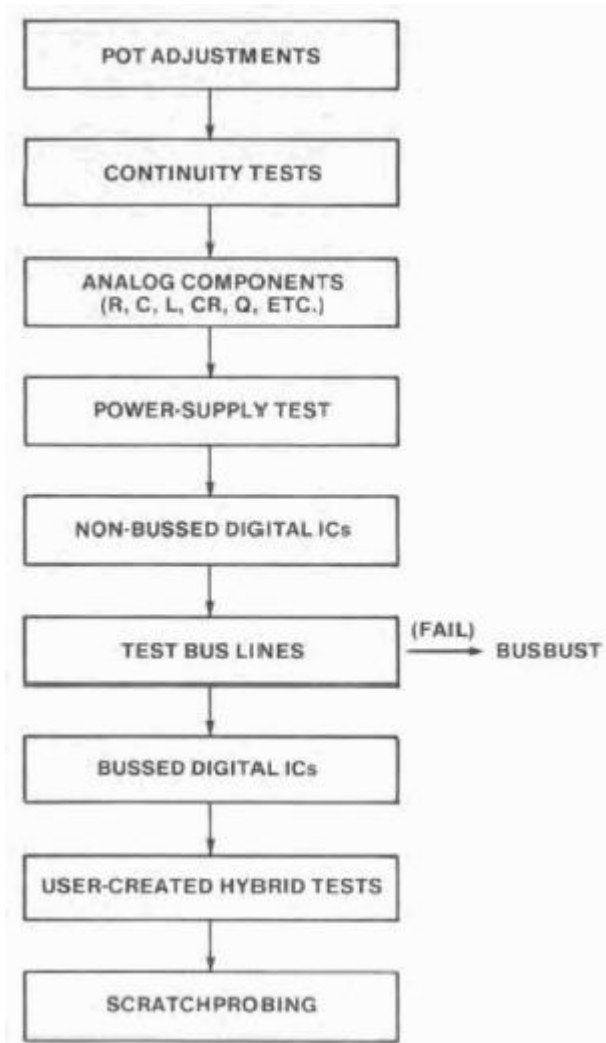
Fig6.3. testing procedures
