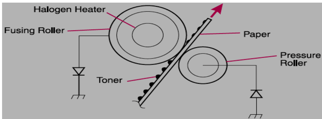
Fig 3.11 Fusing System
