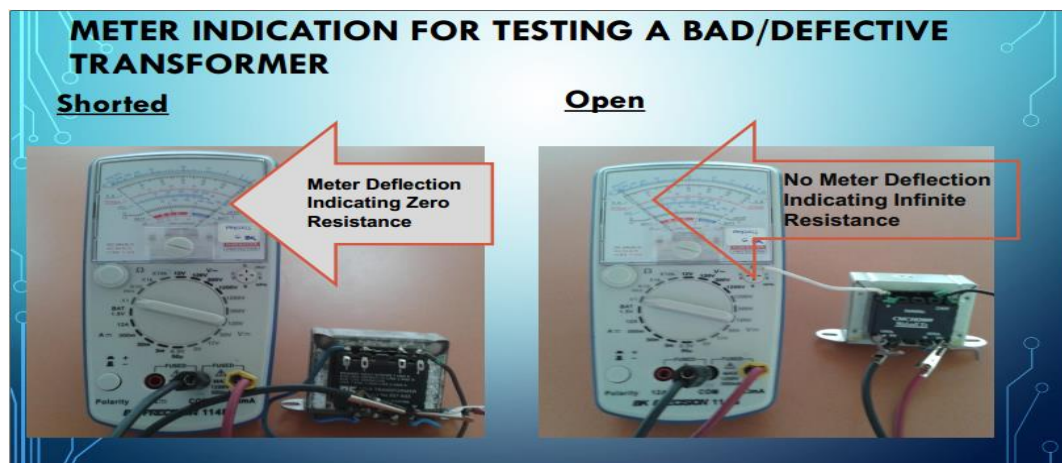
Figure 2.5.b . Transformer testing
