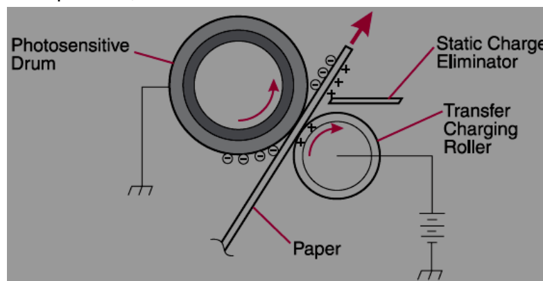
Fig 3.12 transering unit
