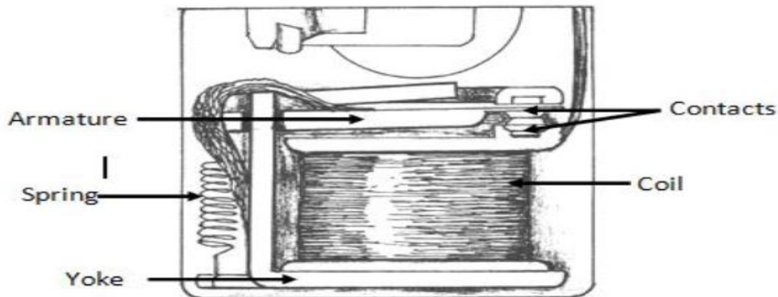
Figure 2.5.c . Electromagnet Type Relay
