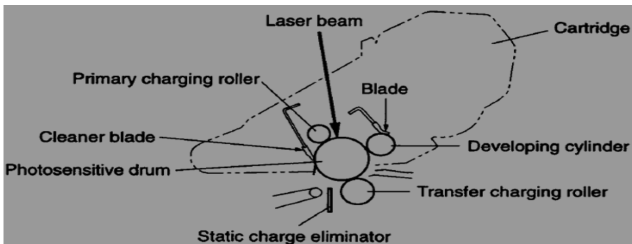
Fig 3.6 units of photocopy units
