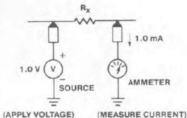
Fig 6.2 voltage/current
