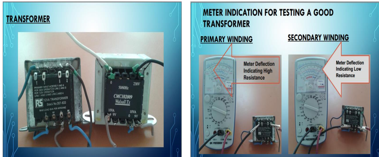
Figure 2.3 a . Transformer testing
