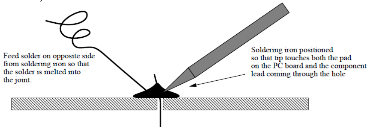
Figure 3.1 : Proper Soldering Technique
