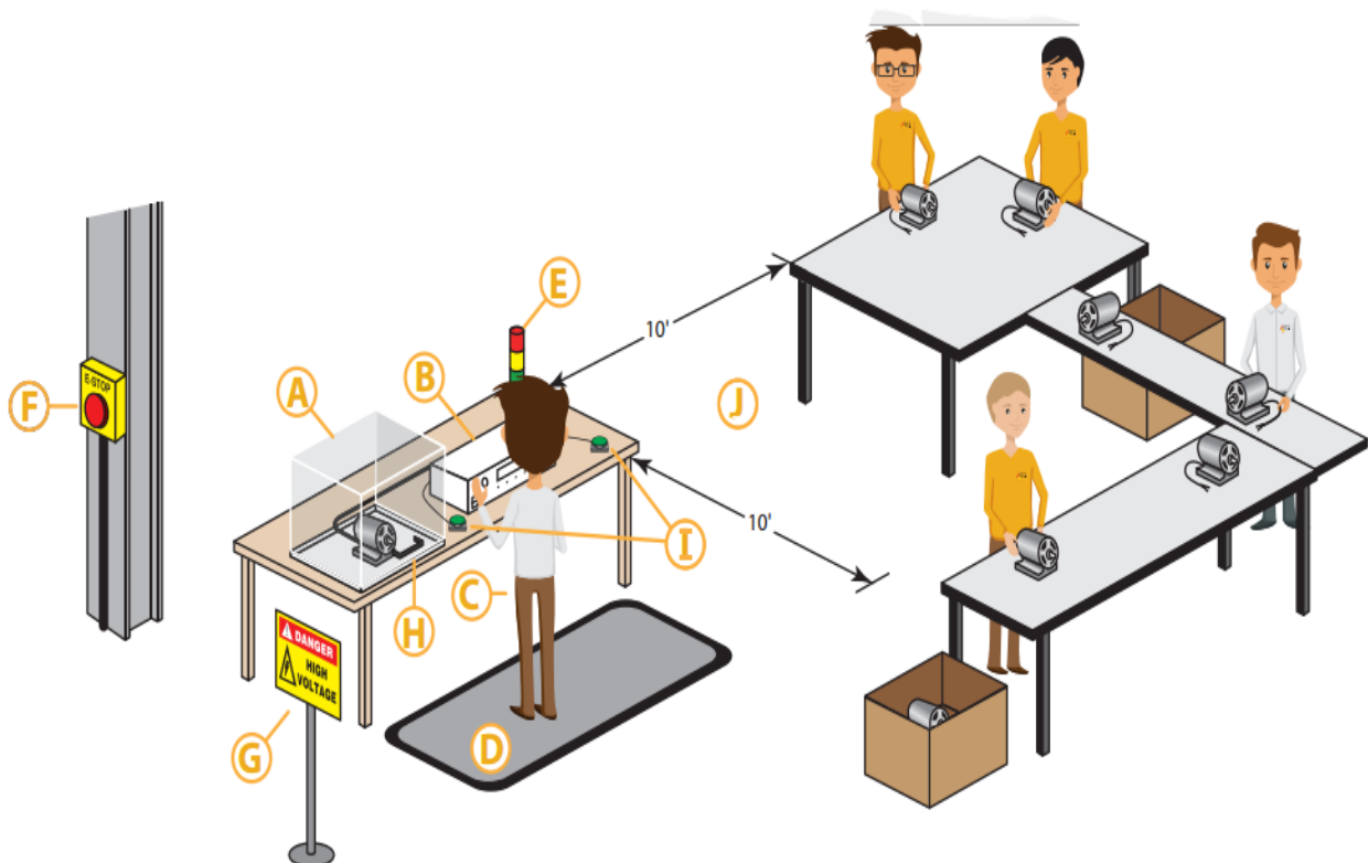
fig 4.1 Arrangement of work place
