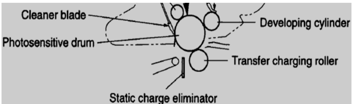
Fig 3.11 separations
