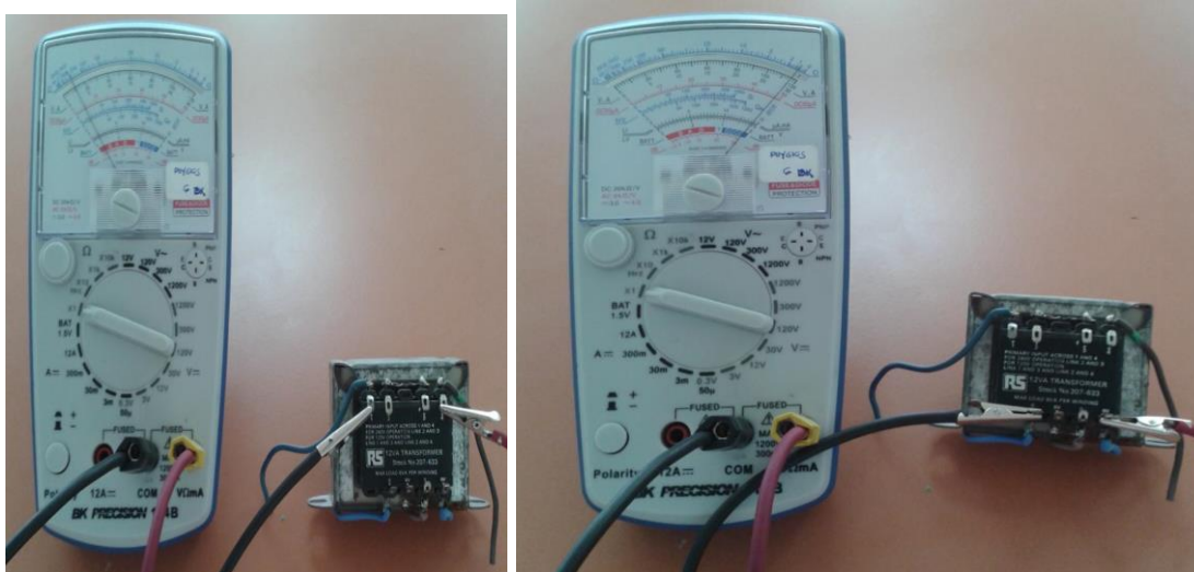
Figure 4.1 test transformer
