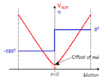
LVDT Displacement Sensor
