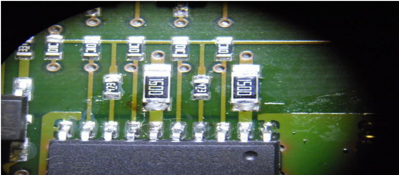
Figure 8.1 Contaminants soldering
