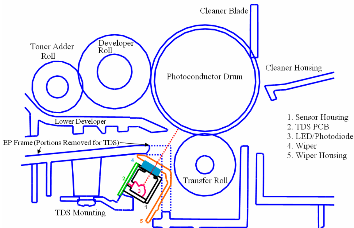
Figure 2.3 . TDS Implemented
