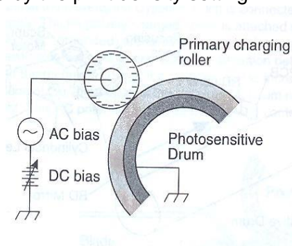
Fig 3.10 primary charging Roller
