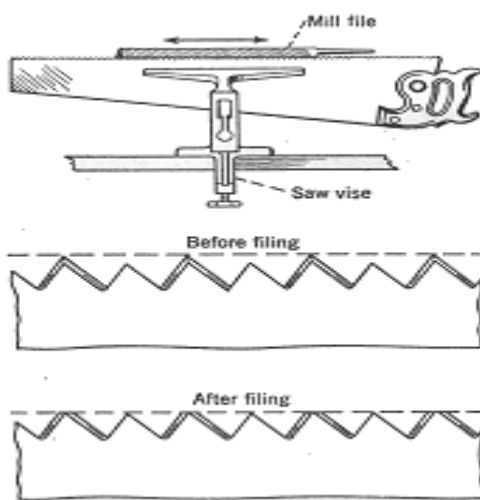
Fig.3.1.1 Jointing of hand saw Rip saw Cross cut saw
