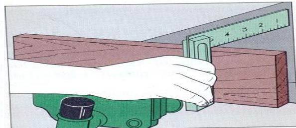
Testing an edge for squareness.
