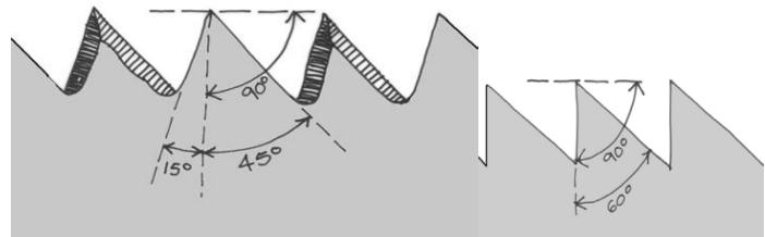
Fig.3.1.1 Jointing of hand saw Rip saw Cross cut saw
