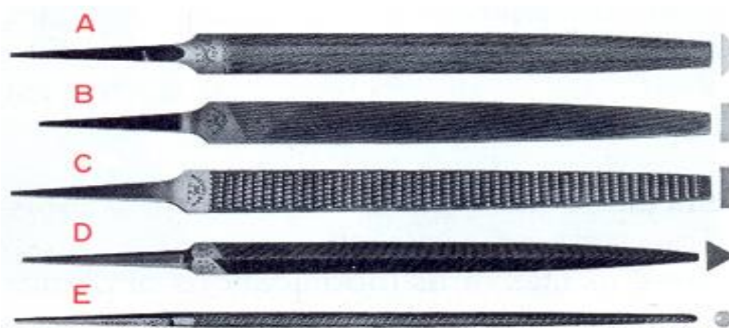
Some common files for wood: (A) half-round, (B) flat double-cut, (C) flat rasp, (D) triangular, and (E) round.
