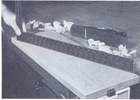
Testing diagonally for a wind
