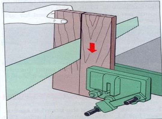
Ripping a board held in a vise.
