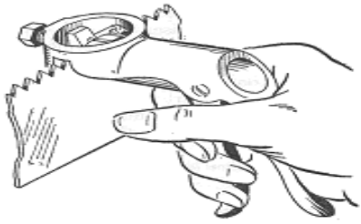
Fig. 3.1.3 setting of hand saw
