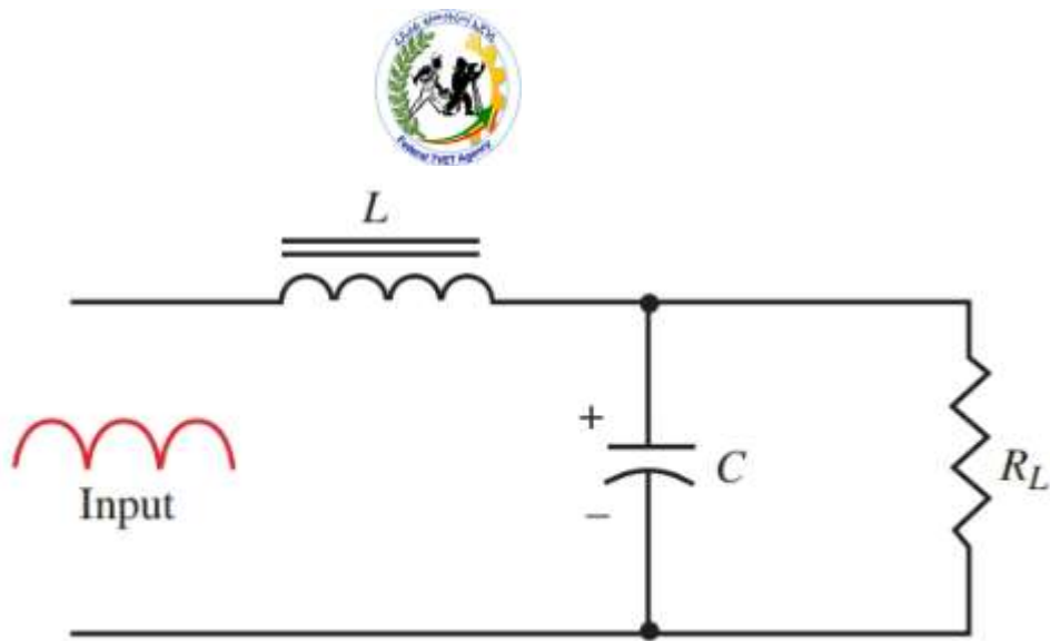
Figure 22. Choke input L filter
