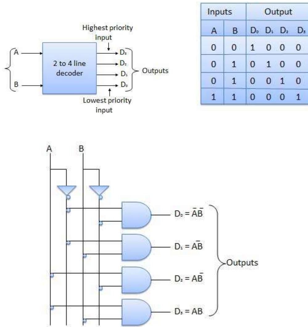
Fig 4.35. Decoder block diagram, truth table and schematic circuit
