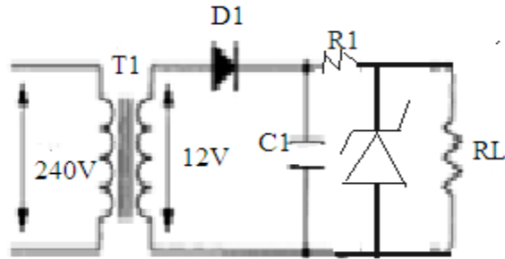
Fig 4.22. Voltage regulator
