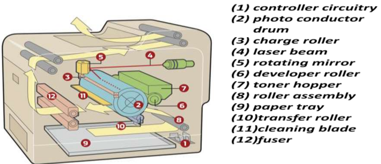
Fig1.12 Laser Printer Parts
