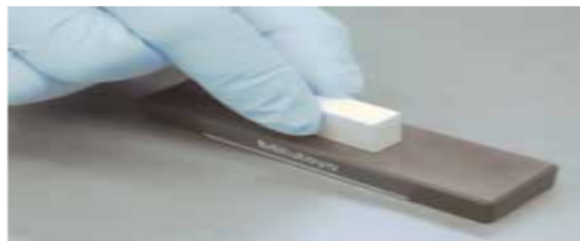
Fig. 2.61. A. Optical flat to check the measuring face B. Ceraston
