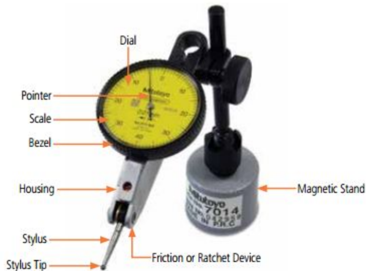
Fig. 2.48. parts of dial test indicator.
