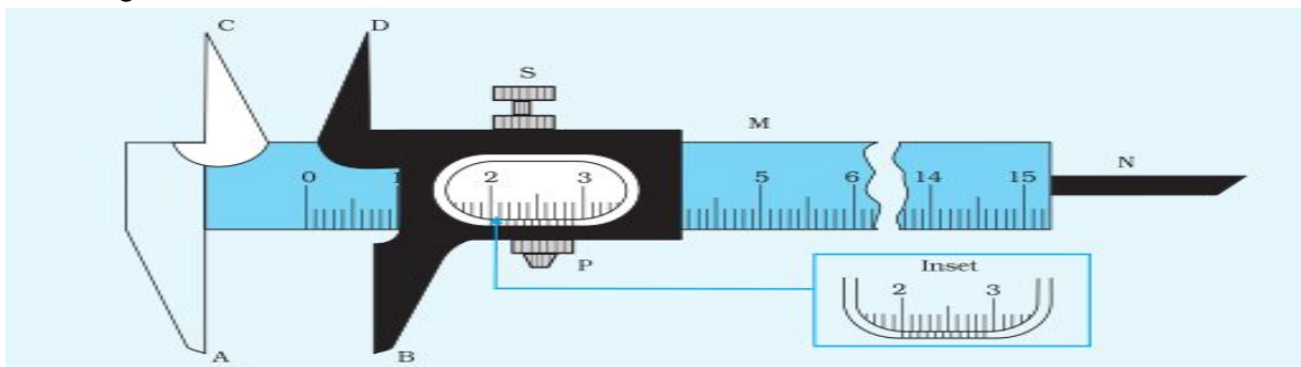
Fig. 3.19. The Vernier caliper and its parts.
