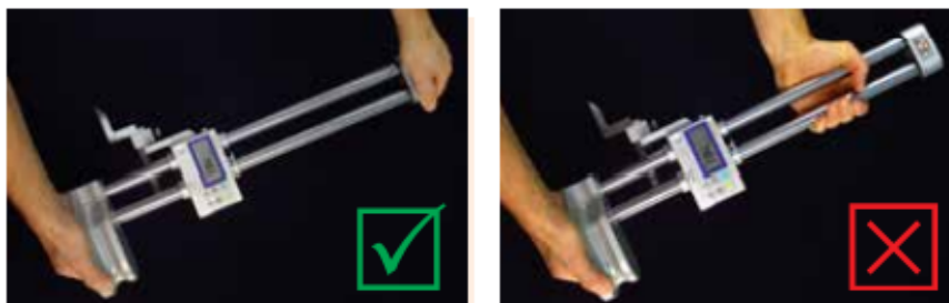
Fig.2. 40. Proper usage of gauge.
