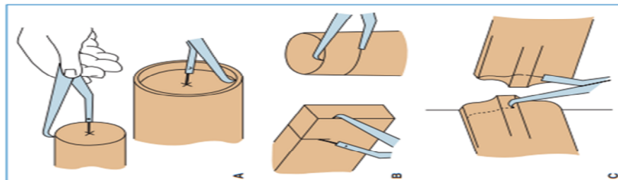
Fig. 3.17. The hermaphrodite caliper
