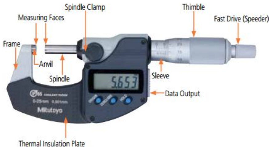
Fig. 2.19. parts of out side micro meter
