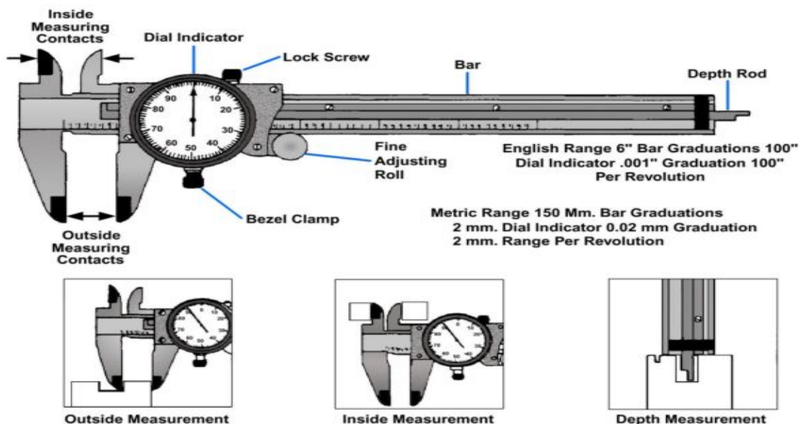
Fig. 3.21. Dial caliper part
