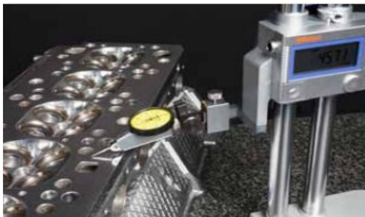
Fig. 2.51. Measurement direction
