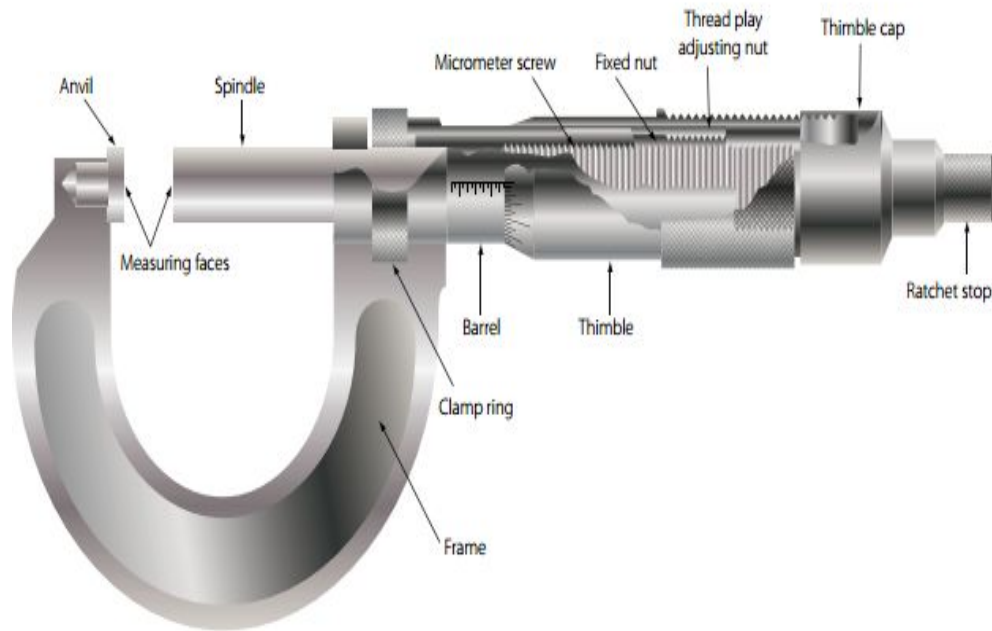
Fig. 3.23. Parts of outside micrometer
