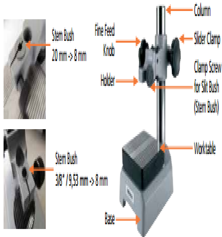
Fig.2.56. parts of Auxiliary Equipment Comparator Stands
