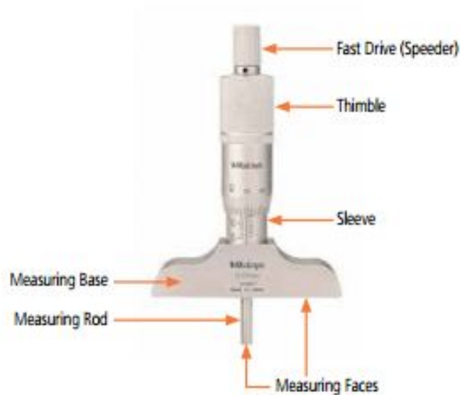
Fig. 2.52. parts of depth measurement.
