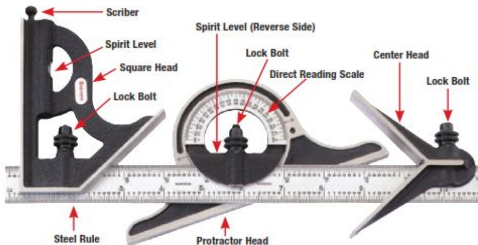
Fig. 3.13. Parts of combination square
