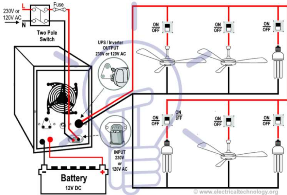
Figure : Automatic UPS / Inverter Wiring with two Wires
