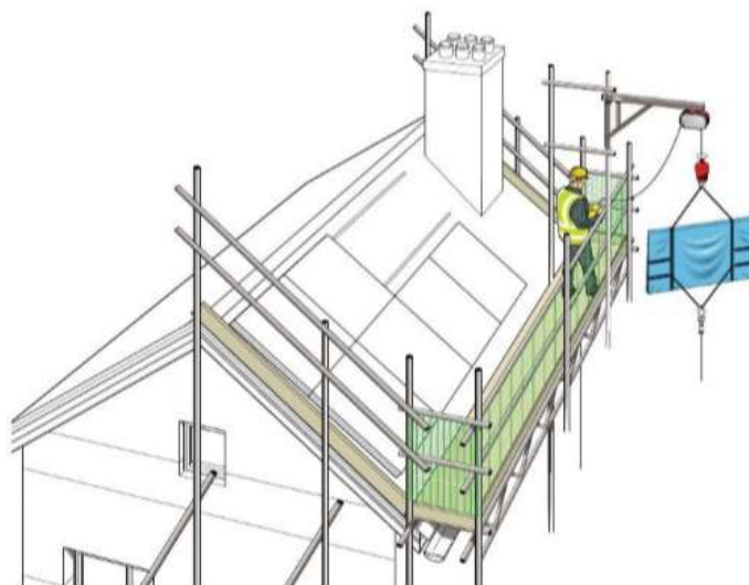
Figure : alternative system with guard-rails and toe-boards
