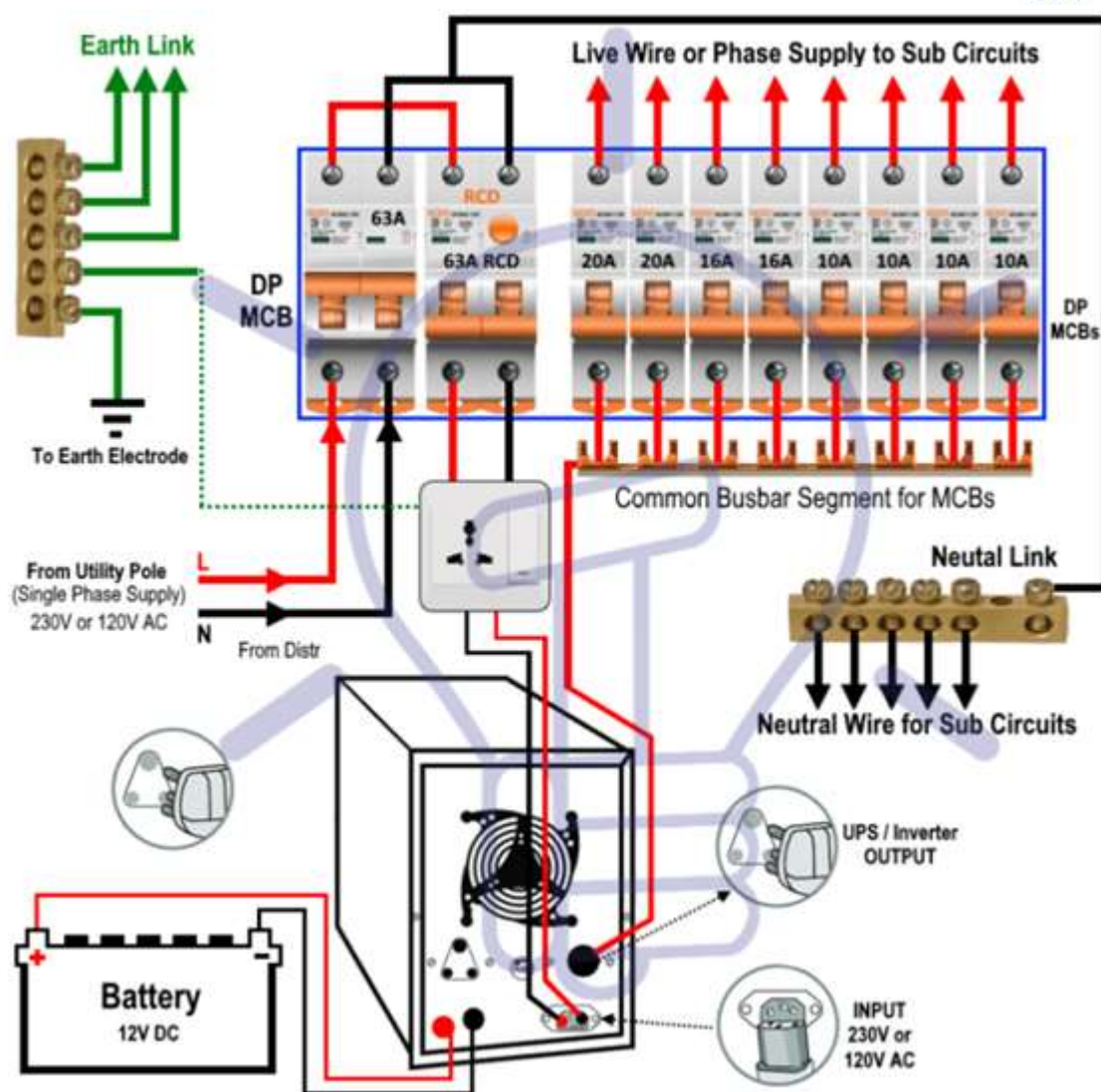
Figure : wire UPS / Inverter to the Home supply
