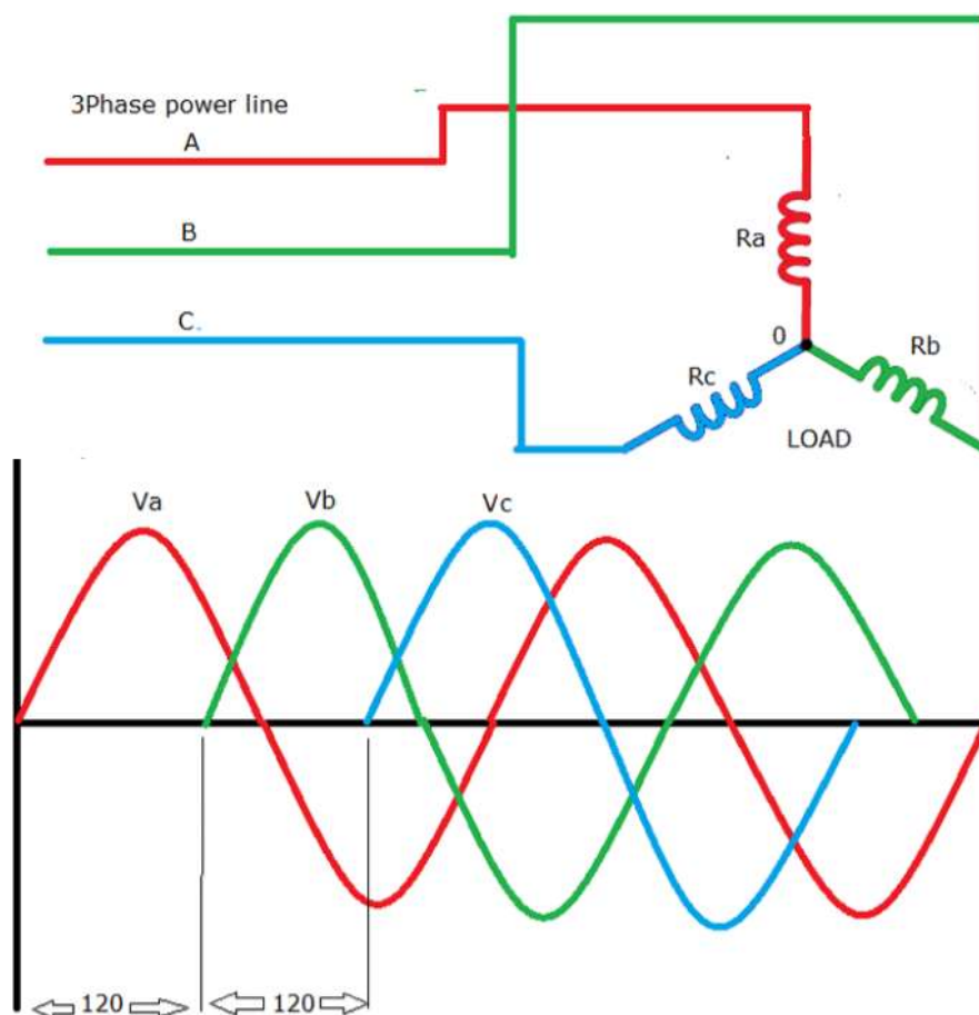
Figure : Three Phase Inverter Circuit
