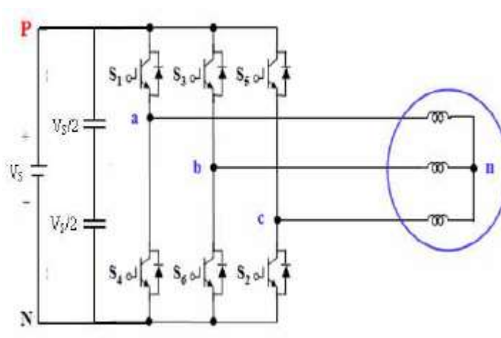
Figure : Three phase inverter using six switches
