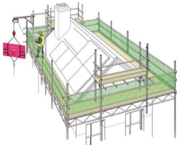
Figure : Fall protection around all edges of the roof of a domestic property during mini grid connected PV system installation
