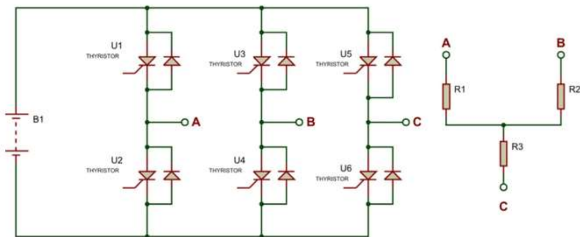
Figure : 3 Phase Inverter Circuit using Thyristors and Diode
