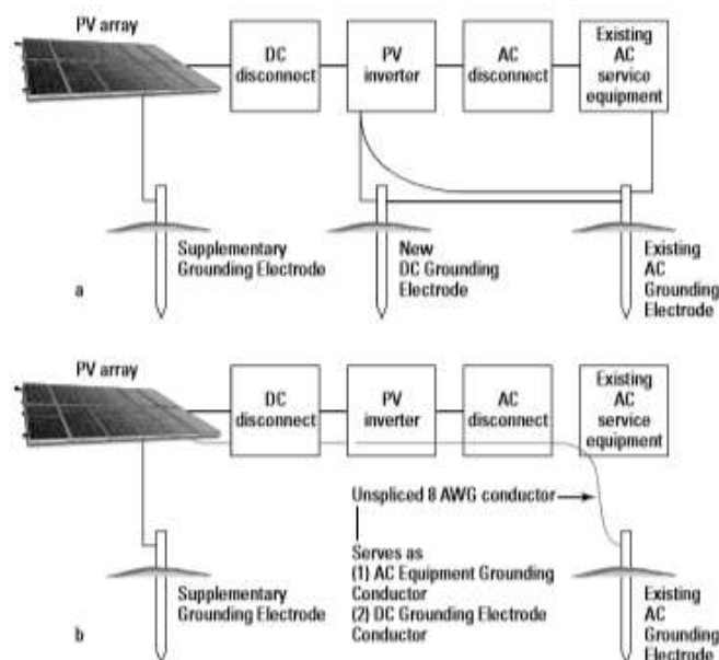
Figure : System-grounding options for utility-interactive PV systems
