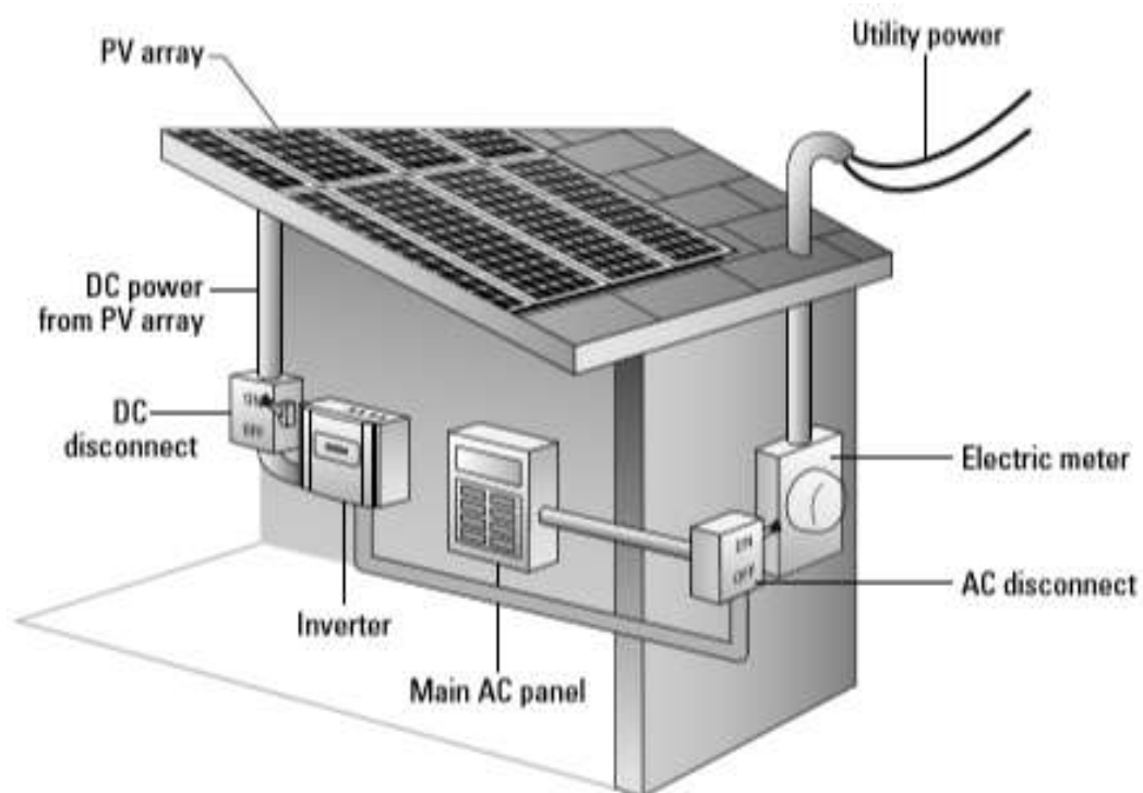
Figure : Typical utility-required disconnect location
