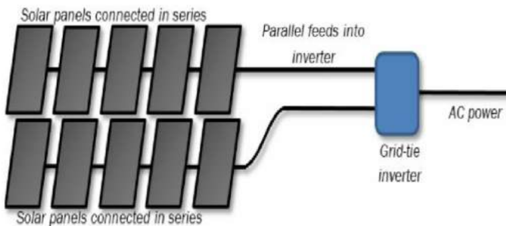
Figure : block diagram showing the basic layout of a low-voltage solar energy system where multiple strings of solar panels are connected in parallel (Boxwell, 2017)
