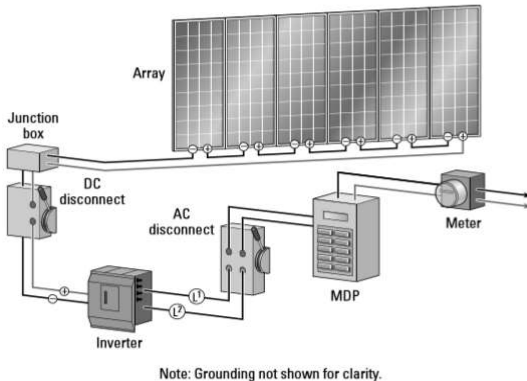
Figure : Typical grid-direct PV system
