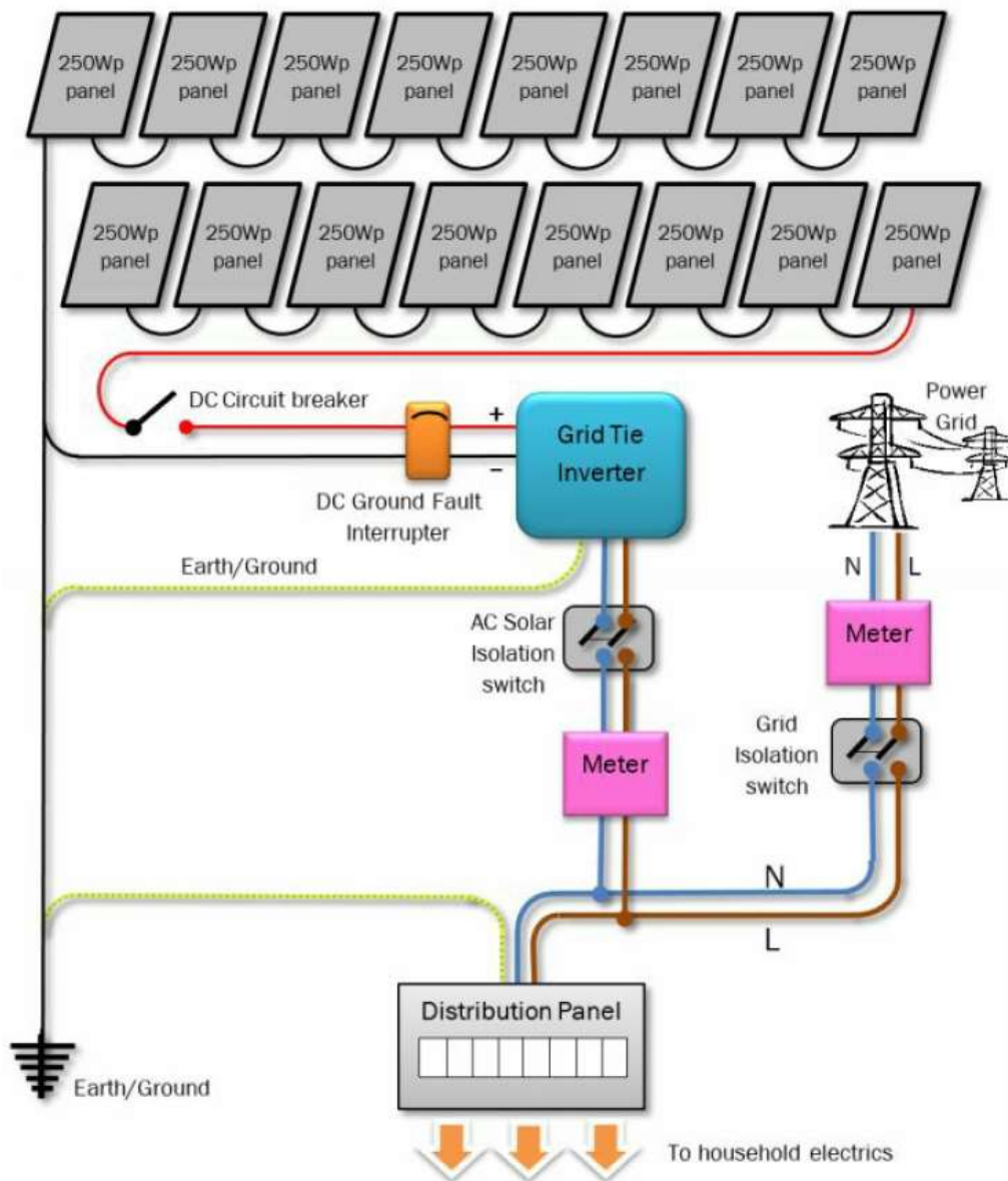
Figure : A sample block diagram for a mini grid connected PV system (Boxwell, 2017)
