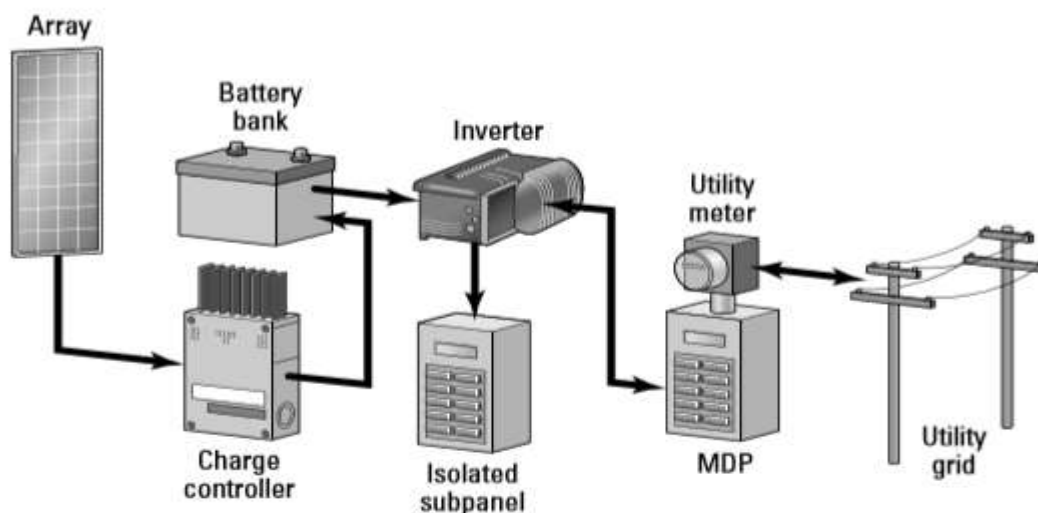
Figure : Utility interactive battery-based PV system
