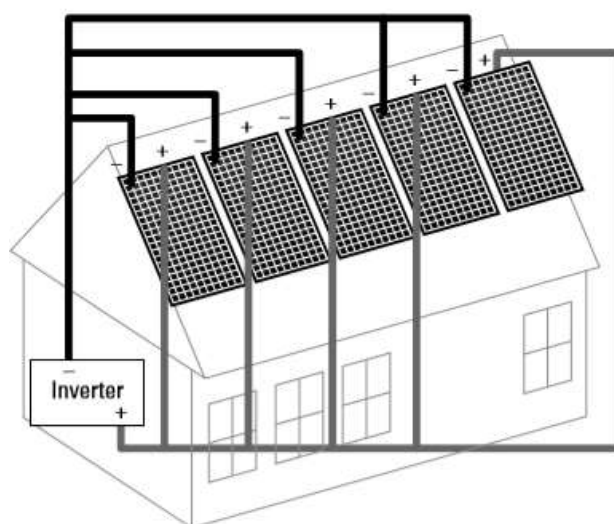
Figure : Five PV modules wired in parallel
