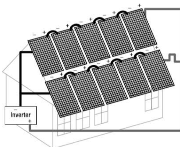
Figure : PV modules wired in a series-parallel configuration
