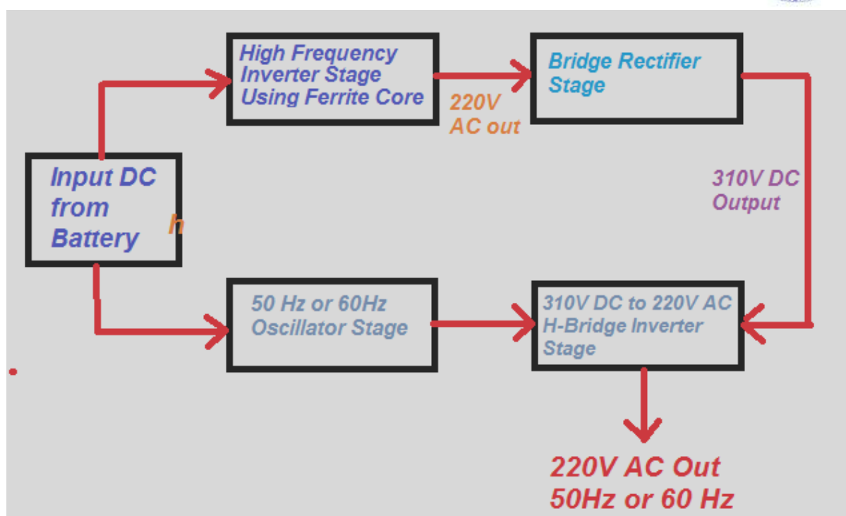
Figure :5kva Ferrite Core Inverter Circuit
