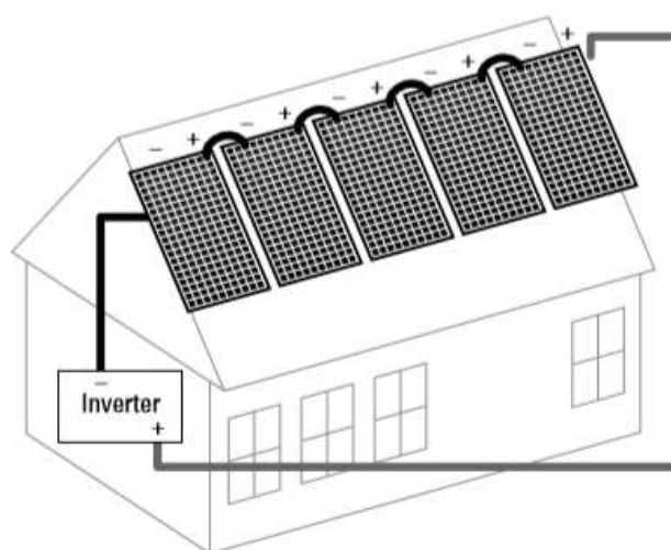
Figure : Five modules wired in series
