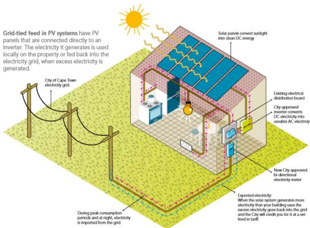
Figure : Grid-tied feed in PV system( www.capetown.gov.za )
