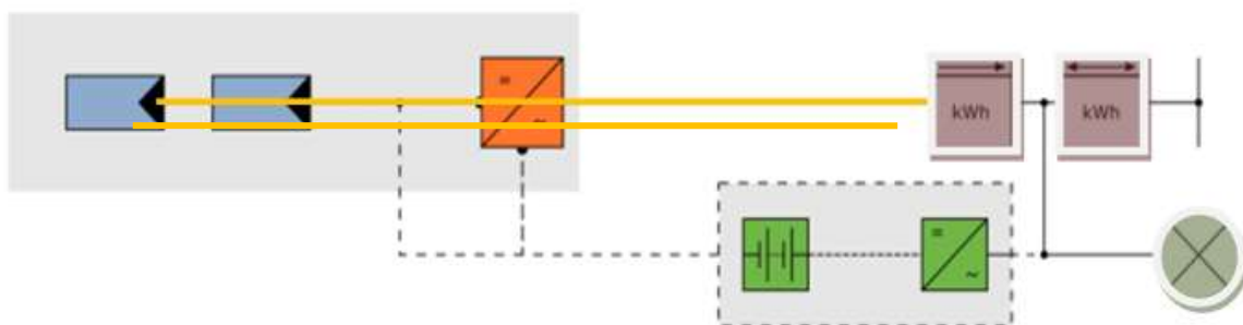
Figure 33: System with appliances and battery system
