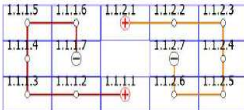
Figure 49: String Diagram
