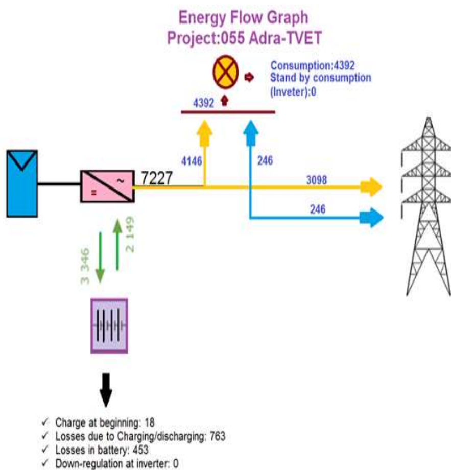
Figure 50: Energy flow graphs
