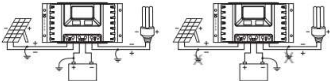
Figure 26: Steca grounding
