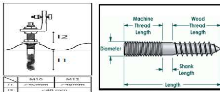
Figure 19: Hanger bolt depth (renusol)
