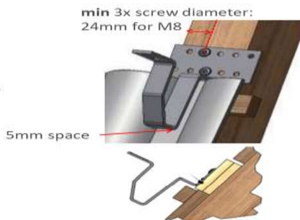
Figure 17: Roof hook mounting
