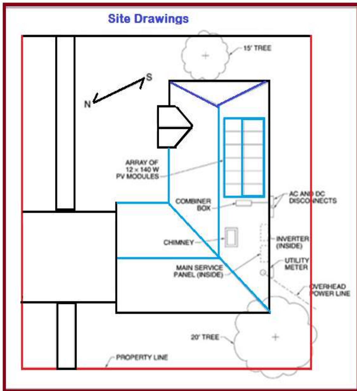
Figure 13: Simple site layout diagram ( https://www.thesolarplanner.com/ )
