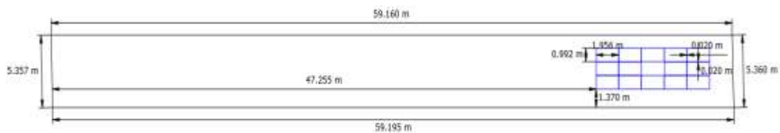
Figure 48: Roof Layout Diagram
