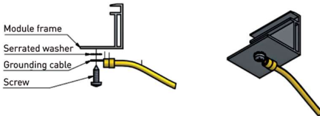
Figure 22: Module grounding (IBC)
