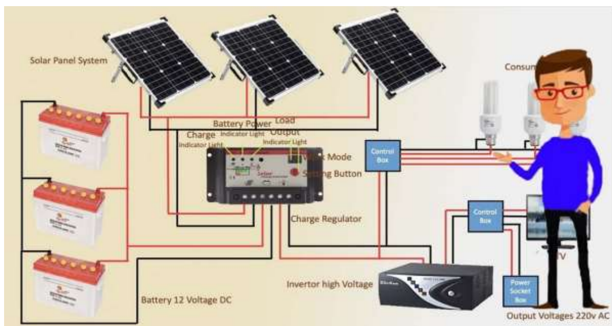
Figure 8: Wiring diagram example ( https://paintingvalley.com/ )
