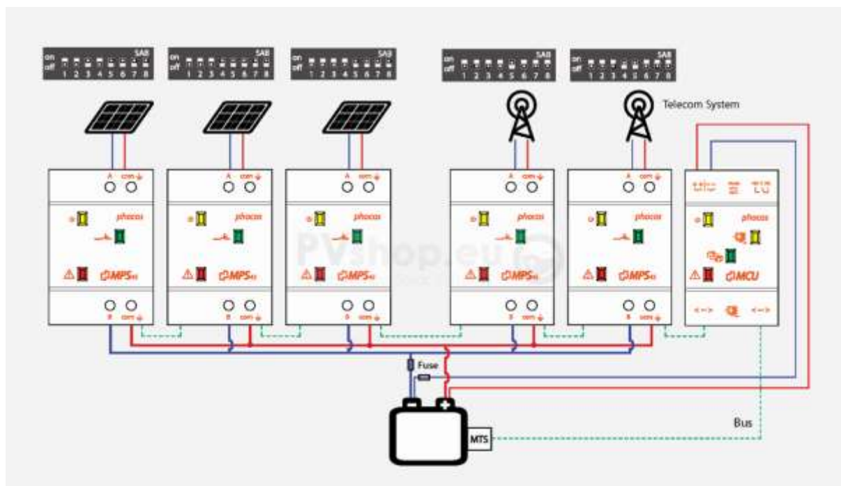
Figure 3: Off Grid Solar System Single Line Diagram
