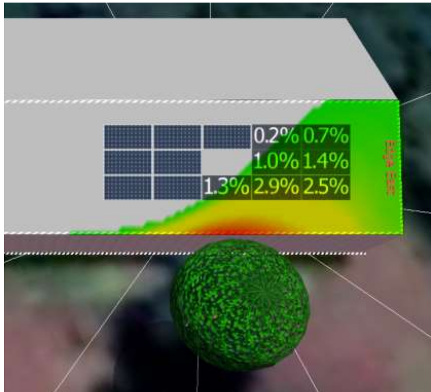
Figure 12: Shading Loss (PVSoL software)
