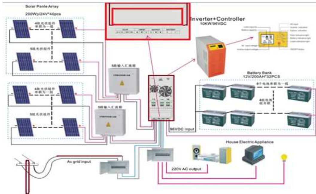
System simplified wiring diagram
