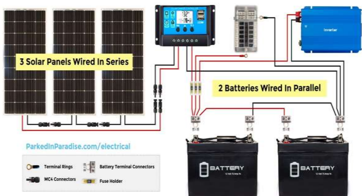
Figure 1: Wiring Connection diagram (pinterest)
