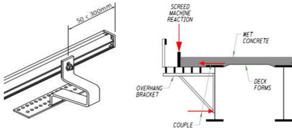
Figure 20: Rail overhangs (Renusol)
