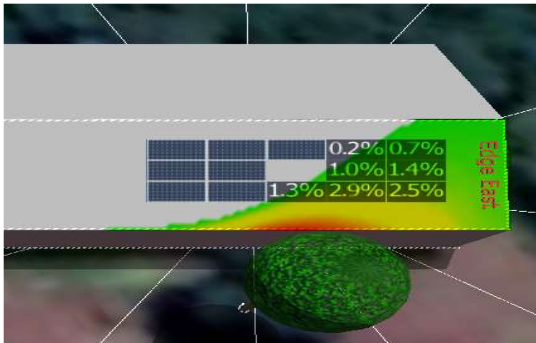
Figure 41: Shade simulation drawing
