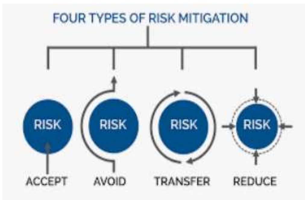
Figure 15: Risk Compliance
