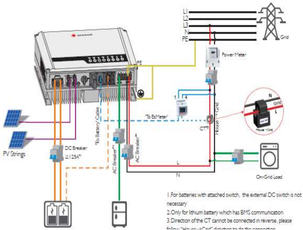
Figure 28: Good we ES Wiring
