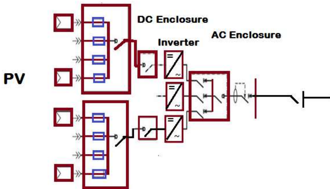
Figure 2: Single Line Diagram ( https://www.indiamart.com/ )
