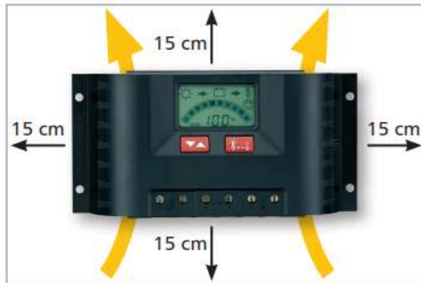
Figure 25: Steca CC mounting
