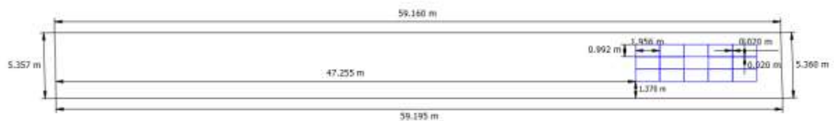
Figure 10: Roof layout diagram (PV SoL Software)
