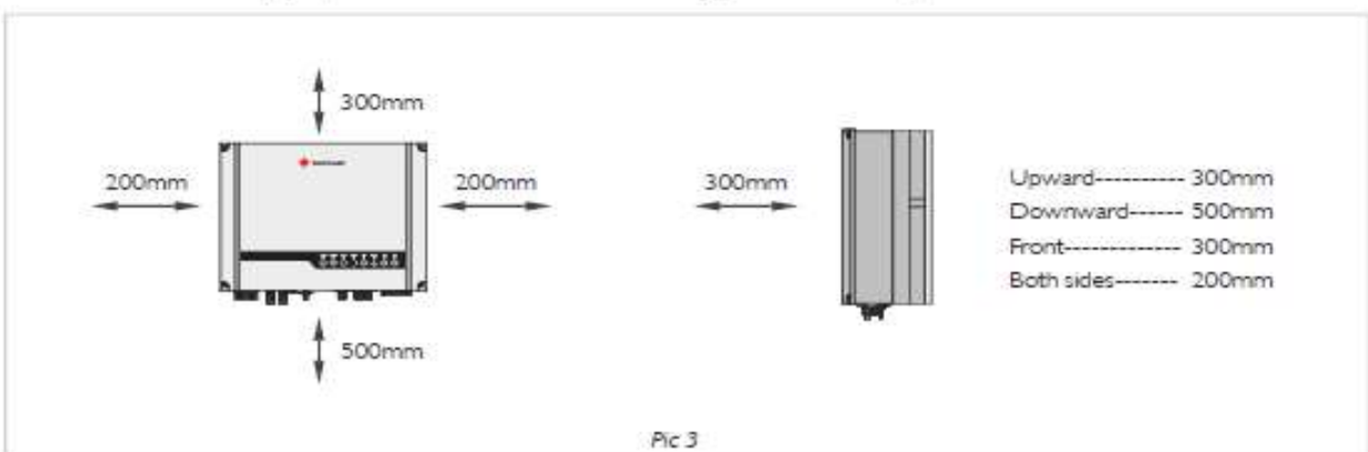
Figure 27: Inverter mounting (Good we ES)
