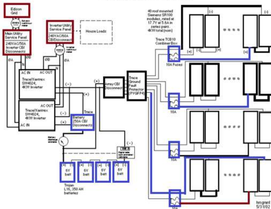
Figure 6: SLD example
