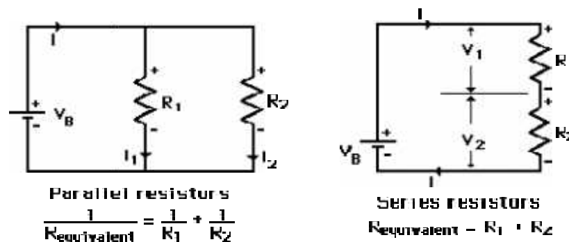
Fig 3.8 comparison of parallel and series circuit Series-parallel circuit
