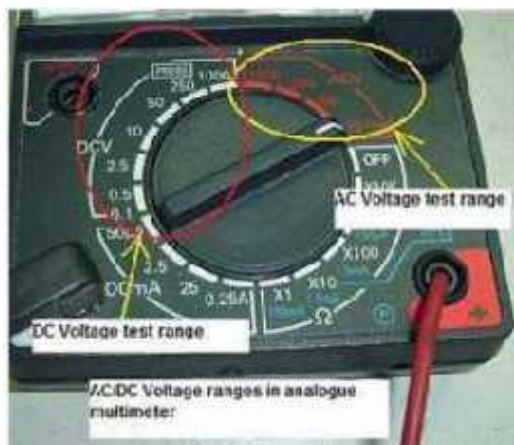
Fig 1.1 adjusting the range of voltmeter
