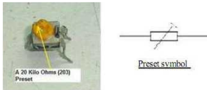
Fig 3.11 variable resistor preset symbol
