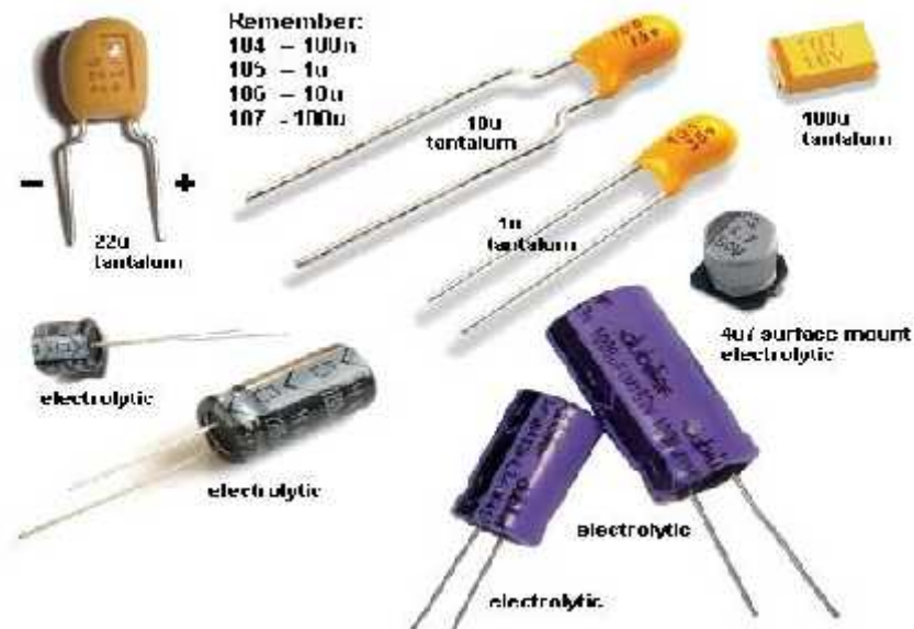
Fig3.13. different types of capacitors
