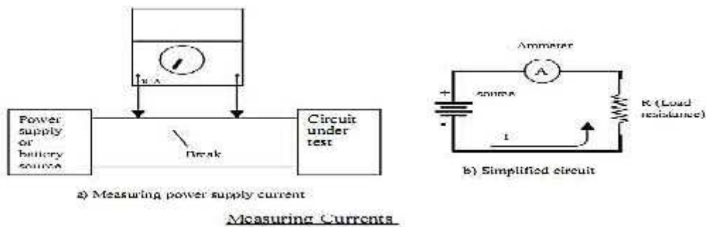
Fig 1.6 measuring current in a circuit
