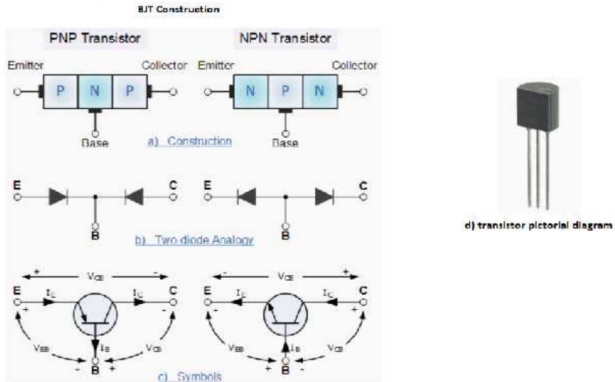
Fig 3.33 BJT construction
