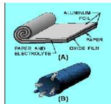
Electrolytic capacitor
