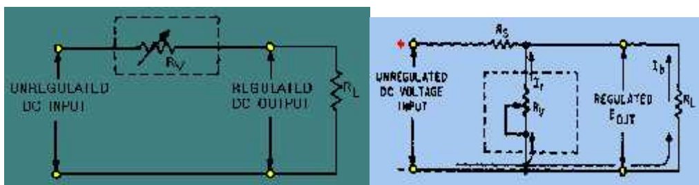
Figure - Series voltage regulator. Shunt voltage regulator
