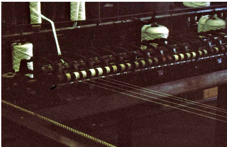
Figure 18. Worsted mule drafting rollers. Courtesy of the Bradford Industrial Museum. Photograph by Alan S. Raistrick.
