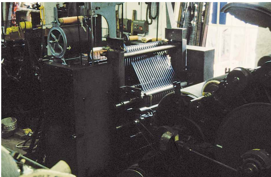
Figure 5. Tape Condenser. Courtesy of the Saddleworth Museum. Photograph by Alan S. Raistrick.
