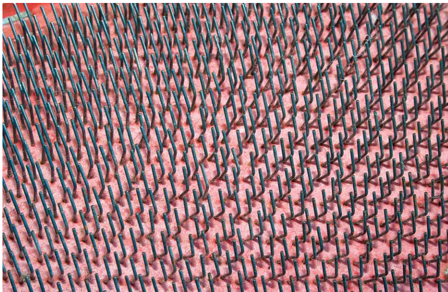
Figure 4. Modern Card Clothing. Photograph by Alan S. Raistrick.
