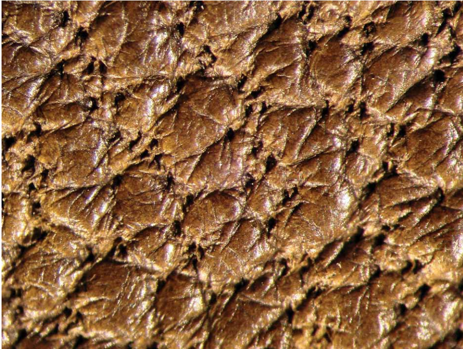
Figure 15. Grain surface of sheepskin leather. Photographed at X25 magnification. Photograph by Amanda Michel.
