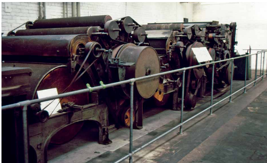
Figure 6. Carding engine. Courtesy of the Leeds Industrial Museum. Photograph by Alan S. Raistrick.
