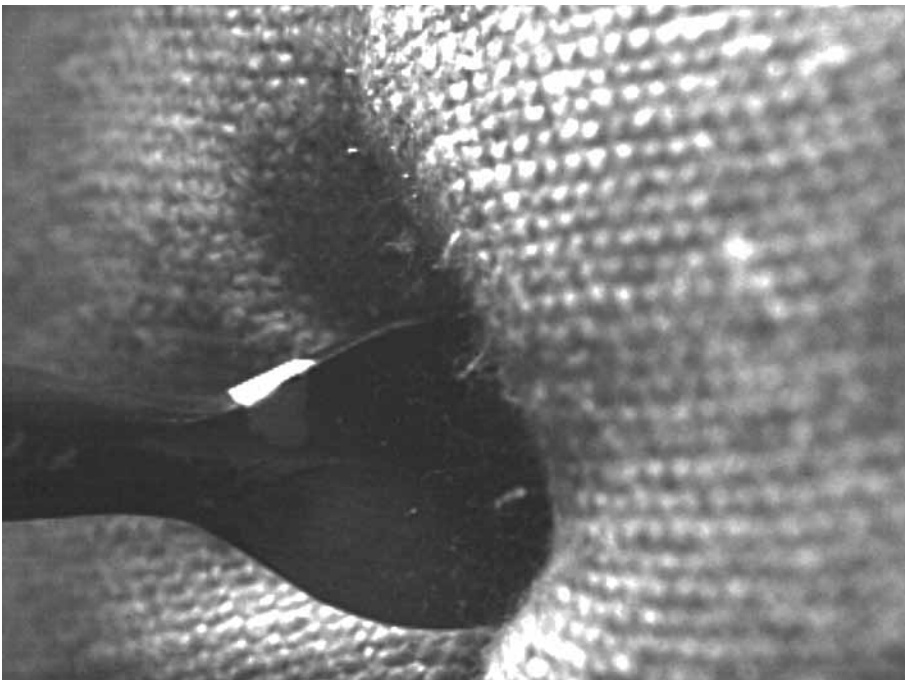
Figure 22. The arrowhead penetrating soft armour 07-06, 1.4 milliseconds after initial contact. The fabric is coming under tension and the fibres must be both absorbing strain energy and sliding across each other to admit the blade, which is nearly twice the width of the final slit in the top layer. Photograph by Edward Cheshire.
