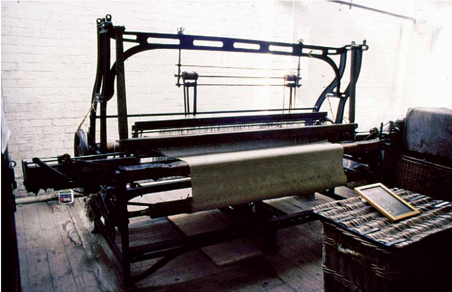
Figure 20. Basic early power loom. Courtesy of the Leeds Industrial Museum. Photograph by Alan S. Raistrick.
