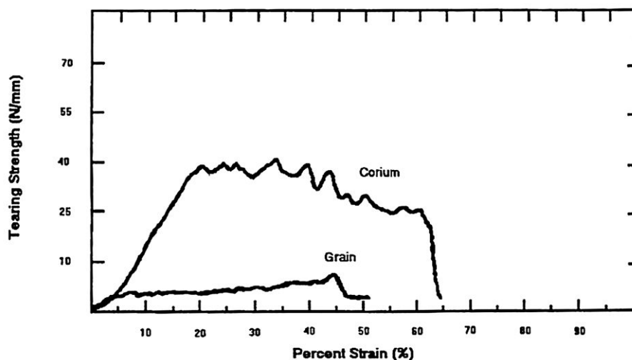
Figure 4. Graph showing the difference in tear strength between the grain and corium layers of leather. Courtesy of the University of Northampton.
