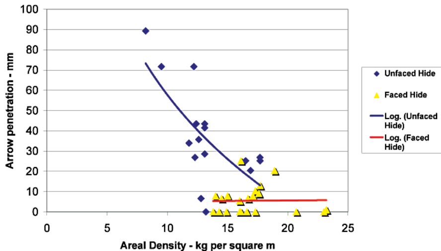
Figure 27. Graph of Penetration against Areal Density. Unfaced boiled rawhide and faced boiled rawhide.
