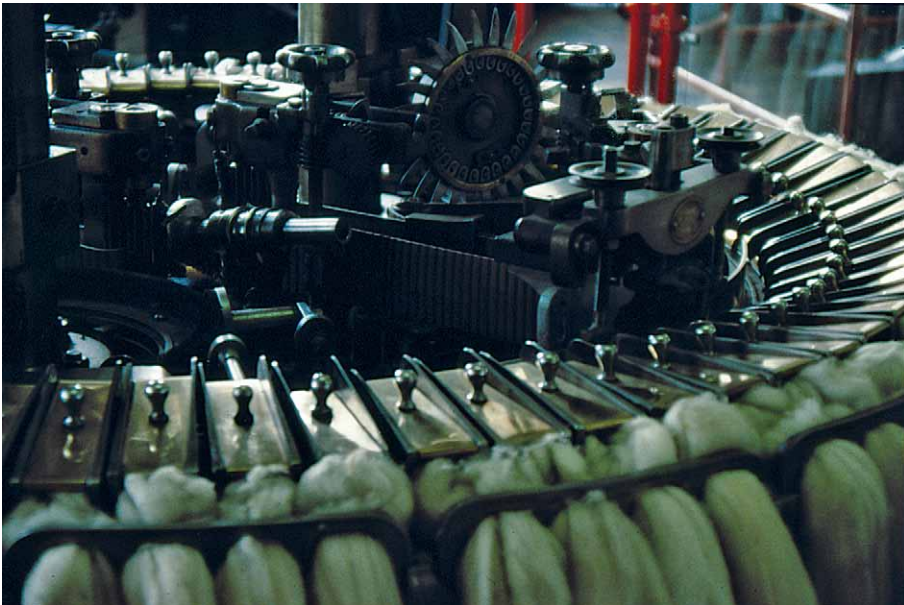
Figure 15. Noble comb with combing leathers just visible. Courtesy of the Bradford Industrial Museum. Photograph by Alan S. Raistrick.
