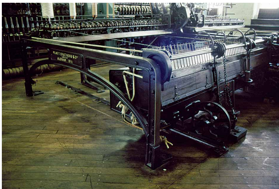
Figure 17. Worsted mule. Courtesy of the Bradford Industrial Museum. Photograph by Alan S. Raistrick.
