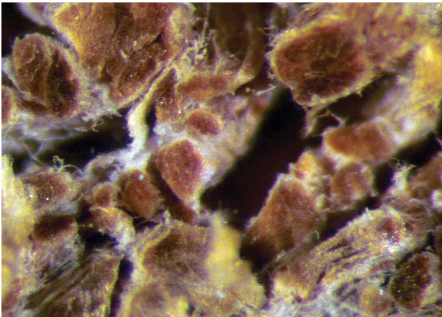
Figure 7. Photomicrograph of the cross section of the belly area of leather showing spaces between the fibre bundles. Photographed at X100. Photograph by Amanda Michel.
