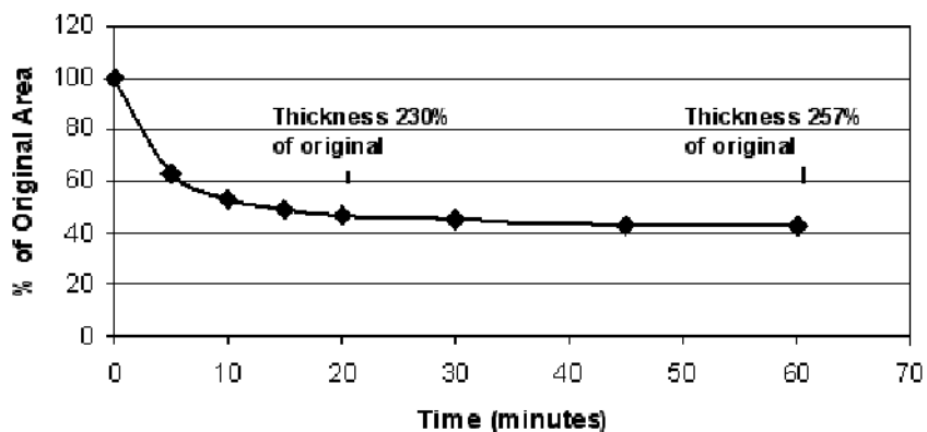
Figure 4. Areal shrinkage of 4.4 mm thick rawhide in boiling water. Diagram by Edward Cheshire.
