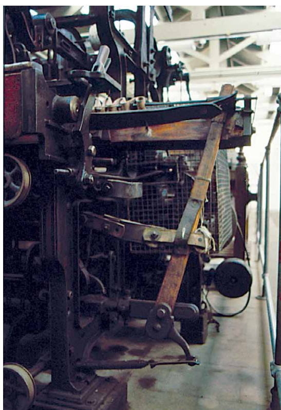
Figure 22. Under pick loom picking mechanism. Courtesy of the Bradford Industrial Museum. Photograph by Alan S. Raistrick.
