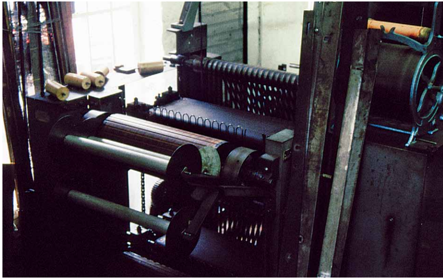
Figure 8. Tape condenser followed by a rubbing leather. Courtesy of the Saddleworth Museum. Photograph by Alan S. Raistrick.
