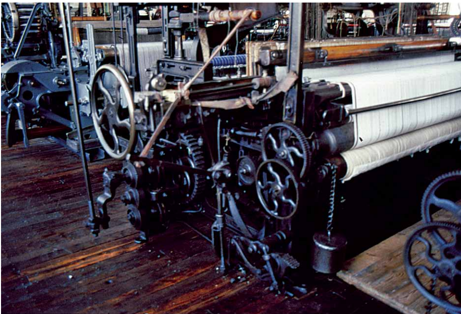
Figure 21. Over pick loom picking mechanism. Courtesy of the Bradford Industrial Museum. Photograph by Alan S. Raistrick.
