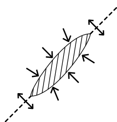
Figure 14. Simplified diagram of the stresses caused by a leaf shaped arrow penetrating into hide-based armour. By Erno Endenburg after Edward Cheshire.
