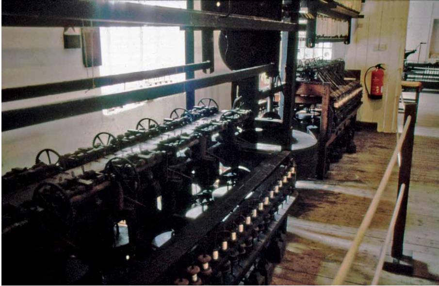
Figure 2. Throstle. Courtesy of the Helmshore Textile Museum. Photograph by Alan S. Raistrick.
