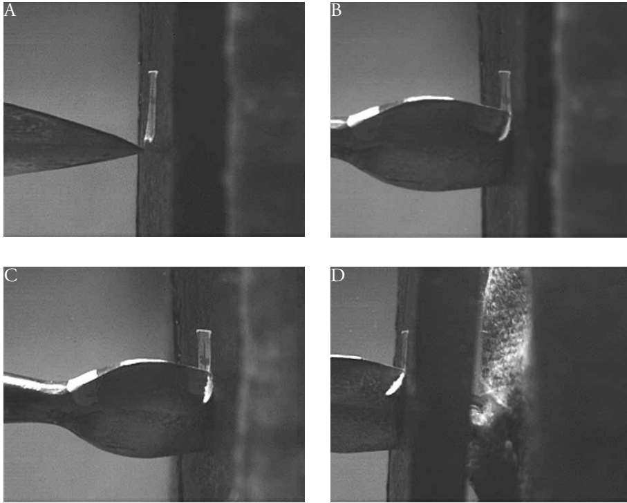
Figure 18. The impact at 36 m/sec and normal incidence of a mild steel headed arrow weighing about 70 grams on replicated rawhide cuir bouilli over an aketon. The small piece of paper is a photographic focusing aid. Photograph by Edward Cheshire.
