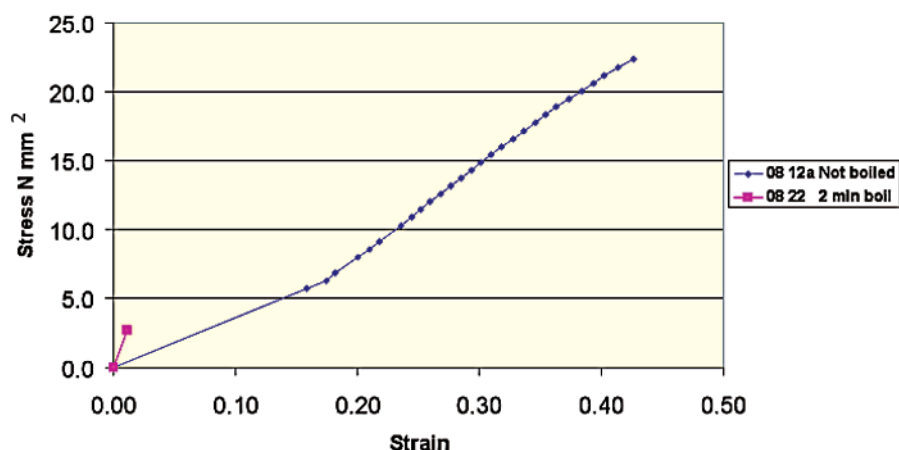
Figure 10. Sample Stress-Strain Graphs of leather (08-12a) and boiled leather (08-22).
