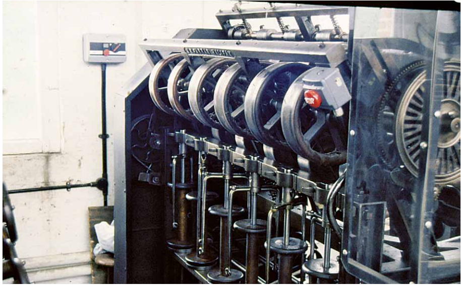
Figure 16. Halifax flyer frame. Courtesy of the Halifax Industrial Museum. Photograph by Alan S. Raistrick.
