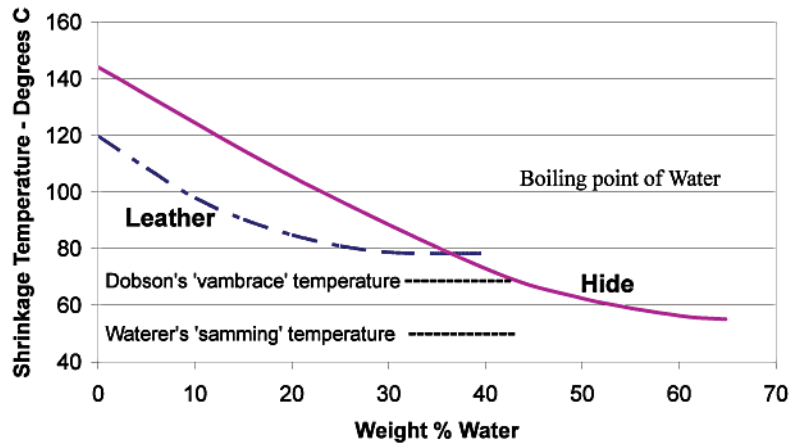
Figure 2. Graph of shrinkage temperature against water content. From: Witnauer, 1960: 441-151.
