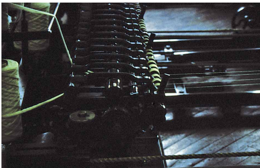
Figure 19. Close-up of the worsted mule drafting rollers. Courtesy of the Bradford Industrial Museum. Photograph by Alan S. Raistrick.
