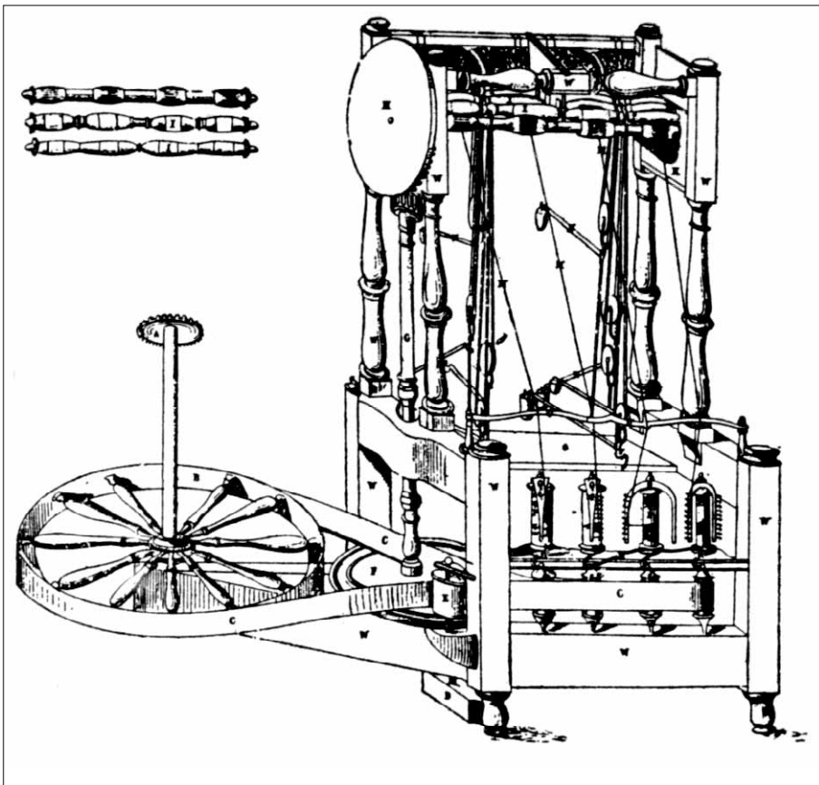
Figure 1. Arkwright's Patent spinning machine (English Patent No. 931,1769, R. Arkwright, 1769).
