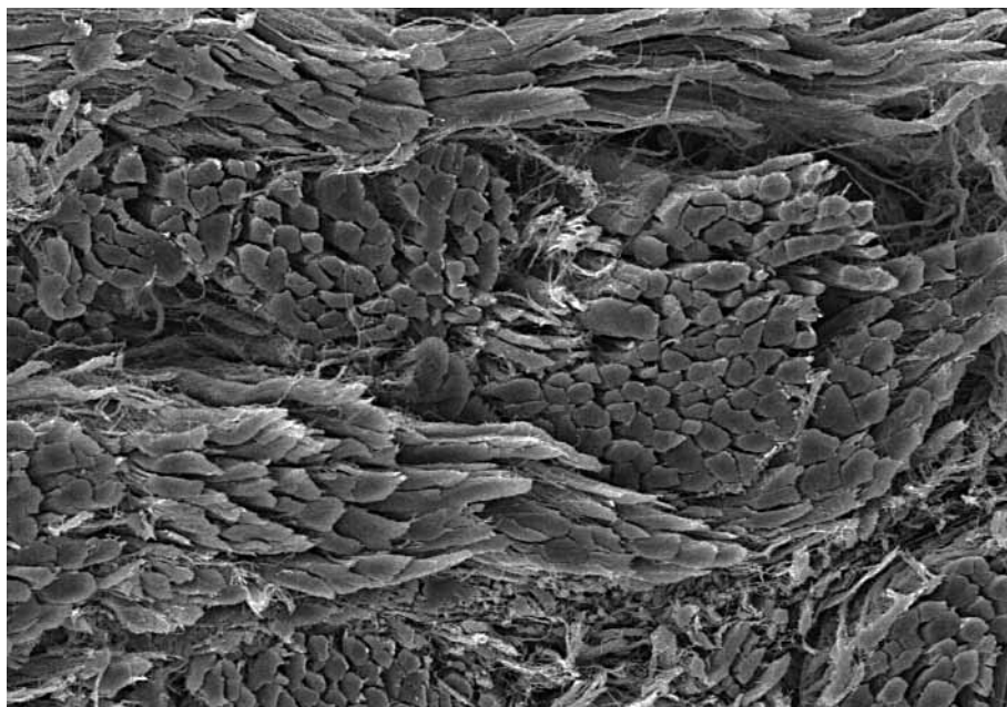
Figure 3. Section through vegetable tanned leather showing fibrous structure and the voids which cause porosity. Magnification X500.
