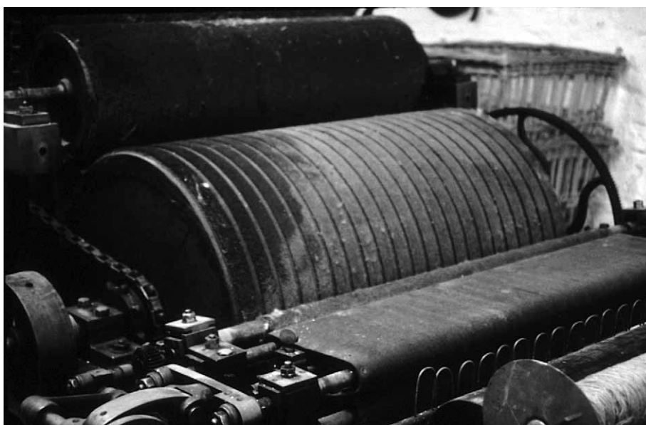
Figure 7. Ring doffer followed by a rubbing leather. Courtesy of the Saddleworth Museum. Photograph by Alan S. Raistrick.
