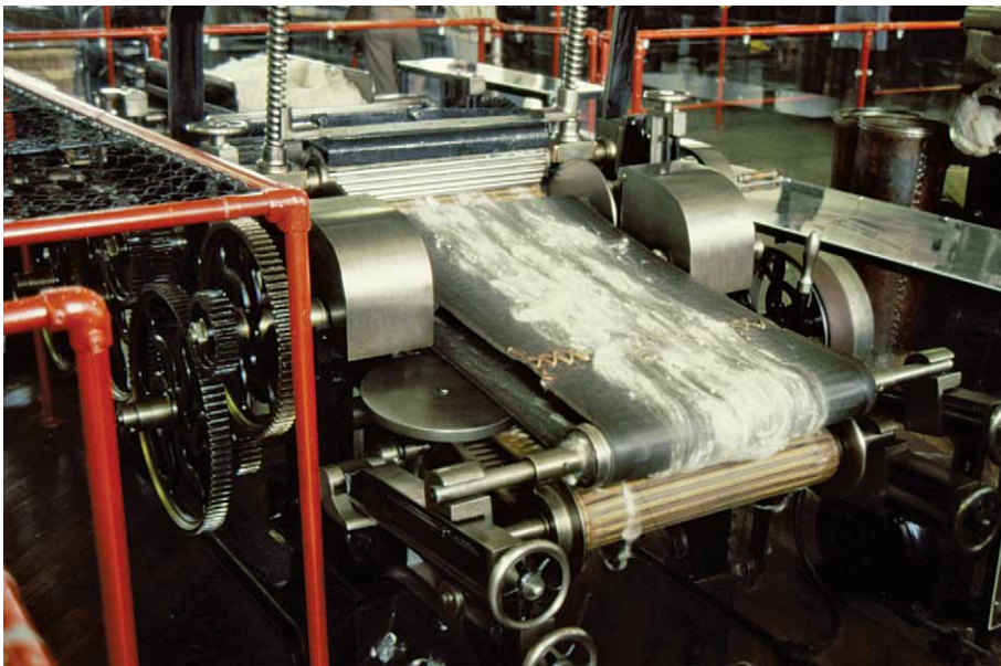
Figure 12. Preparer feed. Courtesy of the Bradford Industrial Museum. Photograph by Alan S. Raistrick.
