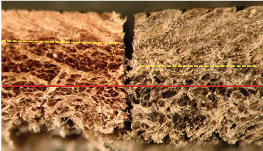
Figure 14. Cross sections of calf leather (left) and adult cattle leather (right) showing differences in grain layer depth resulting in more corium layer remaining after splitting to the desired thickness. Grain layer depth indicated in yellow. Splitting level indicated in red. Photographed at X25 magnification. Photograph by Amanda Michel.
