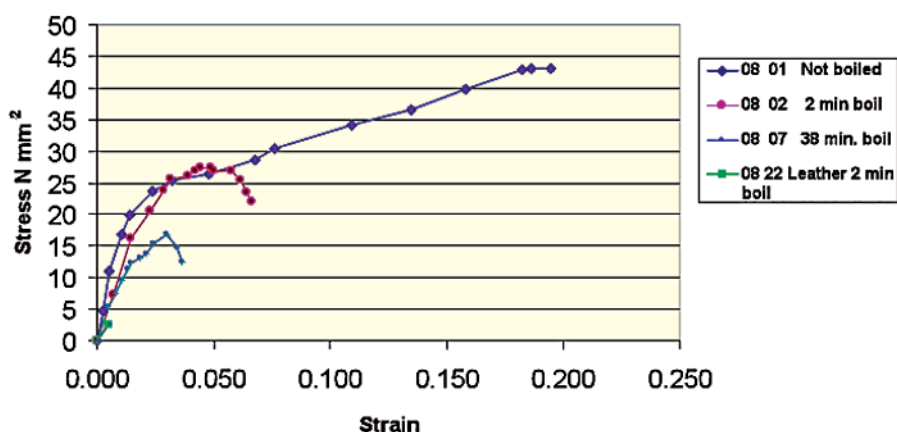
Figure 11. Sample Stress-Strain Graphs of natural rawhide (08-01), boiled rawhide (08-02 and 08-07) and boiled leather (08-22).
