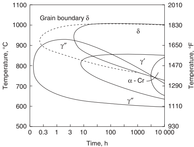
Figure 4.12 TTT diagram for Alloy 718. (From Brooks and Bridges [11])
