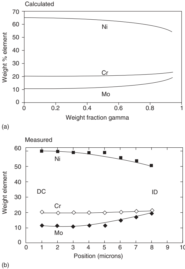
Figure 2.21 Calculated (a) and measured (b) distribution of alloying elements expected to exist across the dendritic substructure of the weld for Ni, Cr, and Mo for Alloy C-22. (From DuPont et al. [33])
