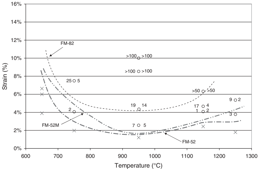
Figure 3.49 Strain-to-fracture tests results for Filler Metals 82, 52 and 52M. The “X” symbols represent no cracks and the “O” symbols represent cracking at a given temperature-strain combination. The lines indicate the threshold strain for fracture for each weld metal and the numbers represent the number of cracks observed. (From Lippold and Nissley [98].)
