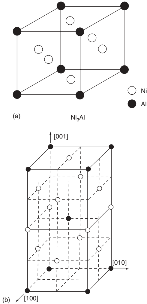
Figure 2.1 a) Crystal structure of the \gamma' - \text{Ni}_3(\text{Ti},\text{Al}) ordered FCC phase (Courtesy ASM International from [4]), b) Crystal structure of the \gamma' - \text{Ni}_3\text{Nb} phase. (From Sundaraman and Mukhopadhyay [8])
