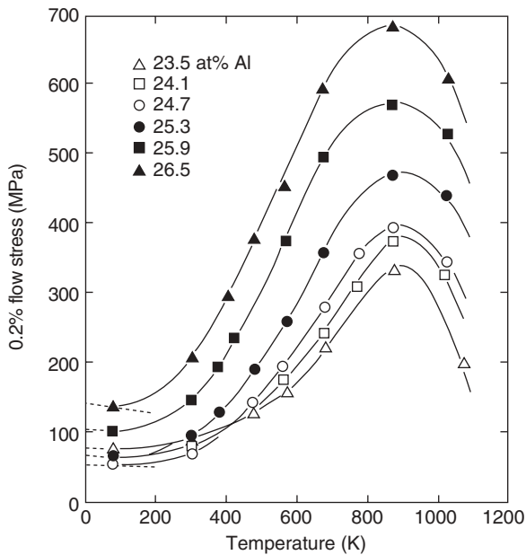
Figure 5.11 Effect of Al content on the flow stress of \text{Ni}_3\text{Al} alloys as a function of temperature. (From Noguchi et al. [18])
