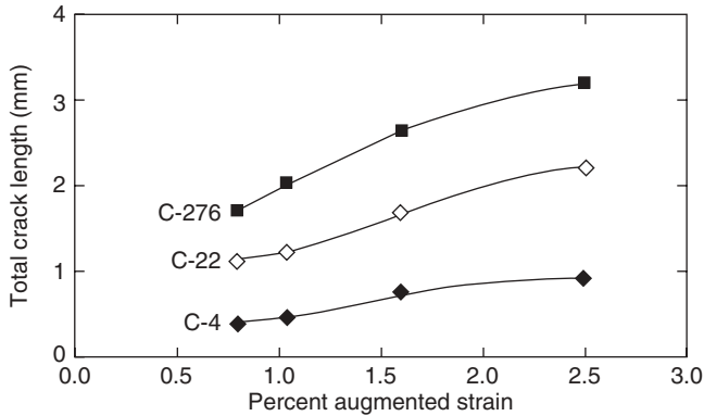
Figure 3.29 Varestraint weldability results for Alloys C-4, C-22, and C-276. (From Cieslak et al. [6].)
