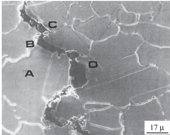
Figure 3.39 Photomicrograph showing evidence of grain boundary liquation (arrows) in the HAZ of Alloy 617. (From Lundin et al. [75].)
