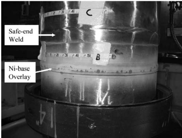
Figure 7.31 Dye penetrant indications in Filler Metal 52M overlay on Type 316L stainless steel. (From Smith [51])
