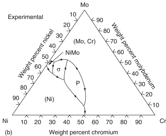
Figure 2.18 Liquidus projections for the ternary Ni-Cr-Mo system, a) calculated projection, b) experimentally determined projection. (From Perricone et al. [31])
