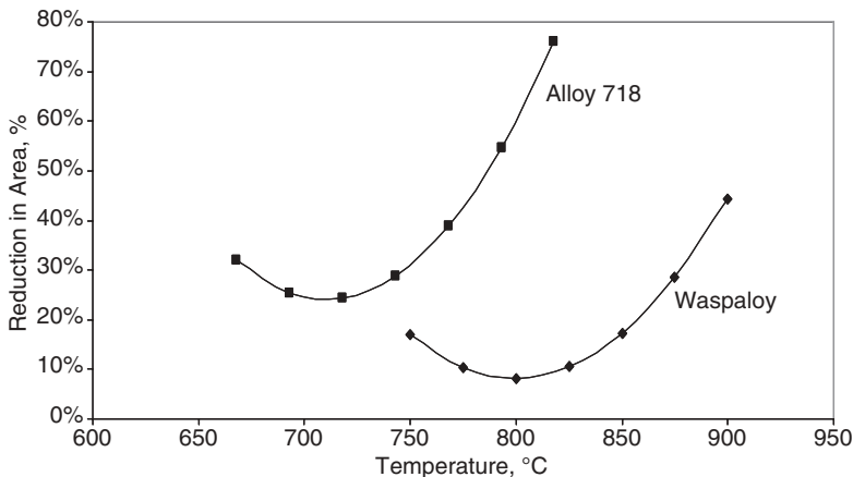
Figure 4.64 Postweld heat treatment ductility curves for Waspaloy, and Alloy 718 after three hours of aging following a simulated HAZ thermal cycle. (From Norton and Lippold [92]).
