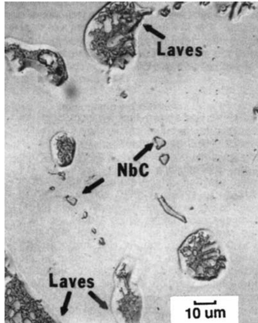
Figure 3.40 Example of HAZ liquation in a Ni-base alloy containing NbC carbide and Laves phase. (From Kelly [74].)
