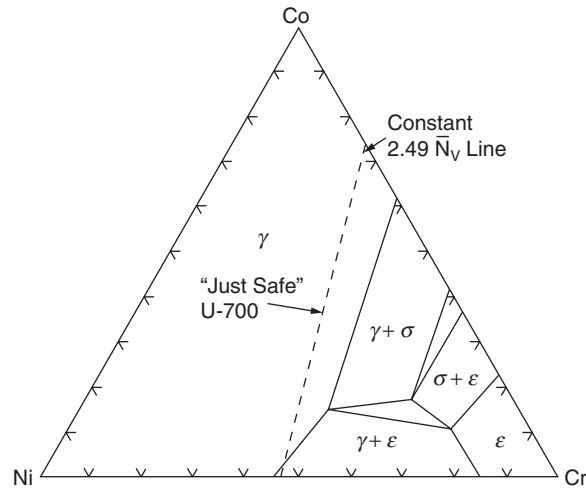
Figure 2.24 Constant N_v = 2.49 line corresponding approximately to the position of the \gamma/(\gamma + \sigma) phase boundary line for Alloy U-700 in the Ni-Co-Cr system. (From Sims [11])
