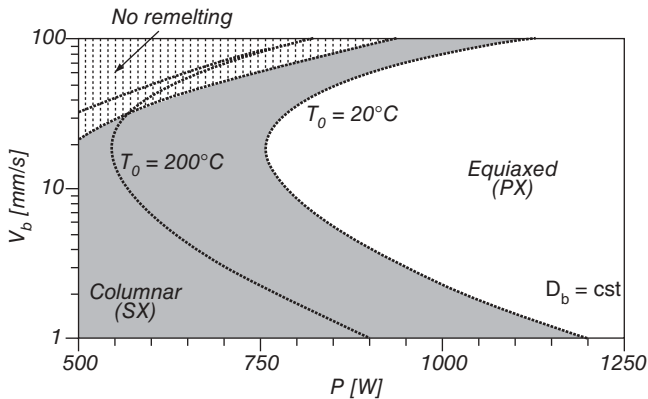
Figure 6.18 Process-microstructure map for Alloy CMSX-4 that reveals the semi-quantitative relations between heat source travel speed ( V_b ), power ( P ), and preheat temperature ( T_0 ) and the type of dendrite growth. (From Gauman et al. [27])
