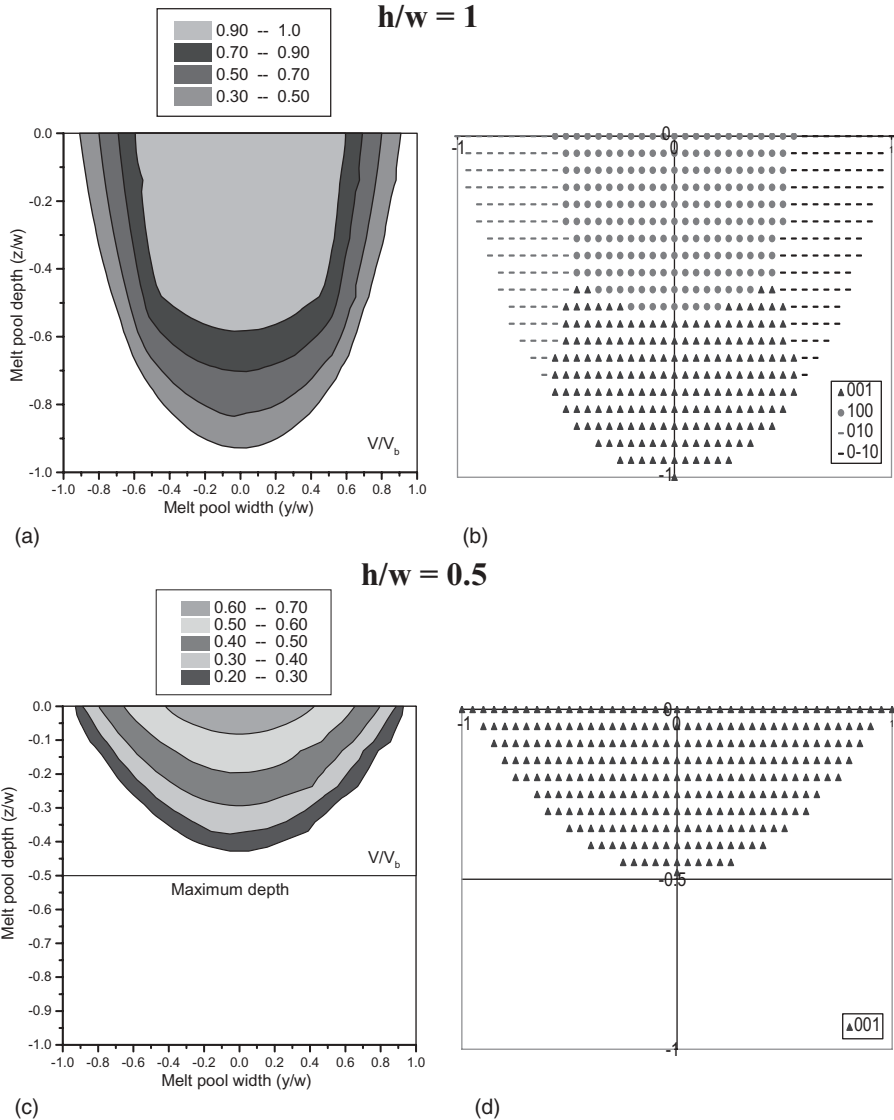
Figure 6.24 Computational results showing ratio of dendrite growth velocity to beam velocity (a and c) and active dendrite growth directions (b and d) as a function of position in the melt pool for two different melt pool shapes. a and b) h/w = 1 , c and d) h/w = 0.5 .
