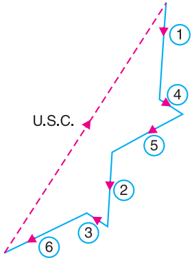
(g) Secondary couple polygon.
