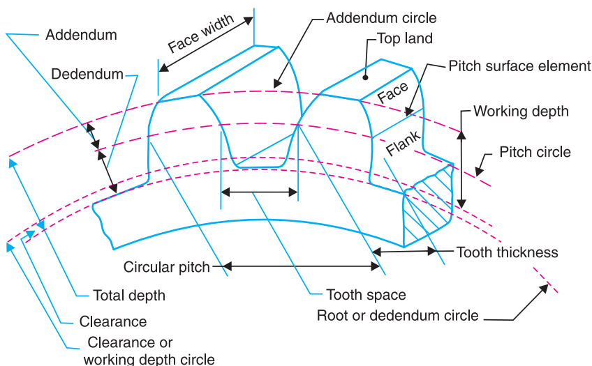
Fig. 12.5. Terms used in gears.
