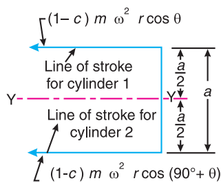
Fig. 22.5. Swaying couple.
