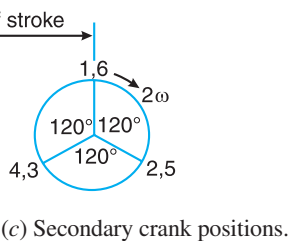
(c) Secondary crank positions.
