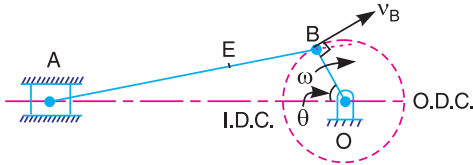
(a) Slider crank mechanism.
