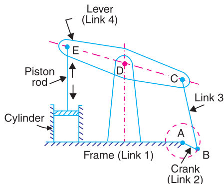
Fig. 5.19. Beam engine.
