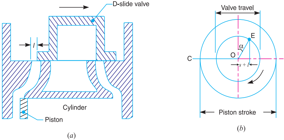
Fig. 17.3. Piston slide valve.
