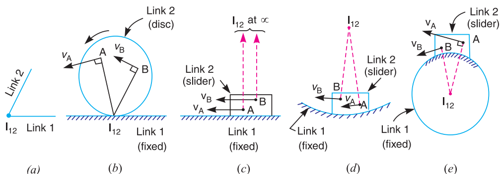
Fig. 6.6. Location of instantaneous centres.
