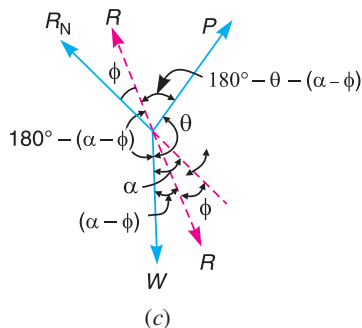
Fig. 10.9. Motion of the body down the plane, considering friction.
