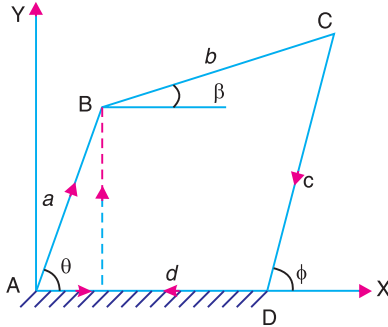
(a) Four bar mechanism.
