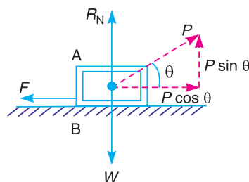
Fig. 10.4. Minimum force required to slide a body.
