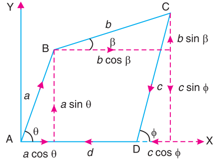
(b) Components along X -axis and Y -axis.
