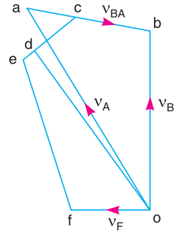
(b) Velocity diagram.
