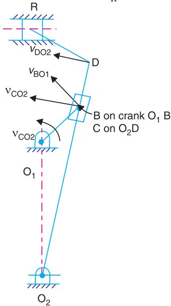
(a) Space diagram
