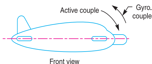
Fig. 14.5. Aeroplane taking a left turn.
