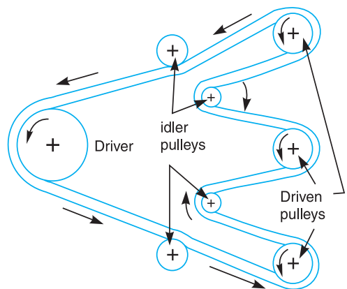
(b) Belt drive with many idler pulleys.
