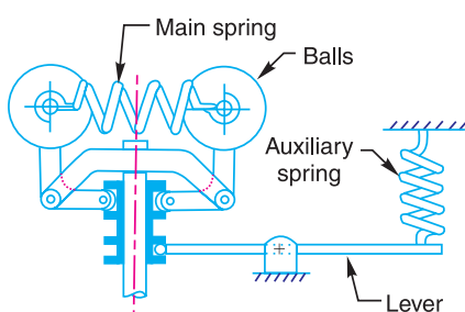
Wilson-Hartnell governor.
