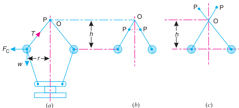
Fig. 18.2. Watt governor.
