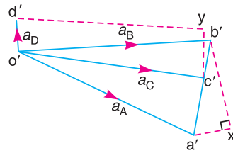
(c) Acceleration diagram.
