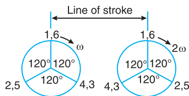
(b) Primary crank positions.
