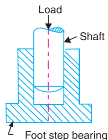
Fig. 5.5. Shaft in a foot step bearing.
