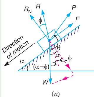
Fig. 10.9. Motion of the body down the plane, considering friction.
