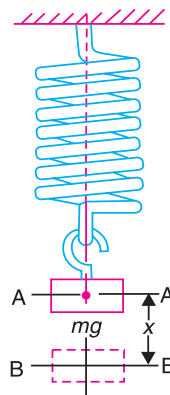
Fig. 4.4. Closely-coiled helical spring.
