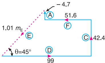
(c) Couple polygon : Driving wheel E .
