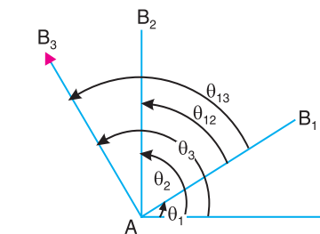
(a) Three positions of the crank.
