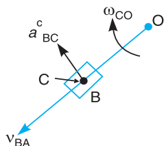
(a) Space diagram.
