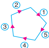
(f) Secondary force polygon.
