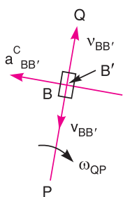
(c) Direction of coriolis component.
