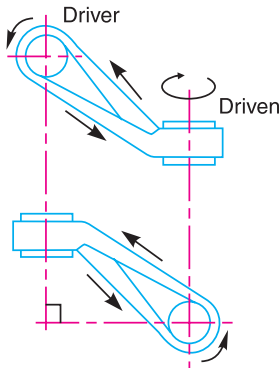
(a) Quarter turn belt drive.
