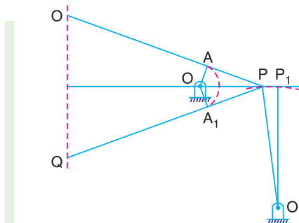
Fig. 9.8. Grasshopper mechanism.
