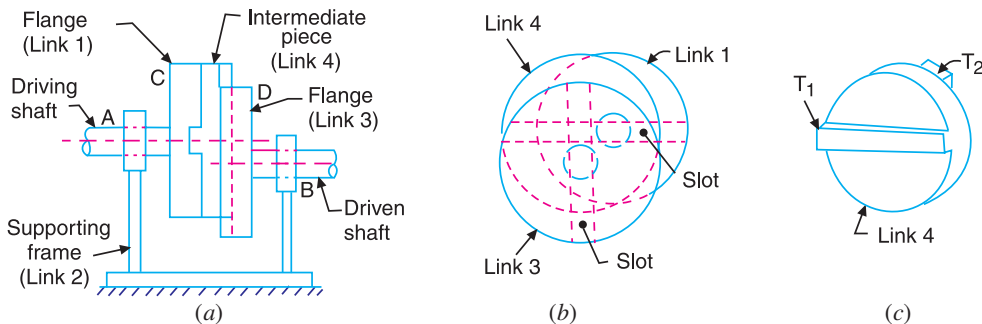
Fig. 5.36. Oldham's coupling.
