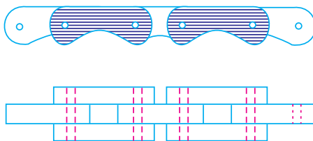
Fig. 11.31. Block chain.
