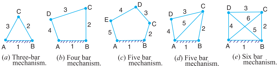
Fig. 5.16. Plane mechanisms.
