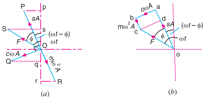
Fig. 23.20. Graphical method.
