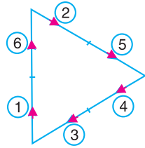
(e) Secondary force polygon.
