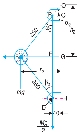
(b) Maximum position.
