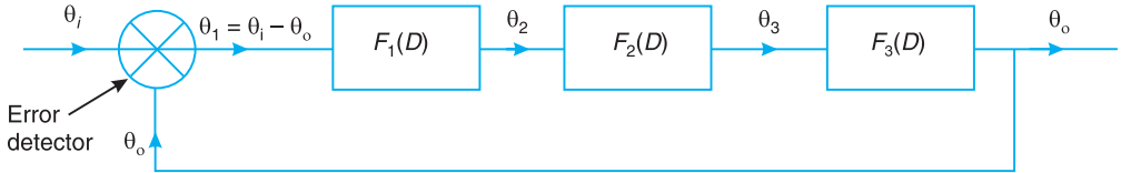
Fig 26.9 Closed-loop transfer function.
