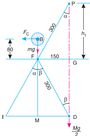
(a) Minimum position.
