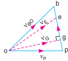
(b) Velocity diagram.
