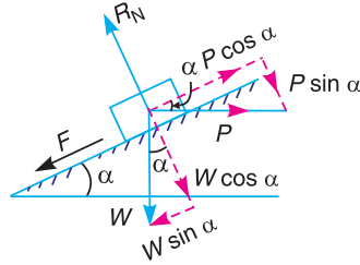
(b) Forces acting on the screw.
