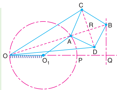
Fig. 9.3. Peaucellier mechanism.
