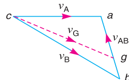
(b) Velocity diagram.
