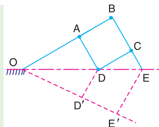
Fig. 9.1. Pantograph.
