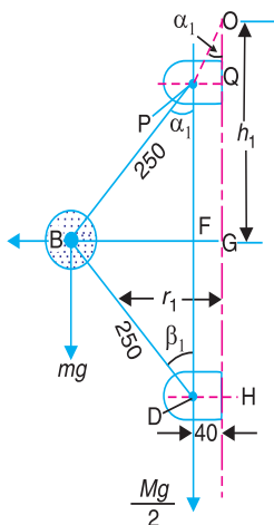
(a) Minimum position.
