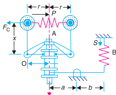
Line diagram of Wilson-Hartnell governor.
