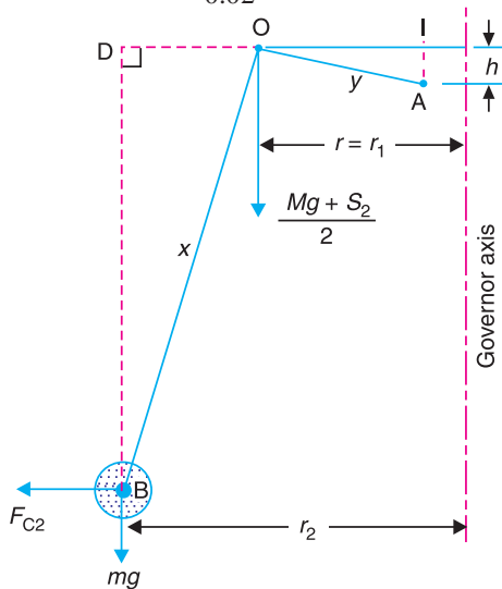
(b) Maximum position.
