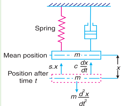
Fig. 23.19. Frequency of under damped forced vibrations.
