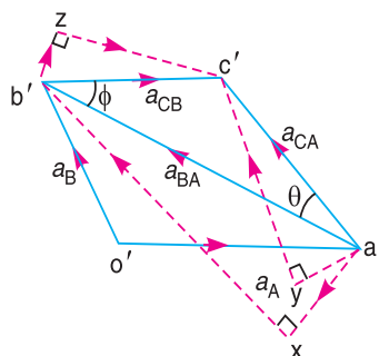
(b) Acceleration diagram.
