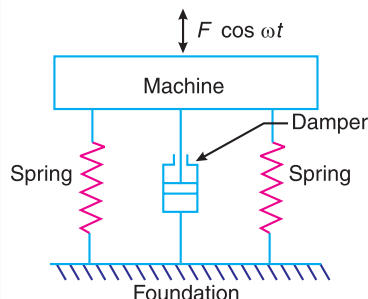
Fig. 23.22. Vibration isolation.
