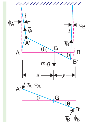
Fig. 4.9. Bifilar suspension.
