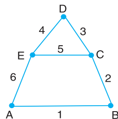
Fig. 5.11. Kinematic chain having binary and ternary joints.
