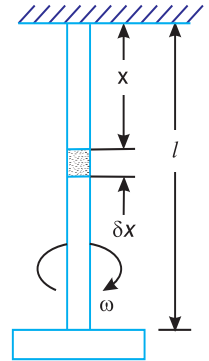
Fig 24.3. Effect of inertia of the constraint on torsional vibrations.
