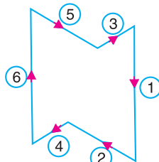
(g) Secondary couple polygon.
