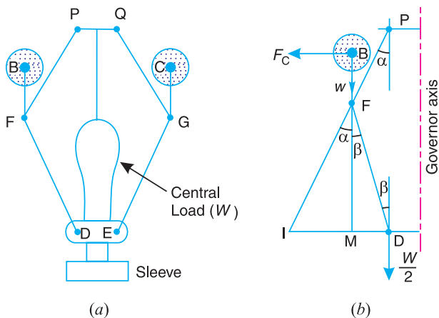
Fig. 18.12. Proell governor.
