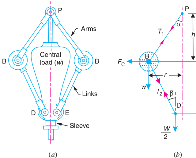
Fig. 18.3. Porter governor.
