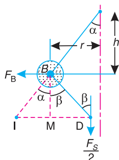
(a) Porter governor.
