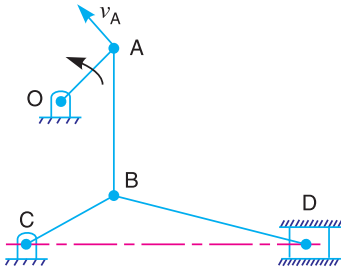
(a) Space diagram.
