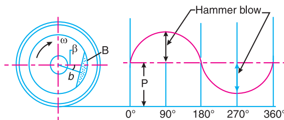
Fig. 22.6. Hammer blow.
