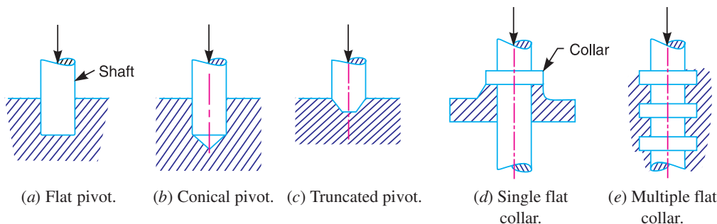
Fig. 10.16. Pivot and collar bearings.
