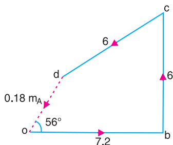
(c) Force polygon.
