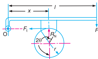
(b) Anticlockwise rotation of brake wheel.
