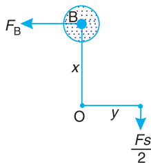
(b) Spring loaded governor.
