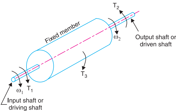
Fig. 13.25. Torques in epicyclic gear trains.
