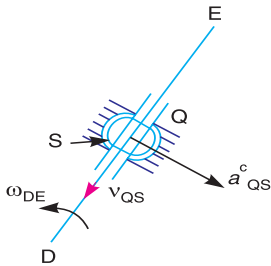
(c) Direction of coriolis component.
