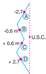
(g) Secondary couple polygon.
