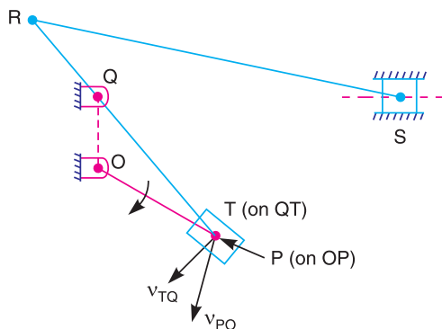
(a) Space diagram.
