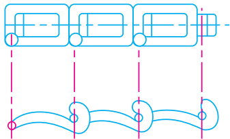
(a) Detachable or hook joint type chain.
