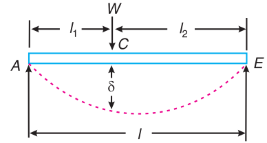
Fig. 23.6. Simply supported beam with a point load.
