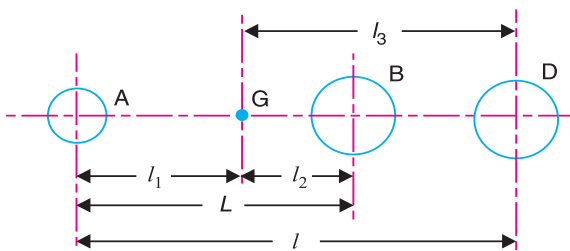
Fig. 15.21. Correction couple to be applied to make the two-mass system dynamically equivalent.
