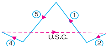
(g) Secondary couple polygon.
