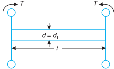
(b) Torsionally equivalent shaft.
