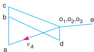
(b) Velocity diagram.
