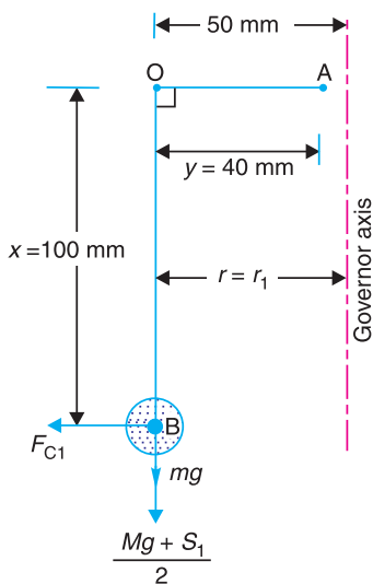
(b) Minimum position.
