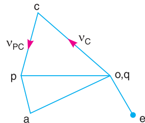
(b) Velocity diagram.
