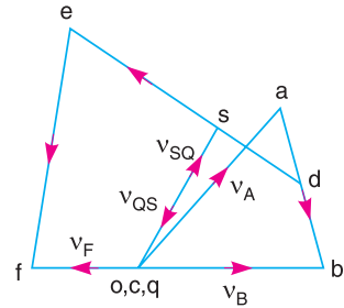
(b) Velocity diagram.
