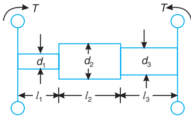
(a) Shaft of varying diameters.
