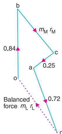
(e) Force polygon.
