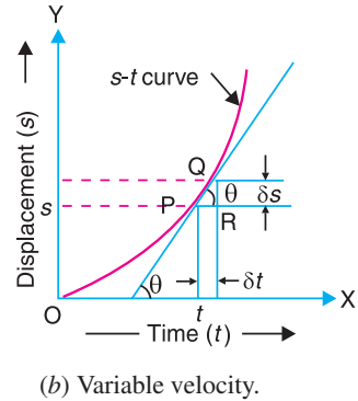
Fig. 2.1. Graphical representation of displacement with respect to time.
