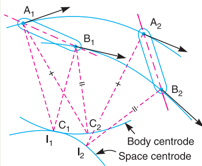
Fig. 6.3. Space and body centroide.
