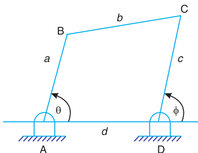
(a) Four bar mechanism.
