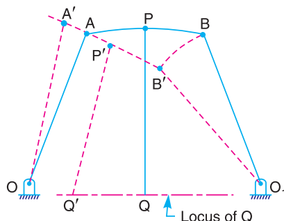
Fig. 9.10. Roberts mechanism
