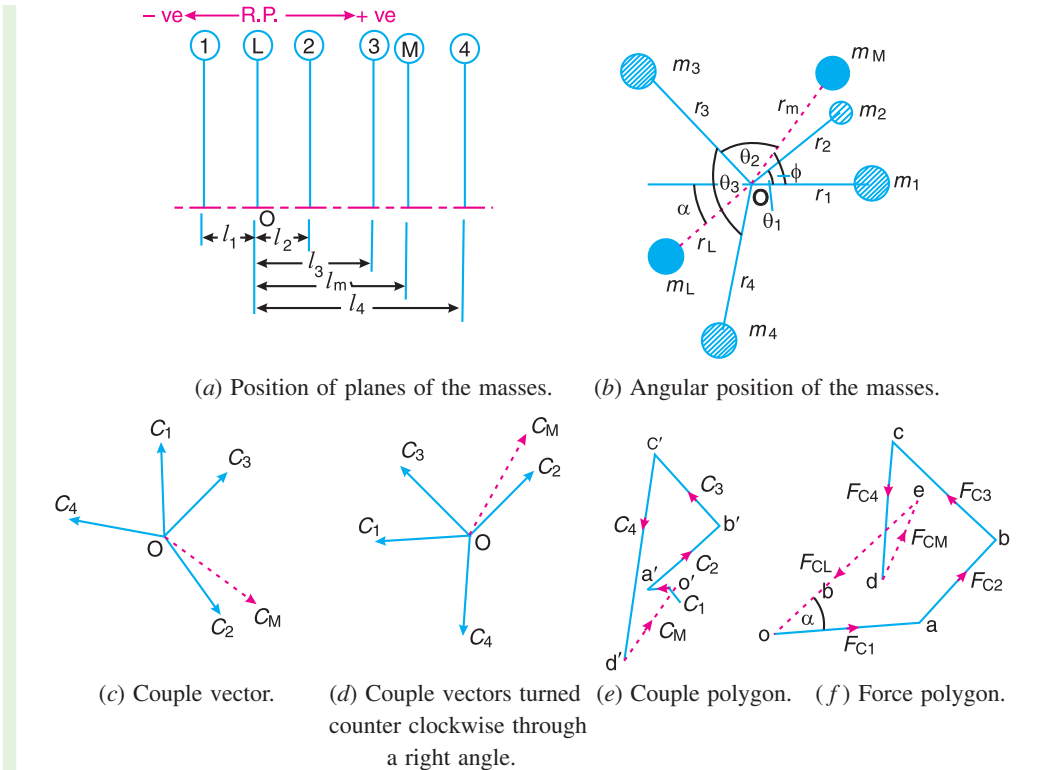
Fig. 21.7. Balancing of several masses rotating in different planes.
