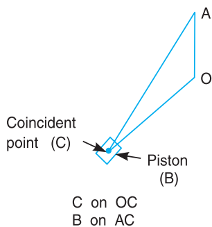
(a) Space diagram.
