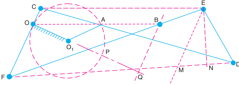
Fig. 9.4. Hart's mechanism.
