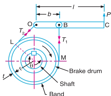
(a) Clockwise rotation of drum.
