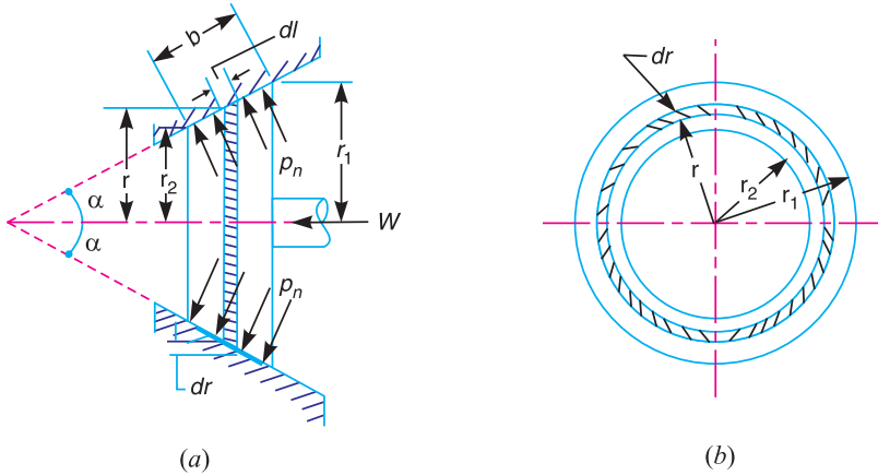
Fig. 10.25. Friction surfaces as a frustum of a cone.
