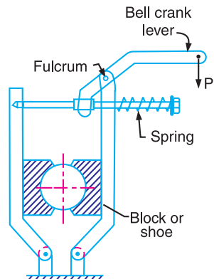
Fig. 19.9. Double block or shoe brake.
