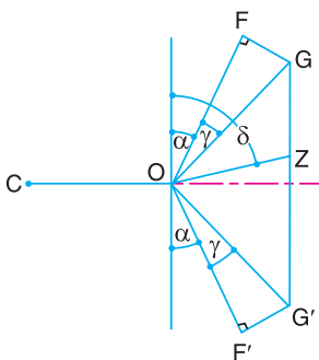
(a) For open rod arrangement
