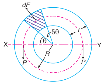
Fig. 16.17. Rim of a flywheel.
