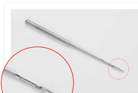
A Ballpoint Needle has a rounded point and slides between the material instead of piercing the yarn. It is used mainly for lingerie fabrics and knitted or stretch fabrics such as jersey. The rounded point reduces the possibility of holes and runs.
