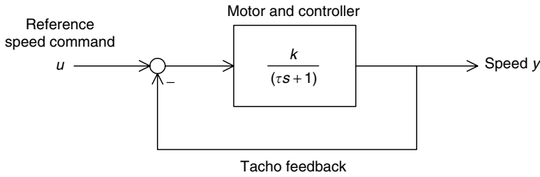
FIGURE P3.24 DC motor speed control system.
