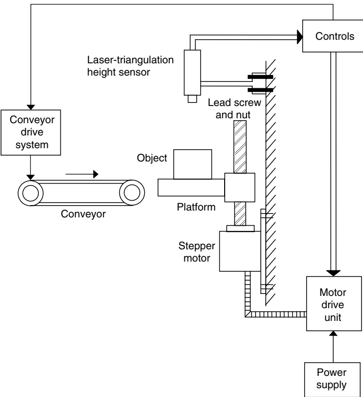
FIGURE P6.37 A material transfer unit in an automated factory.
