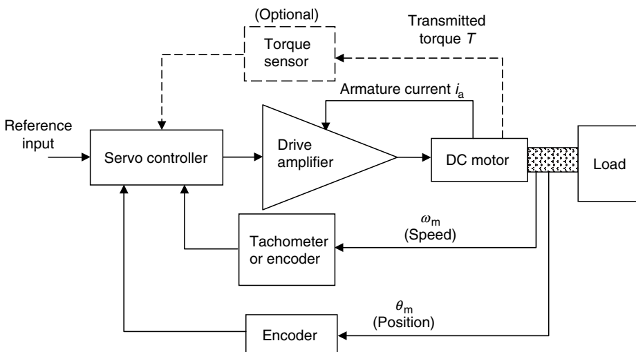
FIGURE 7.15 A dc servomotor system.
