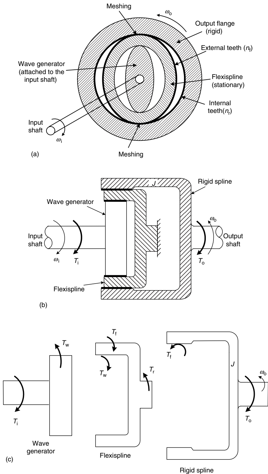
FIGURE 8.7 (a) An alternative design of harmonic drive. (b) Torque and speed transmission of the harmonic drive. (c) Free-body diagrams.
