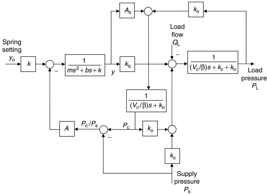
FIGURE 7.65 Block diagram for the single-stage pressure control valve.
