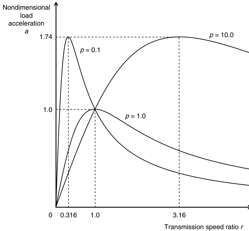
FIGURE 2.6 Normalized acceleration vs. speed ratio.
