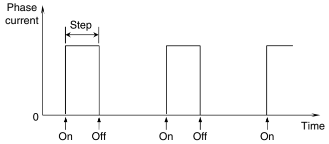
FIGURE P6.17 Ideal phase current waveform for a stepper motor.
