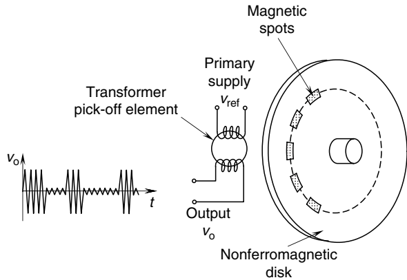
FIGURE 5.2 Schematic representation of a magnetic encoder.
