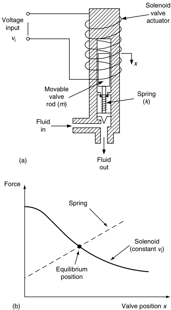
FIGURE P7.48 (a) A solenoid-actuated flow control valve. (b) Steady-state characteristics of the valve.
