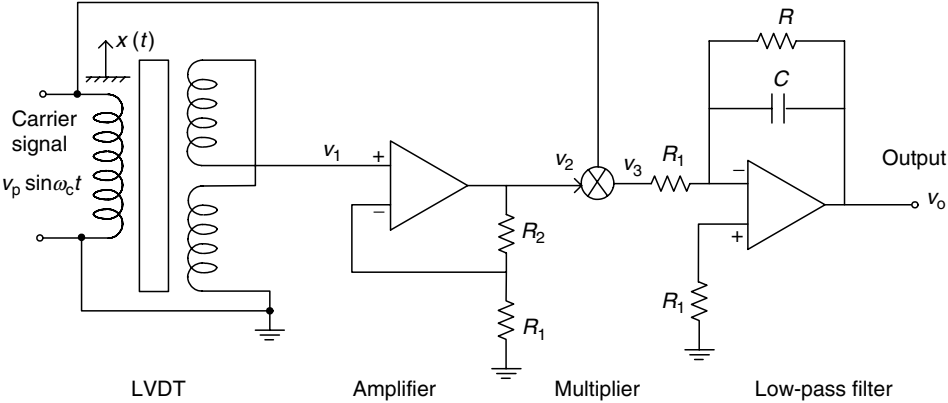
FIGURE 4.12 Signal-conditioning system for an LVDT.
