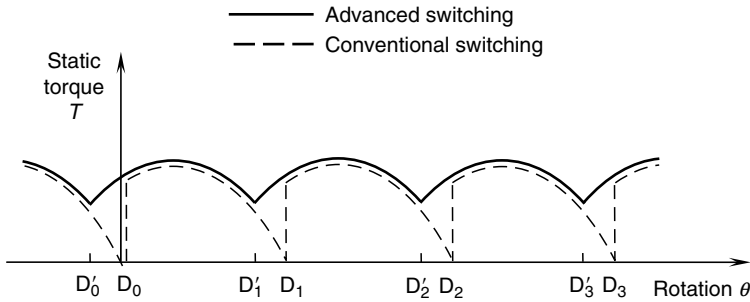
FIGURE 6.38 The effect of advancing the switching pulses.
