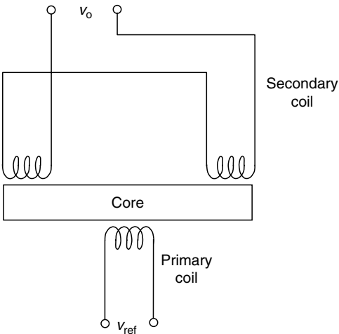
FIGURE 4.9 Series opposition connection of secondary windings.
