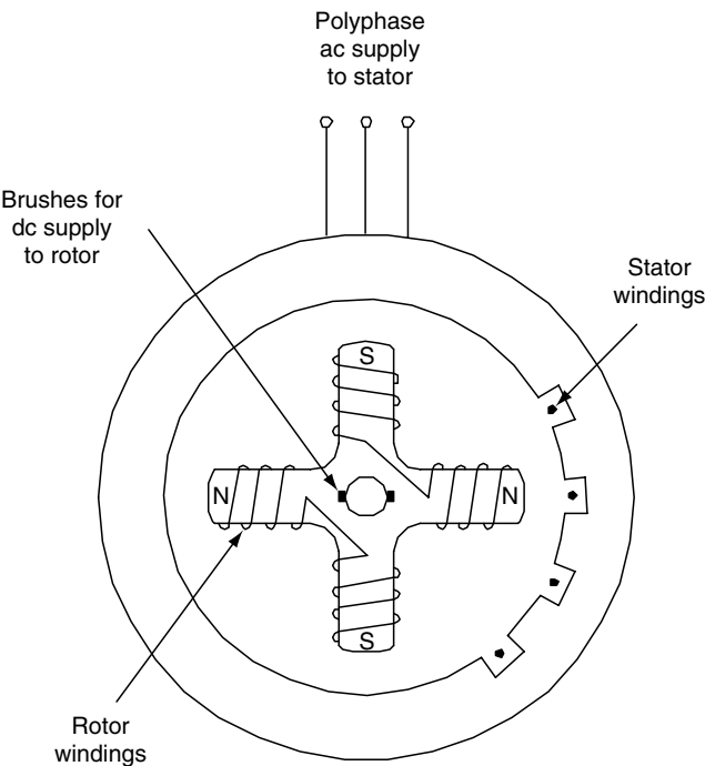
FIGURE 7.50 Schematic diagram of a stator-rotor configuration of a synchronous motor.
