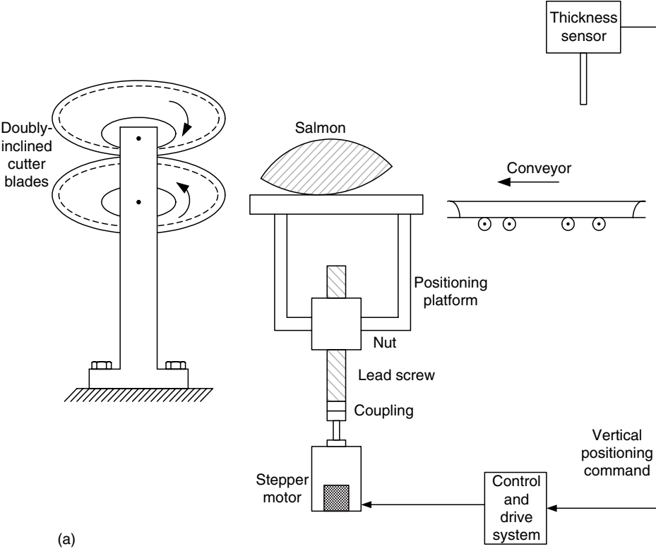
FIGURE P6.36 (a) An automated fish cutting system.
