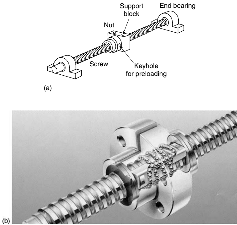
FIGURE 8.2 (a) A lead-screw and nut unit. (b) A commercial ball-screw unit. (Deutsche Star GmbH. With permission.)
