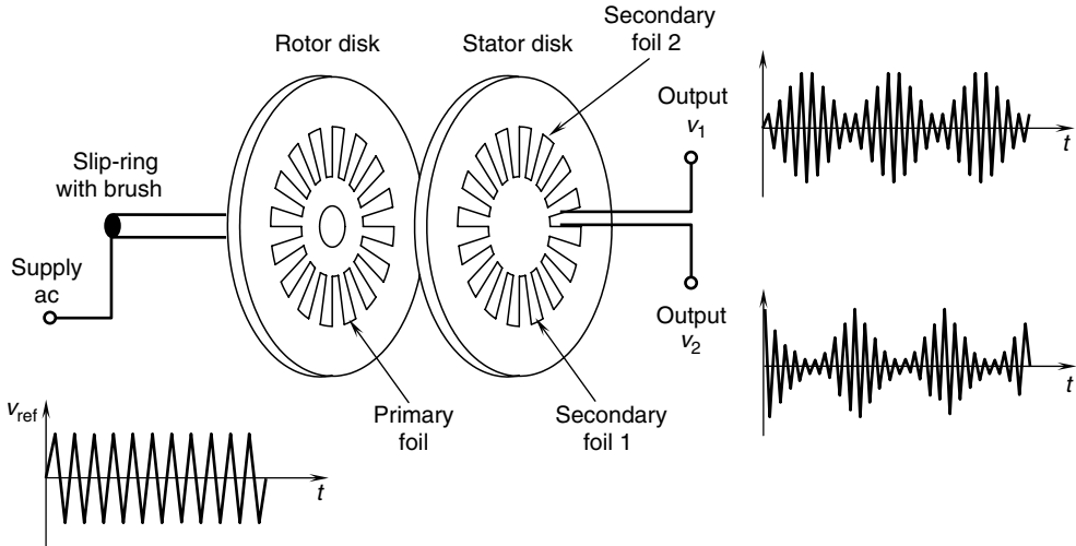
FIGURE 5.12 Schematic diagram of a digital resolver.
