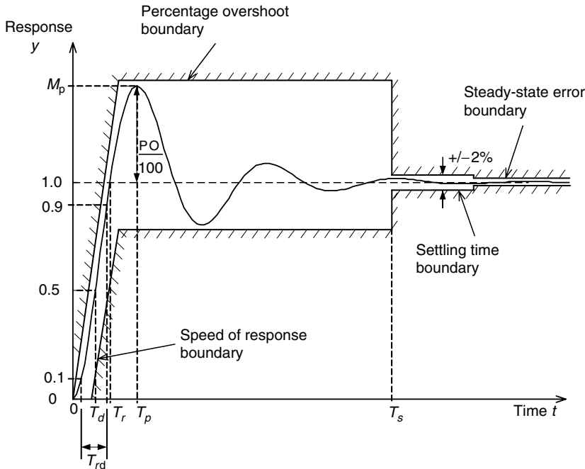
FIGURE 3.1 Response parameters for time-domain specification of performance.
