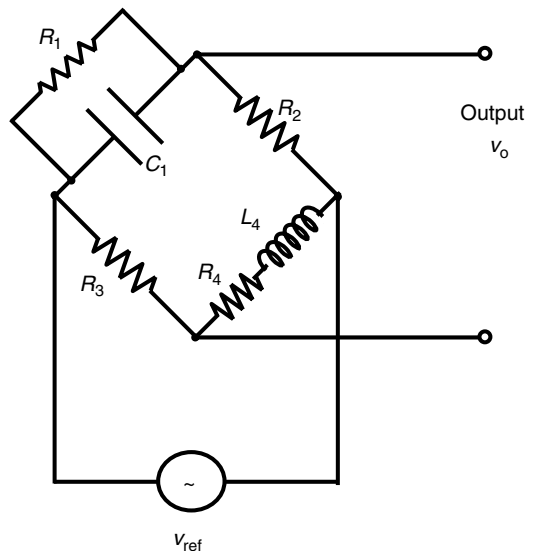
FIGURE P2.30 The Maxwell bridge.
