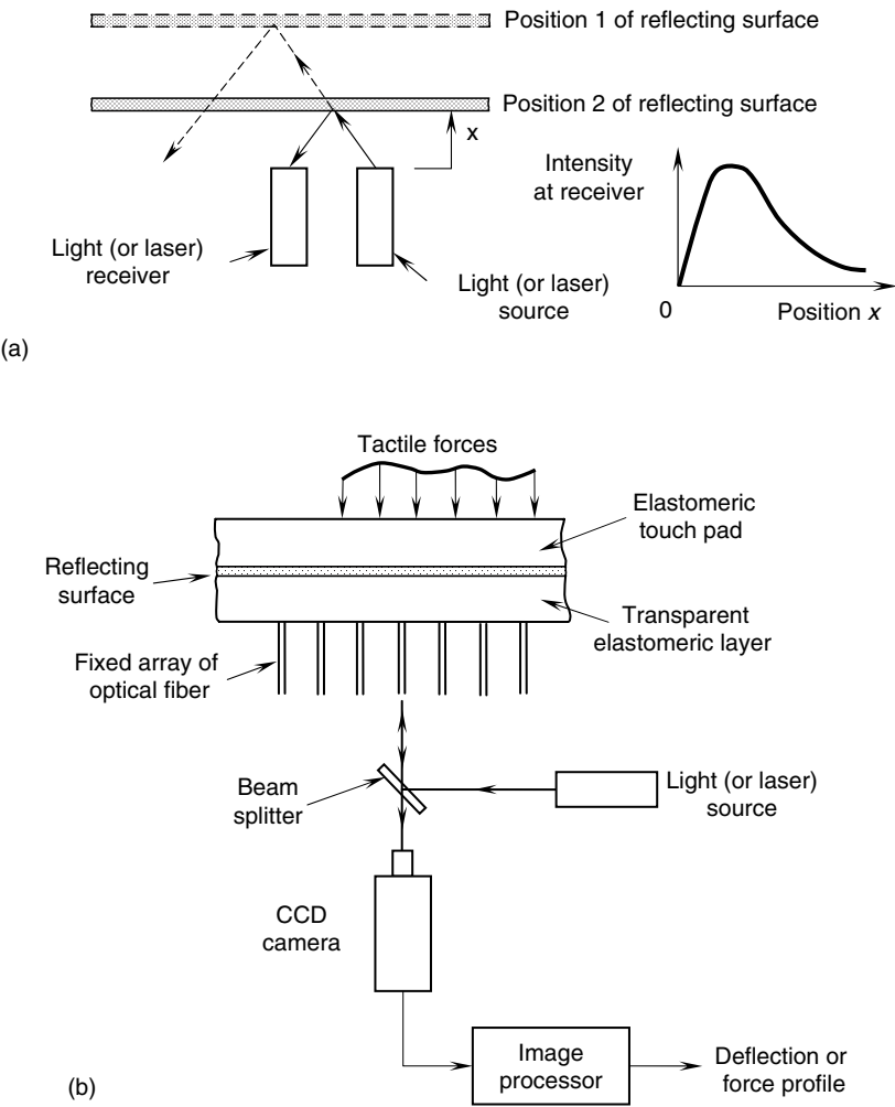
FIGURE 4.66 (a) The principle of an optical proximity sensor. (b) Schematic representation of a fiber-optic tactile sensor.
