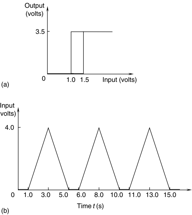
FIGURE P5.18 (a) The input/output characteristic of a Schmitt trigger; (b) a triangular input signal.
