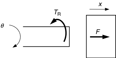
FIGURE 8.3 Effort and motion transmission at the screw and nut interface.
