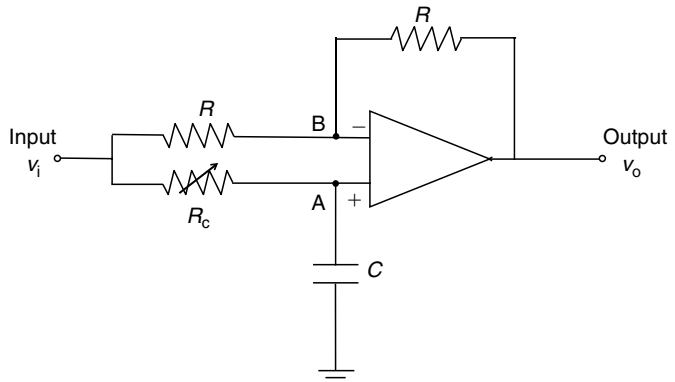
FIGURE 2.42 A phase shifter circuit.
