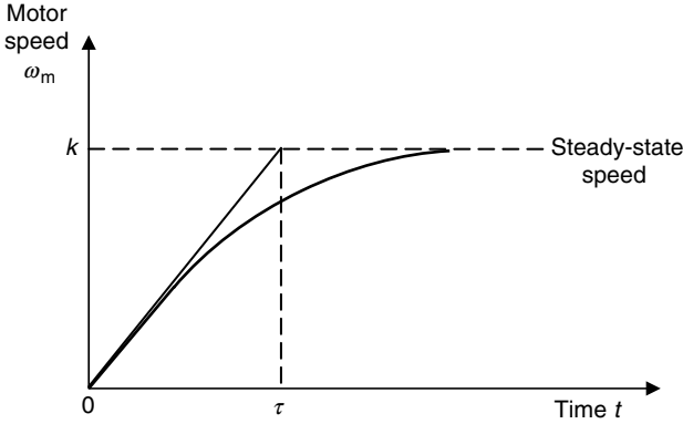
FIGURE 7.17 Open-loop step response of motor speed.
