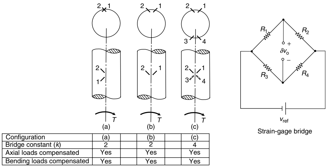
FIGURE 4.55 Strain-gage configurations for a circular shaft torque sensor.
