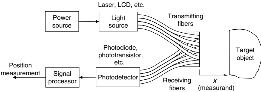
FIGURE 4.70 A fiber-optic position sensor.
