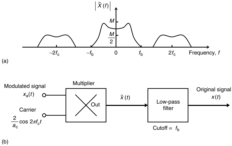
FIGURE 2.24 Amplitude demodulation. (a) Spectrum of the signal after the second modulation. (b) Demodulation schematic diagram (modulation + filtering).
