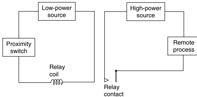
FIGURE P4.26 Proximity switch-operated relay circuit.
