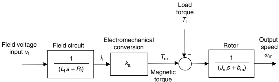
FIGURE 7.21 Open-loop block diagram for a field-controlled dc motor.
