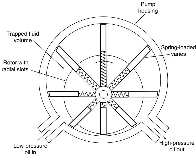
FIGURE 7.54 A hydraulic vane pump.
