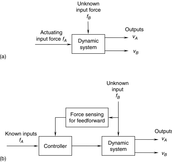
FIGURE 4.39 (a) A system with an unknown input force. (b) Feedforward force control.
