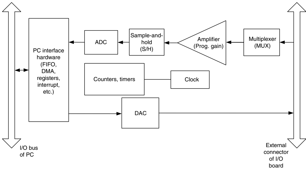
FIGURE 2.26 Main components of an I/O board of a PC.
