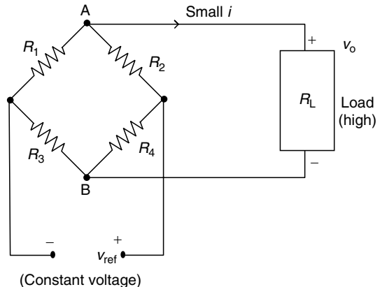
FIGURE 4.45 Wheatstone bridge circuit.
