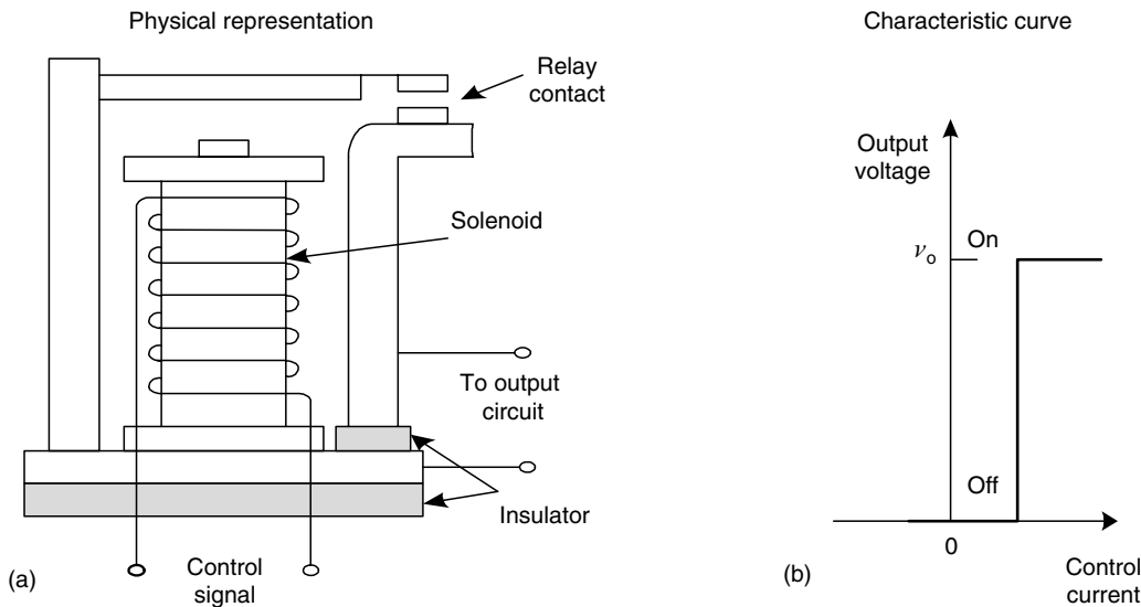
FIGURE 7.51 A solenoid operated relay. (a) Physical components. (b) Characteristic curve.
