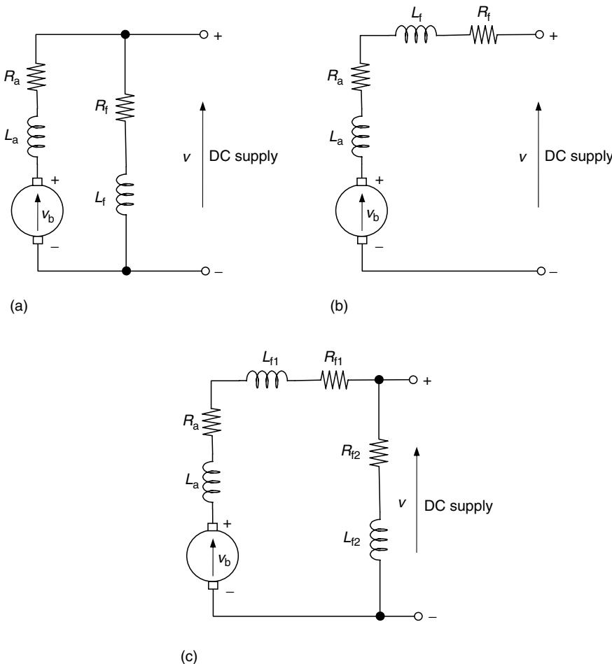
FIGURE 7.12 (a) A shunt-wound motor. (b) A series-wound motor. (c) A compound-wound motor.
