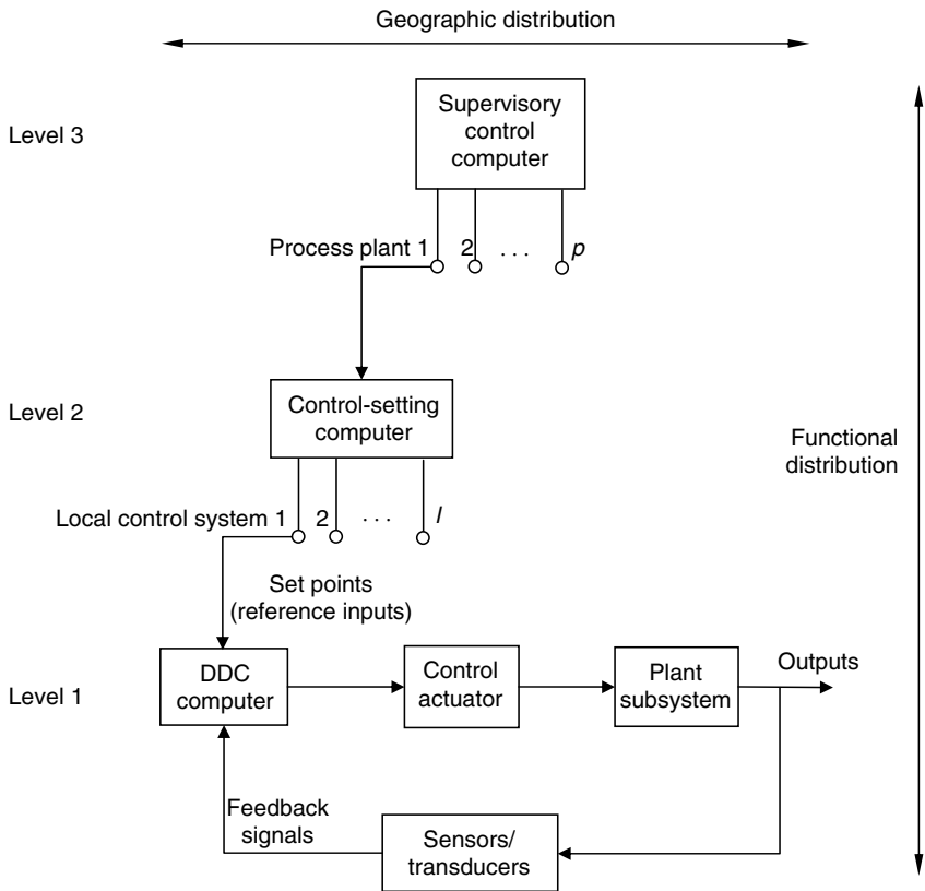
FIGURE 1.11 A three-layer hierarchical control system.
