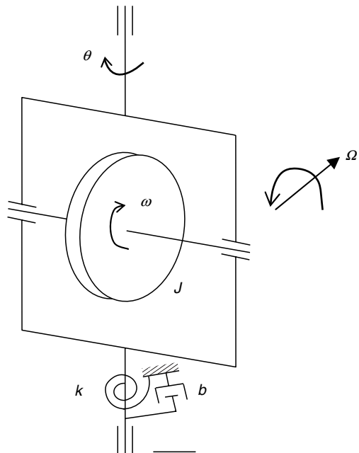
FIGURE P4.67 A rate gyro speed sensor.
