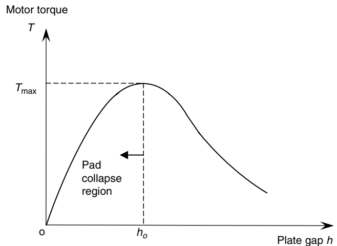
FIGURE 3.18 Characteristic curve of the chip refiner.
