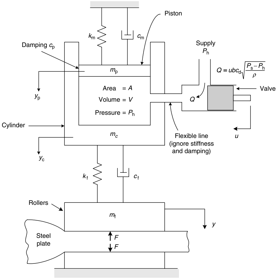
FIGURE 7.62 Automatic gage control (AGC) system of a steel rolling mill.
