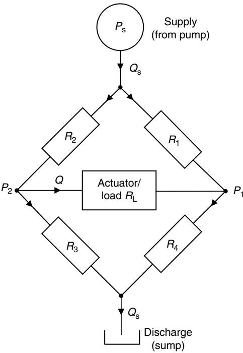
FIGURE 7.69 The bridge circuit representation of a four-way valve and an actuator load.
