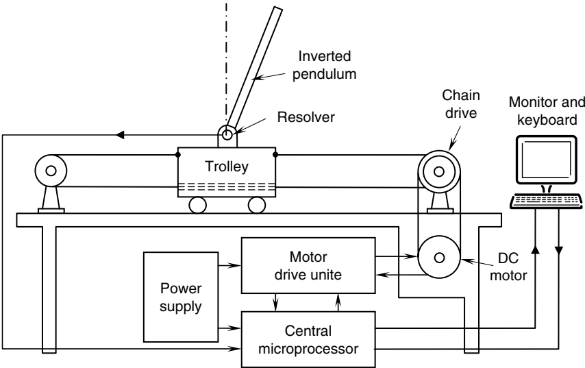
FIGURE P3.30 A microprocessor-controlled inverted pendulum—an application of statistical process control.
