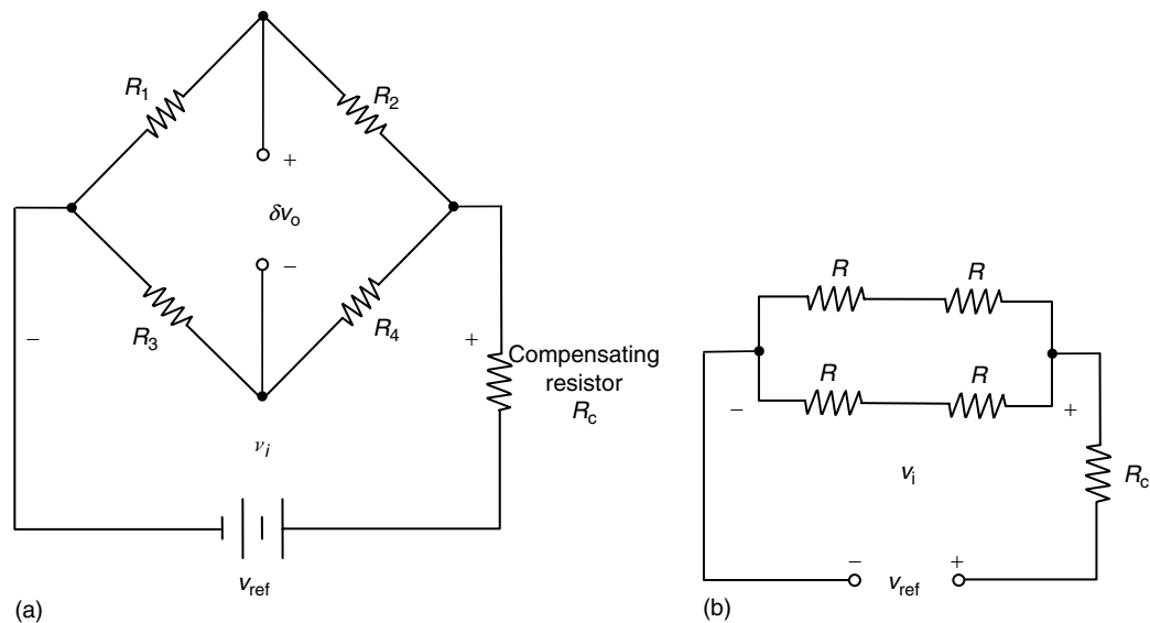
FIGURE 4.53 A strain-gage bridge with a compensating resistor. (a) Constant voltage dc bridge. (b) Equivalent circuit with high load impedance.
