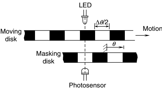
FIGURE P5.17 An encoder with a masking disk.
