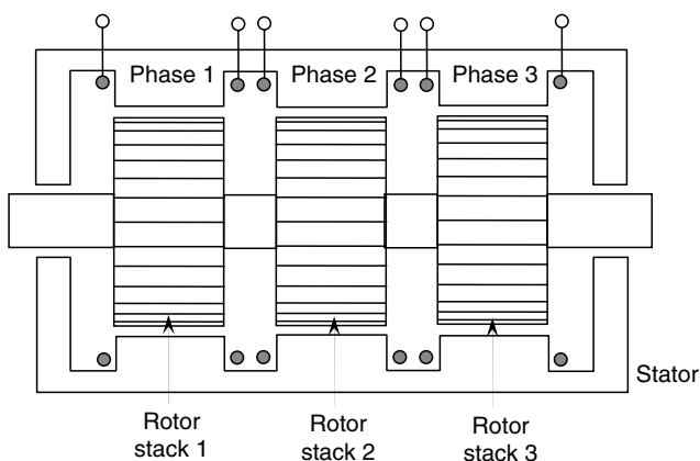
FIGURE 6.13 Longitudinal view of a three-stack (three-phase) stepper motor.
