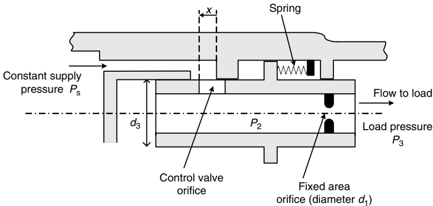
FIGURE P7.46 A flow control valve.
