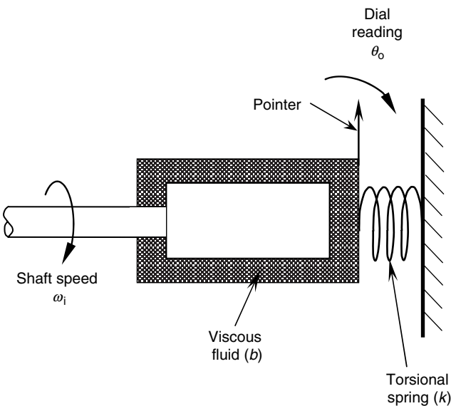
FIGURE 3.8 A mechanical tachometer.
