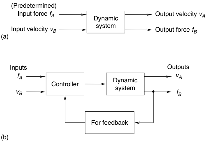
FIGURE 4.38 (a) An open-loop system. (b) A force feedback control system.
