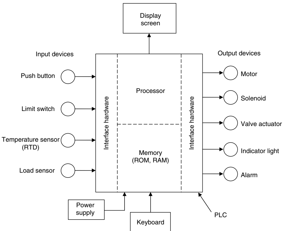
FIGURE 1.7 Schematic representation of a PLC.
