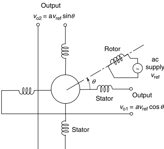
FIGURE 4.16 Schematic diagram of a resolver.
