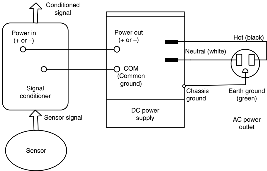
FIGURE 2.10 An example of grounding of instruments.
