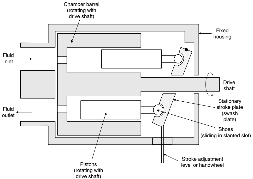
FIGURE 7.56 An axial piston hydraulic pump.
