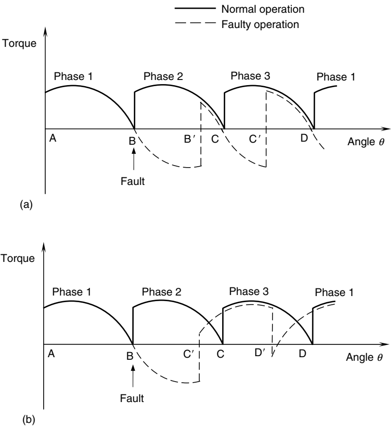
FIGURE 6.35 Motor deceleration due to pulse missing: (a) Case of a missed pulse; (b) Case of a missed phase activation.
