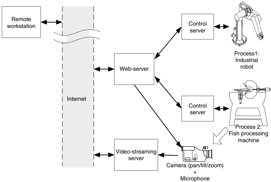
FIGURE 1.10 Network hardware architecture.
