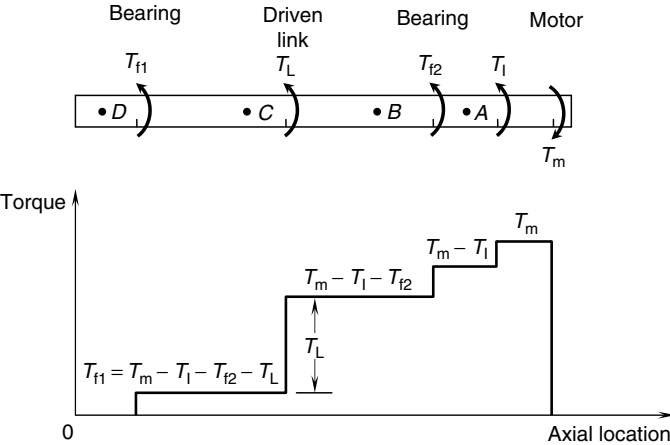
FIGURE 4.59 Torque distribution along the axis of a direct-drive manipulator joint.
