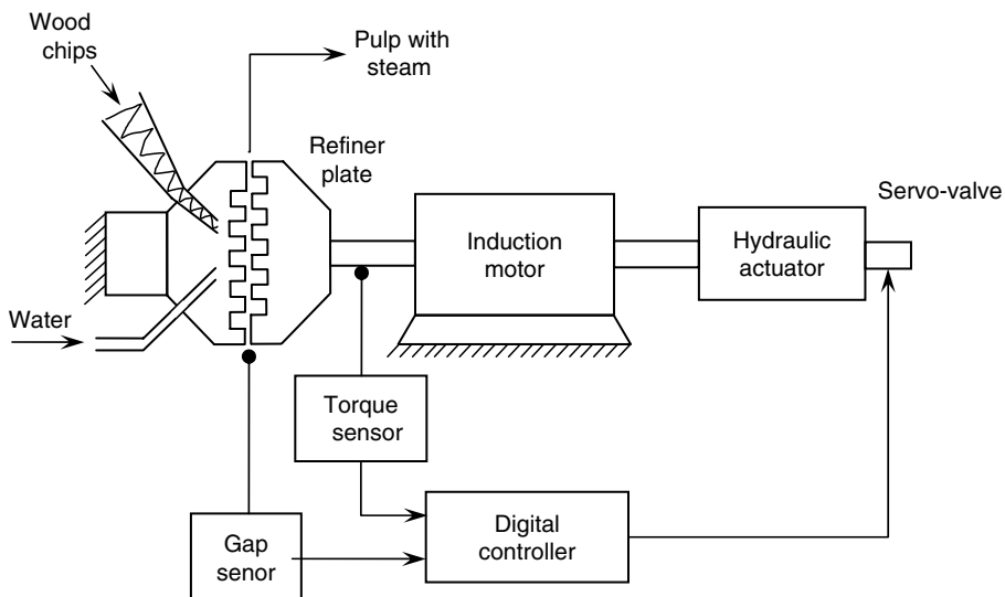
FIGURE 3.17 A single-disk chip refiner.
