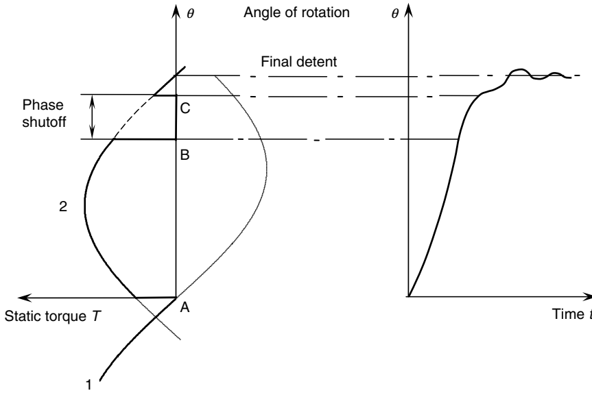
FIGURE 6.31 The pulse turn-off method of electronic damping.
