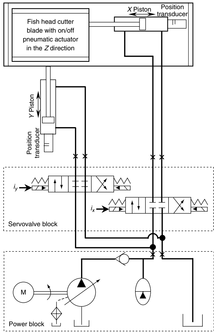
FIGURE P7.51 Two-axis hydraulic positioning system of an industrial fish cutter.
