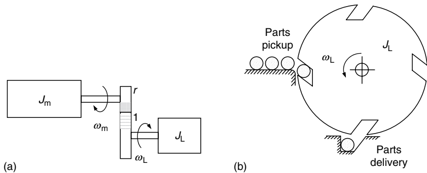
FIGURE P6.39 (a) Stepper motor driving an inertial load. (b) A parts transfer mechanism: an example of inertial load.
