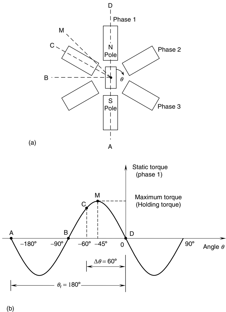
FIGURE 6.22 Static torque distribution of the VR stepper motor in Figure 6.5. (a) Schematic diagram. (b) Static torque curve for phase 1.
