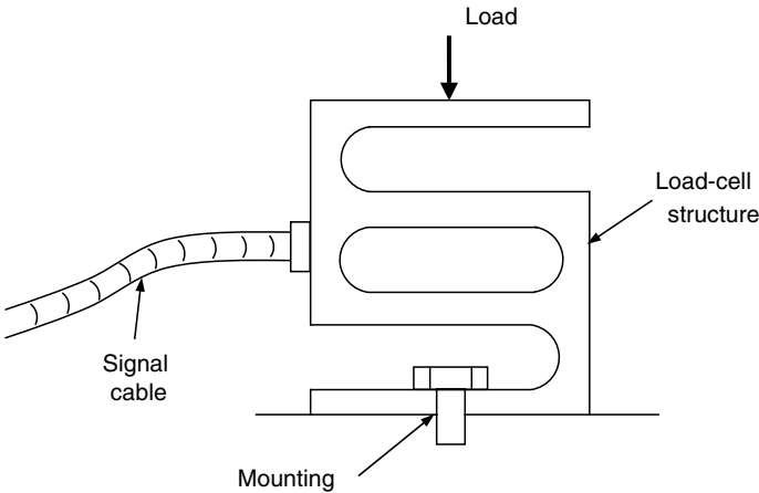
FIGURE 4.64 An industrial force sensor (load cell).
