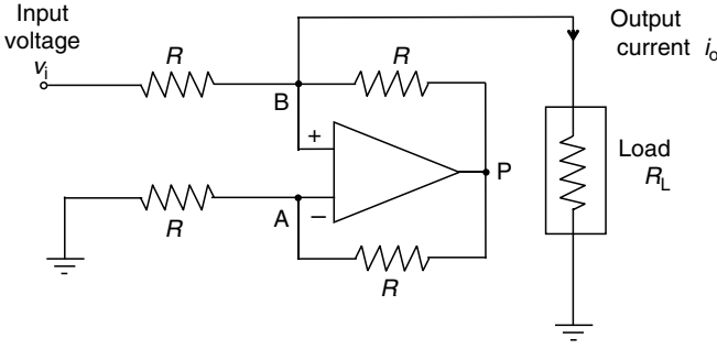
FIGURE 2.45 A voltage-to-current converter.
