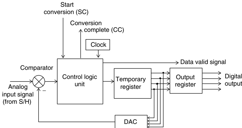
FIGURE 2.29 Successive approximation ADC.
