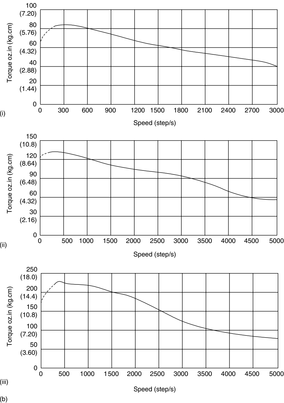
FIGURE P6.36 (continued) (b) Speed–torque characteristics of the motors: (i) Model 1; (ii) Model 2; (iii) Model 3.
