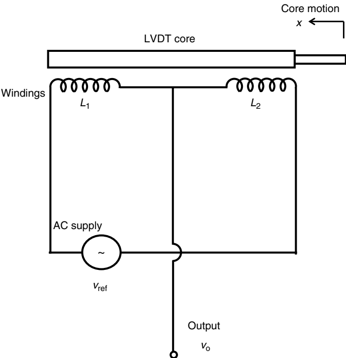
FIGURE P2.31 A half-bridge circuit for an LVDT.
