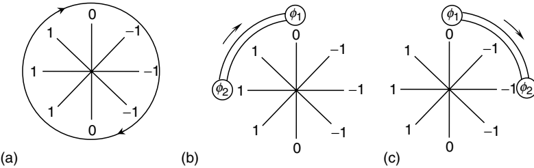
FIGURE 6.4 (a) Half-step switching states. (b) Switching logic for clockwise rotation. (c) Switching logic for CCW rotation.
