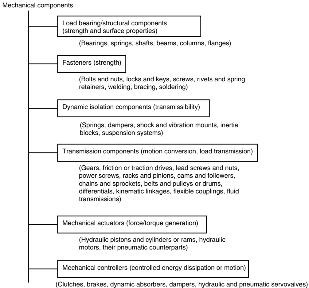
FIGURE 8.1 Classification of mechanical components.
