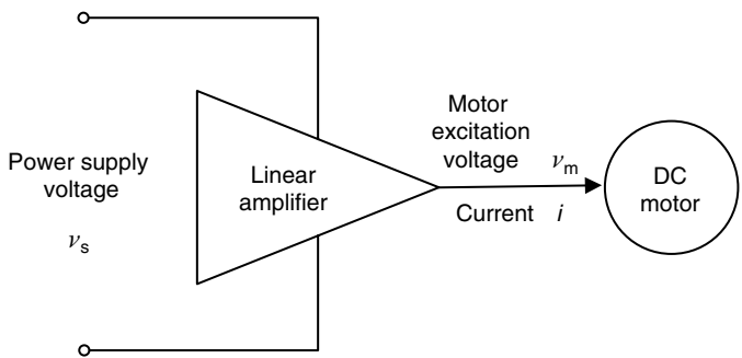
FIGURE P7.11 A linear amplifier for a dc motor.
