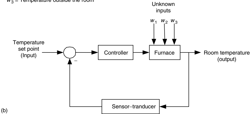
FIGURE 1.6 (a) A natural gas home heating system. (b) A block diagram representation of the system.
