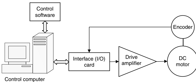
FIGURE 7.25 Components of a dc motor control system.
