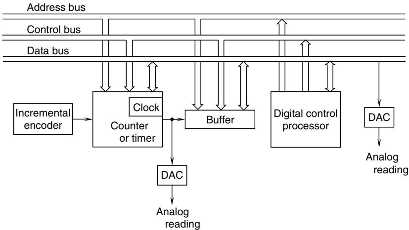
FIGURE 5.7 Computer interface for an incremental encoder.
