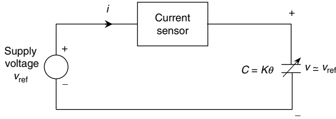
FIGURE 4.26 Rotating-plate capacitive angular velocity sensor.
