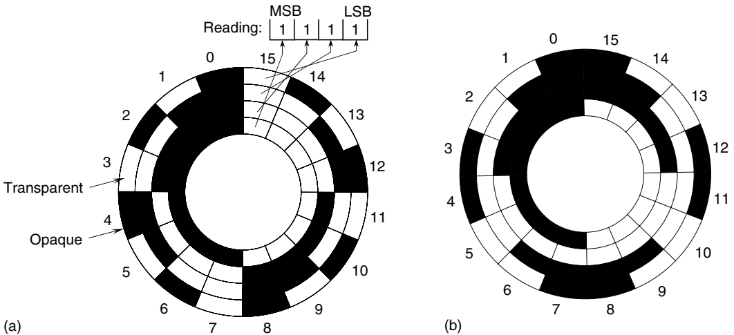
FIGURE 5.8 Illustration of the code pattern of an absolute encoder disk: (a) Binary code; (b) a gray code.
