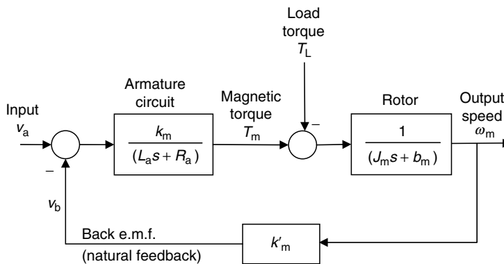
FIGURE 7.16 Open-loop block diagram for an armature-controlled dc motor.
