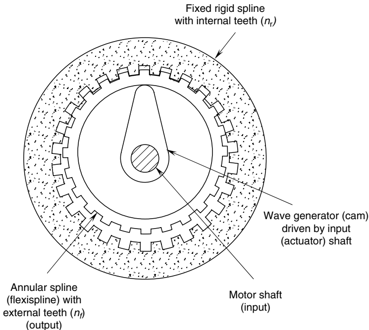
FIGURE 8.5 The principle of operation of a harmonic drive.
