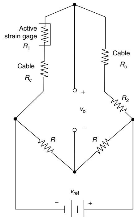
FIGURE P4.56 The influence of cable resistance on strain-gage bridge measurements.
