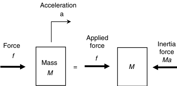
FIGURE 4.30 Illustration of d’Alembert’s principle.
