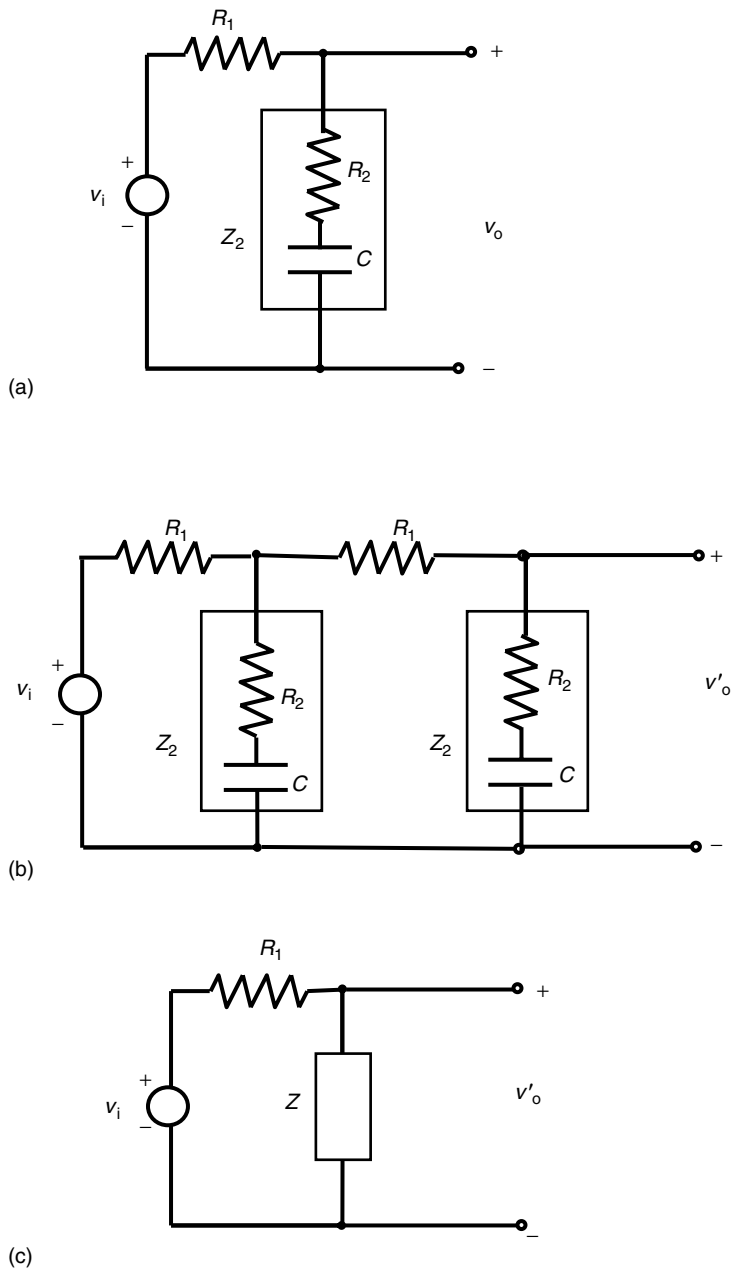
FIGURE 2.2 (a) A single circuit module. (b) Cascade connection of two modules. (c) An equivalent circuit for (b).
