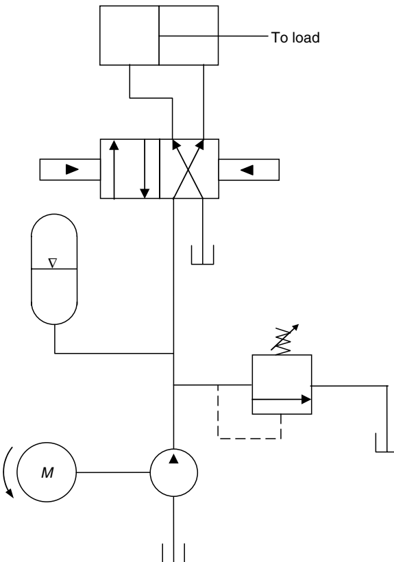
FIGURE P7.43 A hydraulic circuit diagram.
