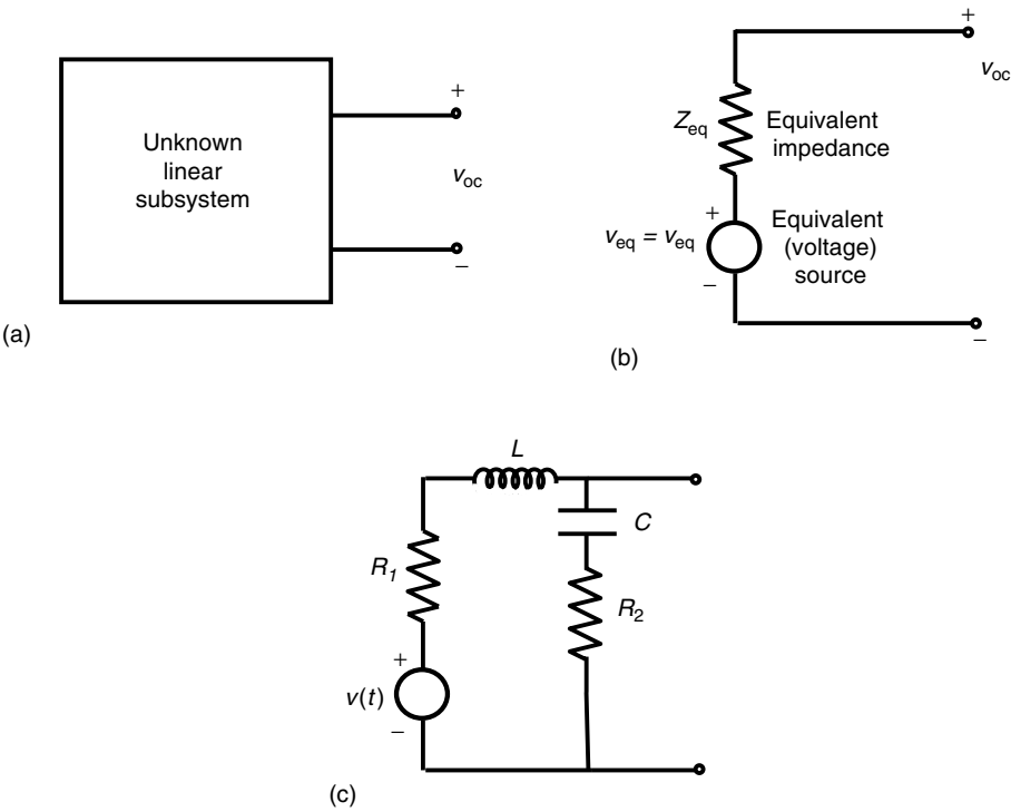
FIGURE P2.3 Illustration of Thevenin's theorem. (a) Unknown linear subsystem. (b) Equivalent representation. (c) Example.
