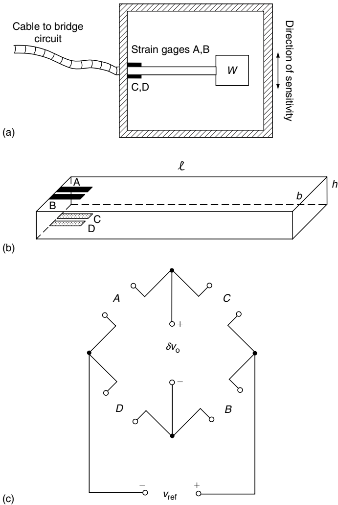
FIGURE 4.47 A miniature accelerometer using strain gages: (a) Schematic diagram; (b) Mounting configuration of the strain gages; (c) Bridge connection.
