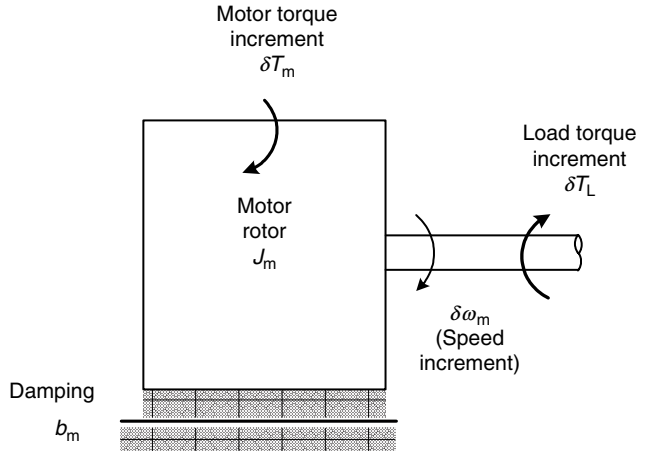
FIGURE 7.47 Incremental load model for an induction motor.
