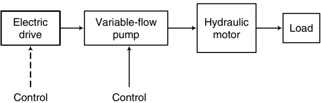
FIGURE 7.70 Configuration of a pump-controlled hydraulic-drive system.
