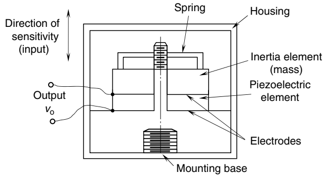
FIGURE 4.31 A compression-type piezoelectric accelerometer.
