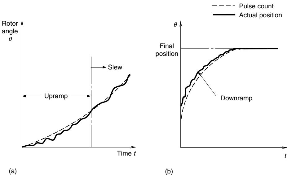
FIGURE 6.24 Ramping response. (a) Accelerating motion. (b) Decelerating motion.
