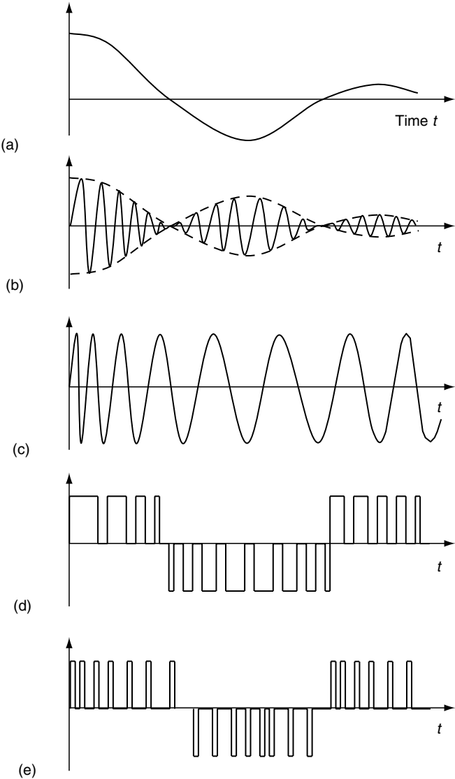
FIGURE 2.20 (a) Modulating signal (data signal). (b) Amplitude-modulated (AM) signal. (c) Frequency-modulated (FM) signal. (d) Pulse-width modulated (PWM) signal. (e) Pulse-frequency-modulated (PFM) signal.
