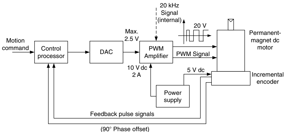
FIGURE P5.20 A servo loop of a robot.
