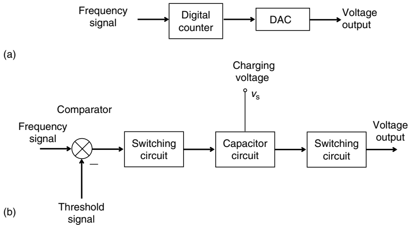
FIGURE 2.44 Frequency-to-voltage converter (FVCs). (a) Digital counter method. (b) Capacitor charging method.
