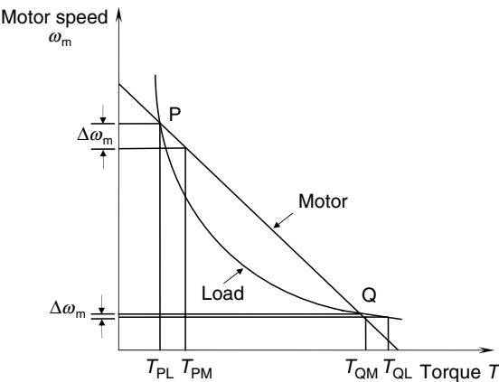
FIGURE 7.10 Operating points for a constant-power load driven by a dc motor.
