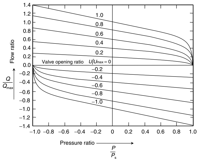
FIGURE 7.59 Steady-state characteristics of a four-way spool valve.
