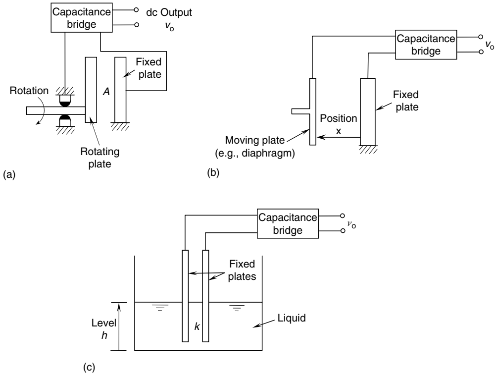
FIGURE 4.23 Schematic diagrams of capacitive sensors. (a) Capacitive rotation sensor. (b) Capacitive displacement sensor. (c) Capacitive liquid level sensor.
