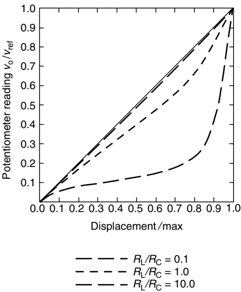
FIGURE 4.4 Electrical loading nonlinearity in a potentiometer.
