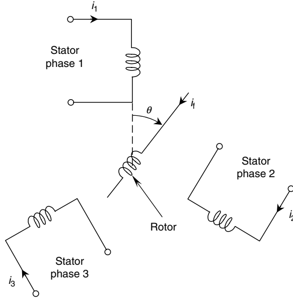
FIGURE 4.63 Schematic representation of a three-phase synchronous motor.
