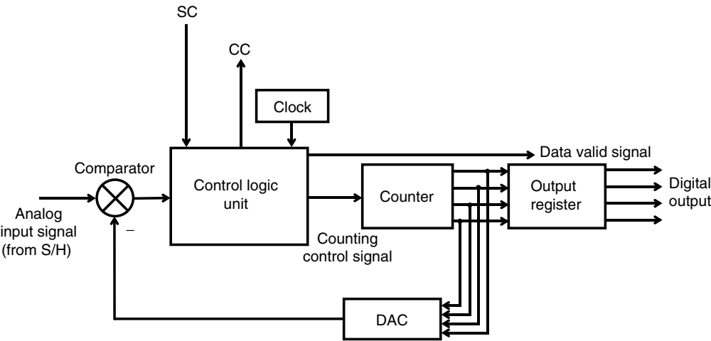
FIGURE 2.31 Counter ADC.
