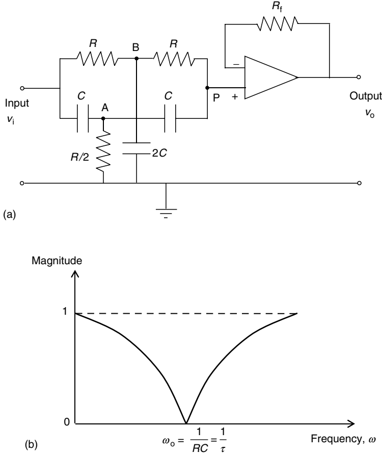
FIGURE 2.19 A notch filter. (a) An active twin T filter circuit. (b) Frequency response characteristic.
