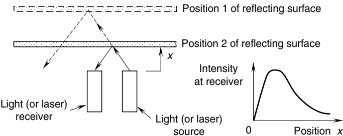
FIGURE 4.71 The principle of a fiber-optic proximity sensor.
