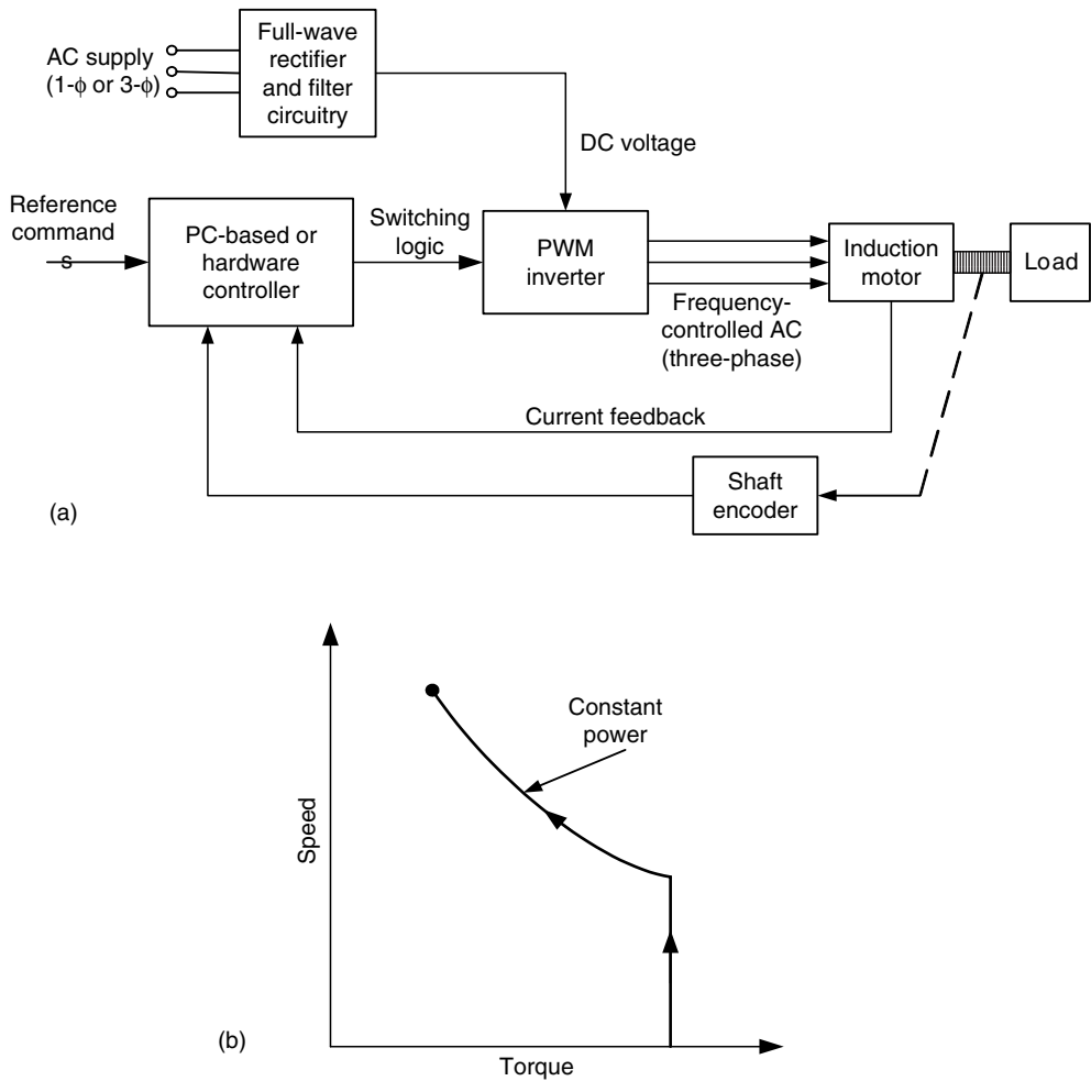
FIGURE 7.43 (a) Variable frequency control of an induction motor. (b) A typical control strategy.
