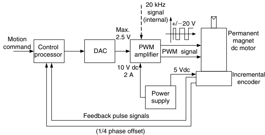
FIGURE P7.13 A servo loop of a robot.
