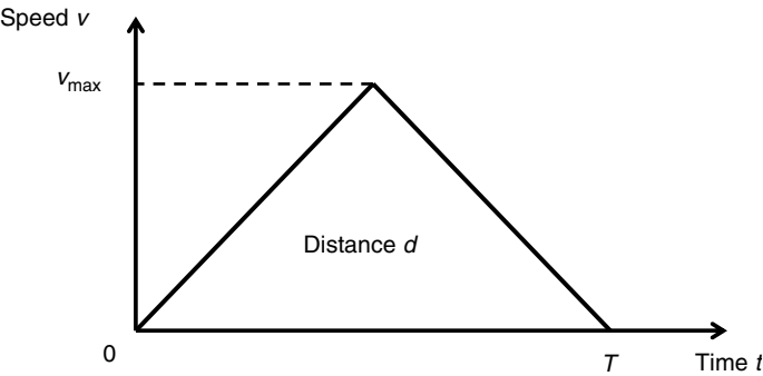
FIGURE 6.45 Speed profile for a motion period of the conveyor.
