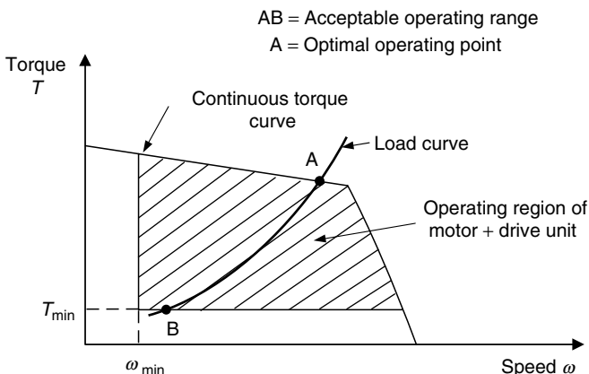
FIGURE 7.34 Sizing a motor for a given load.
