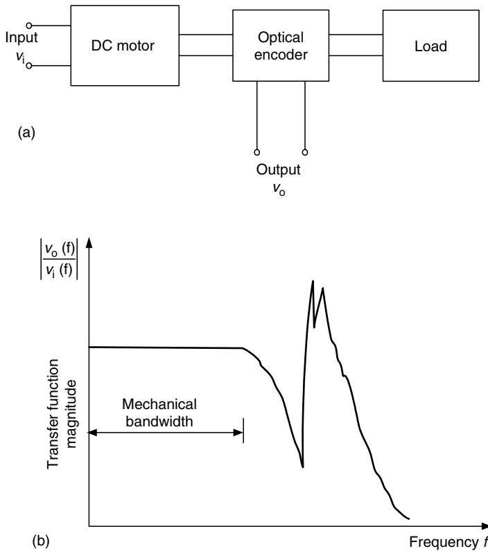
FIGURE 7.32 Determination of the mechanical bandwidth of a dc motor. (a) Test setup. (b) Test result.
