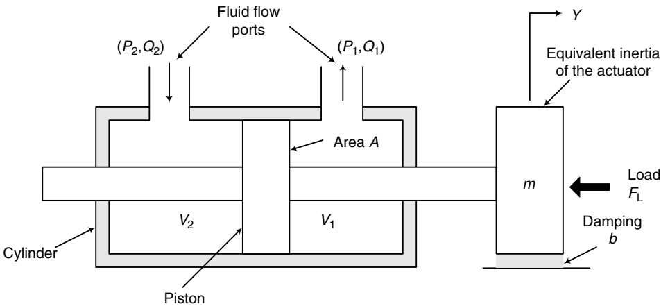
FIGURE 7.60 Double-acting piston-cylinder hydraulic actuator.
