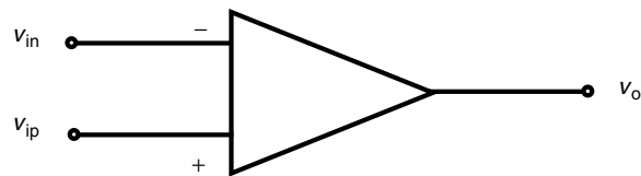
FIGURE 2.7 Operational amplifier. (a) A schematic model. (b) Eight-pin dual in-line package (DIP). (c) Conventional circuit symbol.
