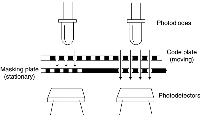
FIGURE P5.21 Photodiode-detector arrangement of a linear optical encoder.
