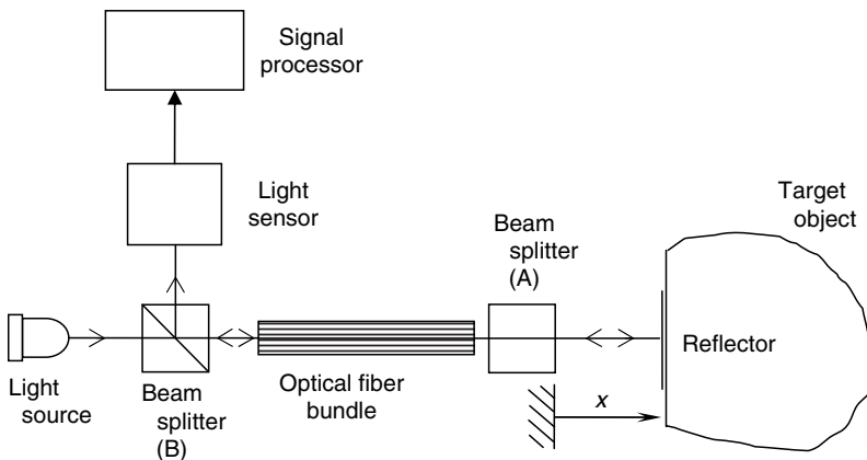
FIGURE 4.72 Laser interferometer position sensor.
