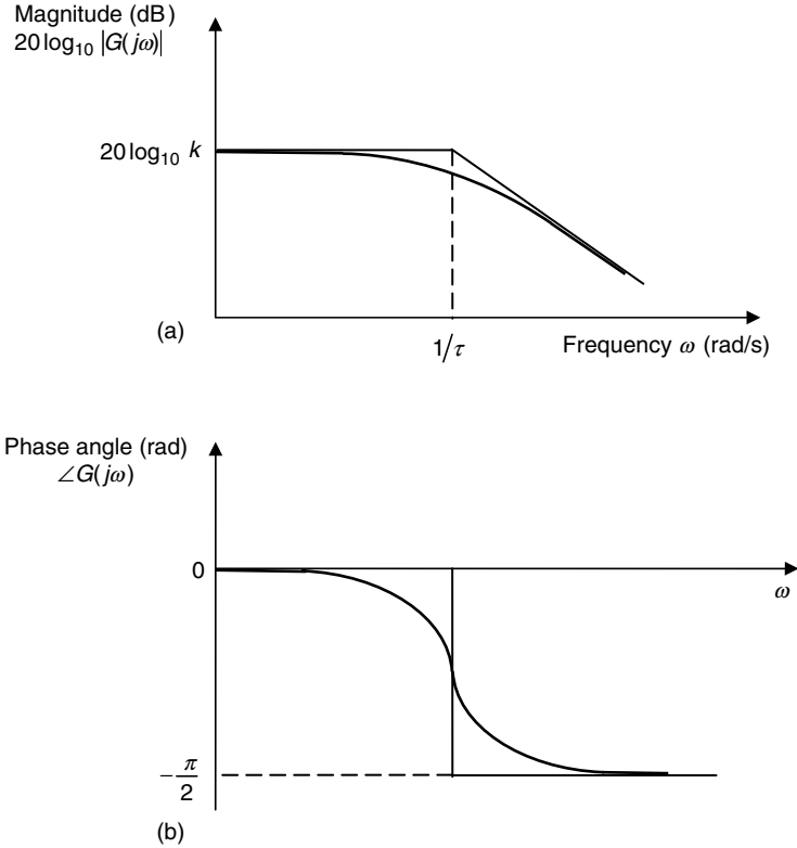
FIGURE 7.18 Open-loop frequency response of motor speed (Bode diagram).
