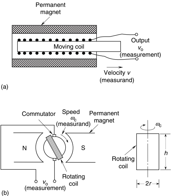
FIGURE 4.19 Permanent-magnet dc transducers. (a) Rectilinear velocity transducer. (b) DC tachometer.
