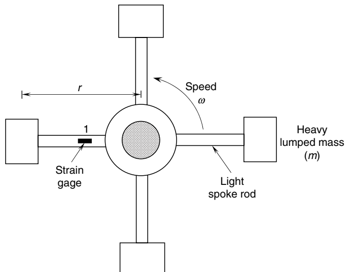
FIGURE P4.64 Strain-gage speed sensor for a fly wheel.
