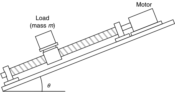
FIGURE 8.4 A lead-screw unit driving an object up an incline.
