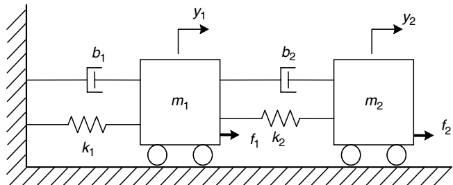
FIGURE 4.36 A model of a mechanical system.
