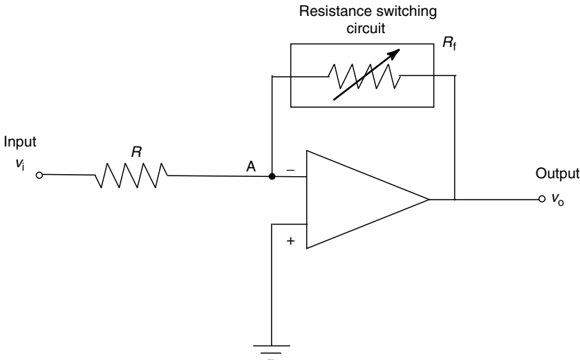
FIGURE 2.41 A curve-shaping circuit.
