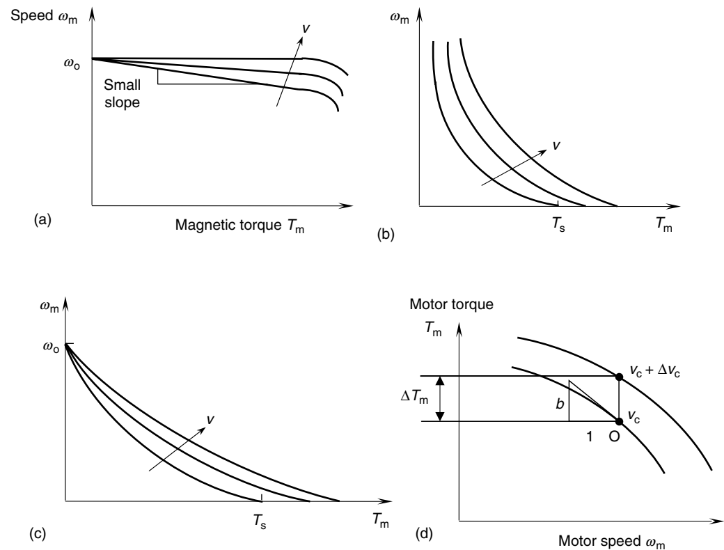
FIGURE 7.13 Torque–speed characteristic curves for dc motors. (a) Shunt-wound. (b) Series-wound. (c) Compound-wound, and (d) Linearization of the general case.
