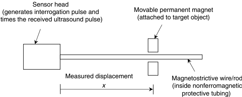
FIGURE 4.76 A magnetostrictive ultrasound displacement sensor.
