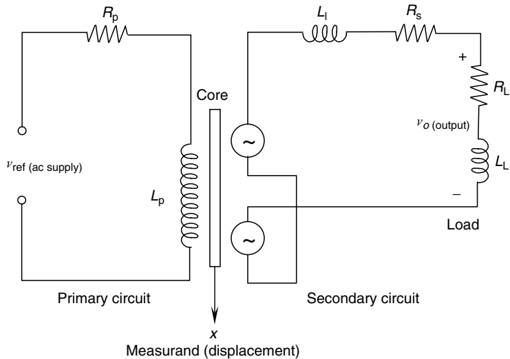
FIGURE 4.10 Equivalent circuit for a differential transformer/transducer.
