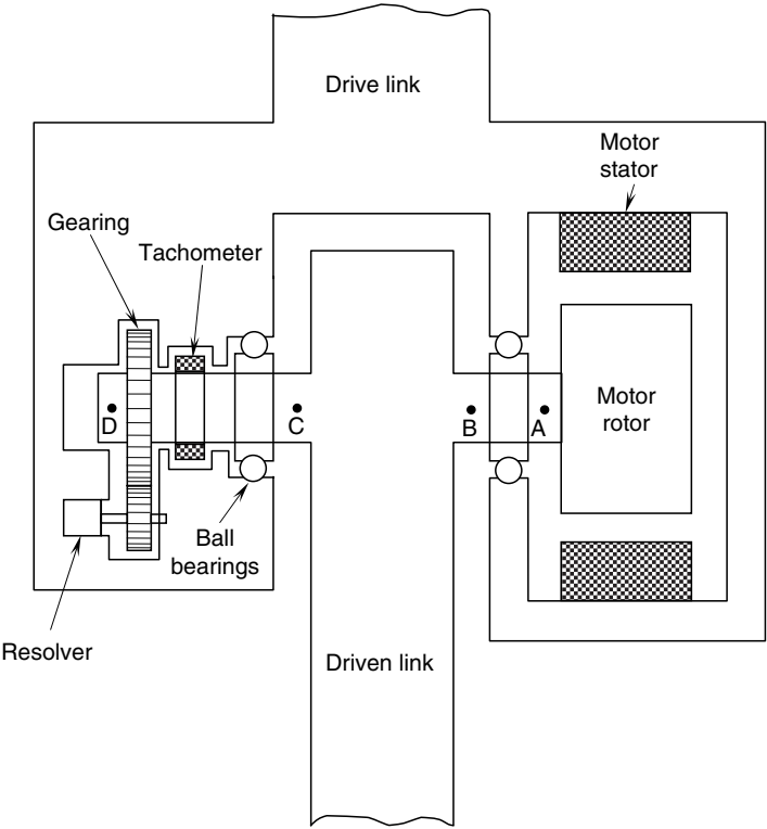
FIGURE 4.58 A joint of a direct-drive robotic arm.
