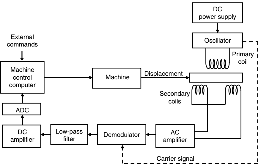
FIGURE P2.7 Components of an LVDT-based machine control loop.
