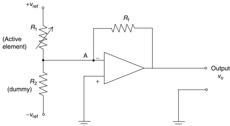
FIGURE 2.36 A half bridge with an output amplifier.
