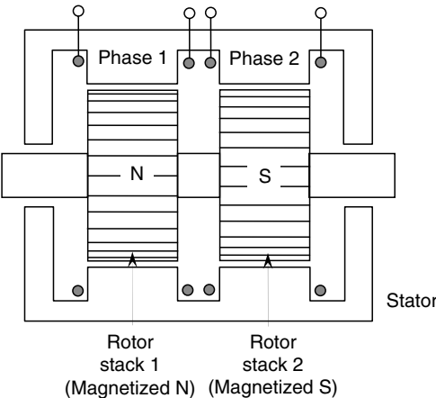
FIGURE 6.14 A hybrid stepper motor.
