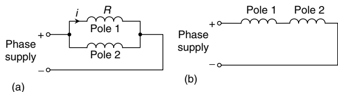
FIGURE P6.18 Pole windings in a phase of a stepper motor that has 2 poles/phase. (a) Parallel connection. (b) Series connection.
