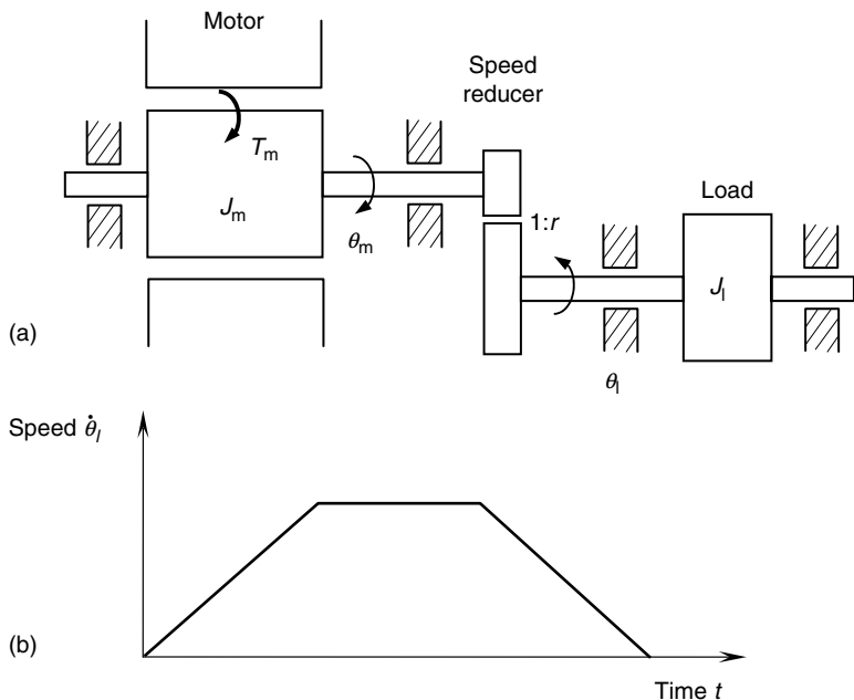
FIGURE P3.21 (a) A single-degree-of-freedom model of a robotic manipulator. (b) A typical reference (desired) speed trajectory for computed-torque control.
