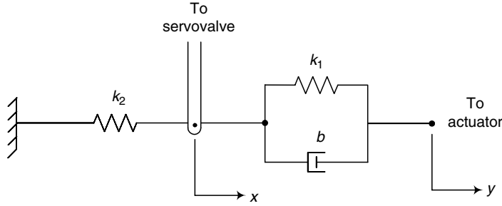
FIGURE P7.45 A mechanical coupling with lead action for a hydraulic servovalve.
