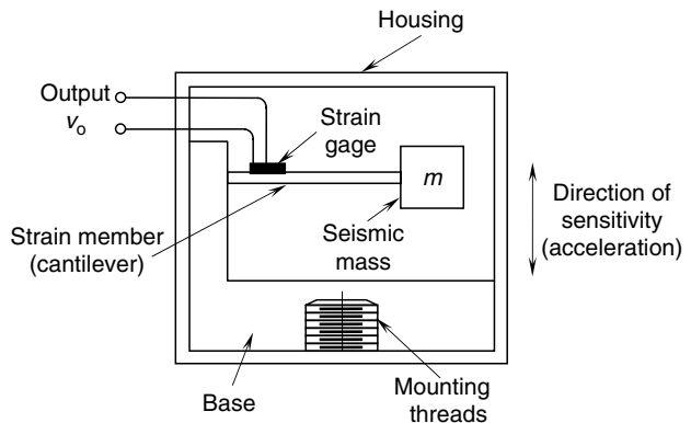
FIGURE 4.43 A strain-gage accelerometer.
