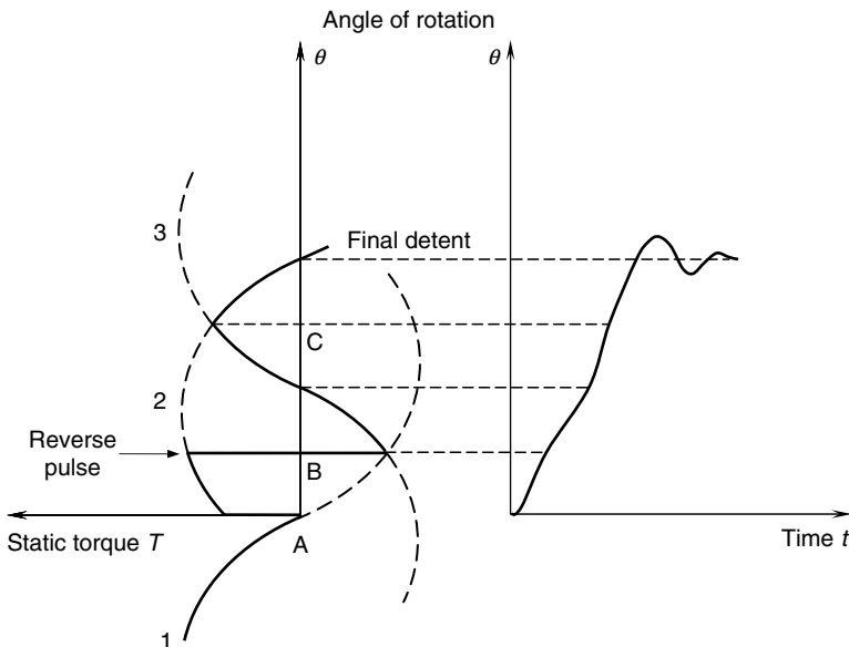
FIGURE 6.32 The pulse reversal method of electronic damping.
