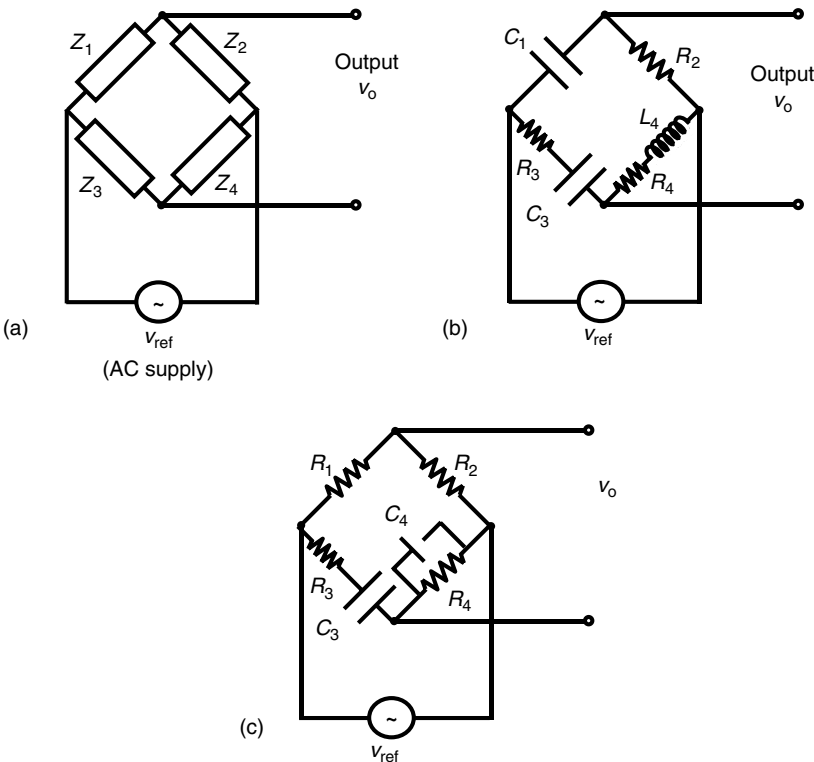
FIGURE 2.37 (a) General impedance bridge. (b) Owen bridge. (c) Wien-bridge oscillator.
