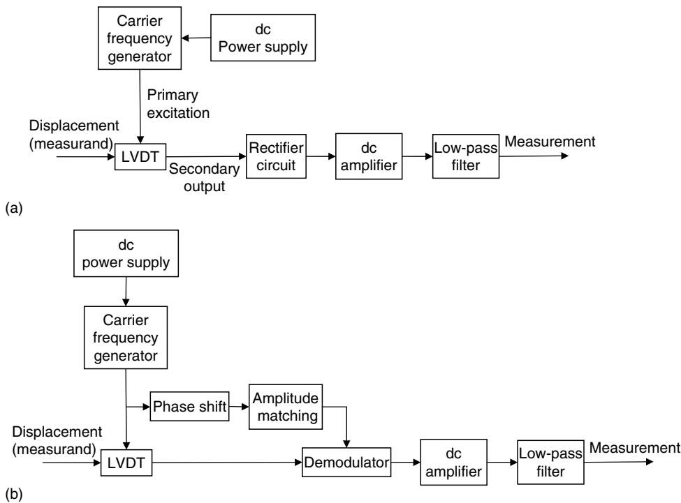
FIGURE 4.11 Signal-conditioning methods for a differential transformer. (a) Rectification. (b) Demodulation.
