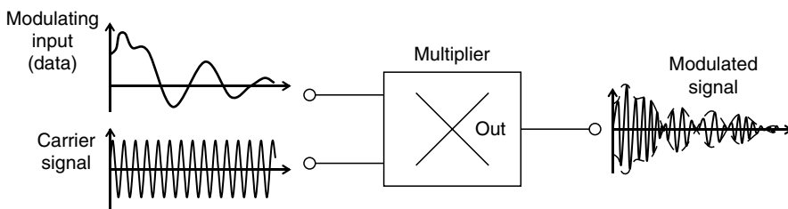
FIGURE 2.23 Representation of an amplitude modulator.
