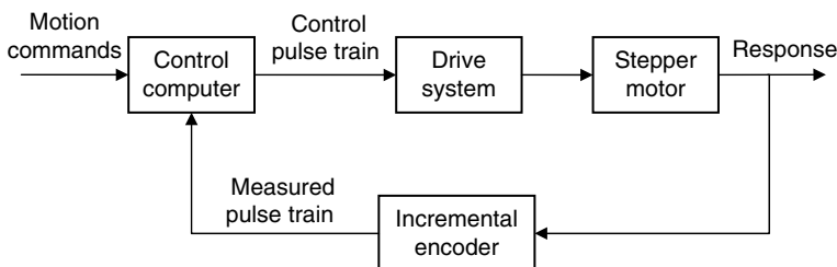
FIGURE 6.36 Feedback control of a stepper motor.
