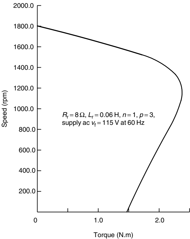
FIGURE 7.41 Torque–speed curve for an induction motor.
