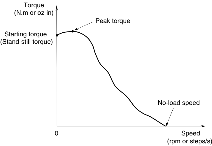
FIGURE 6.40 The speed–torque characteristics of a stepper motor.
