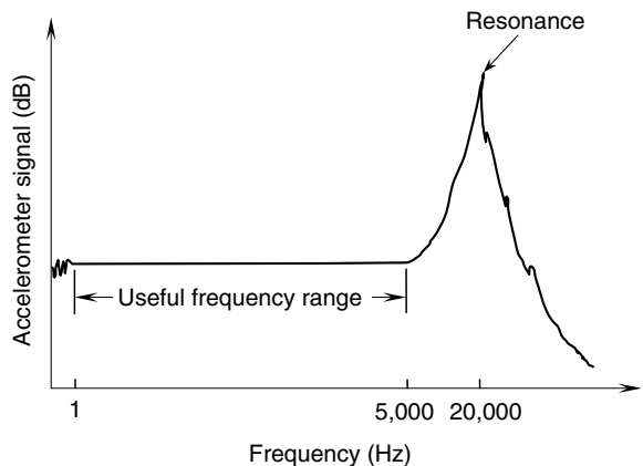
FIGURE 4.32 A typical frequency response curve for a piezoelectric accelerometer.
