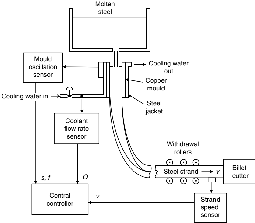
FIGURE P3.25 A steel-billet casting machine.
