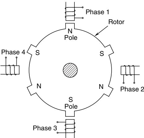
FIGURE P6.9 Schematic diagram of a stepper motor.
