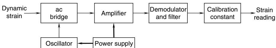
FIGURE 4.48 Measurement of dynamic strains using an ac bridge.
