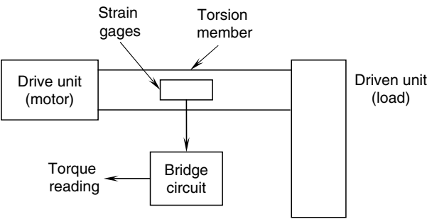
FIGURE 4.54 Torque sensing using a torsion member.
