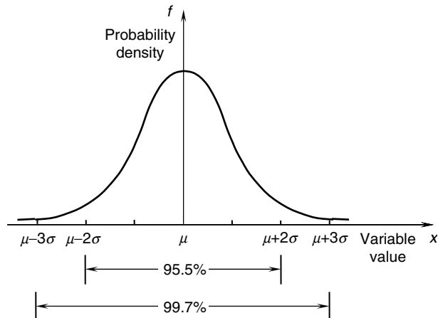
FIGURE 5.9 Gaussian (normal) probability density function.
