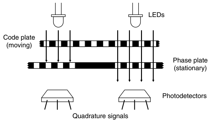
FIGURE 5.16 A rectilinear optical encoder.
