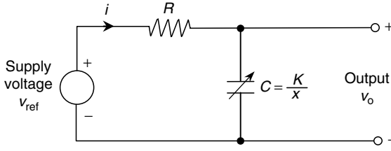
FIGURE 4.25 Capacitive displacement sensor example.
