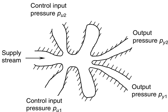
FIGURE 7.77 Jet deflection amplifier.
