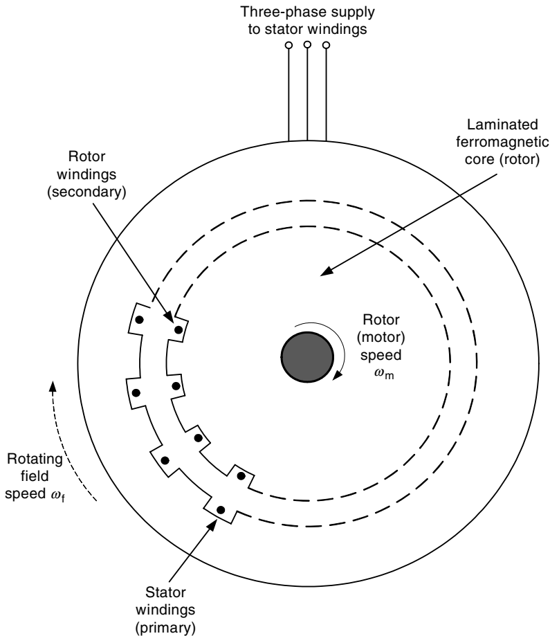
FIGURE 7.38 Schematic diagram of an induction motor.
