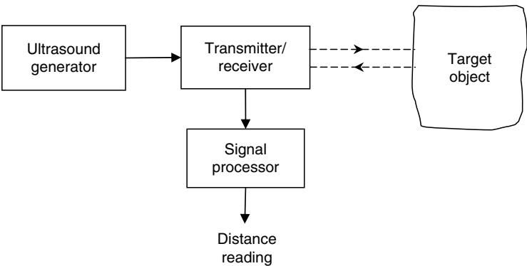
FIGURE 4.75 An ultrasonic position sensor.
