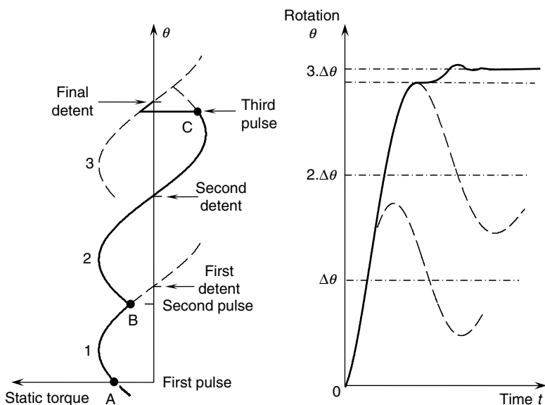
FIGURE 6.25 Torque-response diagram for a three-step drive sequence.
