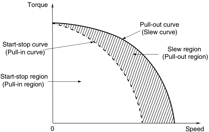
FIGURE 6.41 Further speed–torque characteristics and terminology.
