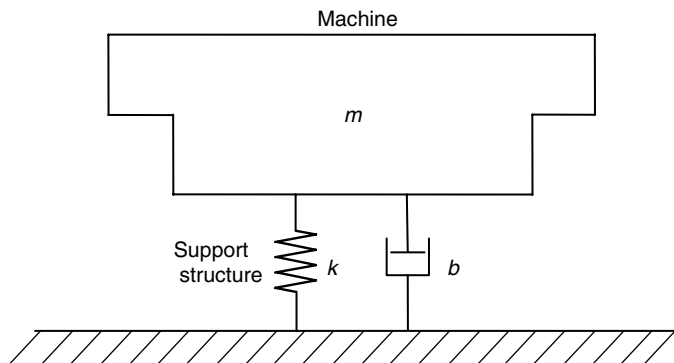
FIGURE P3.19 A model for the mounting structure of a machine.
