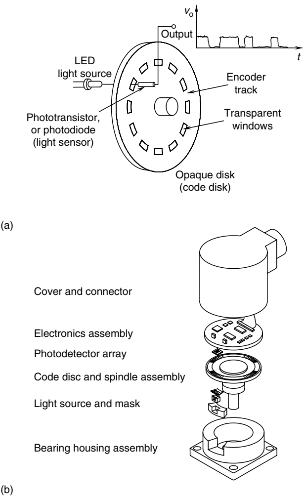
FIGURE 5.1 (a) Schematic representation of an (incremental) optical encoder; (b) components of a commercial incremental encoder. (BEI Electronics, Inc. With permission.)
