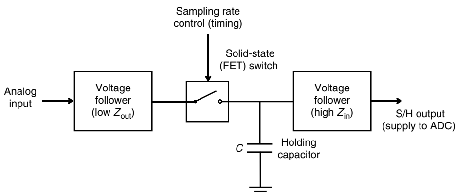
FIGURE 2.32 A sample-and-hold circuit.
