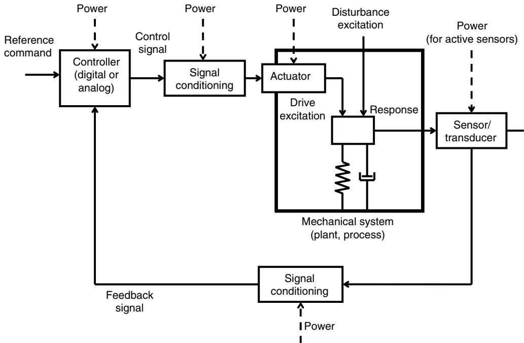
FIGURE 1.2 Schematic diagram of a feedback control system.
