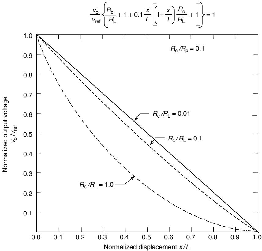
FIGURE 4.7 Behavior of the optical potentiometer for R_c/R_p = 0.1 .
