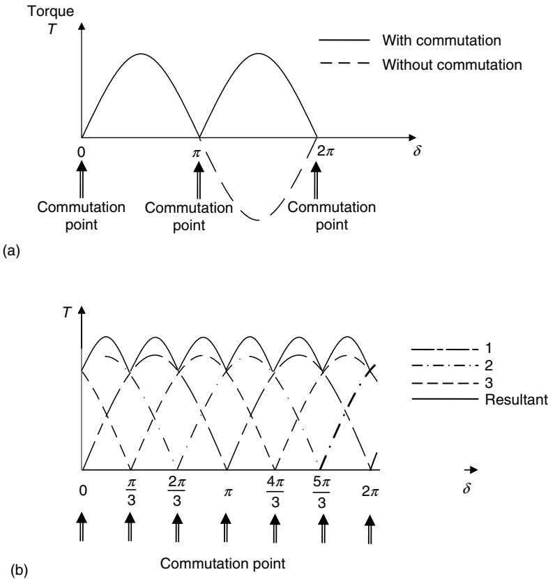
FIGURE 7.5 (a) Torque profile from a coil segment due to commutation. (b) Resultant torque from a rotor with three-coil segments.
