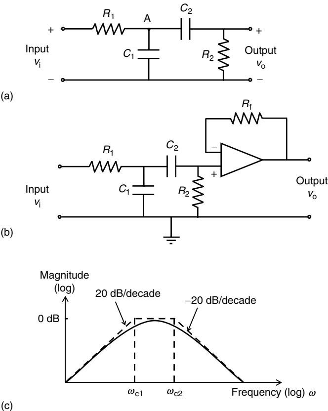
FIGURE 2.17 Band-pass filter. (a) A basic passive filter stage. (b) A basic active filter stage. (c) Frequency response characteristic.
