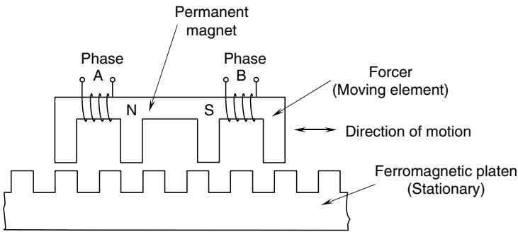
FIGURE P6.16 Schematic representation of a linear hybrid stepping motor.
