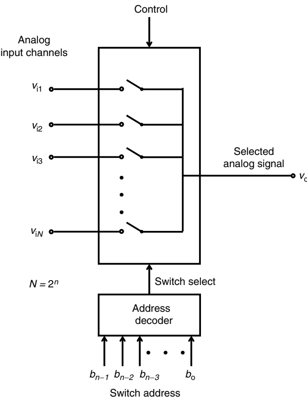
FIGURE 2.33 An N -channel analog multiplexer (MUX) (analog scanner).
