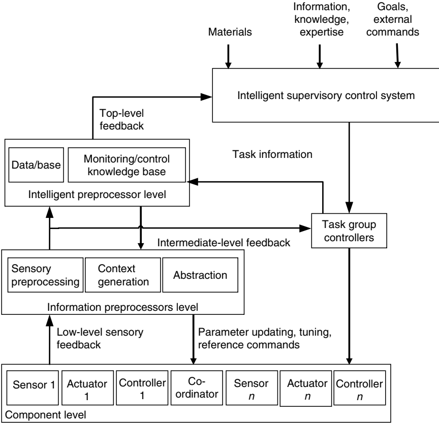
FIGURE 1.12 A hierarchical control and communications structure for an intelligent mechatronic system (IMS).
