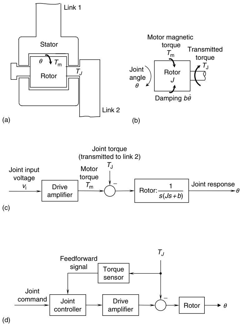
FIGURE 4.40 (a) A single joint of a direct-drive arm. (b) Free-body diagram of the motor rotor. (c) Block diagram of the joint. (d) Feedforward control using the joint torque.
