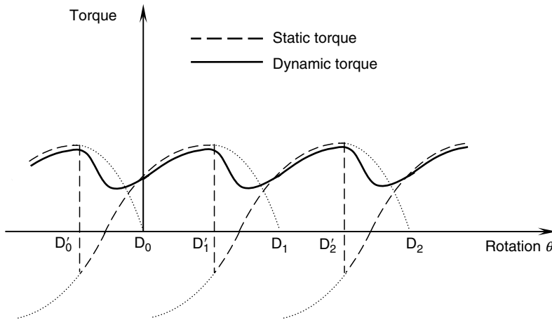
FIGURE 6.39 Dynamic torque at high speeds.
