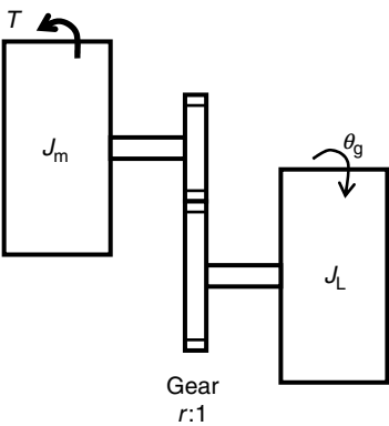
FIGURE P8.6 An inertial load driven by a motor through a gear transmission.
