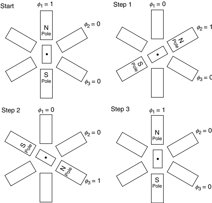
FIGURE 6.6 Full-stepping sequence for the three-phase VR stepper motor (step angle = 60°).
