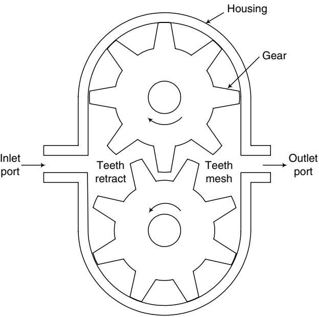
FIGURE 7.55 A hydraulic gear pump.
