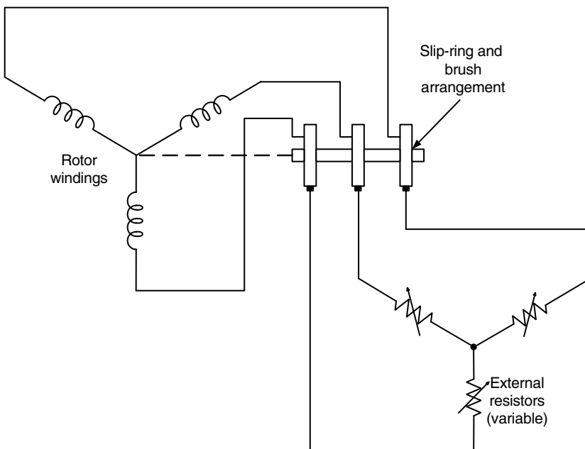
FIGURE 7.45 Rotor resistance control of an induction motor (three phase).
