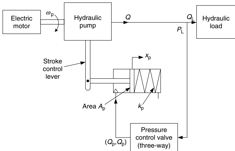
FIGURE P7.47 A pump stroke-regulated hydraulic power supply.
