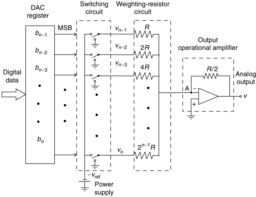
FIGURE 2.27 Weighted-resistor (adder) DAC.
