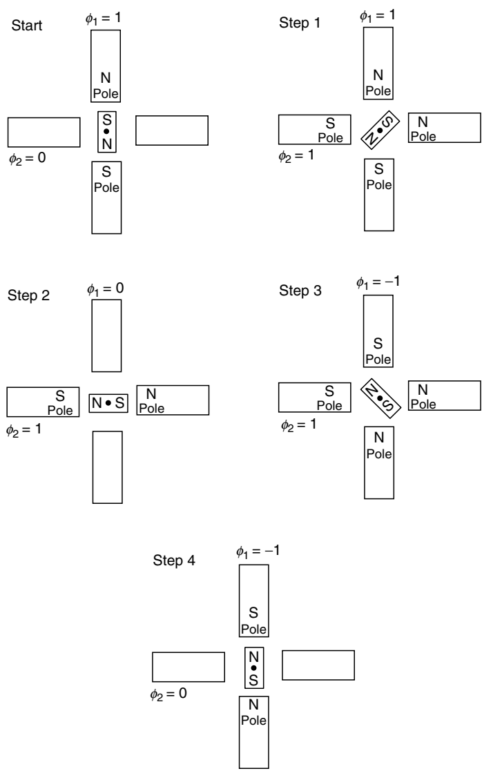
FIGURE 6.3 Stepping sequence (half stepping) in a two-phase PM stepper motor for clockwise rotation.
