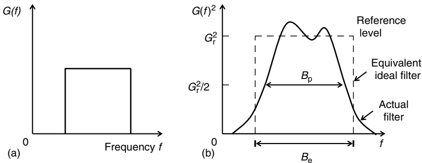
FIGURE 3.6 Characteristics of. (a) An ideal band-pass filter. (b) A practical band-pass filter.
