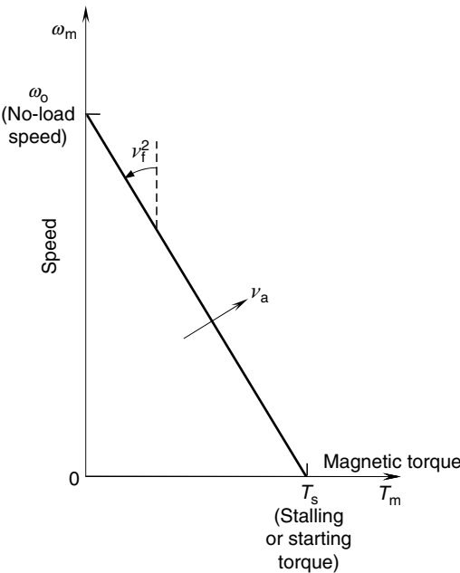
FIGURE 7.9 Steady-state speed–torque characteristics of a separately wound dc motor.
