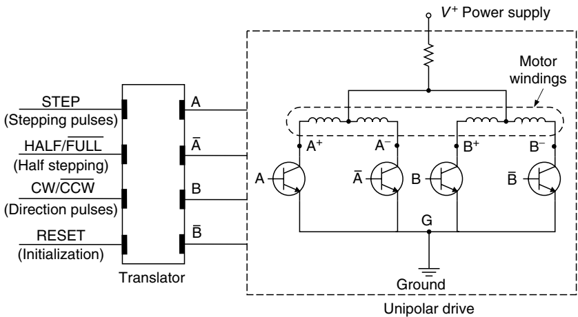
FIGURE 6.17 Basic drive hardware for a two-phase bifilar-wound stepper motor.
