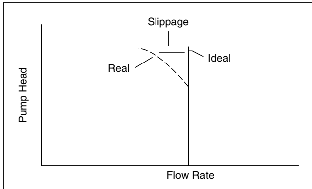
Figure 17.18 Positive-displacement pump characteristic curve.
