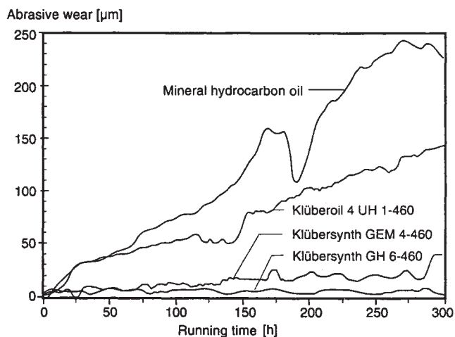
Figure 14-7. Wear curve of mineral hydrocarbon oil compared to synthetic oils.
