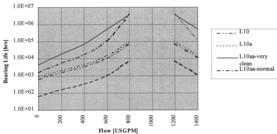
Figure 17-12. Bearing lives and effects of contamination on bearing life—SKF 6212.
