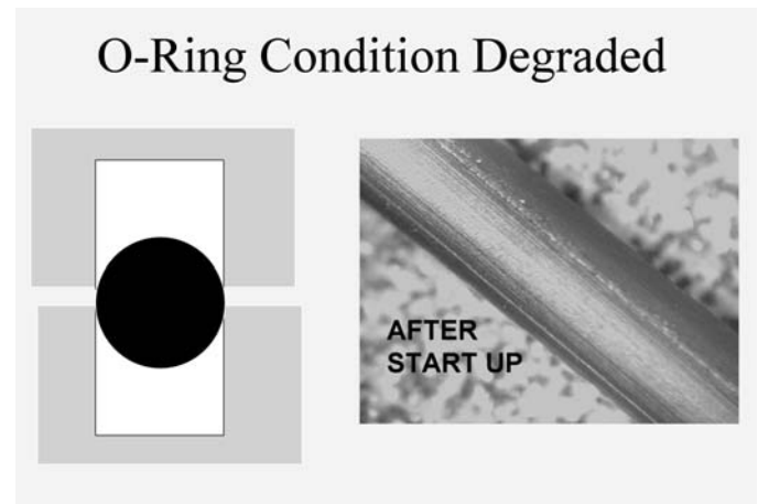
Figure 12-62. O-ring degradation risk with sharp-edged components (Ref. 7)
