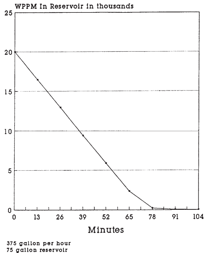
Figure 17-6. Performance simulation for air stripping unit. (Source: Ausdel Pty, Cheltenham, Victoria, Australia)
