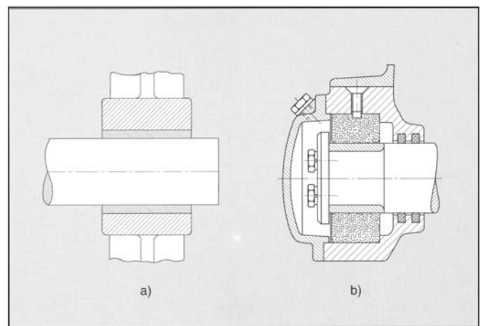
Figure 12-42. Small bearings; a) dry sliding bearing; b) sintered bearing.
