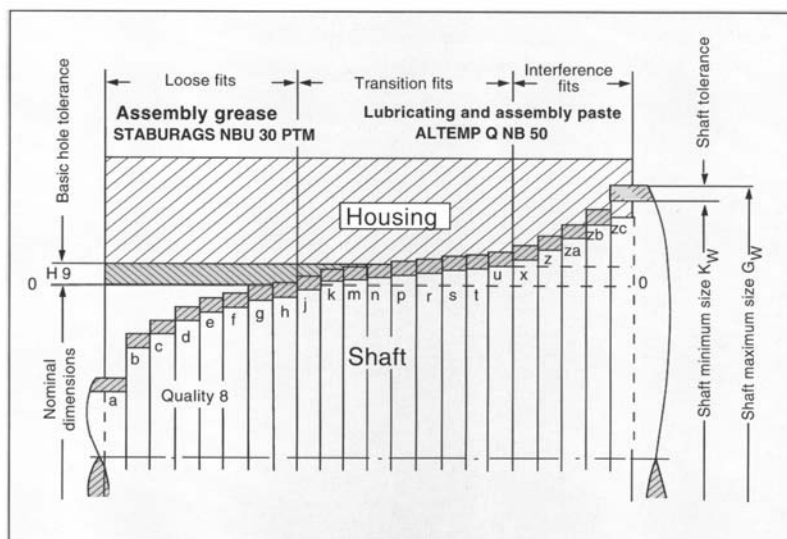
Figure 12-51. Loose fits require different lubricants than interference fits. (Source: Klüber Lubrication North America, Londonderry, New Hampshire.)
