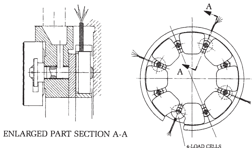
Figure 12-20. Load cells: installation in directed lubrication carrier ring.
