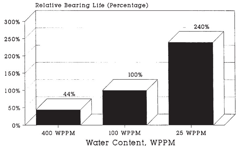
Figure 17-2. Effects of water in lube oil on bearing life.
