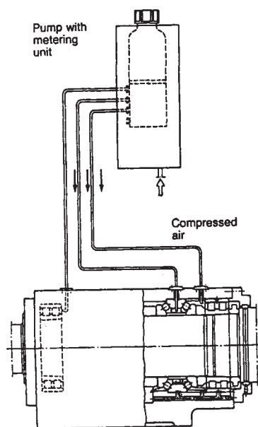
Figure 12-6. Air-oil lubrication schematic.
