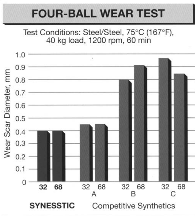
Figure 7-13. Wear test results, SYNESSTIC vs. competitive synthetics.
