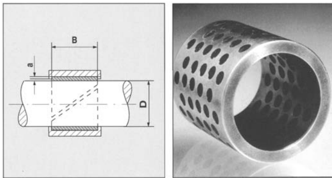
Figure 12-41. Dry-running bearings: sheet bearing (left), having lubricating holes filled (right) with "Klüberdur" tribo-system material.
