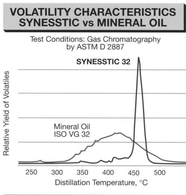
Figure 7-23. There is very little light-end volatility in this diester-base synthetic hydrocarbon lubricant.
