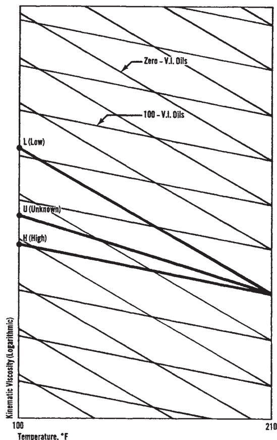
Figure 3-4. The concept of viscosity index.
