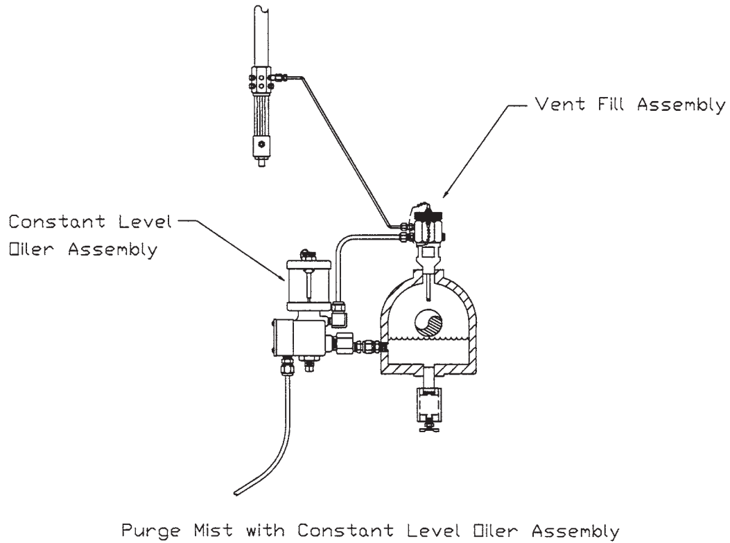
Figure 11-35. Purge mist application using constant level oiler assembly. (Source: Lubrication Systems Company, Houston, Texas.)
