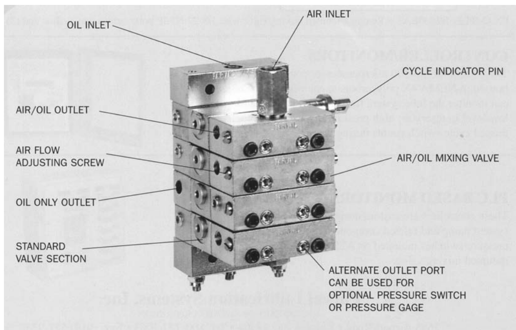
Figure 11-10. Four-section air-oil valve assembly. (Source: Farval Lubrication Systems, Inc., Kinston, North Carolina.)
