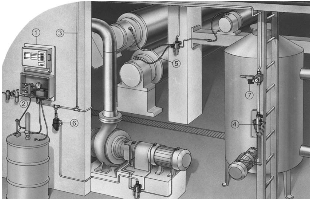
Figure 11-3. Safematic SG1-grease lubrication system, consisting of:
