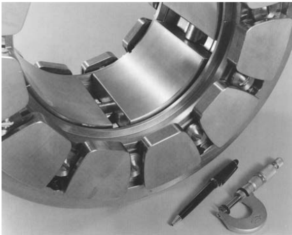
Figure 12-34. Glacier combination thrust/radial tilt pad bearing.
