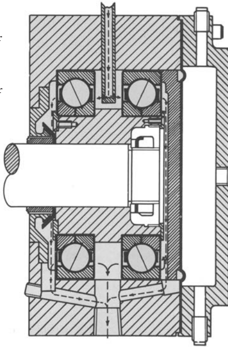
Figure 12-9. Oil mist lubrication applied to a set of split inner ring bearings. (Source: Fafnir Division of Torrington Company, Torrington, Connecticut.)
