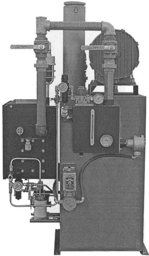
Figure 11-40. Demisting system (closed loop) for the textile industry. (Source: Lubrication Systems Company, Houston, Texas.)
