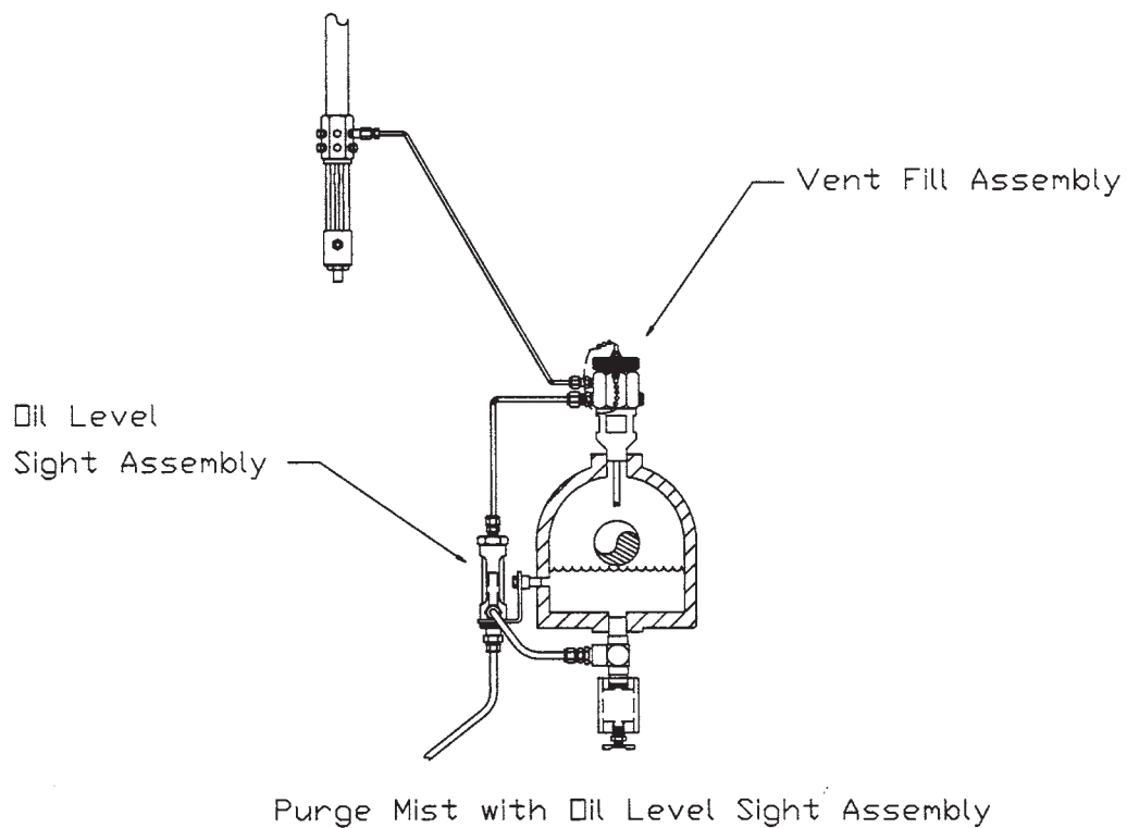
Figure 11-36. Purge mist (wet sump) application using oil level sight glass assembly. (Source: Lubrication Systems Company, Houston, Texas.)
