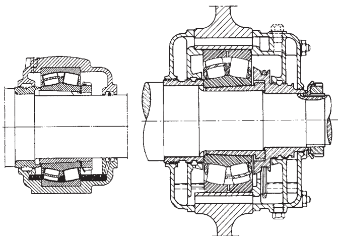
Figure 12-3. Oil bath/oil spray on double row spherical roller bearings. In the oil bath configuration (left), the oil level reaches the center of the rollers at the bottom. In the spray configuration (right), the oil is conveyed to the tapered flinger by an oil ring which dips into the oil bath. An important feature of this application is that the air pressure on both sides of the bearing and enclosures is equalized by connecting ducts. This prevents leakage of the lubricant when the housings are located in an air stream.
