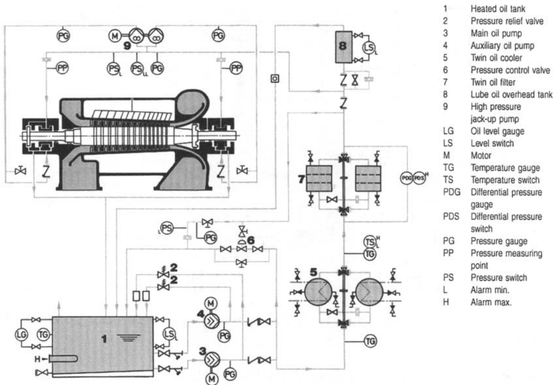
Figure 15-13. Typical lube oil schematic for turbomachinery. (Source: Mannesmann-Demag, Duisburg, Germany)
