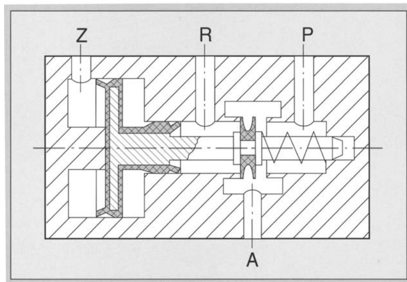
Figure 12-58. Pneumatic valves.
