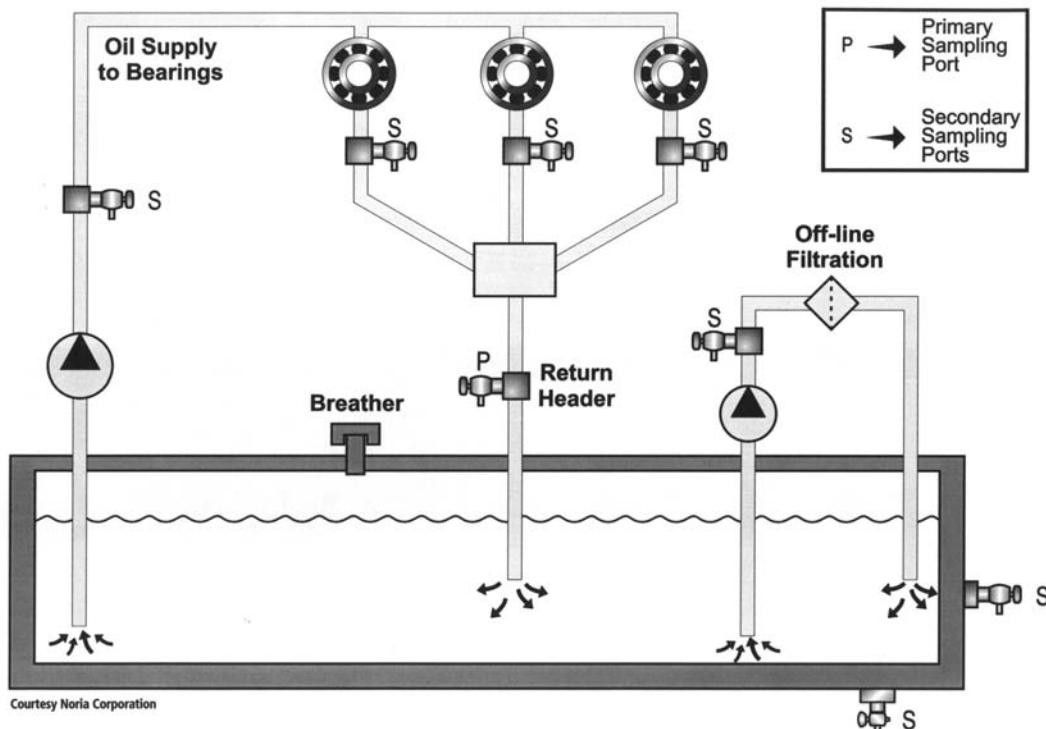
Figure 19-2. Circulating oil system indicating recommended sampling points.
