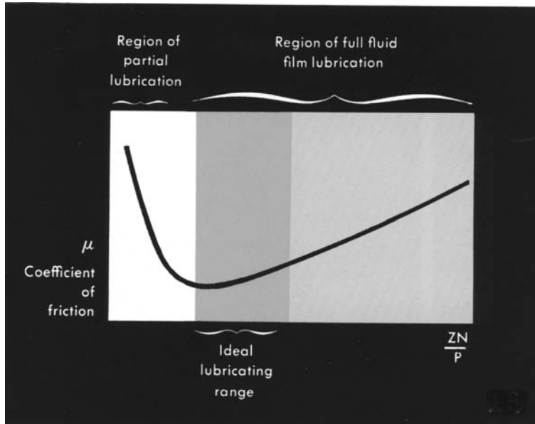
Figure 1-15. Bearing performance.
