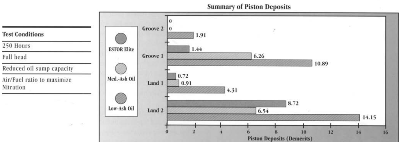
Figure 15-23. Performance comparison, ESTOR Elite gas engine oil.
