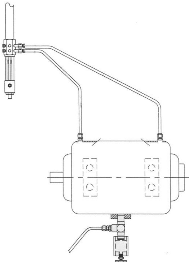
Figure 11-34. Mist manifold and stainless steel tubing directing oil mist to two application points in a bearing housing.
