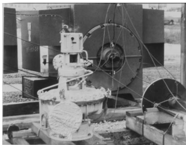
Figure 18-7. Construction site storage oil mist supply lines to a vertical mechanical drive turbine and large electric motor.
