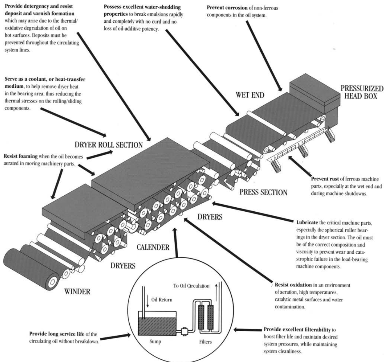
Figure 8-1. Typical paper machine.
