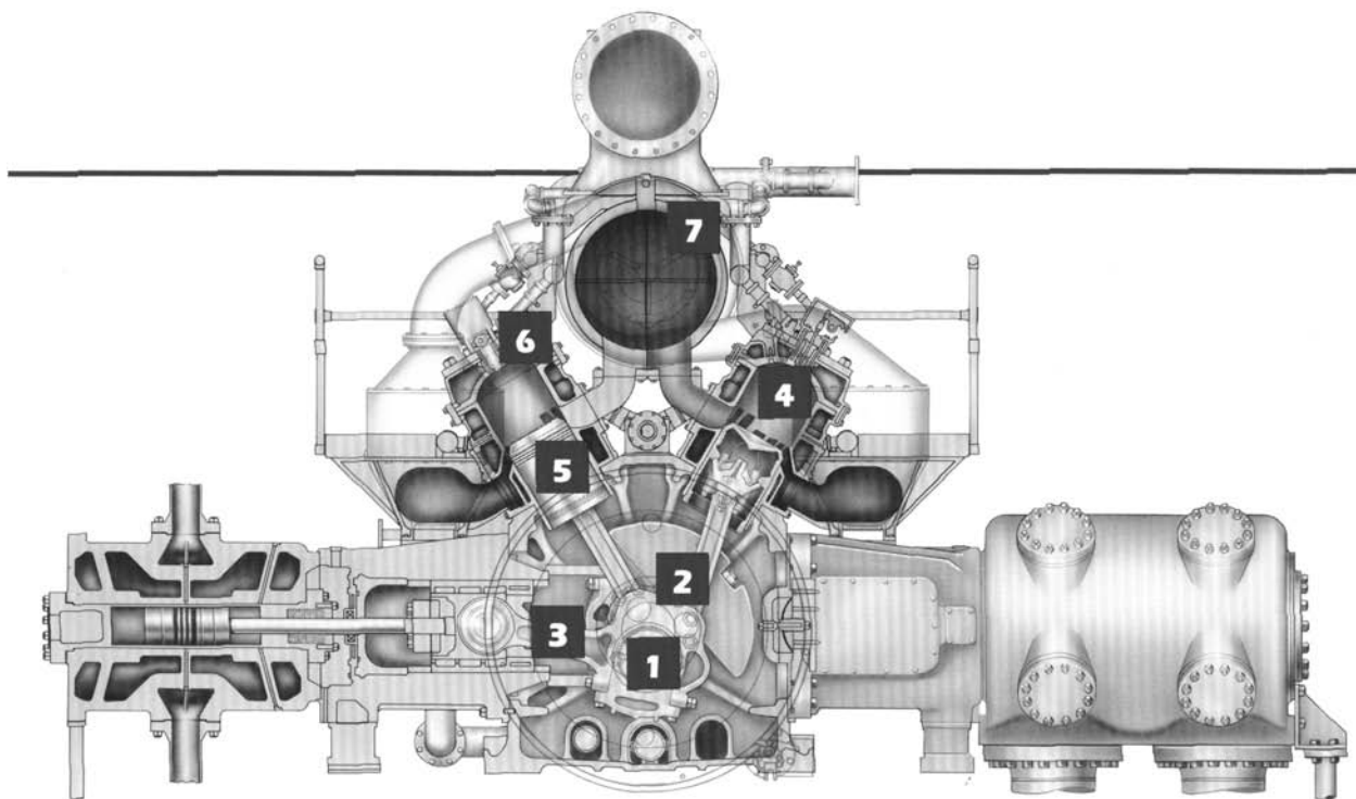
Figure 15-20. This Cooper-Bessemer model V-250 with 16 power cylinders is rated at 5500 hp. Unit is equipped with eight GT pipeline cylinders and is on transmission duty in New York State.
