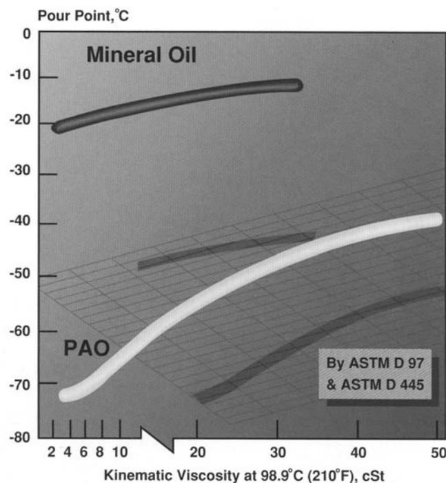
Figure 7-7. PAO-based synthetics have superior cold-weather performance. (Source: Exxon Company, USA, Houston, Texas.)
