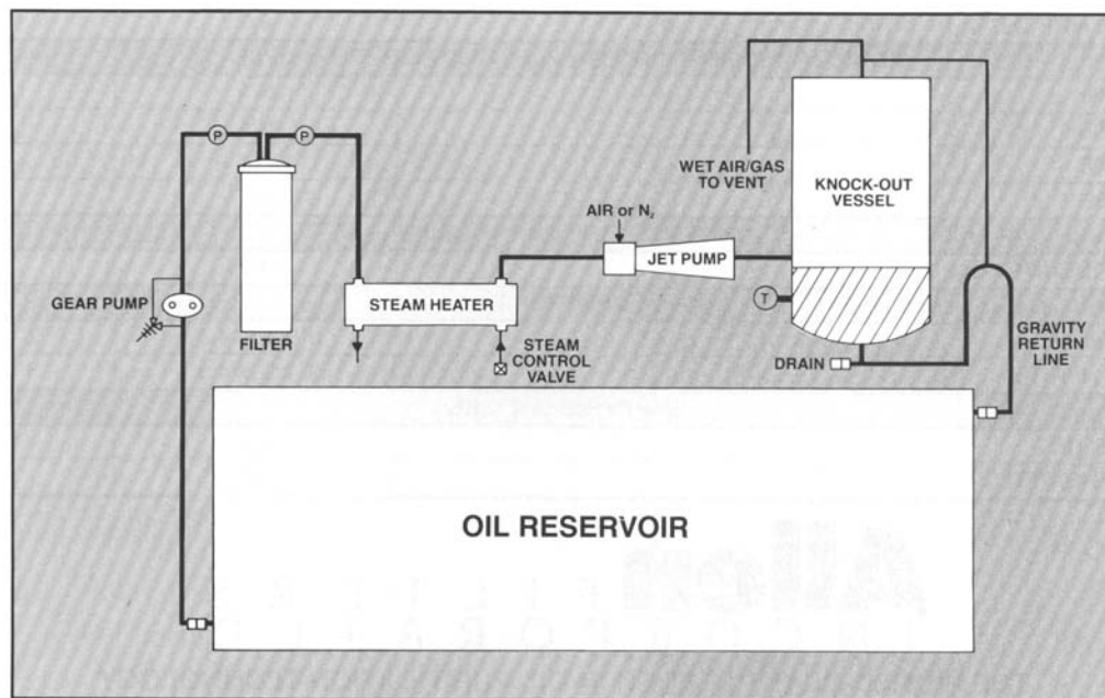
Figure 17-4. Simplified diagram of air stripping unit. (Source: Ausdel Pty, Cheltenham, Victoria, Australia)
