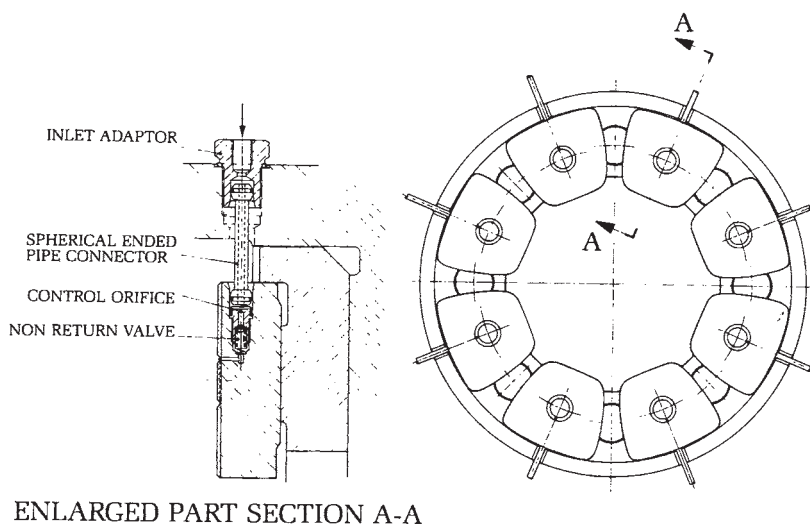
Figure 12-23. Jacking oil system in thrust bearing.
