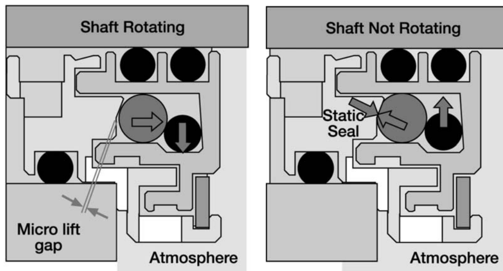
Figure 12-63. Advanced rotating labyrinth-type bearing housing seal (Source: AESSEAL plc, Rotherham, UK and Knoxville, TN)
