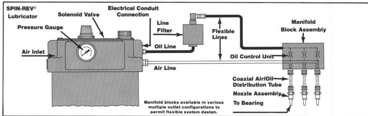
Figure 11-11. Air-oil lubrication systems with coaxial delivery tubing. (Source: Bijour Lubricating Corporation, Bennington, Vermont.)
