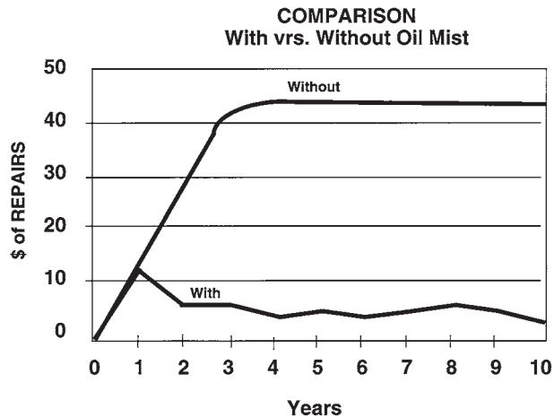
Figure 11-24. Repair cost comparison for 2 identical petrochemical facilities, with vs. without oil mist lubrication.
