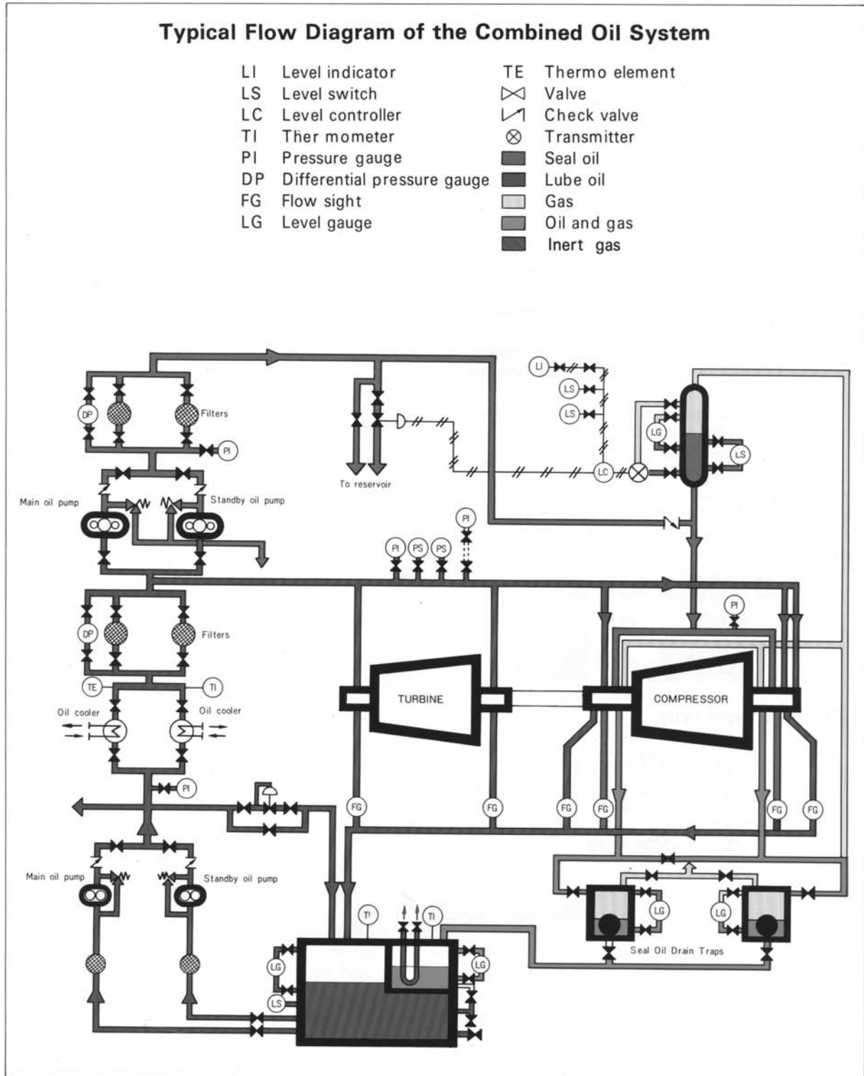
Figure 15-16. Combined lube and seal oil system for turbo compressors. (Source: Hitachi, Tokyo, Japan)
