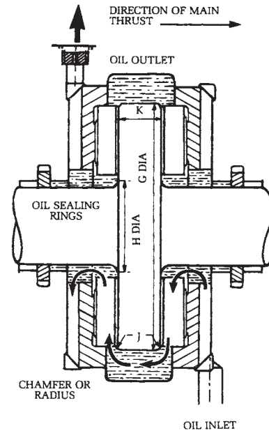
Figure 12-12. Flooded lubrication: typical double thrust arrangement.
