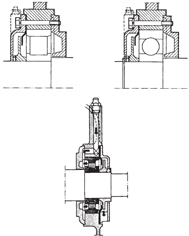
Figure 12-2. Advantageous, simple grease escape "valve." (Arrangements found in ASEA Electric Motors.)
