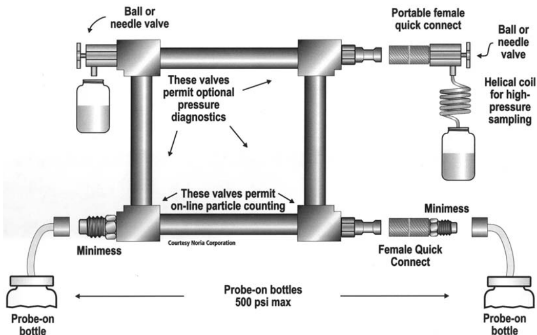
Figure 19-4. More options for taking lube oil samples.
