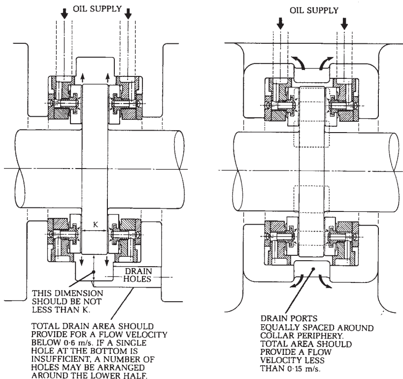
Figure 12-15. Directed lubrication: typical double thrust arrangements designed to prevent bulk oil from contacting the collar.
