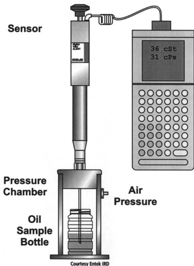
Figure 19-10. Absolute viscometer for plant use.
