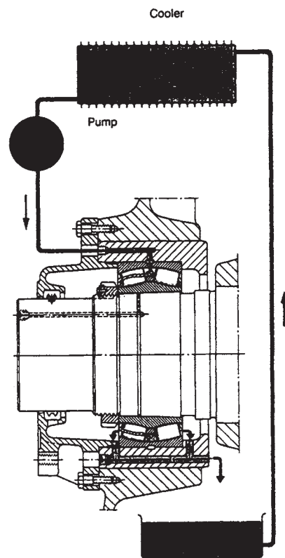
Figure 12-4. Circulating oil lubrication.
