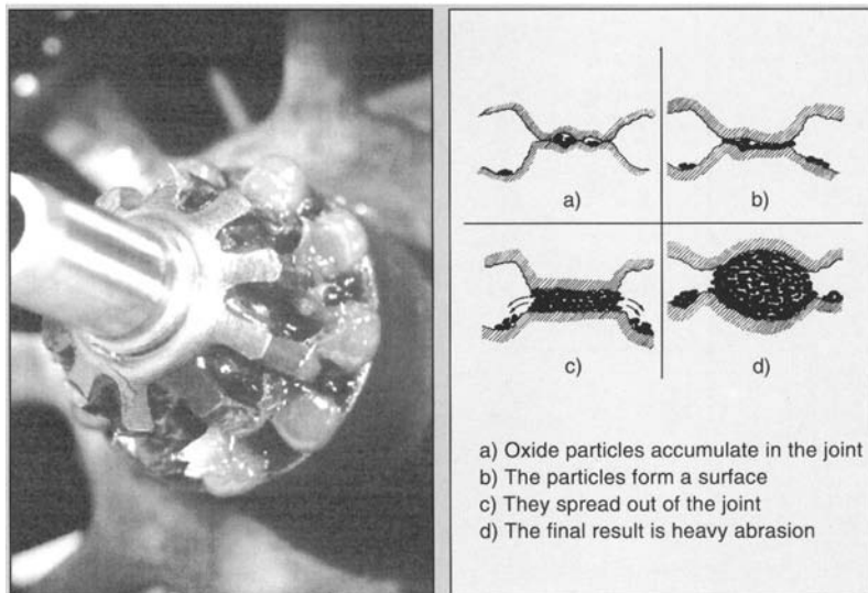
Figure 12-50. Lubrication of a multiple spline shaft and formation of fretting corrosion.
