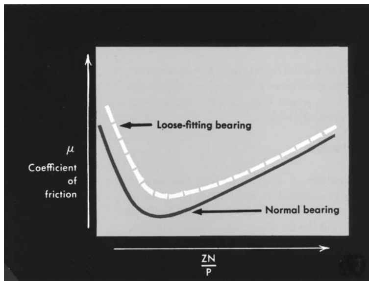
Figure 1-17. Loose-fitting bearings require high-viscosity oils.
