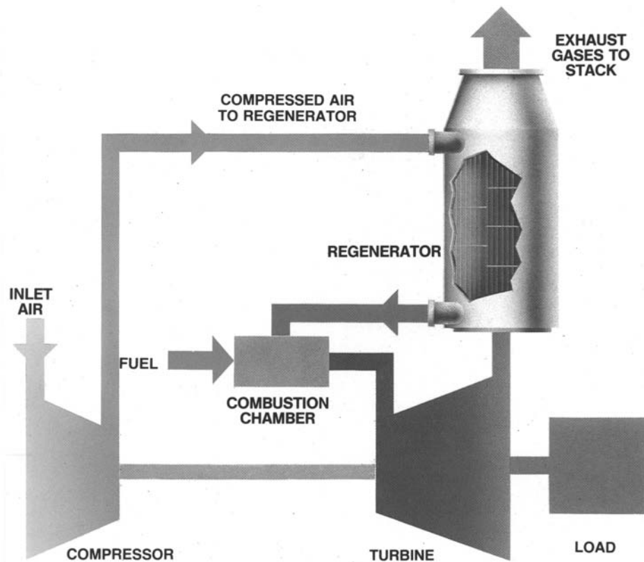
Figure 16-11. Gas turbine regenerative cycle diagram. (Source: Nuovo Pignone, Florence, Italy)
