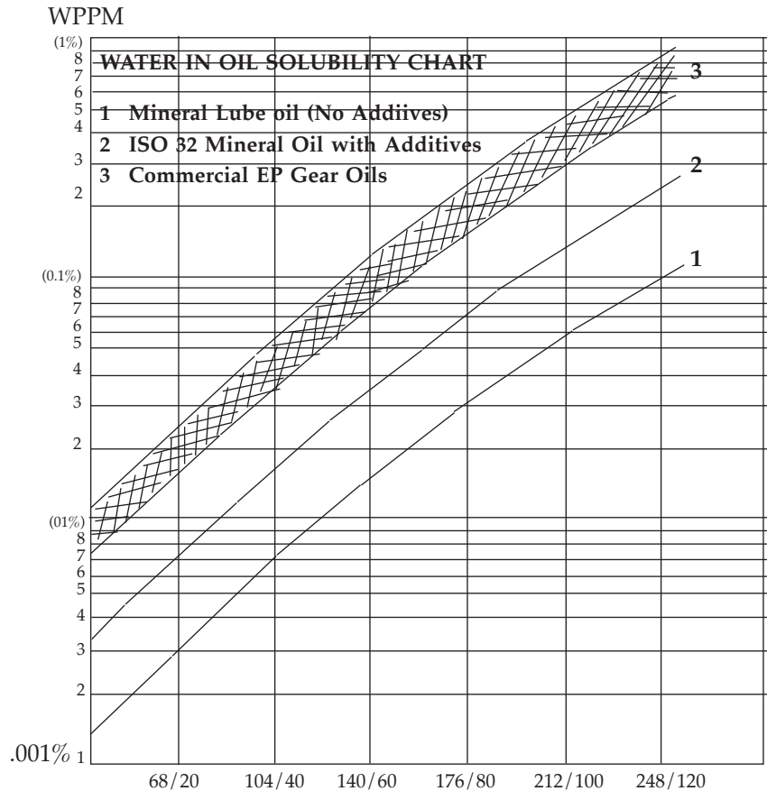
Figure 17-1. Solubility chart for water in oil.
