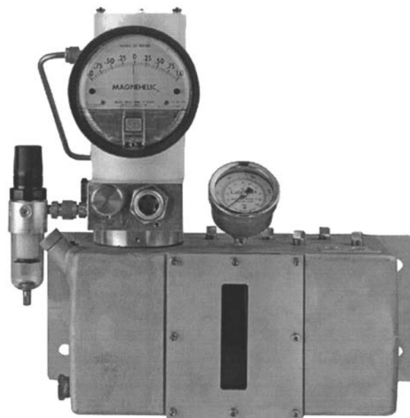
Figure 11-41. Miniaturized closed-loop oil mist system, or “single-machine lubricator.” (Source: Lubrication Systems Company, Houston, Texas.)
