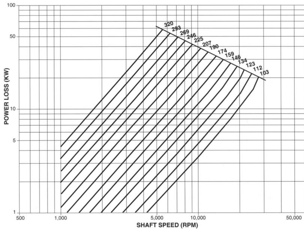
Figure 12-28. Frictional loss for single element 8-pad "LEG" bearings.
