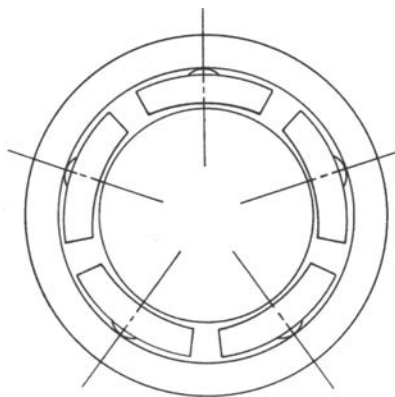
Figure 12-31. Tilting-pad journal bearing, converging geometry.
