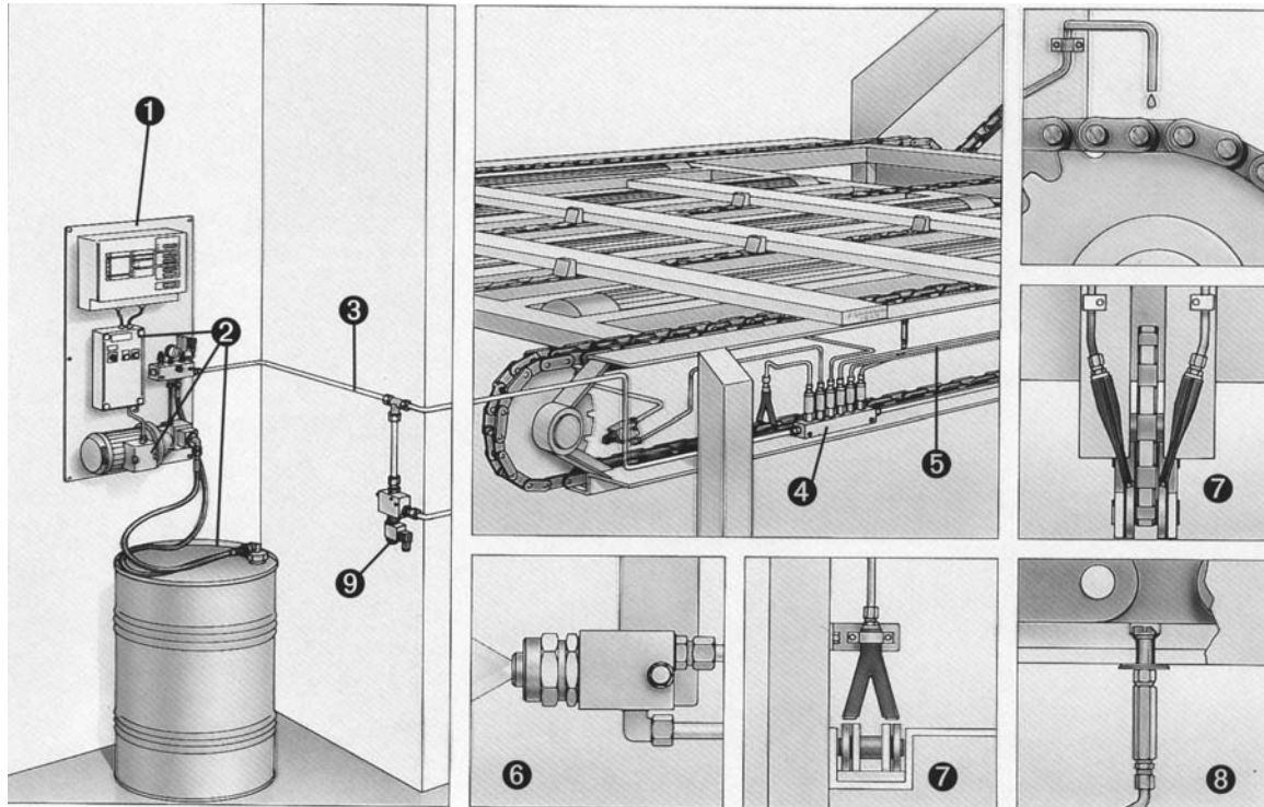
Figure 11-6. Open, centralized oil lubrication system. (Source: Safematic, Inc., Alpharetta, Georgia, and Muurame, Finland.)
