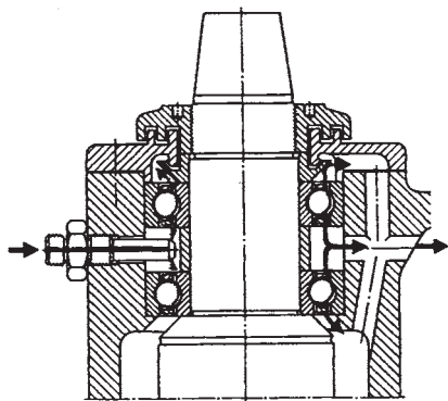
Figure 12-5. Oil-jet lubrication allows bearings to operate at lower temperature or at higher speeds than any other method of lubrication.
