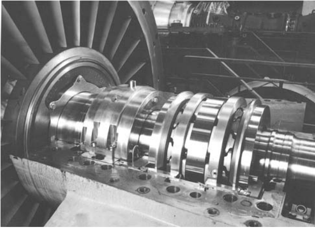
Figure 12-14. Glacier double thrust bearing size 10293 with directed lubrication installed in an ABB gas turbine. (Photo: ABB, Baden, Switzerland.)
