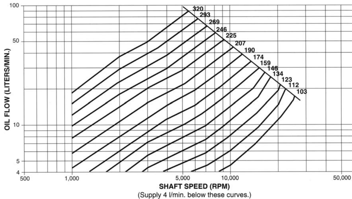
Figure 12-29. Recommended lubricant supply for single element 8-pad "LEG" bearings.
