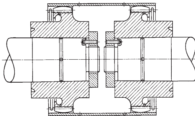
Figure 14-17. Section through a tooth-type coupling. (Source: ASEA Brown-Boveri, Baden, Switzerland)
