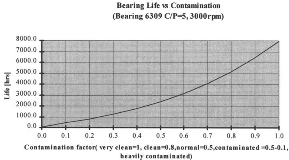
Figure 17-8. Influence of contamination on bearing life.
