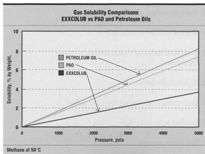
Figure 15-17. Gas solubility comparisons—EXXCOLUM vs. PAO and petroleum oils.
