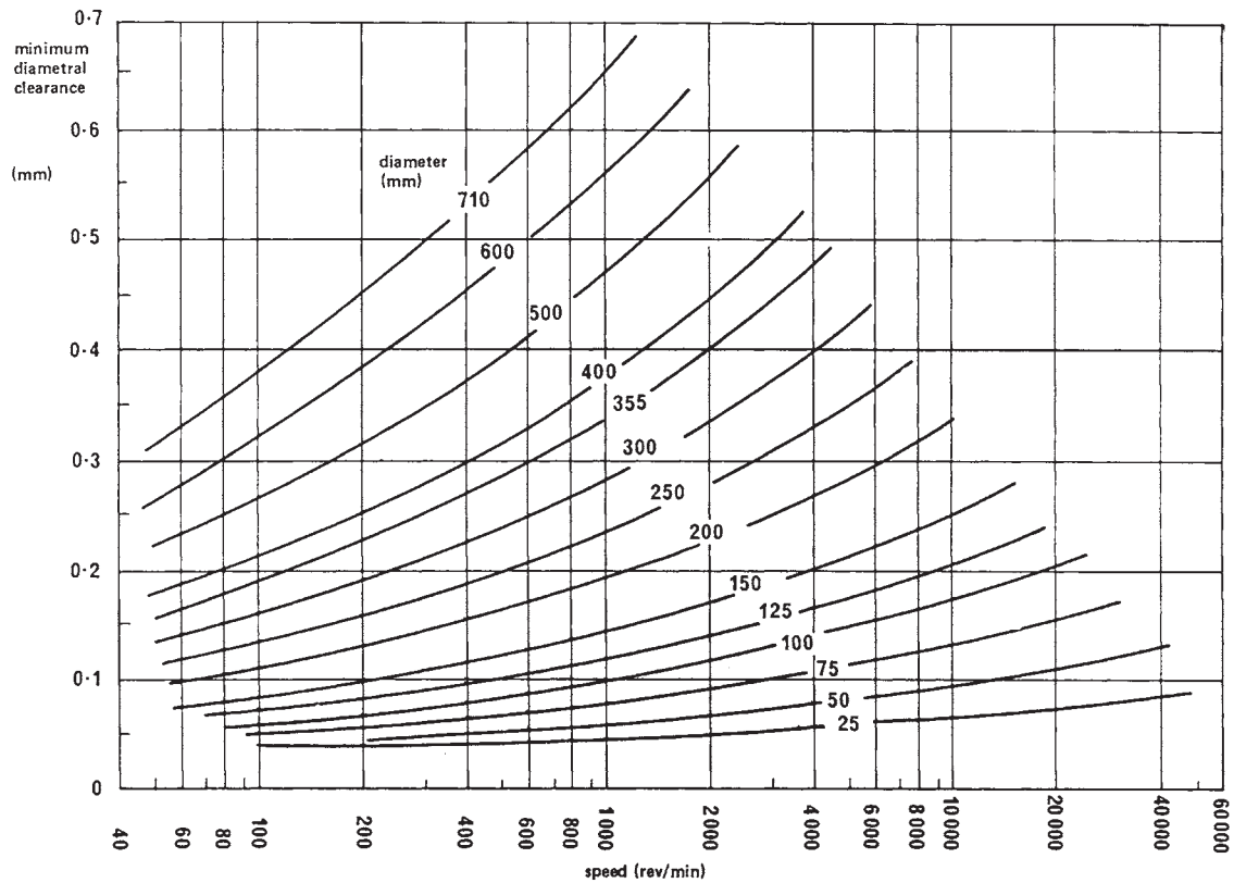
Figure 12-40. Hydrodynamic bearing clearances: recommended minima against speed by shaft diameter.
