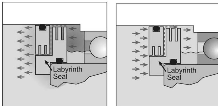
Figure 12-59. "Breathing out" warm air and "breathing in" cooler ambient air
