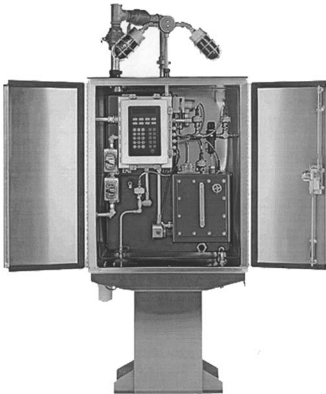
Figure 11-28. Central oil mist generator and supply tank. (Source: Lubrication Systems Company, Houston, Texas.)
