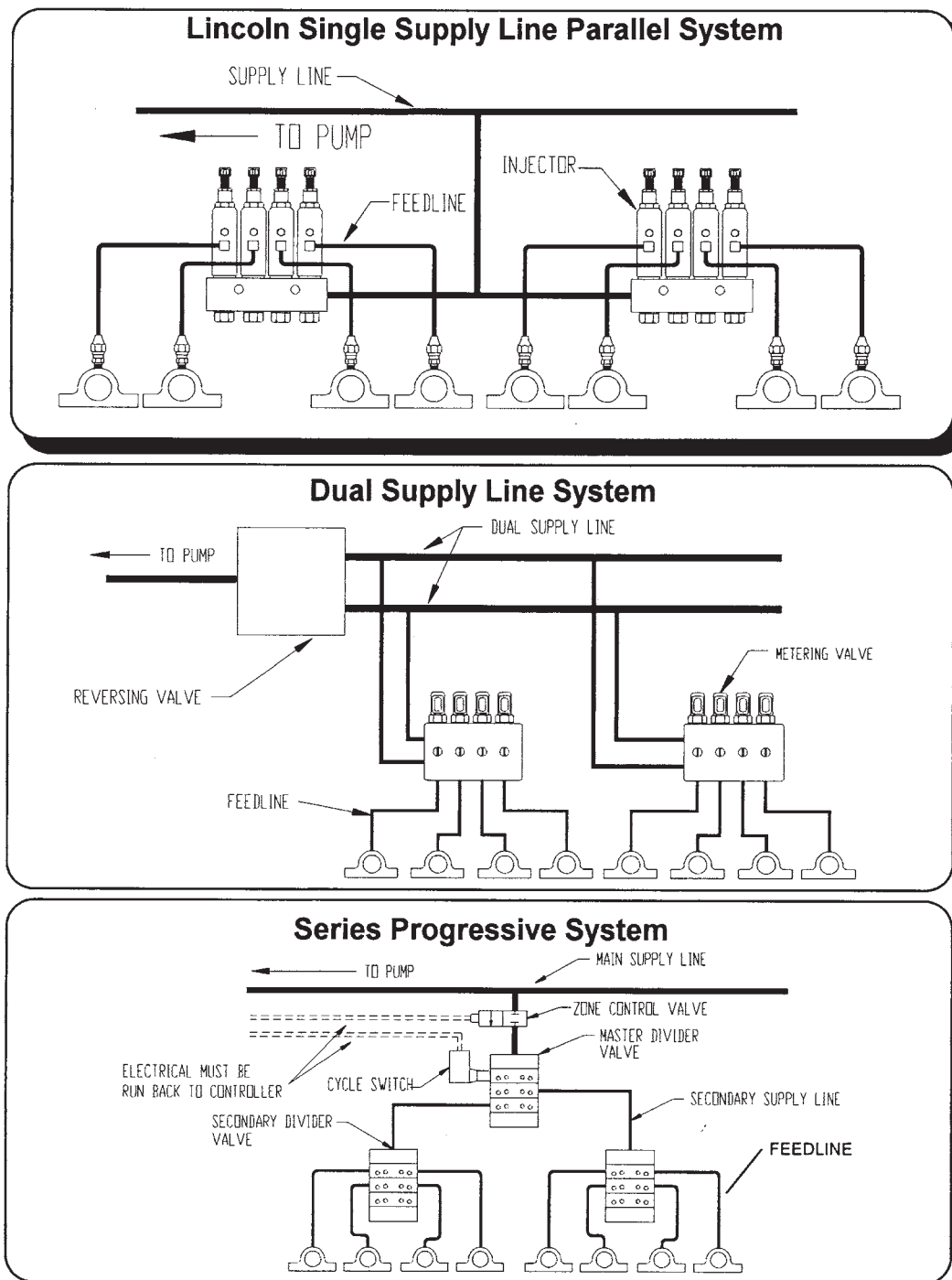
Figure 11-2. Different versions of automated centralized grease systems. (Source: Lincoln Company, St. Louis, Missouri.)
