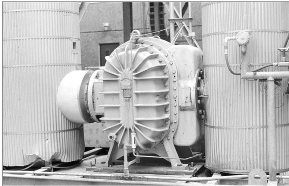
Fig. 14-19: Roots-type positive displacement blower at a petrochemical plant. (Source: Lubrication Systems Company, Houston, Texas)
