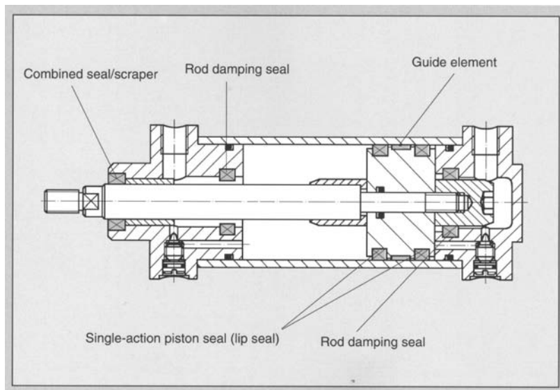
Figure 12-57. Pneumatic cylinder.
