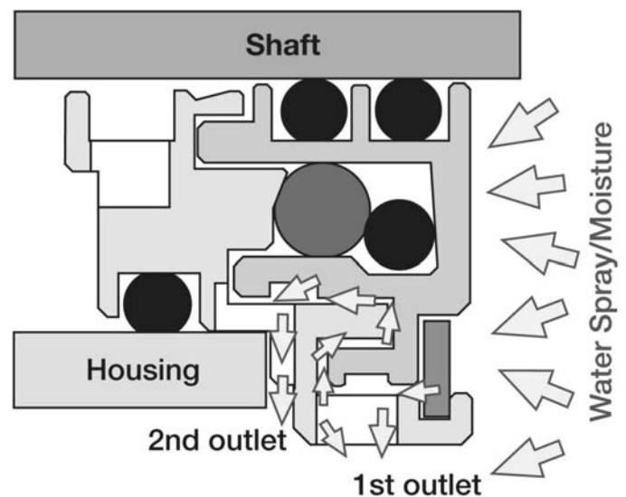
Figure 12-65. Multi-tiered arrangement (tortuous path) and multiple expulsion orifices of modern, field-repairable rotating labyrinth seal (Source: AESSEAL plc, Rotherham, UK, and Knoxville, Tennessee)
