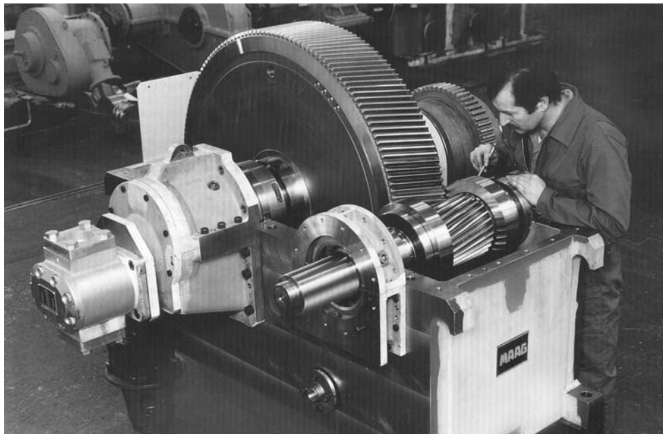
Figure 14-1. Single-helical, high-speed gear unit being assembled. (Source: Maag Gear Company, Zurich, Switzerland)
