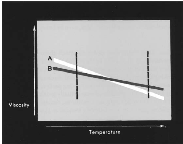
Figure 1-19. For the same temperature change, the viscosity of oil "B" changes much less than that of oil "A."
