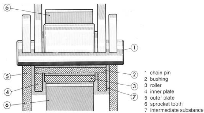
Figure 12-48. Chain components.
