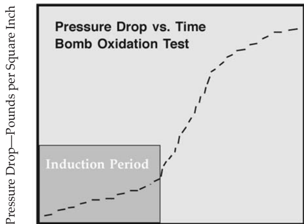
Figure 3-1. When pressure drop is plotted against time, the resulting curve will indicate a period of comparatively slow oxidation followed by a pronounced rise. The relatively flat portion at the beginning represents what is known as the "induction period," a phase during which oxidation is not ordinarily of serious magnitude. For practical reasons, it is not customary to continue the test beyond the induction period, its end being indicated by a sudden rise. Should the test be carried further, however, this rise would eventually taper off again as oxidation becomes complete. In some cases, test results have been expressed in terms of the duration of the induction period.
