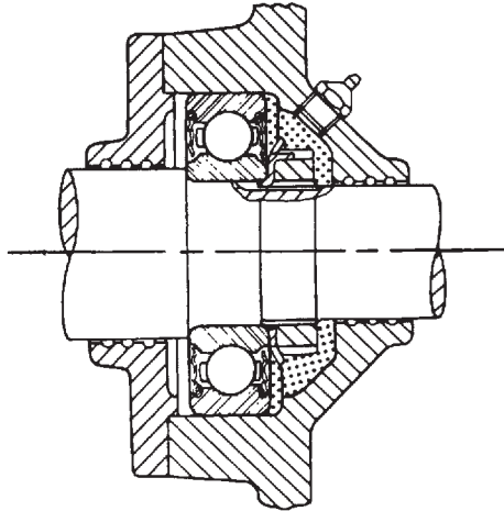
Figure 13-1. Shielded, grease-lubricated bearing.
