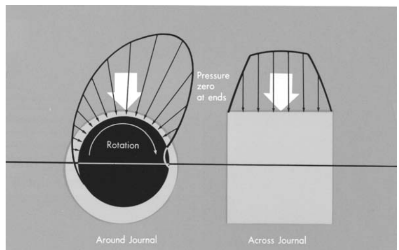
Figure 1-11. Oil pressure distribution diagrams.
