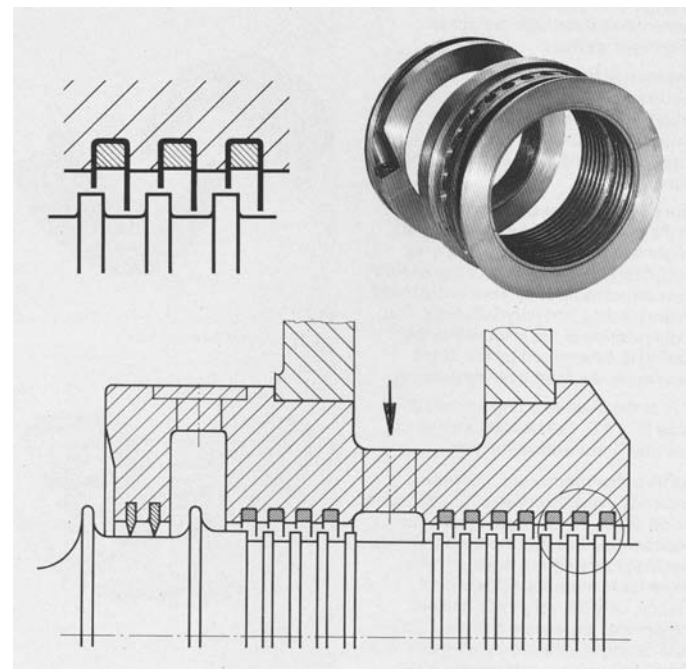
Figure 16-8. Labyrinth-type steam seals for Siemens steam turbines. An air purge can be introduced into the space between sealing groups (arrow).
