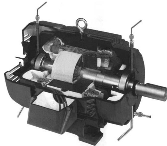
Figure 13-10. Oil mist applied to the same side of a bearing is not providing optimal lubrication; much of the mist is simply flowing from entry to drain.
