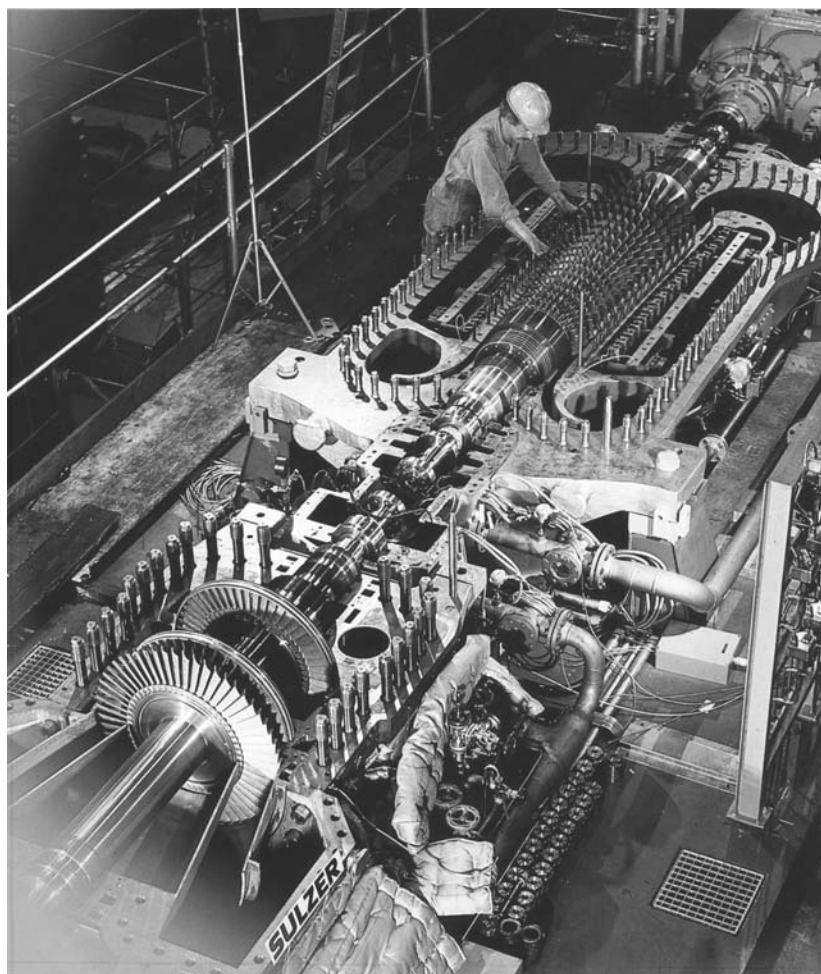
Figure 15-3. Turbotrains assembly in progress. (Source: Sulzer Brothers, Winterthur, Switzerland)
