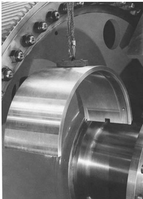
Figure 12-39. Lowering a large Glacier medium wall bearing into a marine propulsion gearbox. (Photo: GEC Alsthom Gears Ltd.)
