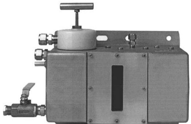
Figure 11-38. Oil collection container with manually operated pump. (Source: Lubrication Systems Company, Houston, Texas.)
