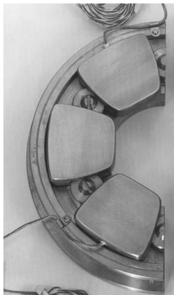
Figure 12-17. Glacier bearing fitted with thermocouples ready for high-speed petrochemical application. Note half pad stops which avoid handling loose pads on assembly.
