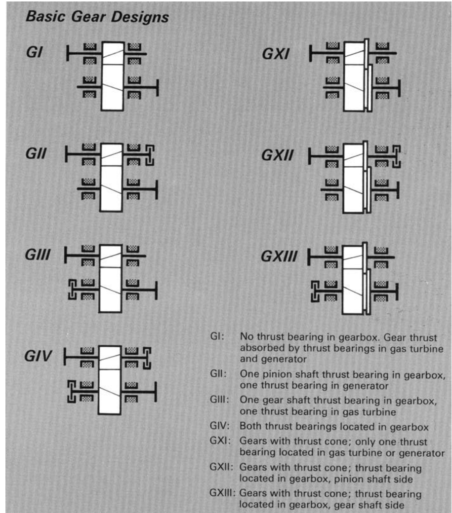
Figure 14-3. Basic gear designs. (Source: Maag Gear Company, Zurich, Switzerland)
