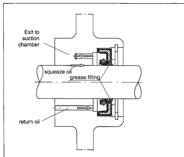
Sealing against pressure (example: oil pump)
