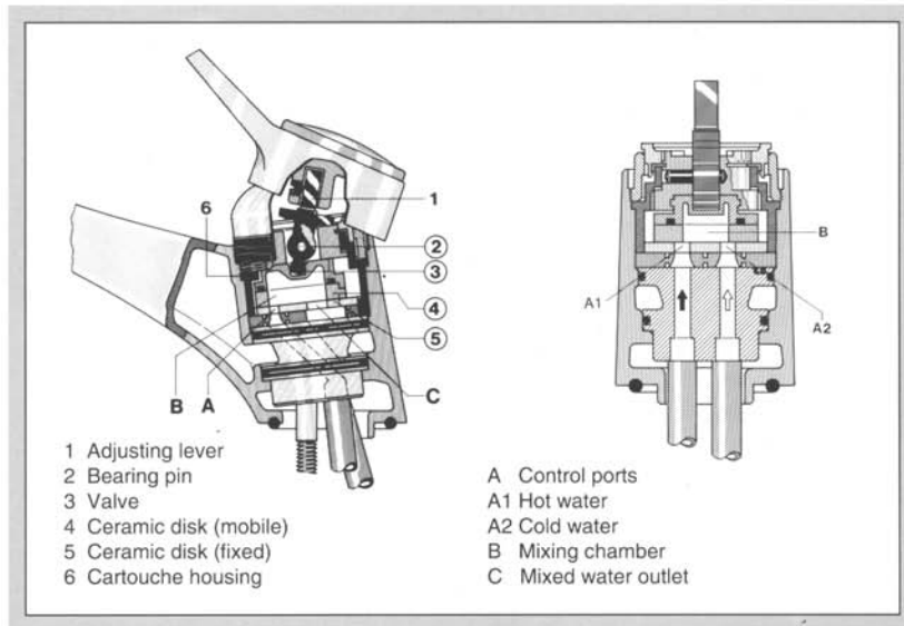
Single-lever mixer tap with ceramic disks (② - ⑤ = lubricated)
