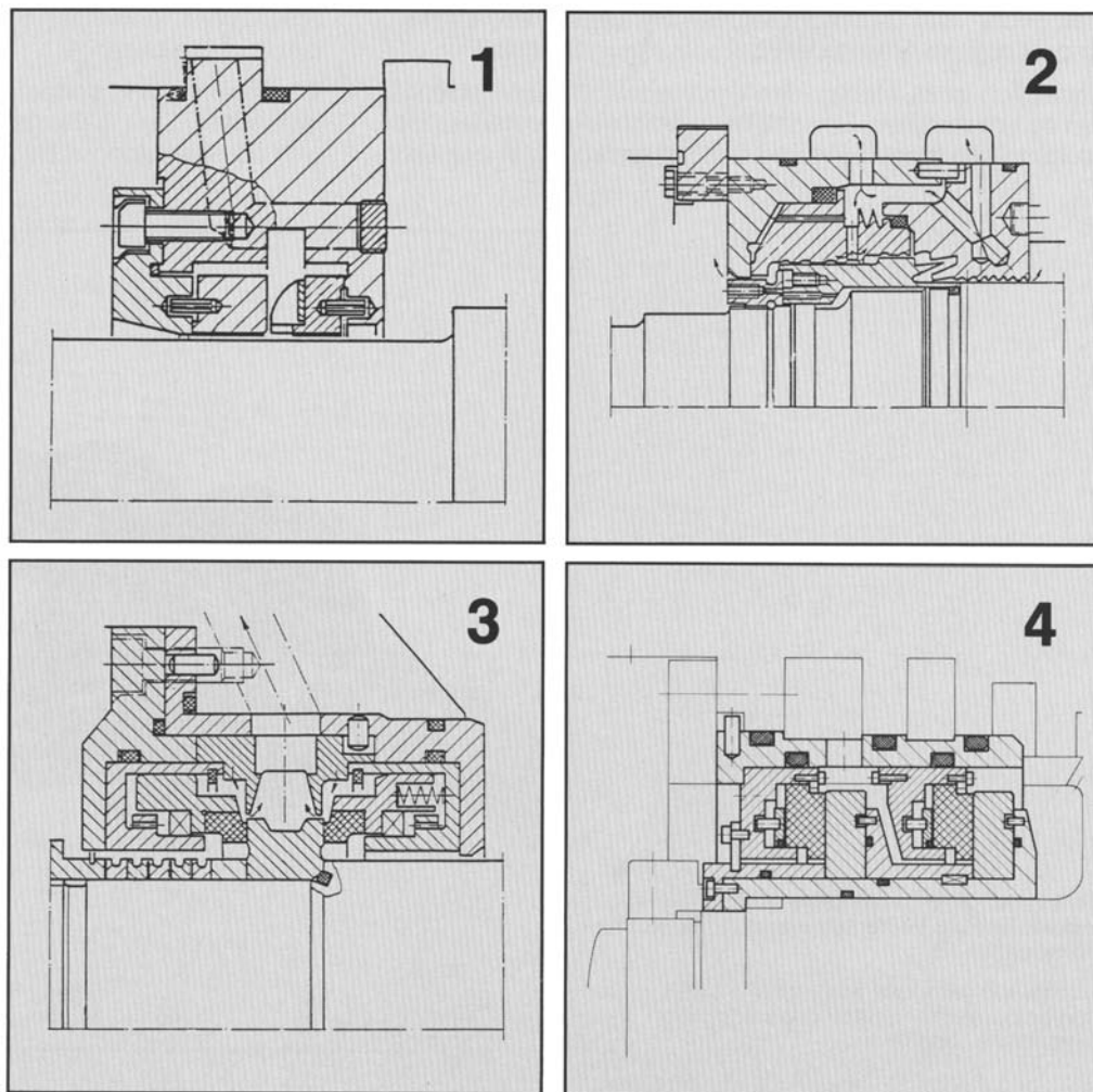
Figure 15-4. Seal geometries typically incorporated in dynamic compressors: 1 Floating ring seal; 2 Trapped bushing seal; 3 Liquid-lubricated mechanical contact seal; 4 Dry gas face seal. (Source: GHH-Borsig, Berlin, Germany)
