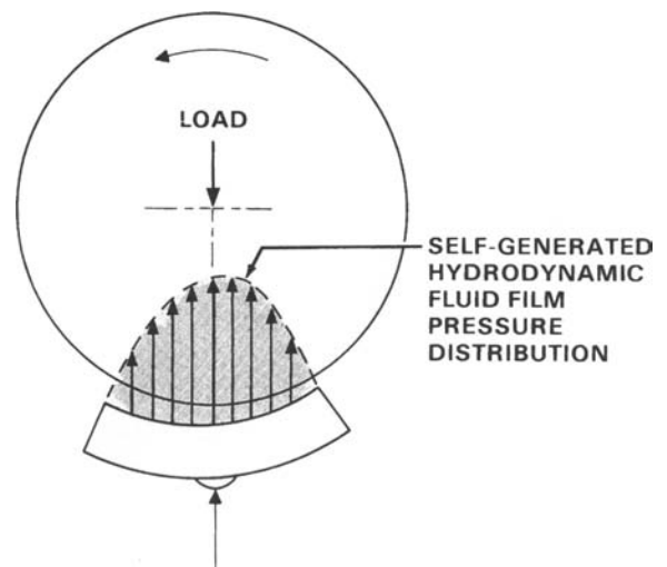
Figure 12-32. Geo-metry and pressure.
