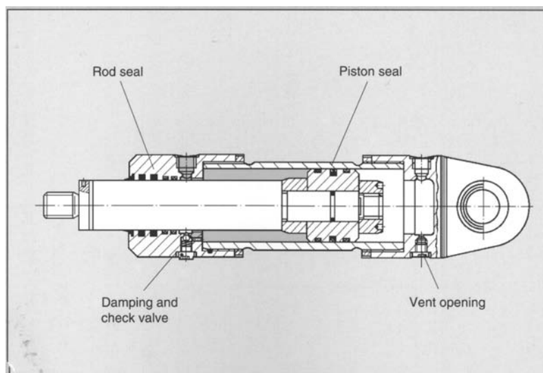
Figure 5-1. Hydraulic cylinder. (Source: Klüber Lubrication North America, Inc., Londonderry, New Hampshire)
