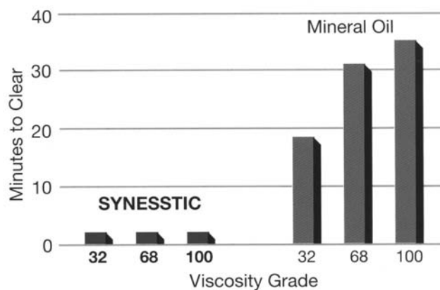
Figure 7-22. Diester-base lubricants will release entrained air much more rapidly than mineral oils.
