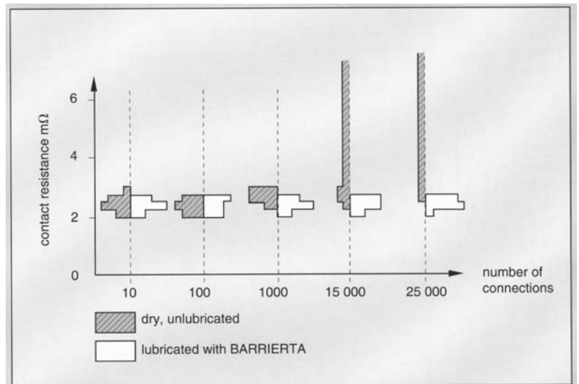
Figure 12-55. Advantages of a lubricated, gold-plated plug contact as a function of the number of connections.
