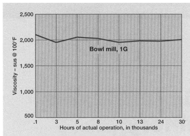
Figure 7-2. Viscosity stability of synthetic lubricant in bowl mill gear unit.
