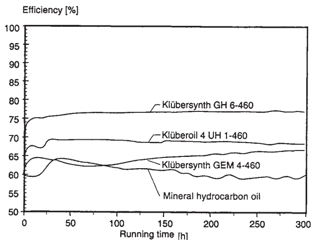
Figure 14-6. Efficiency of mineral hydrocarbon oil compared to synthetic oils.
