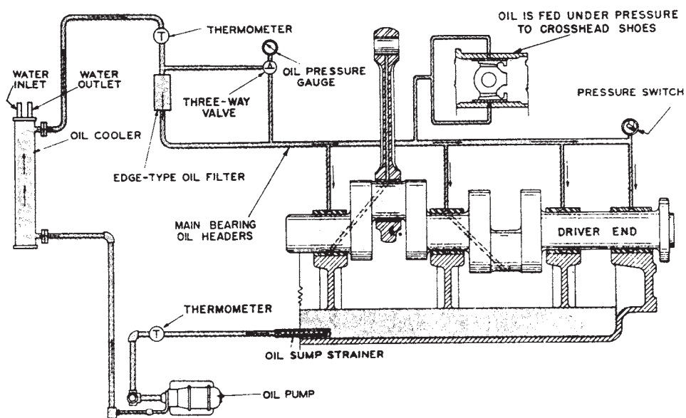
Figure 15-14. Reciprocating compressor lube oil system. (Source: Dresser-Rand, Painted Post, New York)
