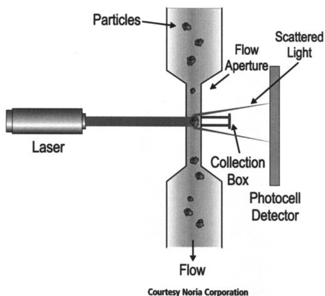
Figure 19-13. Particle counter.
