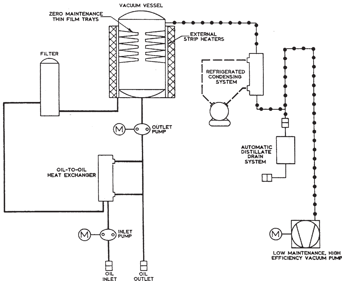
Figure 17-3. Schematic view of vacuum dehydrator. (Source: Allen Filters, Inc., Springfield, Missouri)
