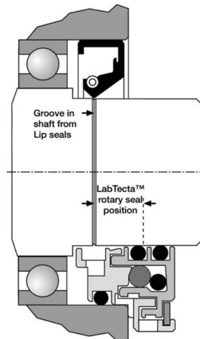
Figure 12-61. Relative location of lip seal (upper view) v. advanced, field-repairable rotating labyrinth seal (lower view). Two O-rings clamp the seal to the shaft in a region not previously damaged by the lip seal (Source: AESSEAL plc, Rotherham, UK and Knoxville, TN)
