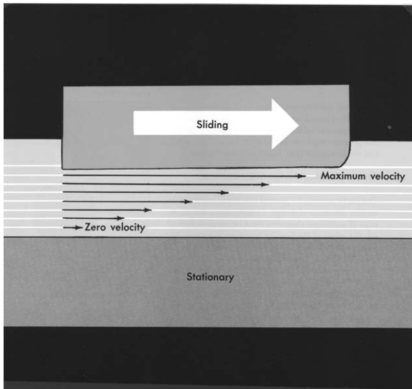
Figure 1-13. Fluid bearing friction is the drag imposed by one layer of oil sliding upon another.
