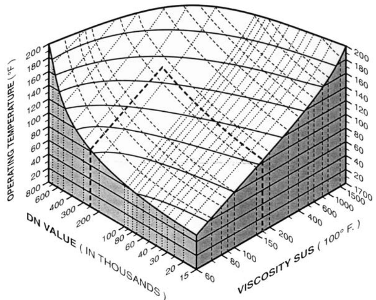
Figure 12-10. Simplified oil viscosity selection chart.
