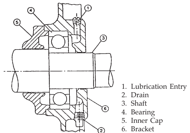
Figure 13-4. High load and/or high speed bearings are often supplied without shield, as shown.
