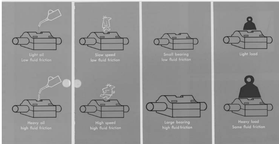
Figure 14. Factors that affect bearing friction under full-fluid-film lubrication.
