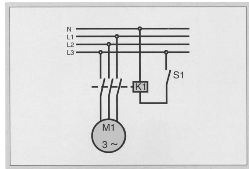
Simplified connection diagram depicting a three-phase motor switched on/off by a contactor K 1 via a manual switch S 1
