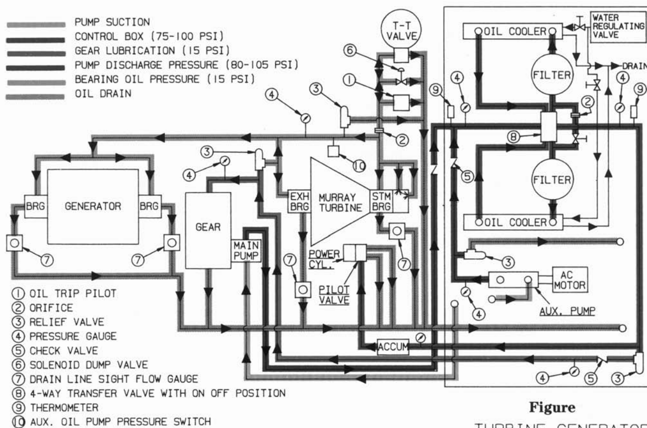
Figure 16-7. Turbine-generator lube system (typical).
