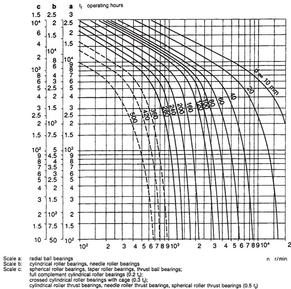
Figure 12-1. Grease relubrication intervals as a function of bearing type, size, and speed. (Source: SKF America, Kulpville, Pennsylvania.)
