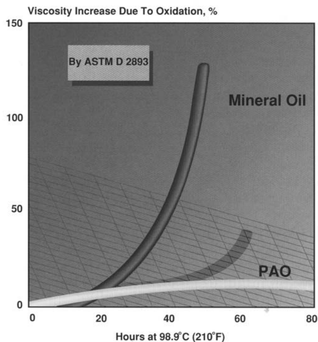
Figure 7-5. Viscosity increase due to oxidation, mineral oil vs. synthetic EP product. (Source: Exxon Company, USA, Houston, Texas.)
