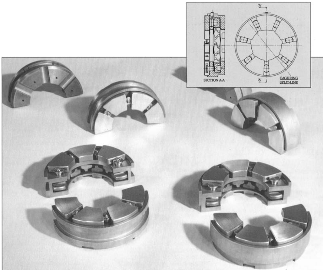
Figure 12-13. Glacier's standard 7 series bearings for both flooded and directed lubrication.
