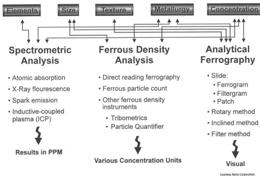
Figure 19-17. Three common categories of wear particle detection.
