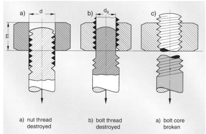
Figure 12-44. Screw connections that are too tightly preloaded tend to fail.
