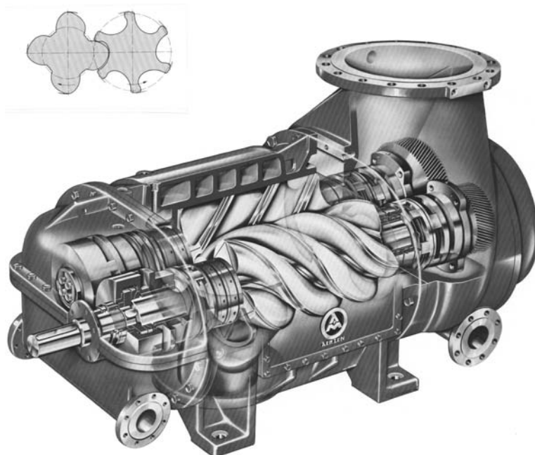
Figure 15-11. Helical screw compressor. (Source: Aerzen USA, Coatesville, Pennsylvania).
