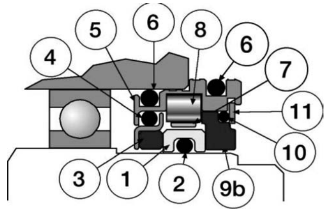
Figure 12-64. Dual-face magnetic seal and O-rings (2, 4, 6, 10), snap ring (11), rotating face (1), stationary faces (3, 9b), stationary magnets (8), magnet carrier (7), and outer body (5). (Source: AESSEAL plc, Rotherham, UK, and Knoxville, Tennessee)
