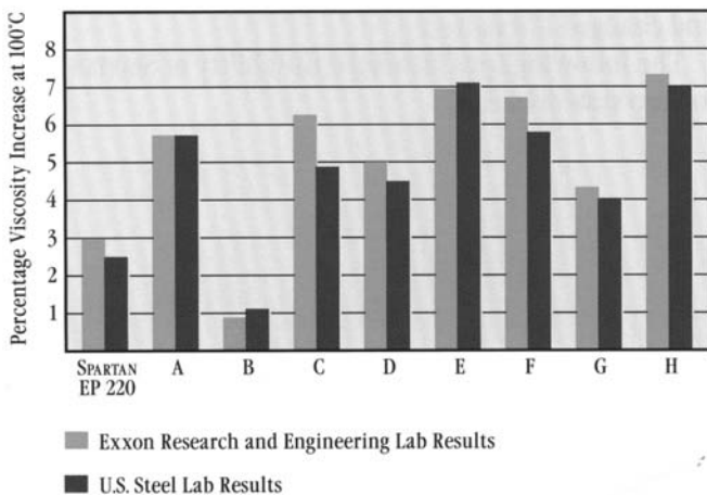
Figure 14-11. SPARTAN EP: low additive depletion results in extended life.
