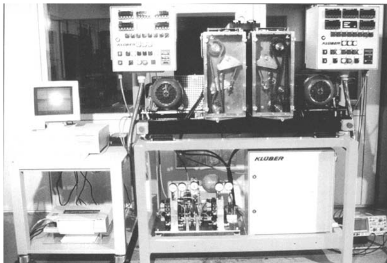
Figure 12-49. Chain test rig at Klüber laboratories.
