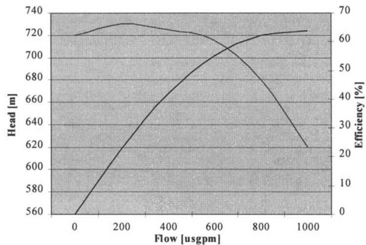
Figure 17-9. Performance curves.
