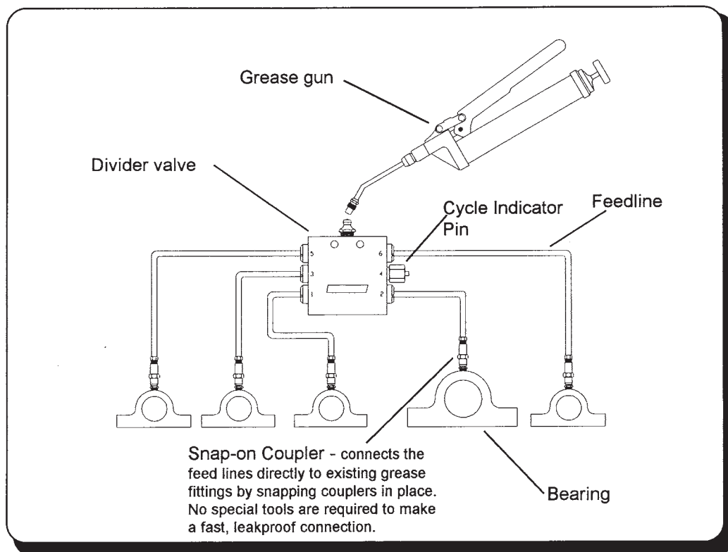
Figure 11-1. Simple centralized grease lubrication system. (Source: Lincoln Company, St. Louis, Missouri.)
