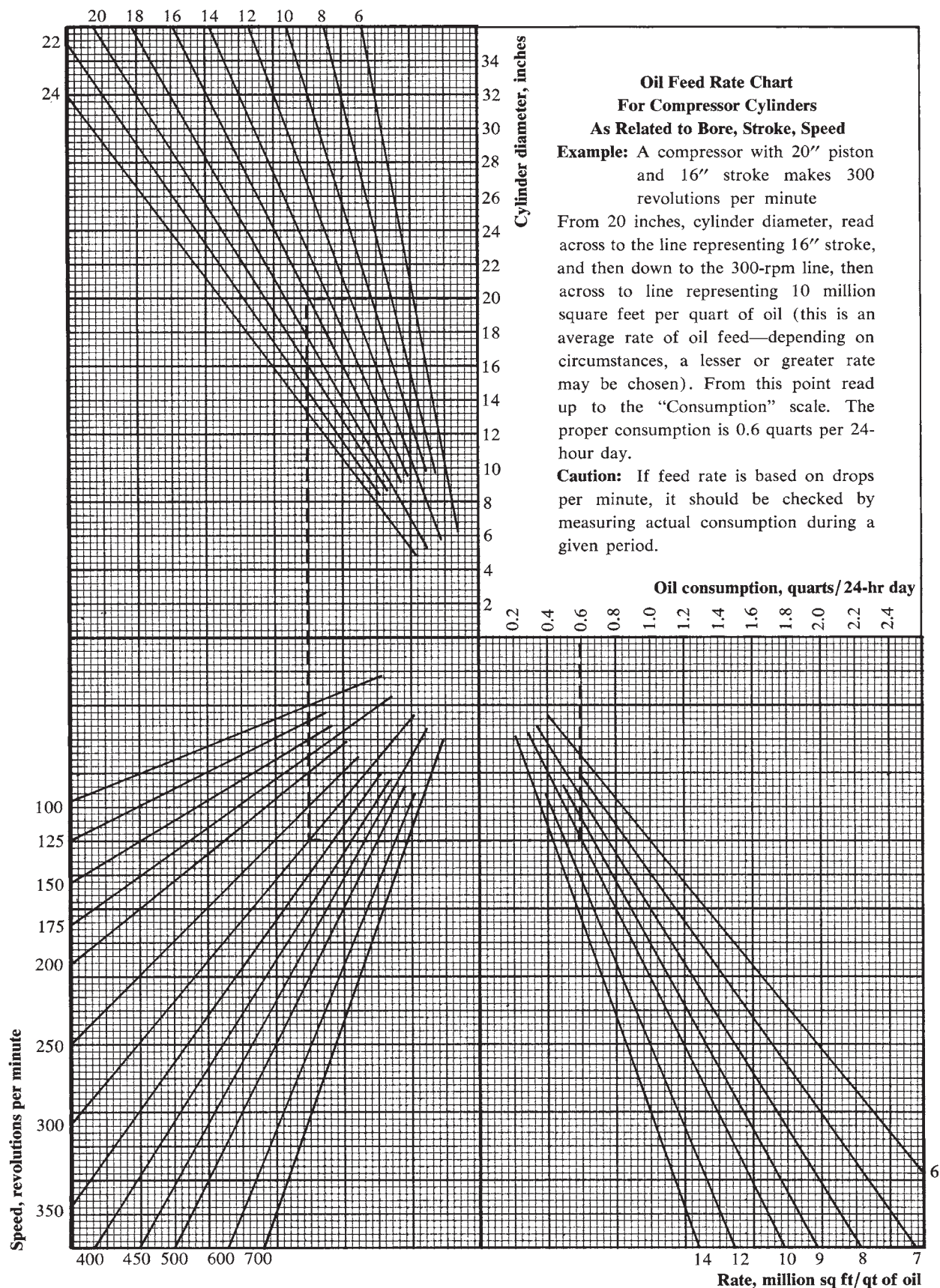
Figure 15-19. Oil feed rate to double-acting compressor cylinders.
