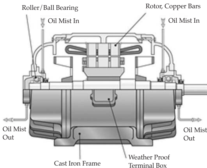
Figure 11-33. Oil mist lubrication applied to electric motor. Note that no liquid-oil sump exists in this dry-sump ("pure mist") application. (Source: AESSEAL plc, Rotherham, UK, and Knoxville, TN.)
