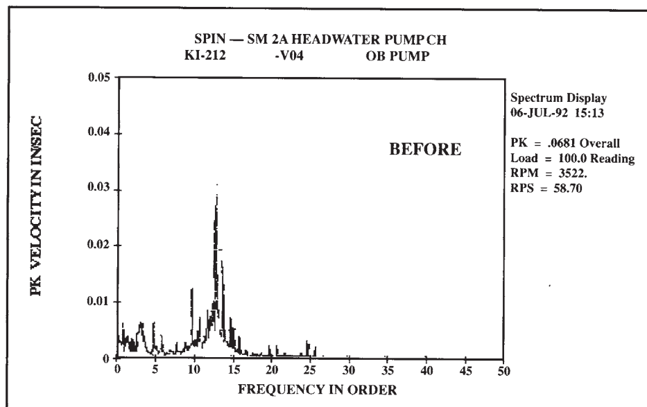
Figure 7-28(a). The overall vibration level of a 10 hp centrifugal pump was 0.068 ips; however, bearing housing temperatures of 175°F were borderline when operating on a premium grade mineral oil.
