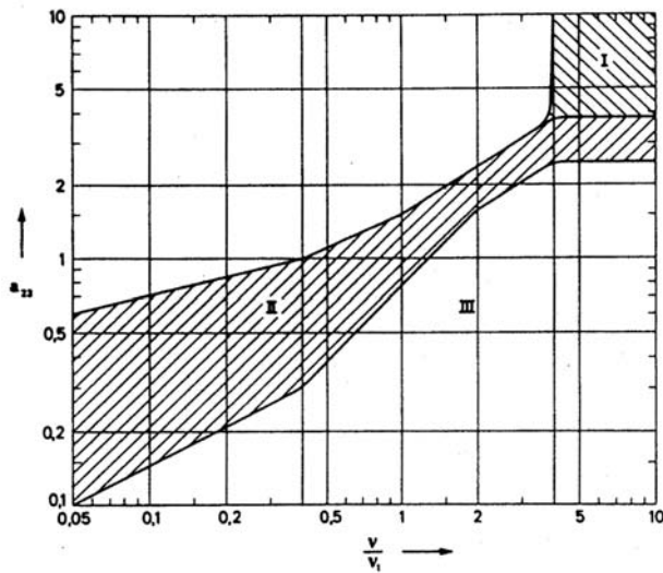
Figure 12-60. Contamination adjustment factor “a23” vs. viscosity ratio (Source: FAG Bearings, Schweinfurt, Germany, also Ref. 1)
