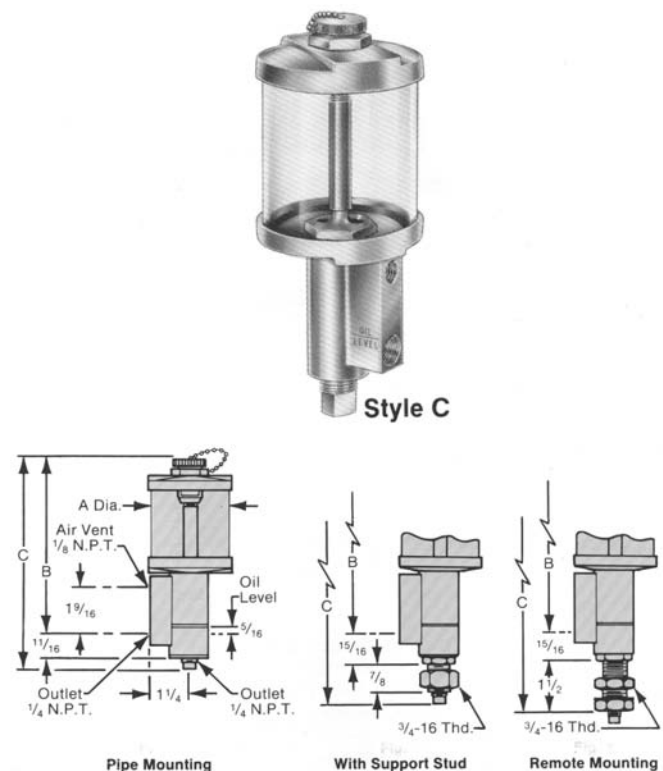
Figure 11-13. Piping "Air Vent" back into the equipment bearing housing produces a reliable pressure—balanced lubricator. (Source: Oil-Rite Corporation, Manitowoc, Wisconsin.)
