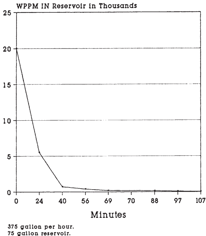
Figure 17-5. Typical residual water vs. time performance of vacuum dehydrators. (Source: Allen Filters, Inc., Springfield, Missouri)
