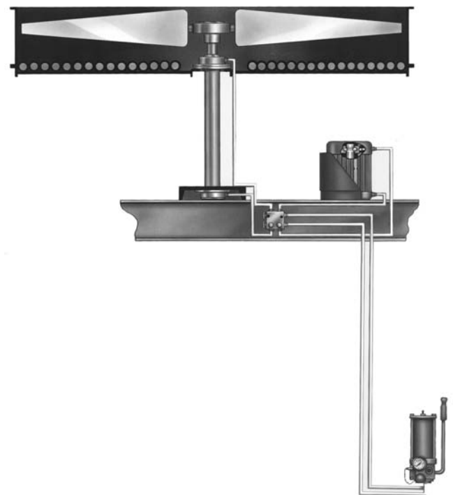
Figure 11-23. Hand-operated injector pump system serving a cooling fan assembly.
