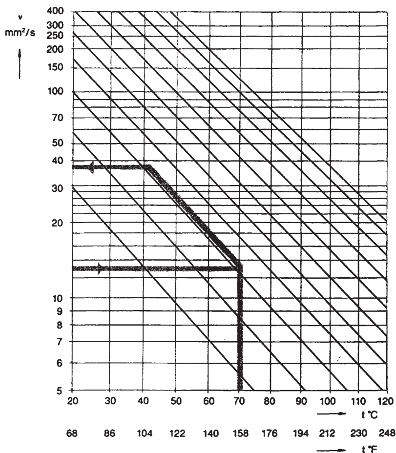
Figure 12-8. The required ISO-grade of a lubricant can be obtained from this graph.
