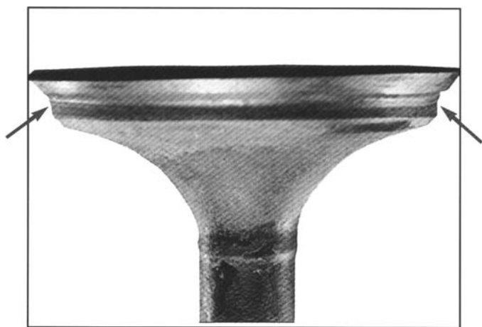
Figure 15-22. Gas engine valve with indications of wear. Recess on the valve face indicates valve beat-in.
