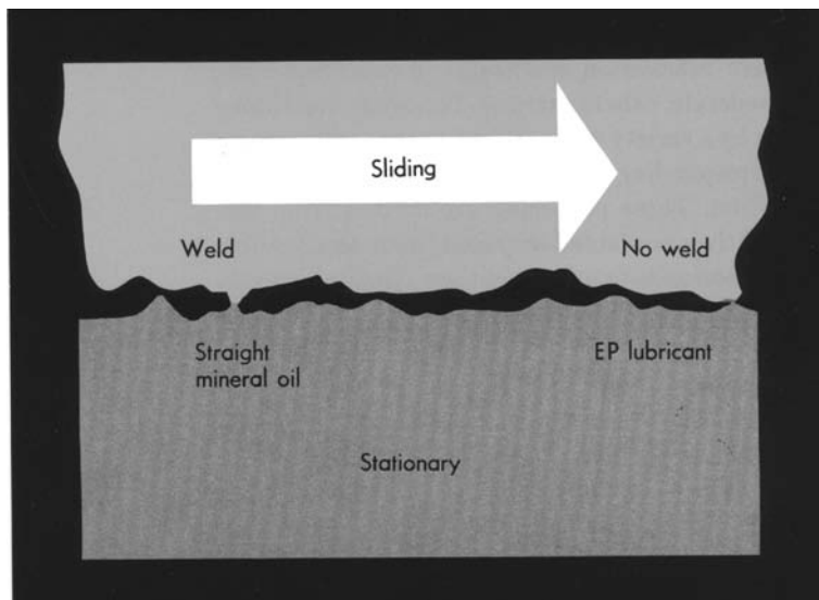
Figure 1-21. Extreme-pressure conditions.
