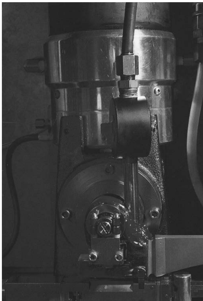
Figure 9-3. The Timken machine shown above simulates extreme pressure service conditions to measure the EP properties of lubricants.
