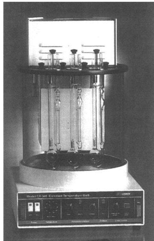
Figure 19-9. U-tube kinematic viscometer.
