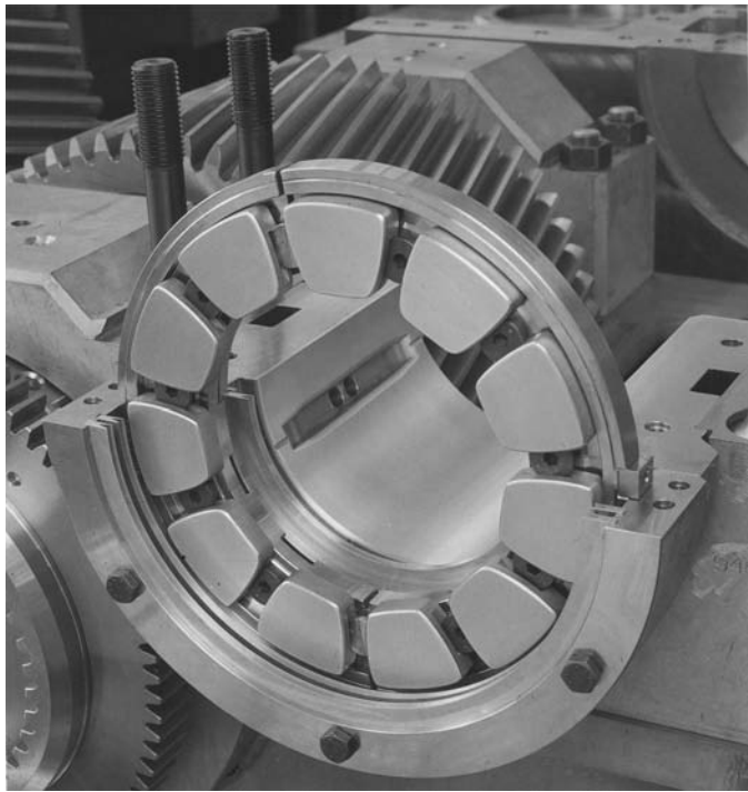
Figure 12-11. 20MW naval gearbox fitted with Glacier Series II flooded lubrication standard bearings for medium speed duties. (Photo courtesy of Maag Gear Company, Zurich, Switzerland.)
