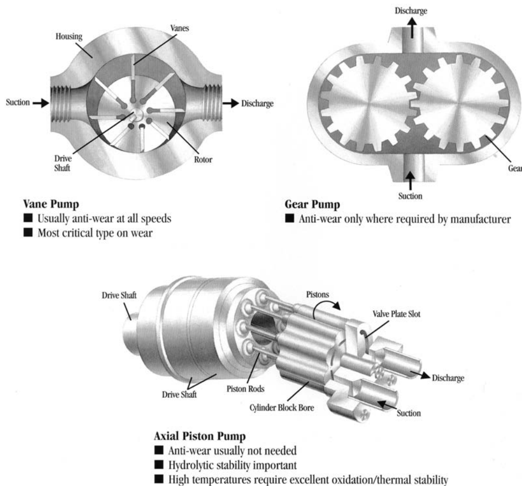
Figure 5-3. Main types of pumps found in hydraulic system. (Source: Exxon Company, U.S.A., Houston, Texas)
