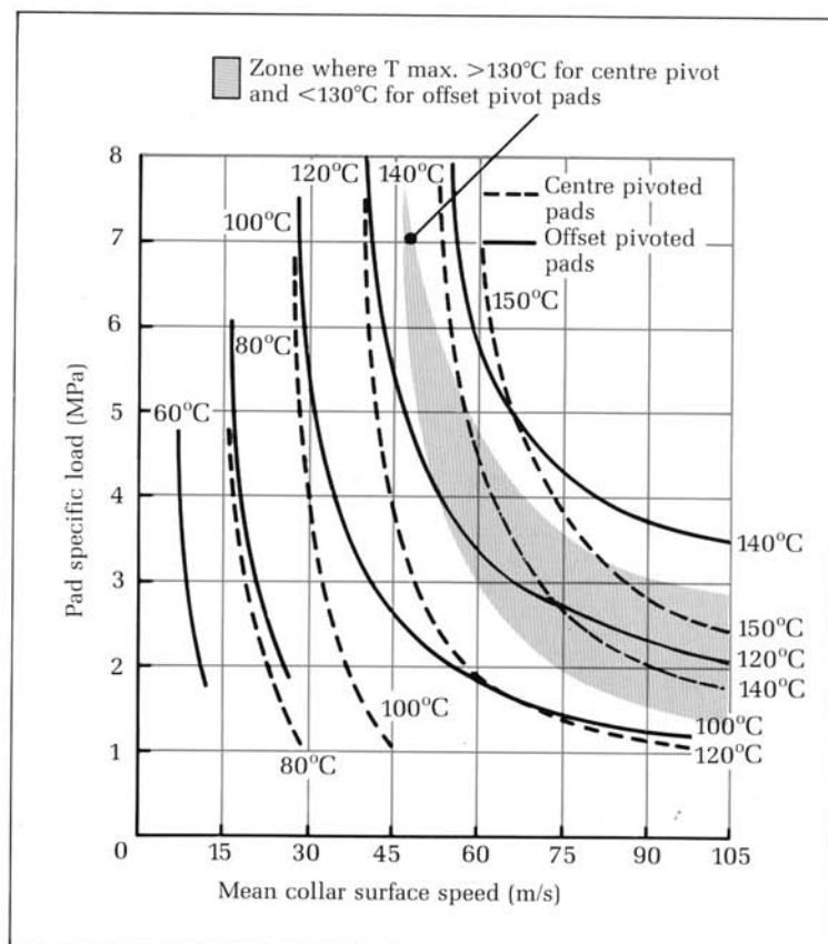
Figure 12-16. Offset pivots: effect on thrust pad temperature.
