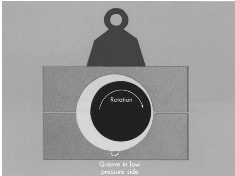
Figure 1-12. Edges of bearing face are rounded to prevent scraping of oil from journal.
