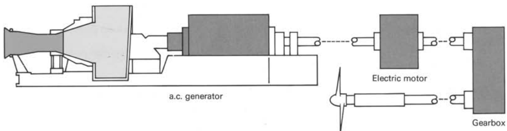
Figure 16-14. Rolls Royce aeroderivative gas turbine—generator and applications.
