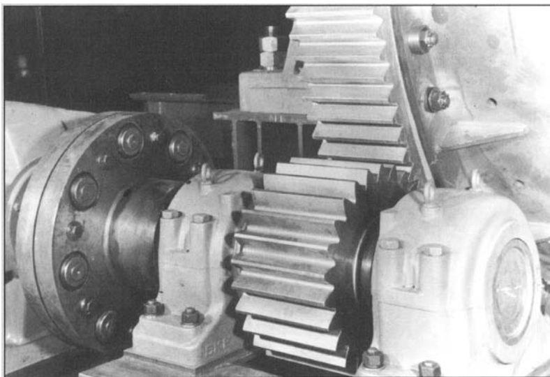
Figure 14-5. Girth gear drive of a drying cylinder.
