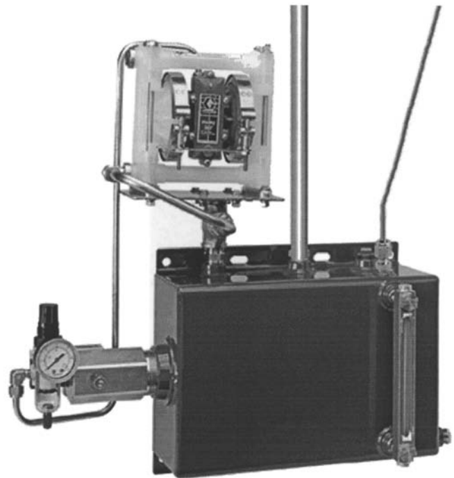
Figure 11-30. Automated drain leg assembly incorporating drain lines, collection container, and air-operated switch and pump assemblies. (Source: Lubrication Systems Company, Houston, Texas.)
