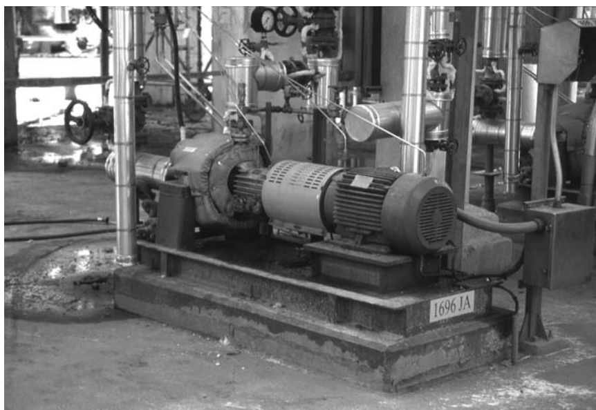
Figure 11-42: Oil mist application on a pump-and-motor set, with routing per API-610. (Source: Lubrication Systems Company, Inc., Houston, Texas.)
