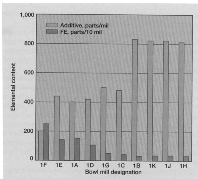
Figure 7-1. Bowl mill wear, 1,000 operating hours.
