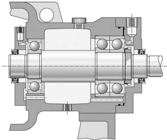
Figure 11-25. Dry sump oil mist applied between the bearing housing seal and bearing (per API-610). The mist is vented from the bottom (drain location) of the bearing housing
