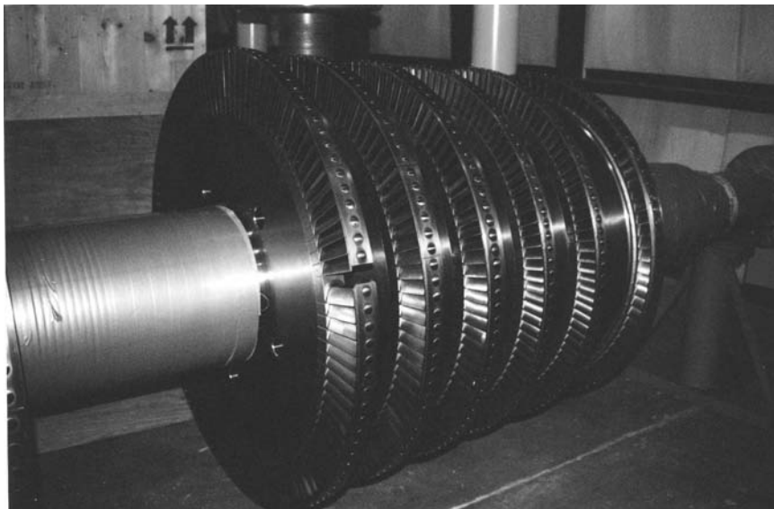
Figure 18-10. Turbomachinery rotor protected by RUST-BAN 326. (Source: Sulzer-Hickham Industries, Inc., LaPorte, Texas)
