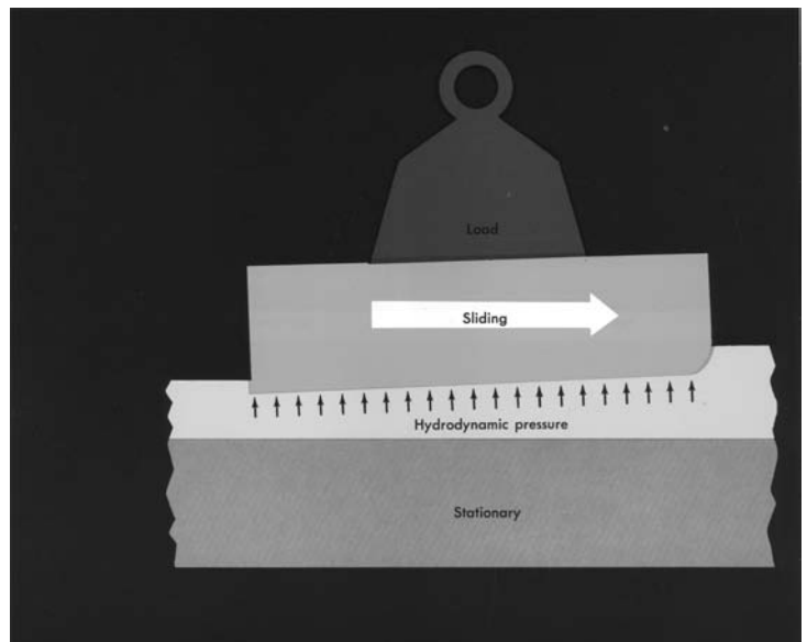
Figure 1-8. Sliding load supported by a wedge-shaped lubricating film.
