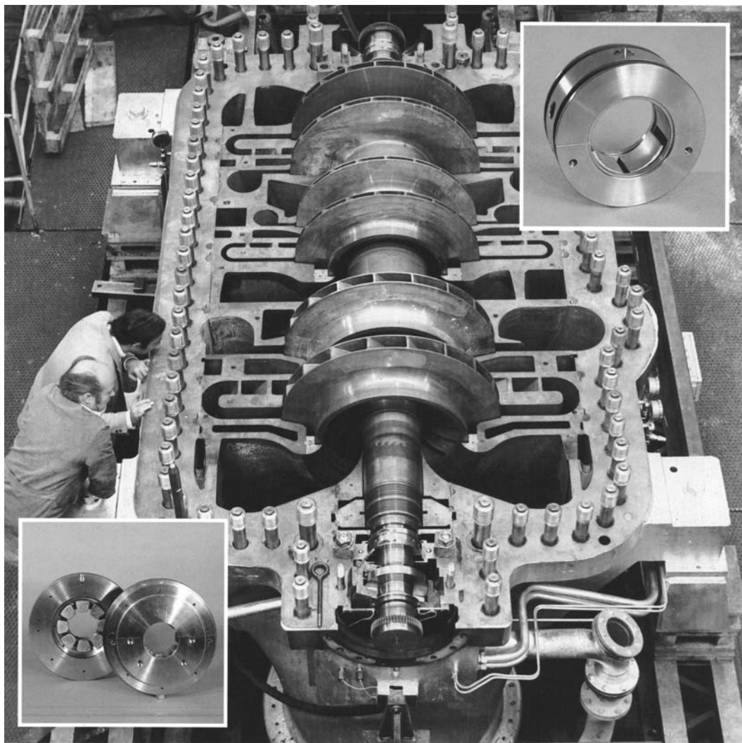
Figure 15-2. Centrifugal compressor with thrust bearing (inset, lower left) and radial bearing (inset, upper right). Source: GHH-Borsig, Berlin, Germany.
