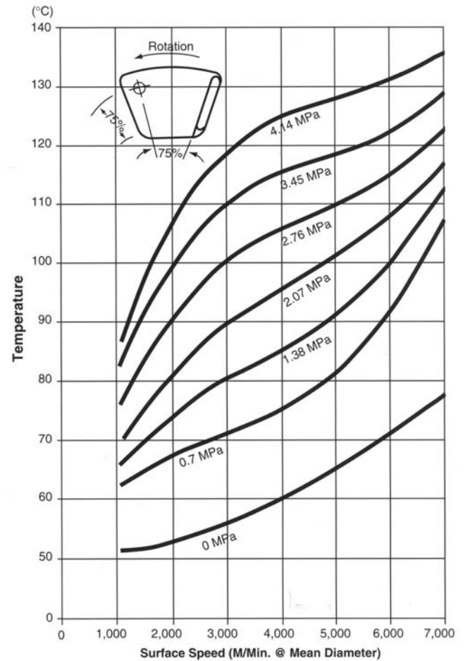
Figure 12-26. "LEG" white metal temperatures at 75/75 position (6 and 8-pad series, steel pads).
