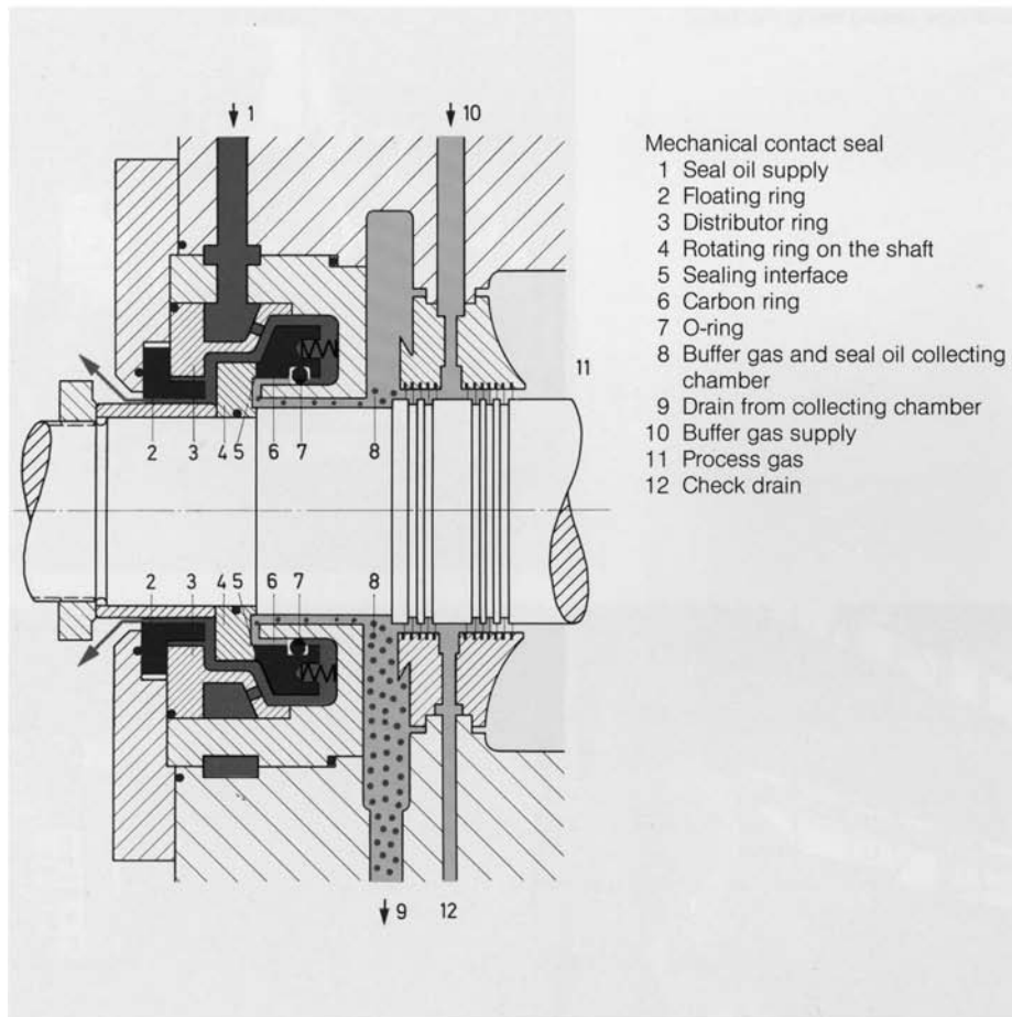
Figure 15-5. Mechanical contact seal showing seal oil inlet at point 1. (Source: Mannesmann-Demag, Duisburg, Germany)
