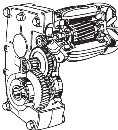
Figure 14-9. Gear motor, double-stage spur gear.
