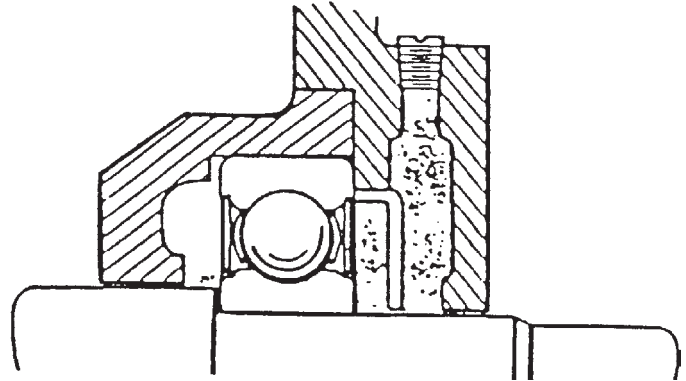
Figure 13-3. Double-shielded bearing with grease metering plate facing grease reservoir.
