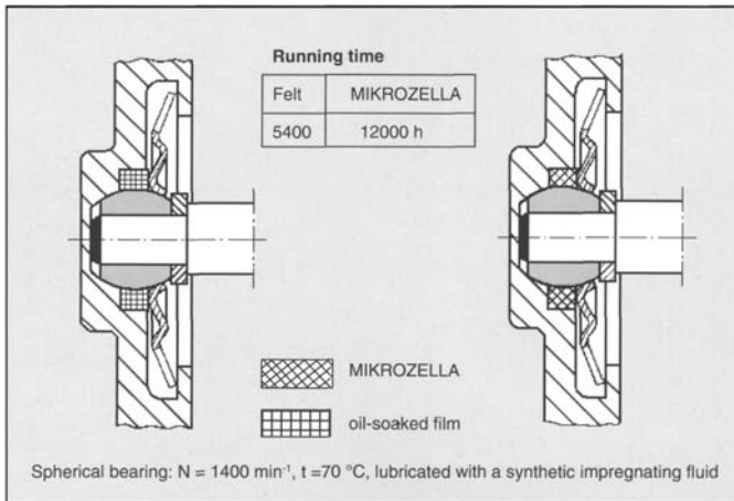
Figure 12-43. Plastic oil depot lubrication of a spherical bearing.
