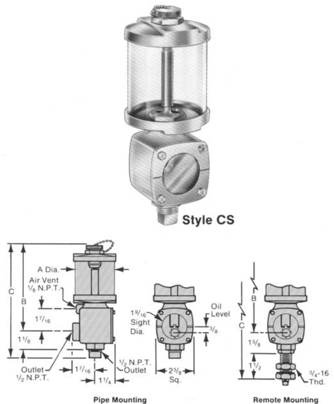
Figure 11-15. Pressure-balanced constant level oiler with integral sight glass. (Source: Oil-Rite Corporation, Manitowoc, Wisconsin.)
