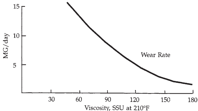
Figure 14-18. Viscosity vs. wear plot.
