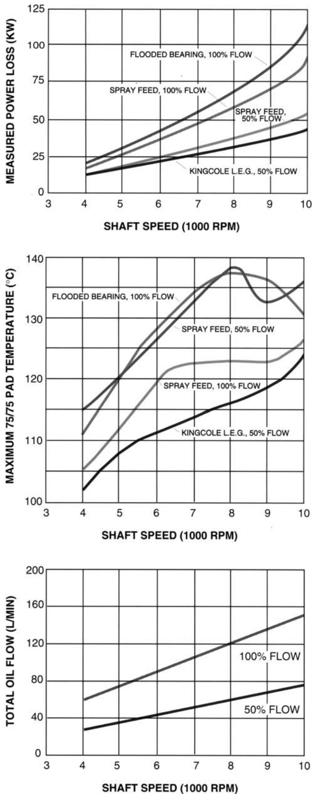
Figure 12-25. "LEG" bearings vs. standard flooded bearings and spray-fed bearings.
