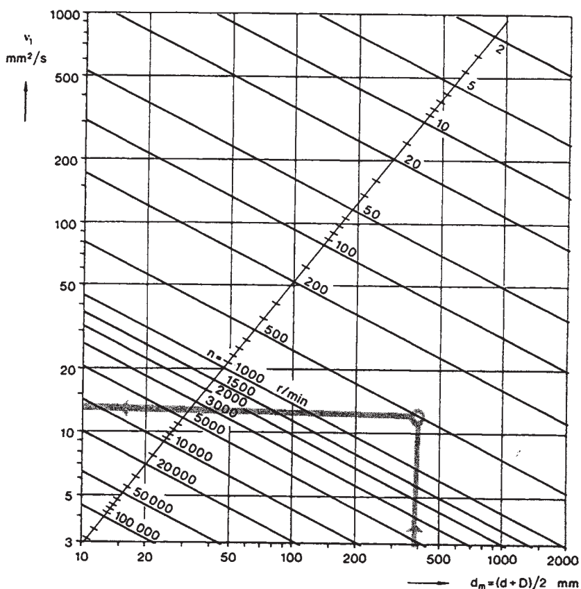
Figure 12-7. Kinematic viscosity requirement as a function of bearing mean diameter and speed.
