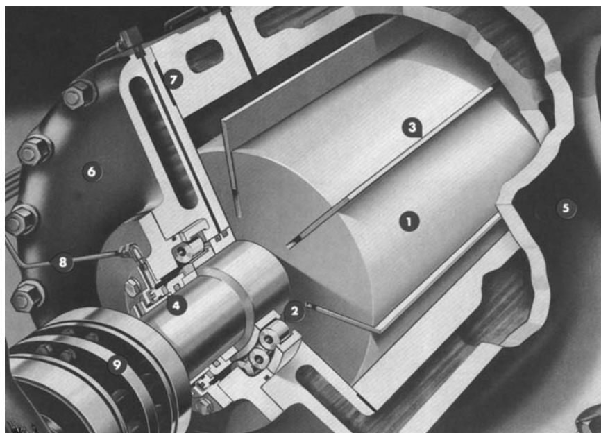
Figure 15-9. Sliding vane compressor and principal components: rotor and shaft (1), bearings (2), blades (3), mechanical seals (4), cylinder/housing (5), heads/covers (6) gaskets (7), lube supply line (8), coupling (9). (Source: A-C Compressor Corporation, Appleton, Wisconsin, USA)
