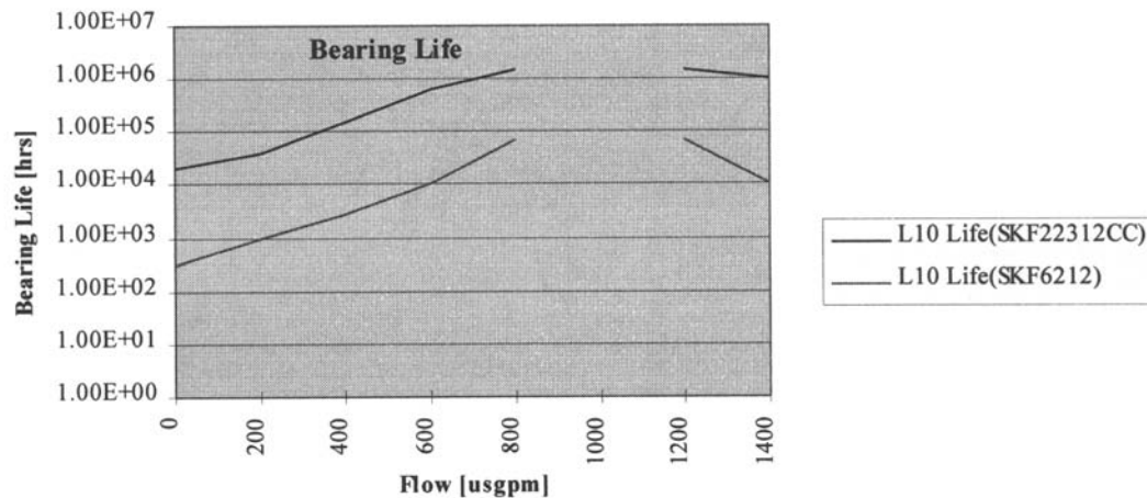
Figure 17-11. Comparison of bearing lives.
