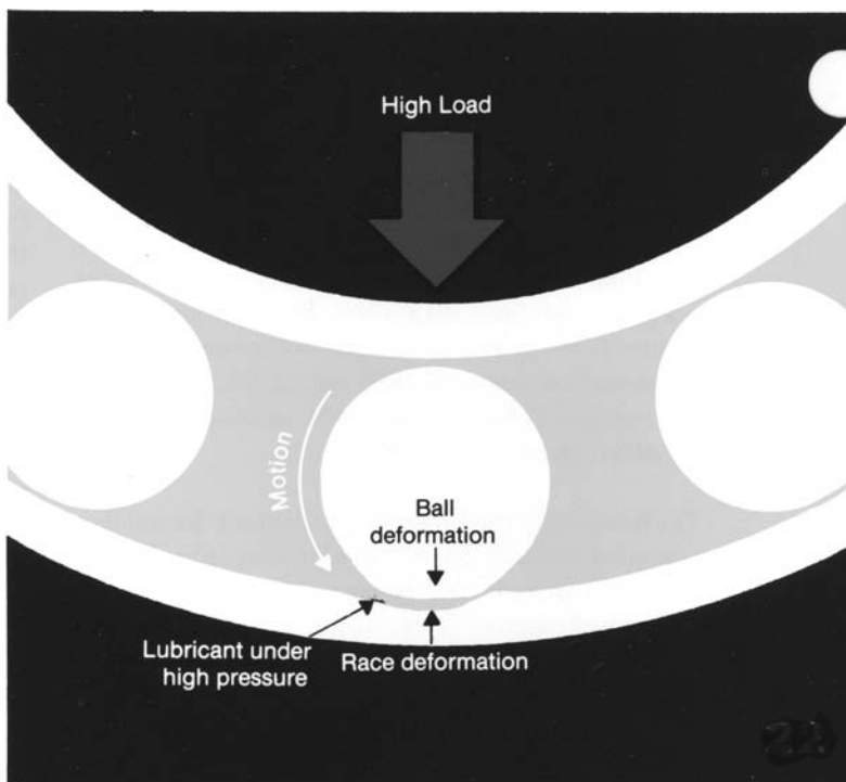
Figure 1-22. EHD lubrication in a rolling-contact bearing.
