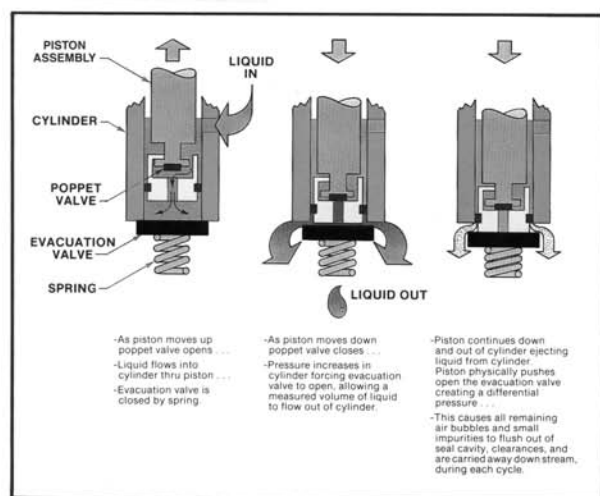
Figure 11-21. Cut-away view of "Oil Rite" air-operated injector pump.
