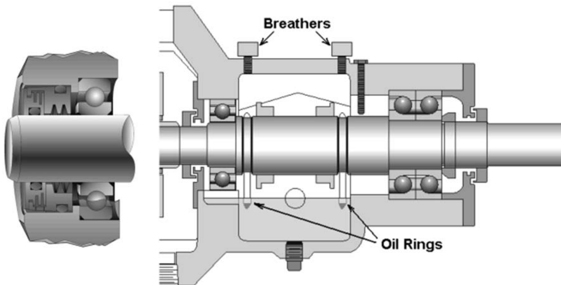
Figure 11-16. Bearing housings with (shown on left) a static oil sump reaching to center of bottom rolling element. Alternatively, a lowered oil level (shown on right) will require one or two oil rings dipping in the oil so as to “lift” oil into the bearings.
