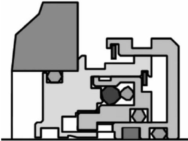
Figure 12-66. This variant of Figure 12-65 incorporates considerable axial float capability and is used on small steam turbines (Source: AESSEAL plc, Rotherham, UK and Knoxville, Tennessee)
