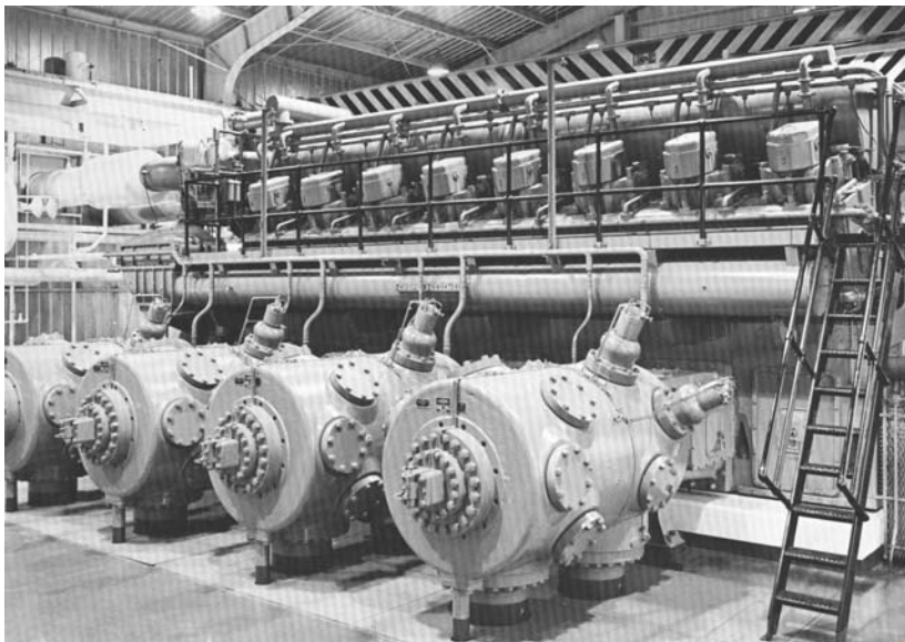
Figure 15-20. This Cooper-Bessemer model V-250 with 16 power cylinders is rated at 5500 hp. Unit is equipped with eight GT pipeline cylinders and is on transmission duty in New York State.
