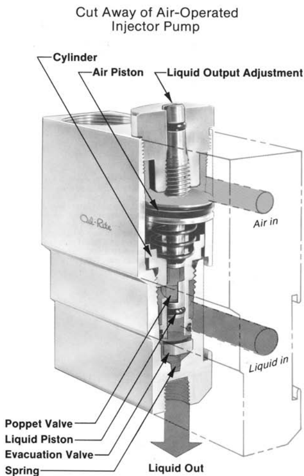
Figure 11-21. Cut-away view of "Oil Rite" air-operated injector pump.
