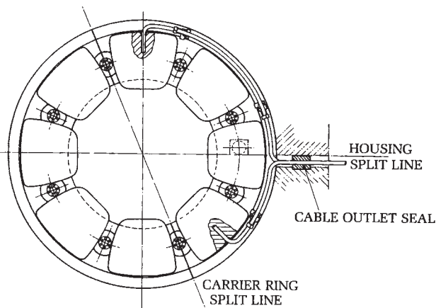
Figure 12-18. Temperature sensors: typical method of fitting to thrust rings.
