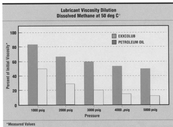
Figure 15-18. Lubricant viscosity dilution—EXXCOLUB vs. petroleum oil.
