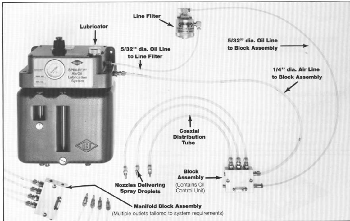
Figure 11-9. Small air-oil lubrication system. (Source: Bijour Lubricating Corporation, Bennington, Vermont.)
