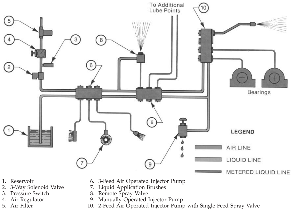
Figure 11-20. Air-operated injector pump system. (Source: Oil-Rite Corporation, Manitowoc, Wisconsin.)
