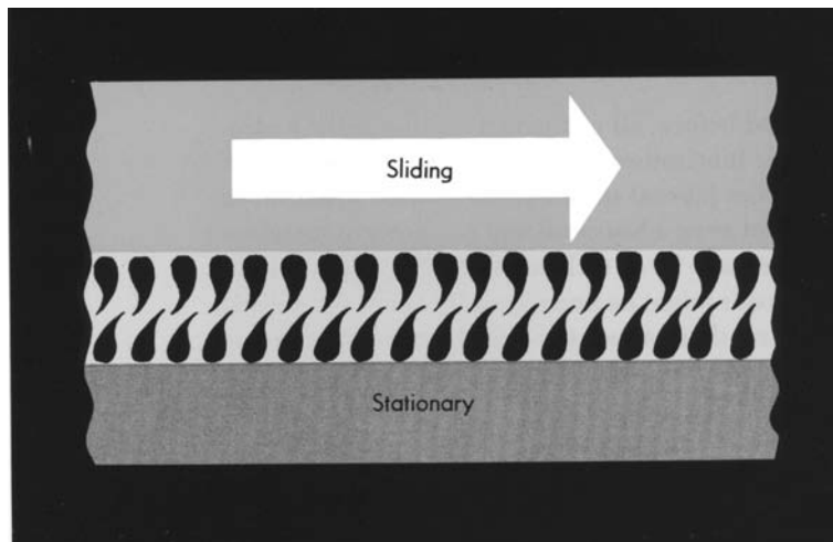
Figure 1-20. Sliding surfaces separated by a boundary lubricant of the polar type.
