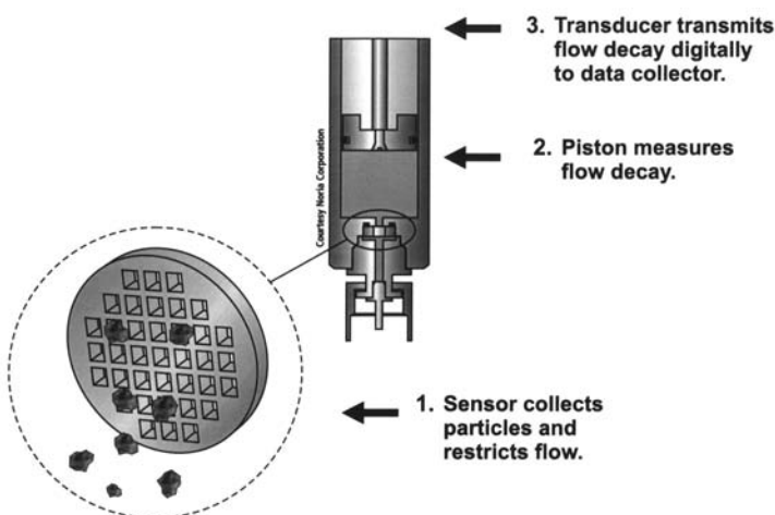
Figure 19-14. Pore blockage-type particle counter.
