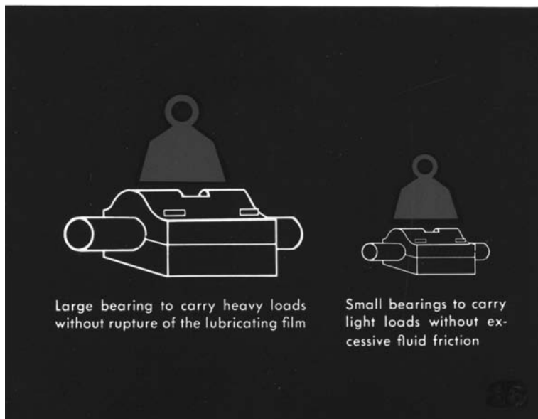
Figure 1-16. Bearing design should permit the development of a full-fluid film.
