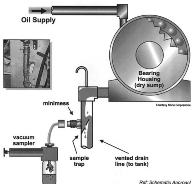
Figure 19-5. Sample trap installed in drain line below bearing housing.
