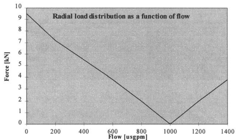
Figure 17-10. Radial load.
