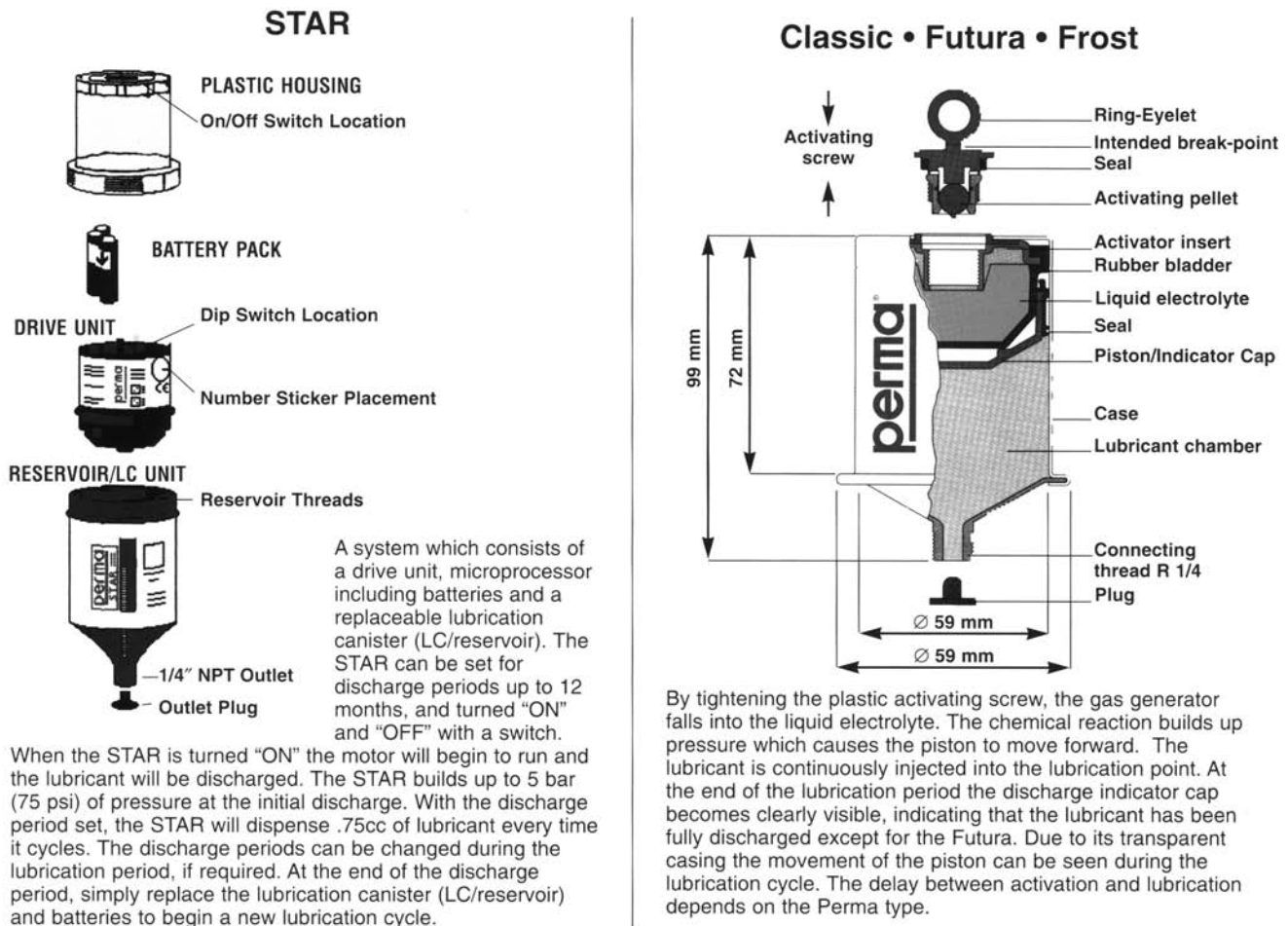
Figure 13-8. Two models of automatic single-point grease lubricators (ASPGLs) manufactured by Perma USA ( www.permausa.com ).
