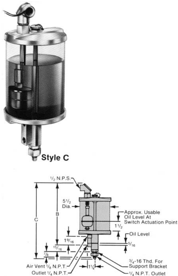
Figure 11-14. Pressure-balanced lubricator with low level safety (warning or shut-down) switch. (Source: Oil-Rite Corporation, Manitowoc, Wisconsin.)
