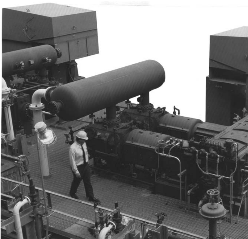
Figure 15-7. Reciprocating compressor installation. (Source: Dresser-Rand Company, Painted Post, New York)
