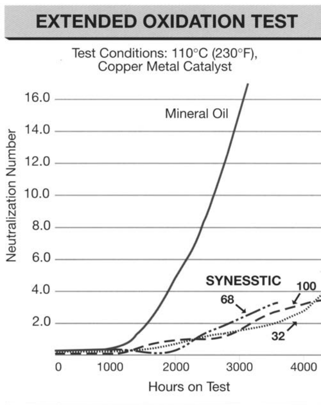
Figure 7-15. Oxidation tests show diester-base synthetics excel over mineral oils.
