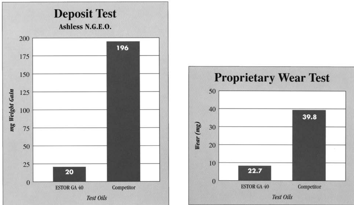
Figure 15-30. Deposit and wear test comparisons, ESTOR GA 40 vs. competitor.
