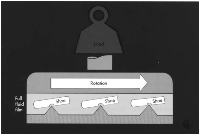
Figure 1-9. Shoe-type thrust bearing.
