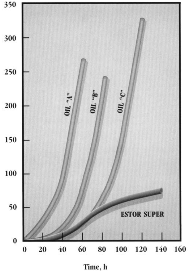
Figure 15-26. Nitration and oxidation inhibition viscosity increase laboratory engine test. The graph illustrates the excellent viscosity control demonstrated by ESTOR Super compared with three competitive commercial gas engine oils in the severe Nitration/Oxidation Engine Test.
