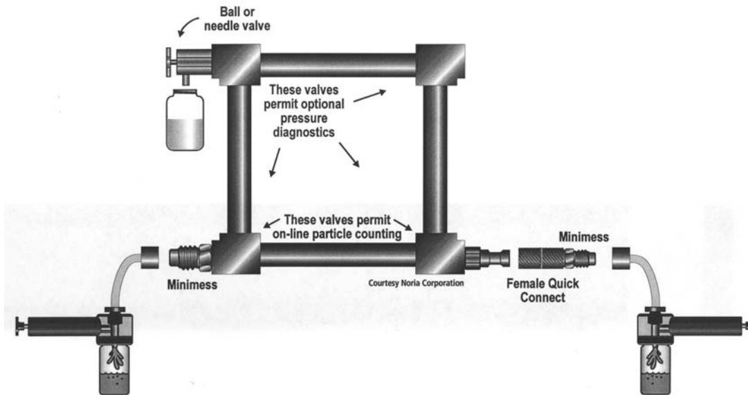
Figure 19-3. Different options for sampling oil from low pressure return lines.
