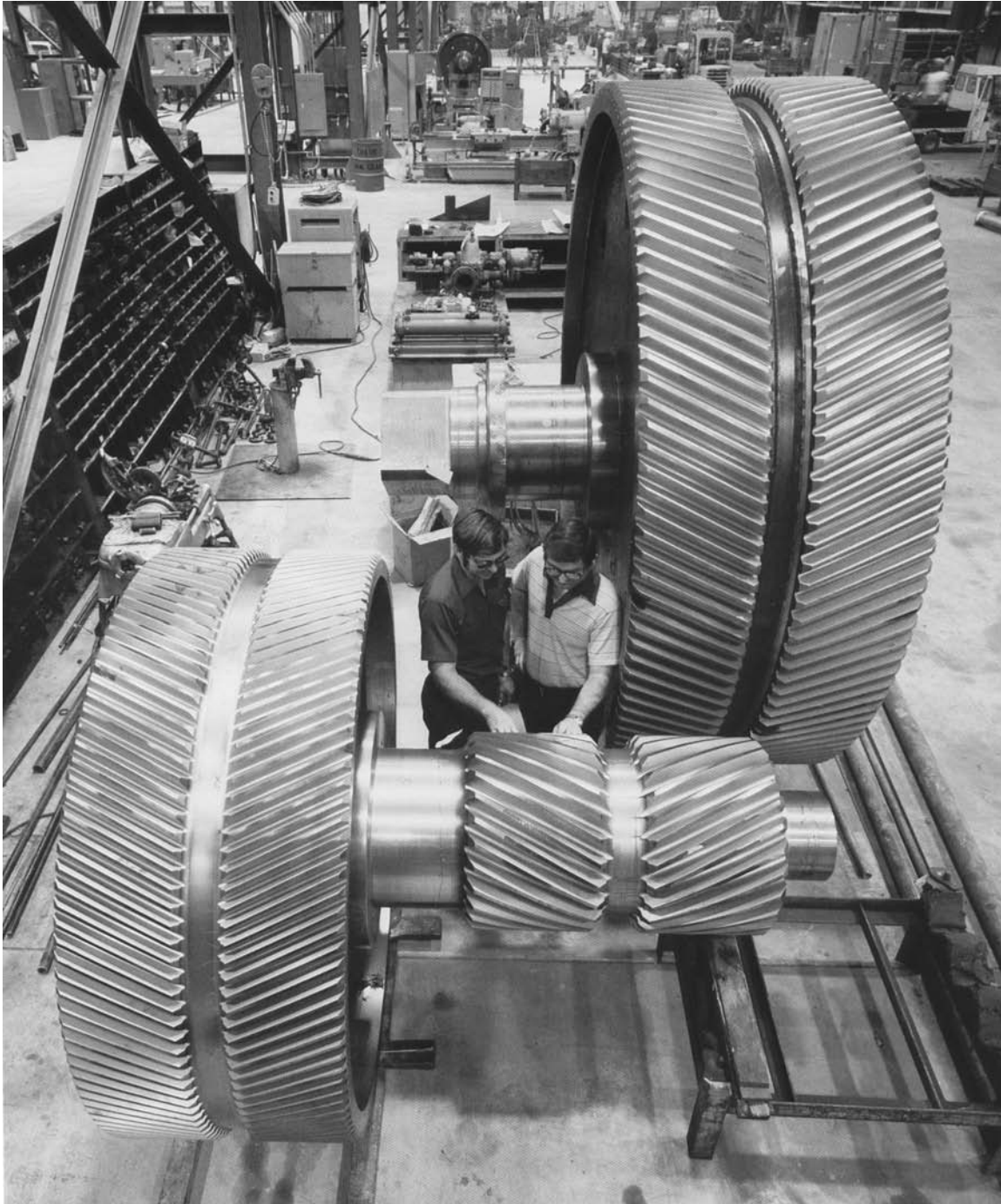
Figure 14-2. Double-helical, low-speed gear unit being checked at Lufkin Gear Company, Lufkin, Texas.
