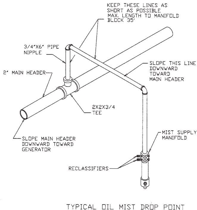
Figure 11-29. Oil mist distribution piping. (Source: Lubrication Systems Company, Houston, Texas.)
