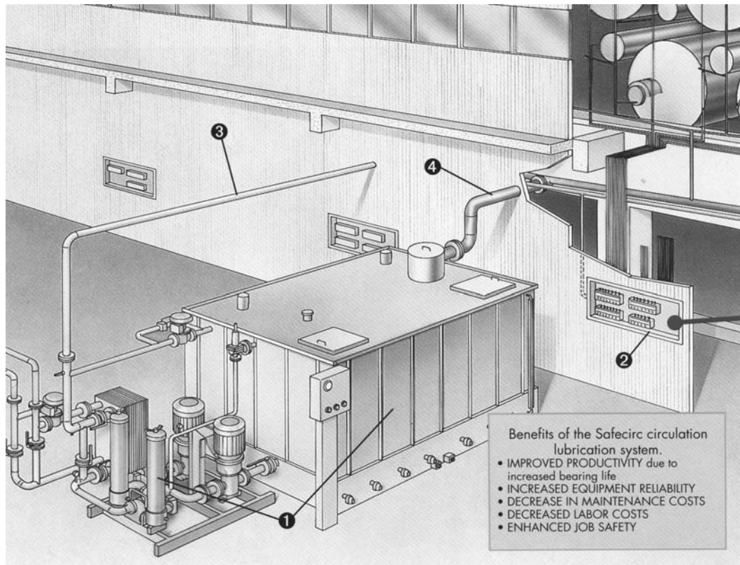
Figure 11-5. Circulating lubrication system comprised of filters/cooler/pumps and reservoir (1), oil flow metering modules (2), pressure piping (3), and return piping (4). (Source: Safematic, Inc., Alpharetta, Georgia, and Muurame, Finland.)
