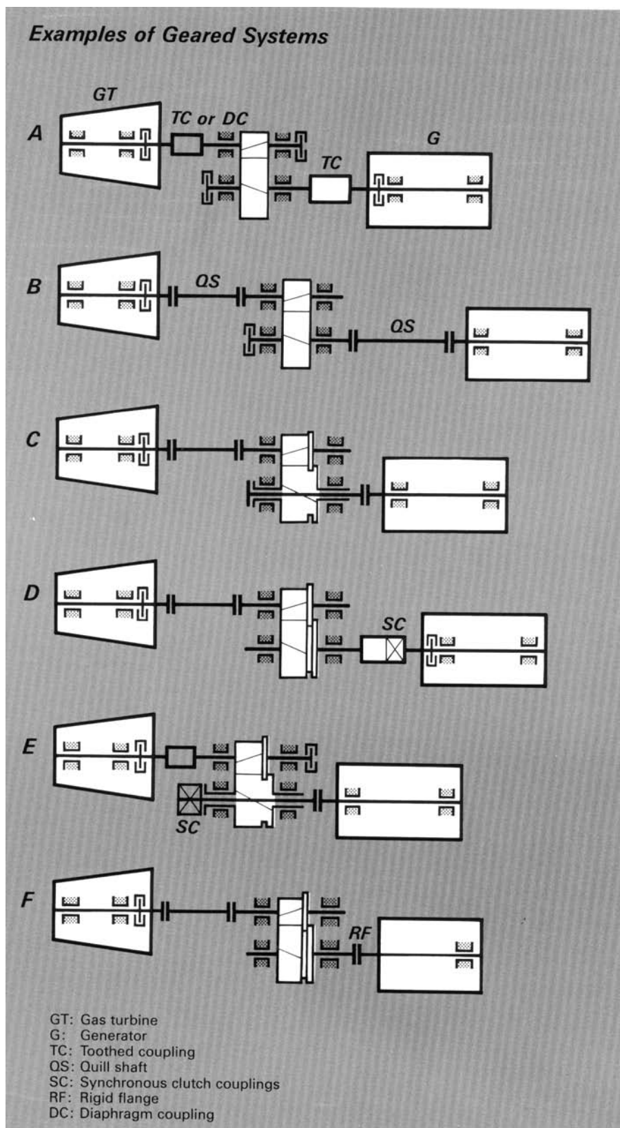
Figure 14-4. Examples of geared systems. (Source: Maag Gear Company, Zurich, Switzerland)
