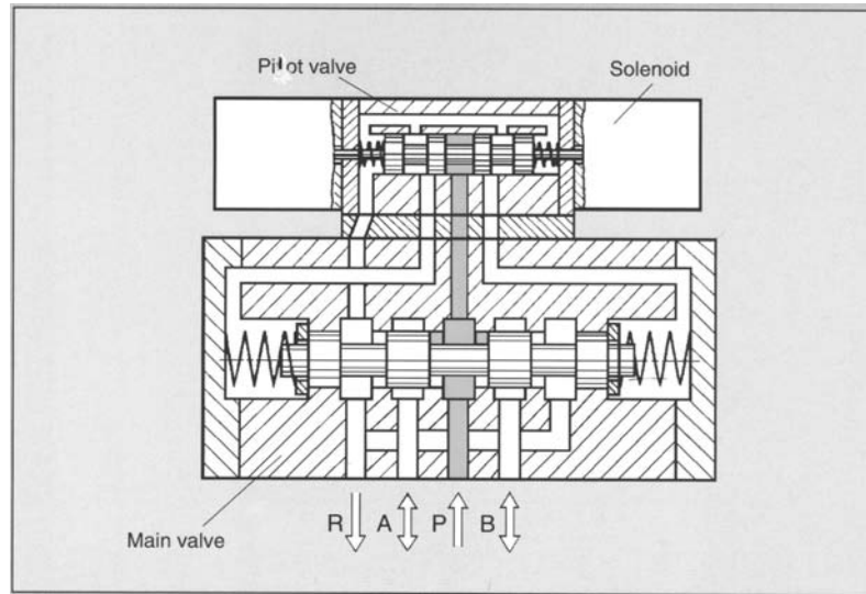
Figure 5-2. Electromagnetically operated 4/3-way valve with pilot valve. (Source: Klüber Lubrication North America, Inc., Londonderry, New Hampshire)
