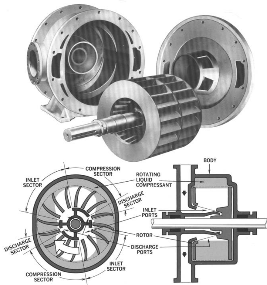
Figure 15-10. Liquid ring compressor with elongated casing (A), and schematic section at inlet and discharge sectors (B). (Source: Nash Engineering, Norwalk, Connecticut, USA)
