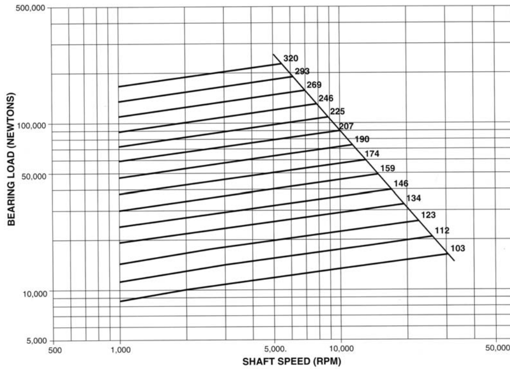
Figure 12-27. Rated load for 8-pad "LEG" bearings
