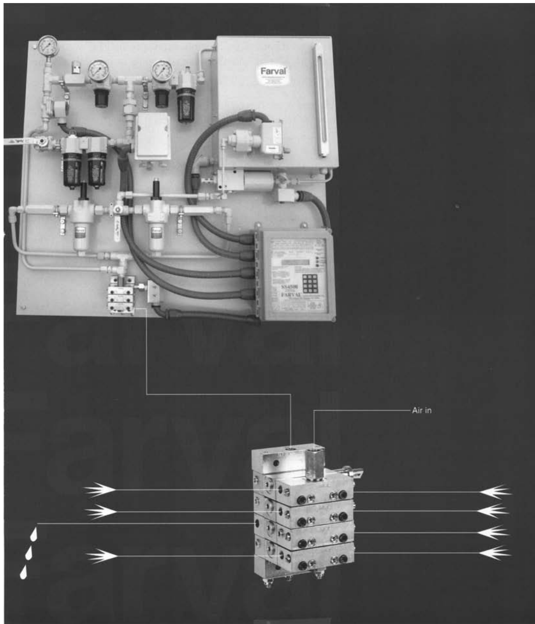
Figure 11-8. Typical air-oil lubrication system. (Source: Farval Lubrication Systems, Inc., Kinston, North Carolina.)
