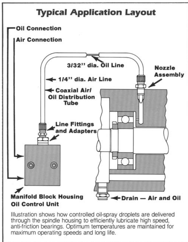
Figure 11-12. Typical application layout for air-oil lubrication. (Source: Bijour Lubricating Corporation, Bennington, Vermont.)
