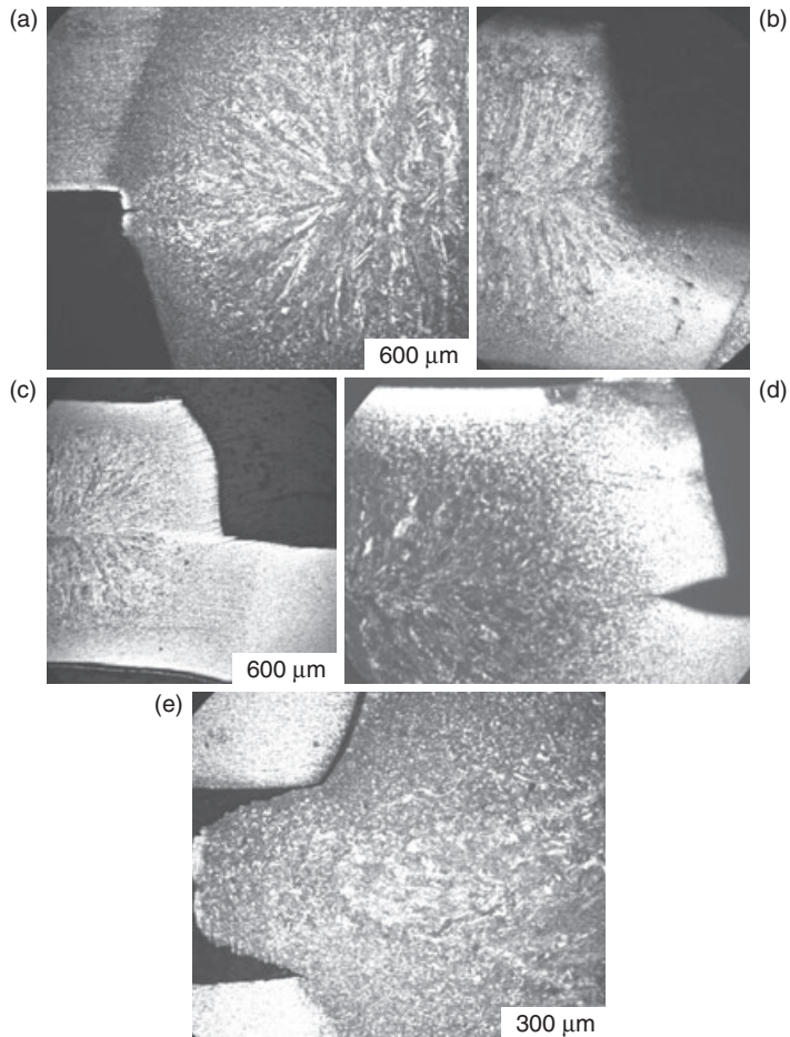
4.11 Fatigue cracking behavior with respect to the microstructure of spot welds in various steels: (a) DP600, (b) Boron, (c) HSLA, (d) CQSK, (e) TRIP.
