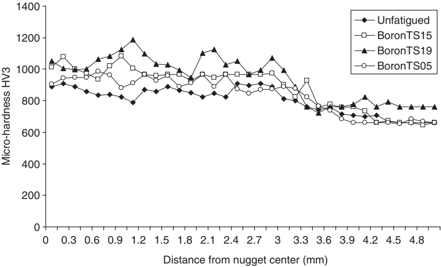
4.8 Micro-hardness variation in the half-thickness plane of the nugget, where sample 15 has 616 000 cycles to failure, sample 19 has 137 5000 cycles to failure and sample 05 has 36 900 cycles to failure.
