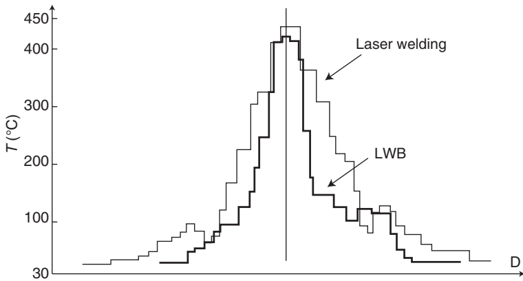
8.17 Results of the line scan of temperature on the surface of Mg alloy.
