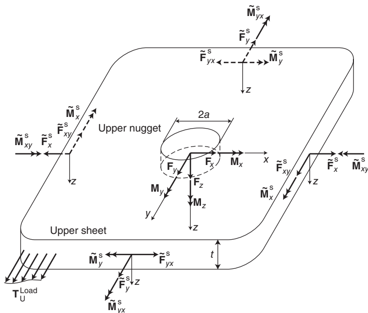
1.2 Upper sheet with the upper half nugget is shown with the surface traction \mathbf{T}_U^{\text{Load}} , the resultant loads \mathbf{F} and \mathbf{M} and the self-balanced resultant loads \mathbf{F}^s and \mathbf{M}^s . The upper sheet has the thickness t and the nugget has the diameter 2a .
