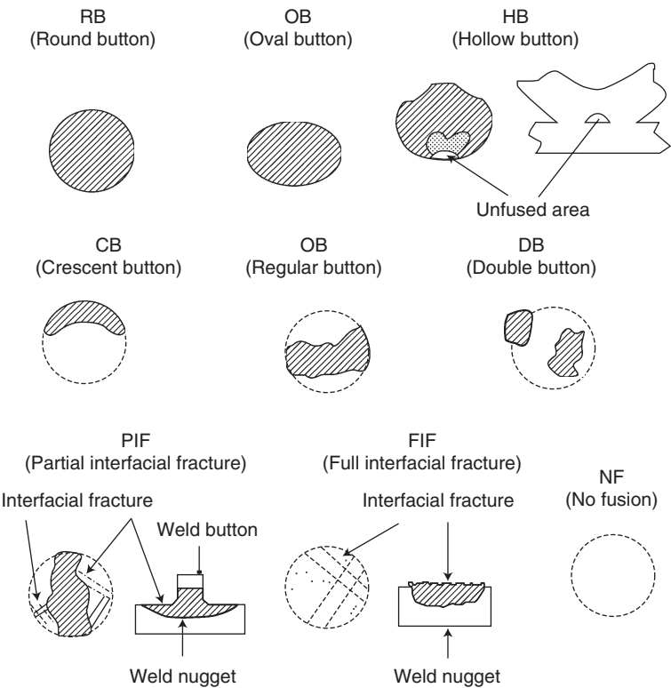
4.4 Fracture or pull-out mode in spot-welded sheets.
