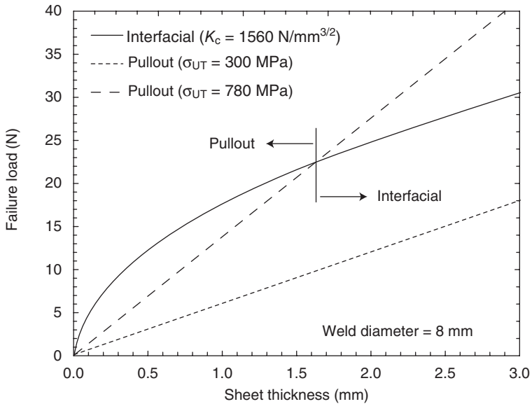
3.10 Plot showing the predicted competition between failure by full button pullout and interfacial fracture modes in the shear-tension test. K_c is the fracture toughness and \sigma_{UT} is the ultimate tensile strength of the steel (Radakovic and Tumuluru, 2008).
