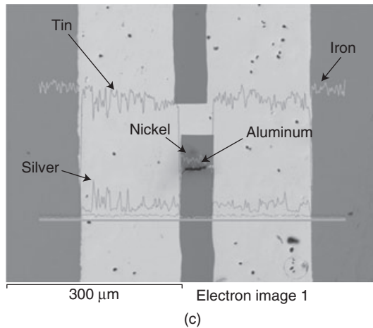
11.3 Typical bond strength test results for the solder joint of 1.4-mm SAE 1008/1.4-mm SAE 1008: (a) load versus displacement curve; (b) failure mode; (c) SEM cross-section of the joint area.
