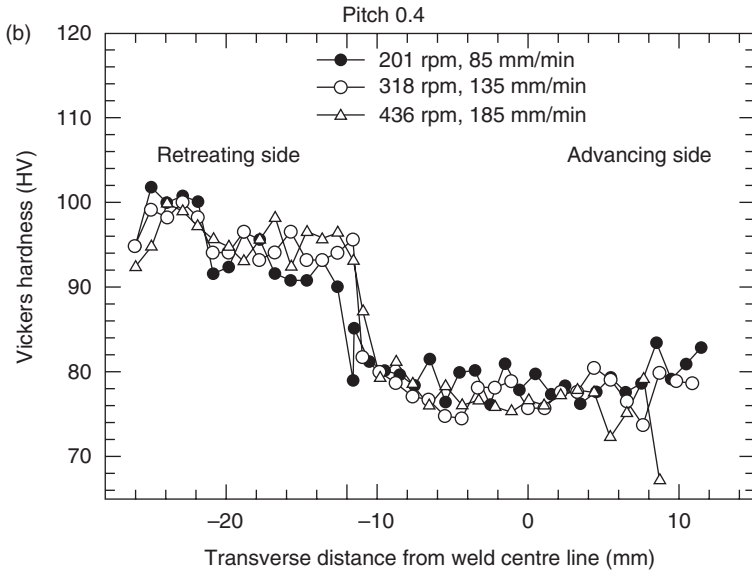
7.11 (a) Vickers microhardness ( HV_{25} ) measurements in the onion skin structure vary between approximately 77 and 92. (b) HV_{200} values range from around 98 in the parent plate to 77 in the weld metal.
