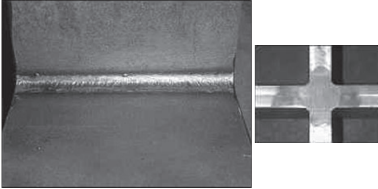
9.13 Cruciform specimen.
