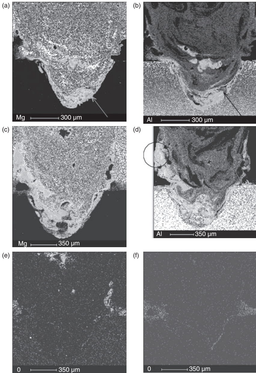
8.22 Transverse section EPMA analyses of the joint of laser welding and LWB. (a) Face scan of element Mg in laser welding joint, (b) face scan of element Al in laser welding joint, (c) face scan of element Mg in LWB joint, (d) face scan of element Al in LWB joint, (e) face scan of element C in LWB joint, (f) face scan of element O in LWB joint.
