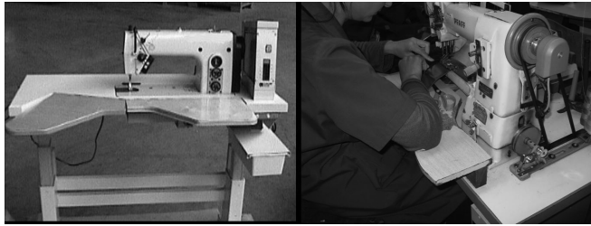
Figure 5.26 New ergonomically designed sewing tables and position of elbows at work
