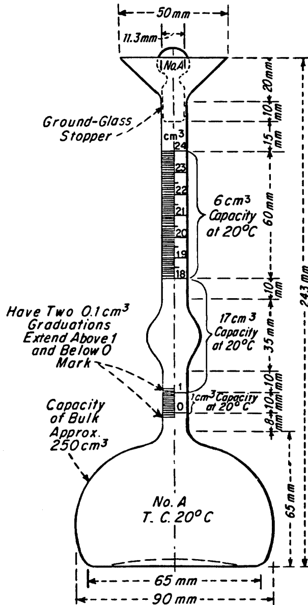
Figure 6 Le Chatelier flask for density determination of mineral filler. (From ASTM. With permission.)
