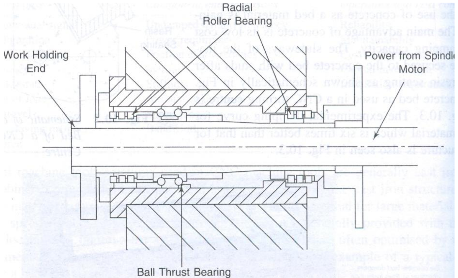
Fig. 10.4 Spindle Design for a CNC Turning Centre
