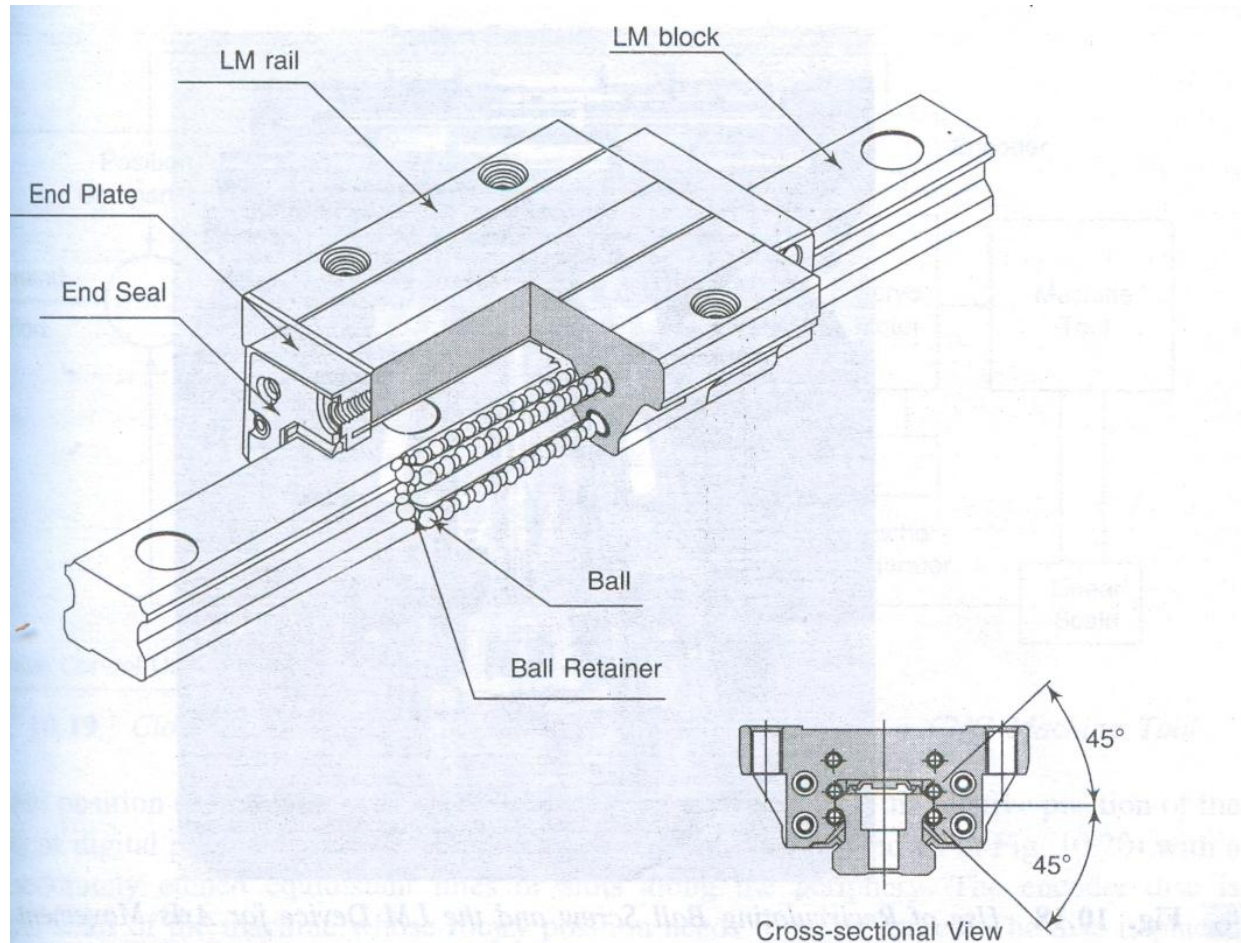
10.16 Antifriction Guideways used in CNC Machine Tools (Courtesy: THK Co. Ltd., Japan)
