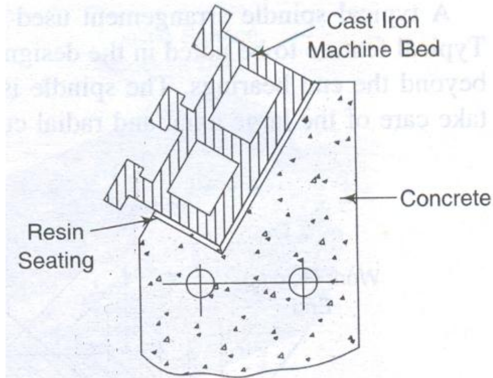
Fig. 10.2 Schematic of a Concrete Bed of a CNC Turning Centre
