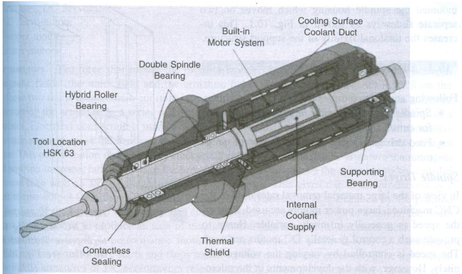
Fig. 10.5 Spindle Design with an Integral Spindle Motor and Cooling System for a CNC Machining Centre (Courtesy: Hüller Hille GMBH, Germany)
