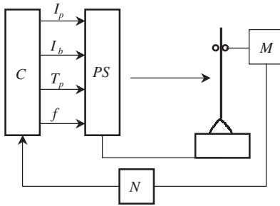
5.2 Synergic control
