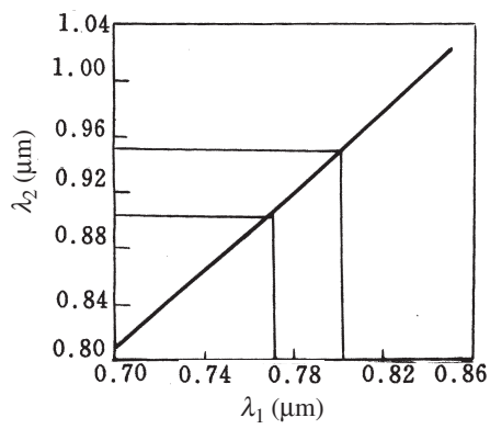
13.9 Curve for the selection of \lambda_1 \lambda_2
