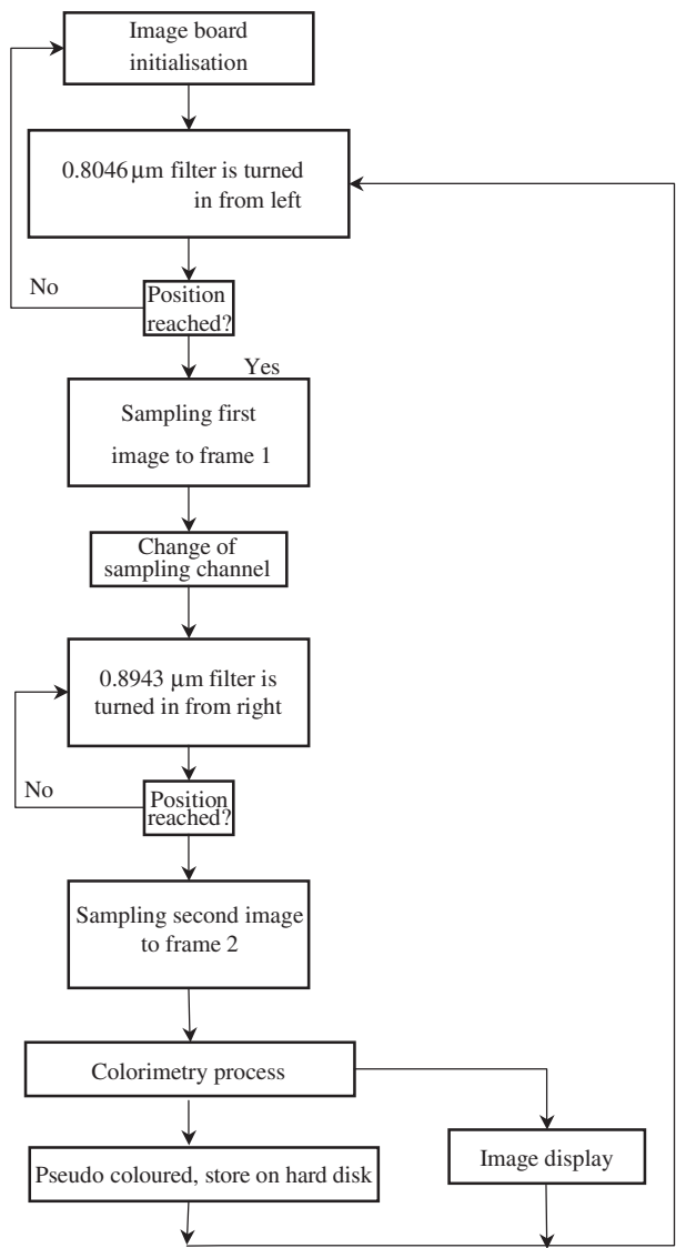
12.12 Flow chart of temperature-field measurement
