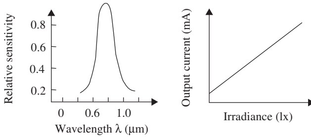
5.35 Characteristics of the 3DU photo-sensitive transistors
