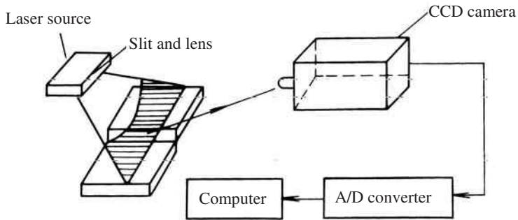
7.5 Principle of a linear laser sensor
