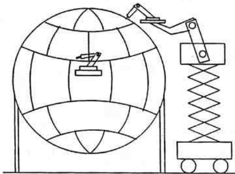
15.1 Anticipated welding method for large spherical tanks
