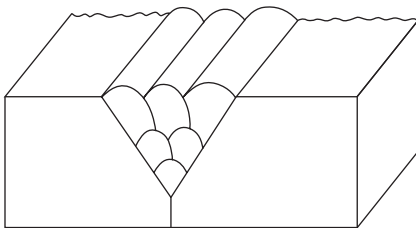
15.40 Multi-pass weld
