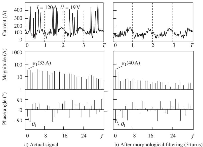
9.34 Current waveform and frequency spectrum for CO 2 welding ( f = 12 \text{ Hz} )
