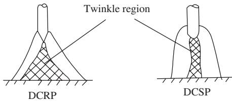
6.24 Twinkle region of DCRP and DCSP welding
