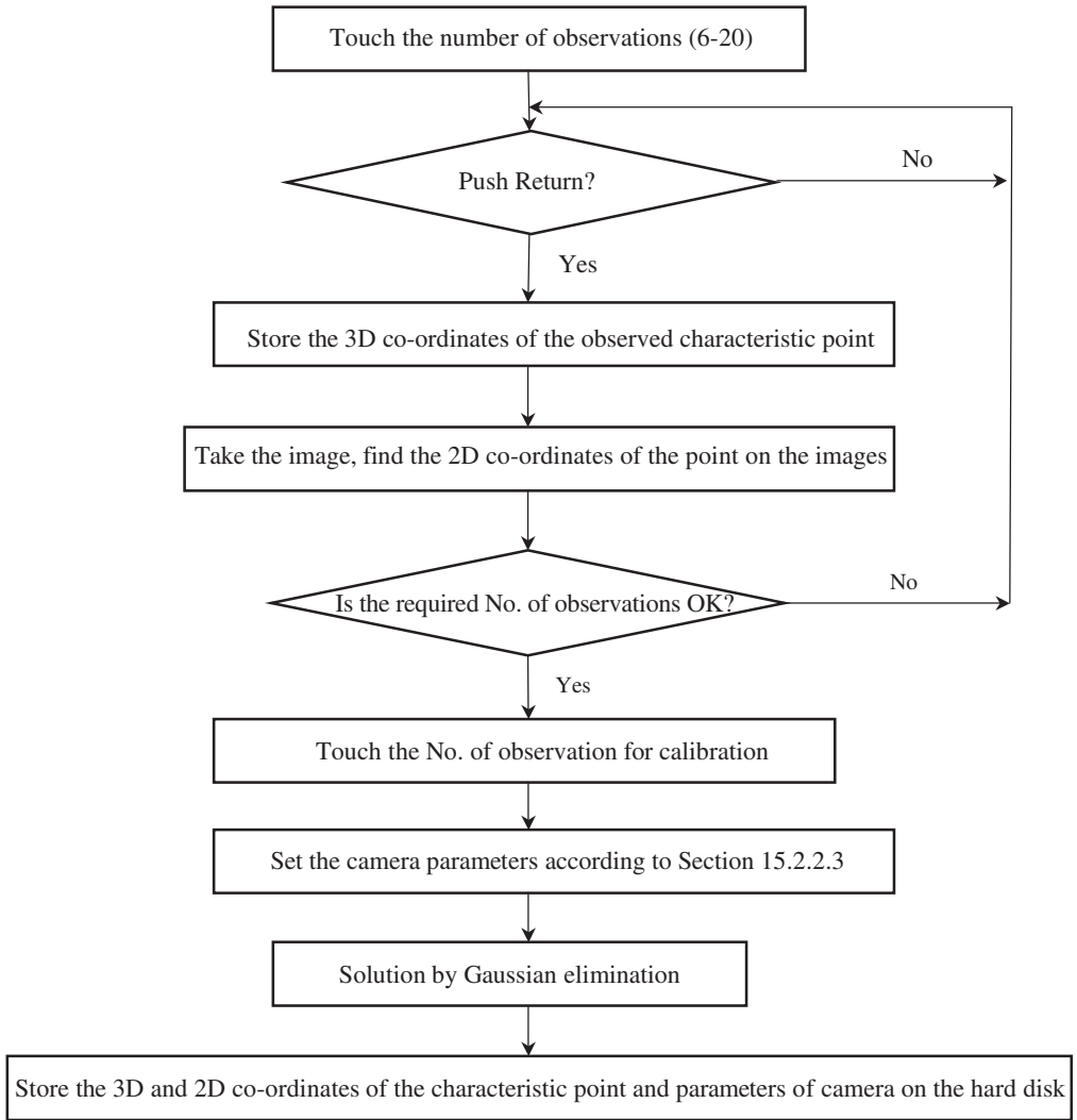
15.35 Flow chart for calibration
