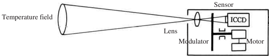
13.17 Single-path sensor
