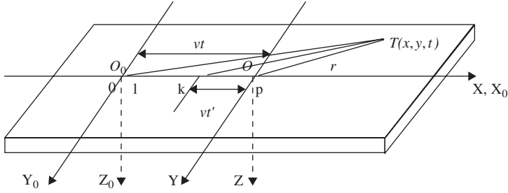
14.7 The co-ordinate system for calculation
