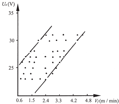
6.14 Allowable range of V_f and U_x for \phi 1.6\text{mm} wire
