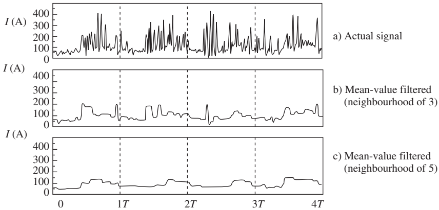
9.30 Welding current for CO 2 welding ( f = 3\text{ Hz} )
