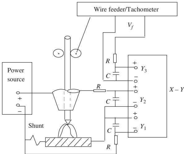
8.3 Circuit diagram for the study of a static mathematical model
