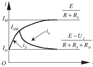
3.2 Welding current during short-circuiting arc welding
