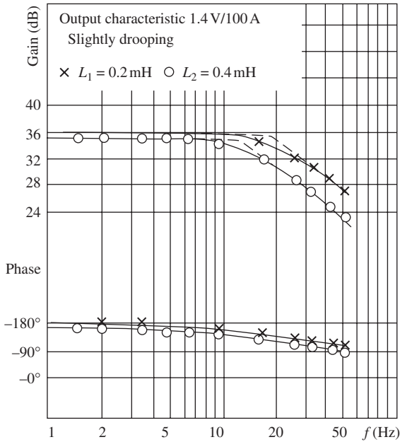
8.28 Frequency response of power-source
