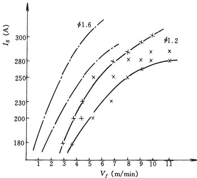
6.9 Allowable ranges of I_s and V_f
