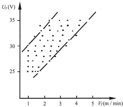
6.13 Allowable range of V_f and U_y for \phi 1.6\text{mm} wire
