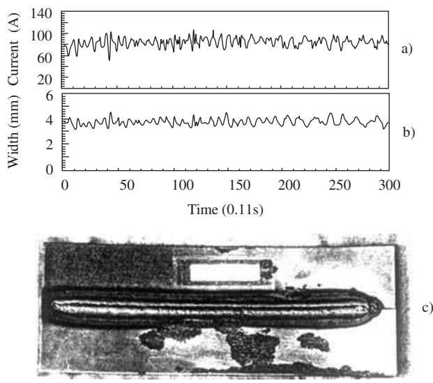
14.40 Closed-loop controlled welding of an I-butt joint without a gap
