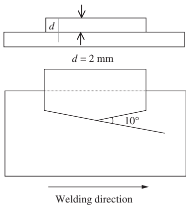
10.19 Lap joint
