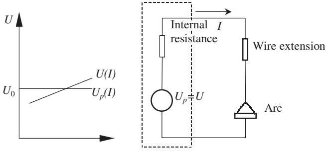
8.2 Equilibrium between an arc and a power source
