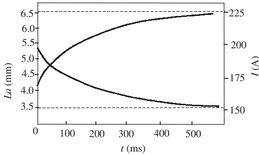
1.3 Response to arc-length disturbance
