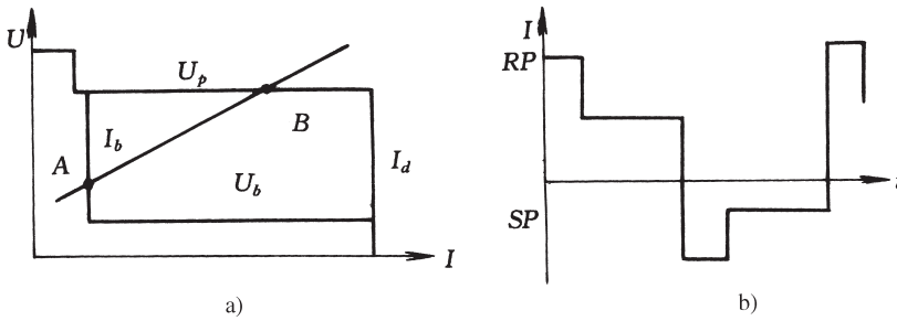
6.30 Output characteristics and current waveform for Control Method I
