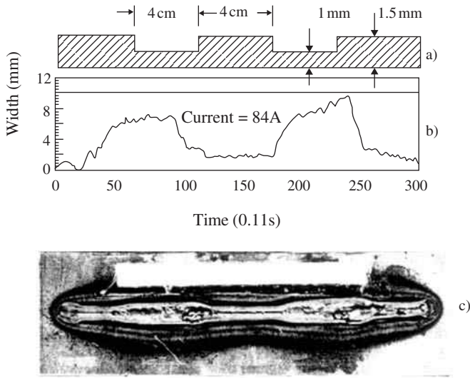
14.32 Effect of thickness variation (open-loop control)
