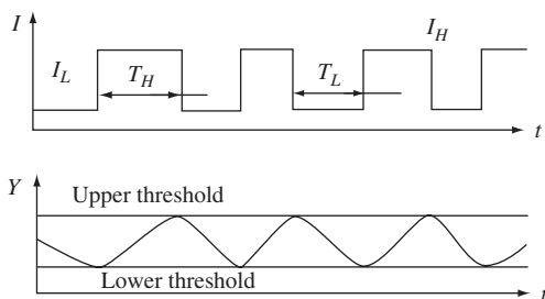
5.43 I and Y recorded in practice
