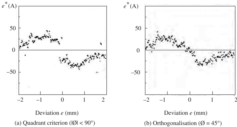
9.53 Sensing signal for \text{CO}_2 welding of a lap joint
