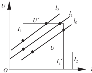
4.4 Rectangle-output characteristic
