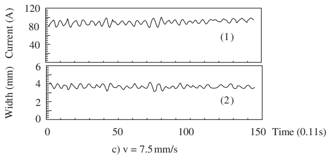
14.37 Closed-loop controlled welding with different welding speeds
