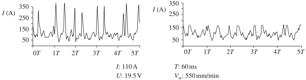
9.29 Sampled and filtered signal in CO 2 welding
