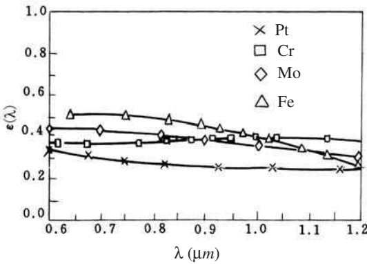
13.23 Emissivity obtained by experiment
