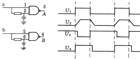
6.38 Circuit for obtaining the simultaneous conducting duration
