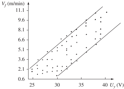
6.11 Allowable range of the V_f and U_y for \phi 1.2 mm wire
