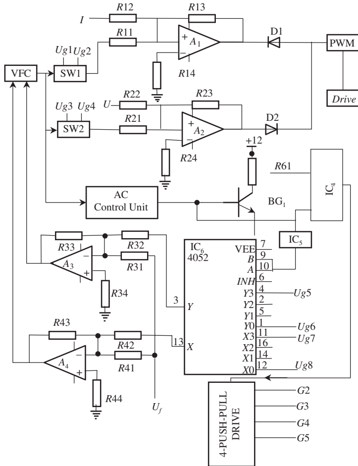
6.44 Electrical circuit for controlling a pulsed AC MIG power source
