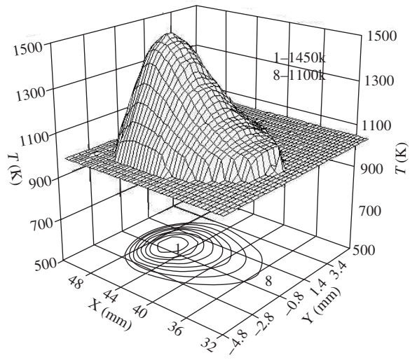
14.9 Experimental temperature distribution
