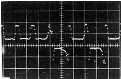
6.60 Current wave-form for AC/DCRP process
