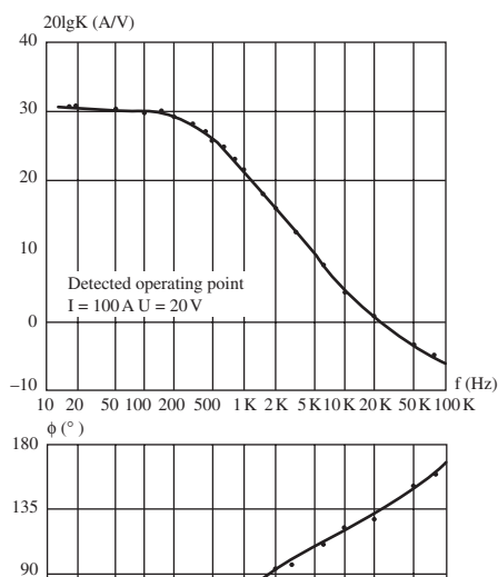
(b) Analogue type transistorized power source with flat output characteristics (A) (Made in TH University, Modified QHT-80)
