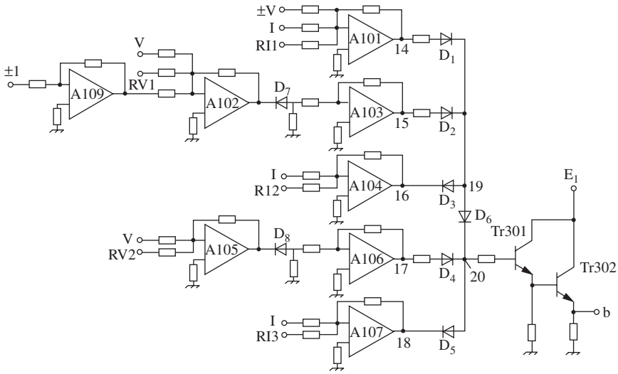
5.15 Automatic-transfer circuit
