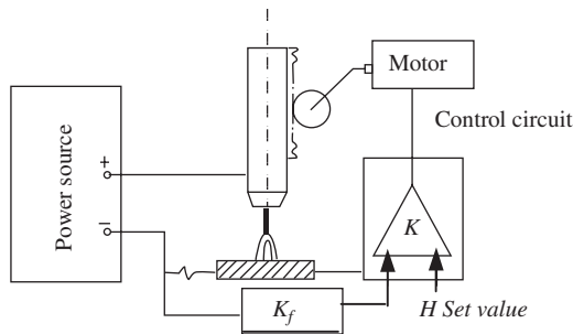
8.8 ACC control system
