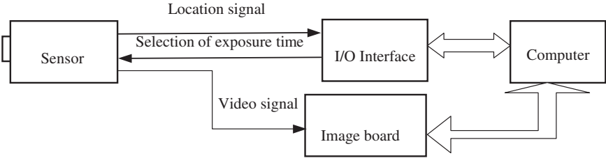
13.20 Two-colour sensor and computer I/O interface
