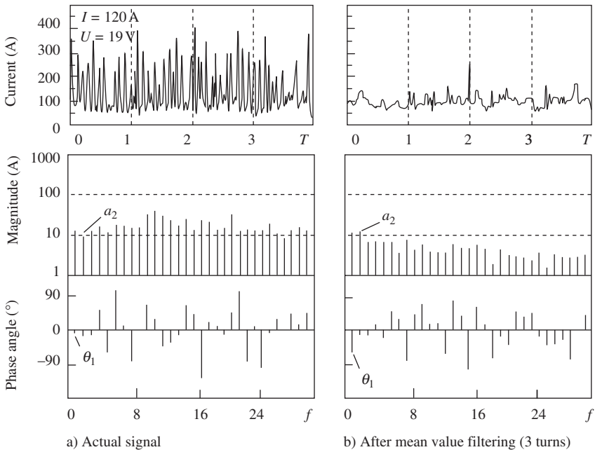
9.33 Current waveform and frequency spectrum for CO 2 ( f = 5 Hz)
