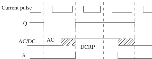
6.62 Time sequence of the control circuit in Fig. 6.61
