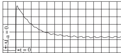
Abscissa t : 0.1 ms/Div., Ordinate \Delta L_a : 0.2 mm/Div. c) Pulsed MIG controlled by arc-length feedback
