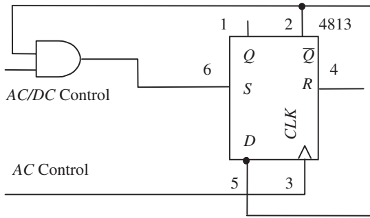
6.61 Control circuit for AC/DCRP
