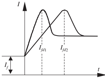
2.4 Schematic drawing of current waveform
