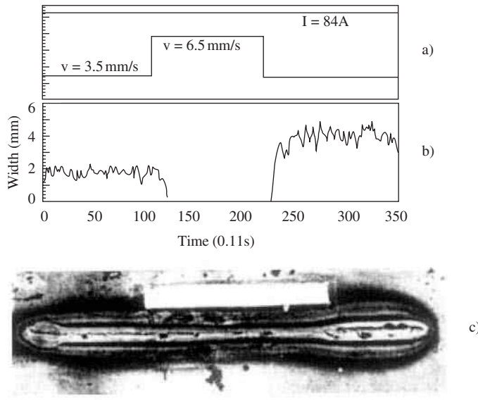
14.34 Effect of welding-speed change (open-loop control)
