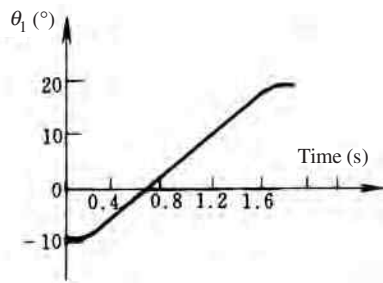
15.20 Turning of column -10^{\circ} to 20^{\circ}
