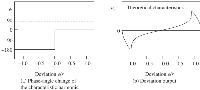
9.54 Theoretical detection characteristics
