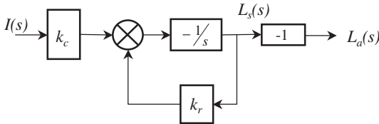
8.11 Simplification of Fig. 8.10
