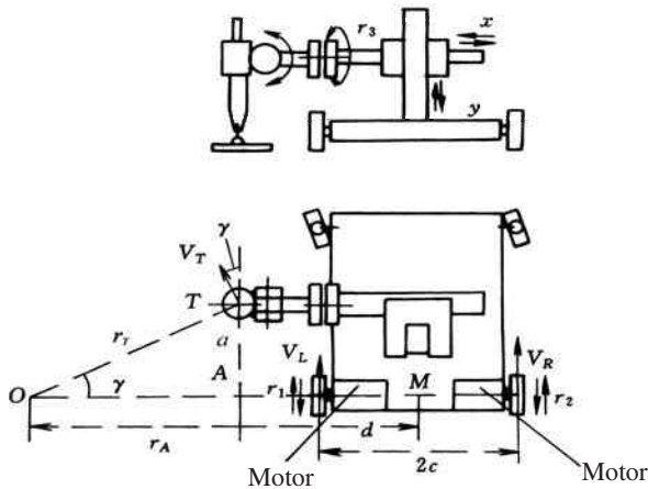
10.28 Schematic drawing of the tractor's construction
