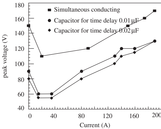
6.39 Voltage peak on MOSFET under different circuit parameters
