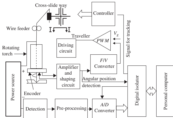
10.1 Schematic diagram of a tracking system using an arc sensor
