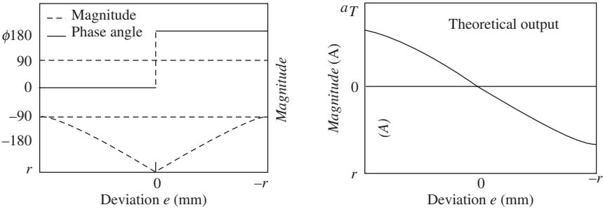
9.46 Theoretical detection characteristics
