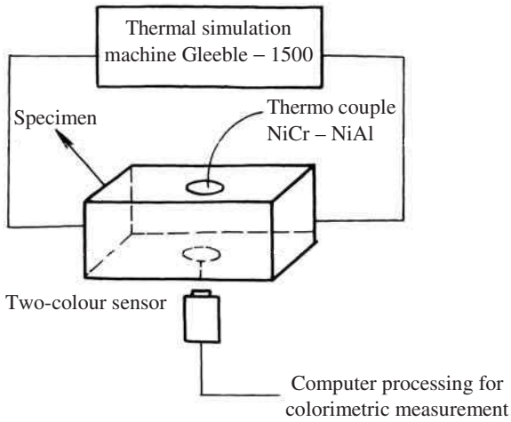
13.24 Off-line calibration
