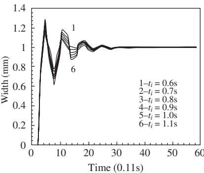
a) Step response
