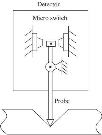
7.2 Contact-type sensor
