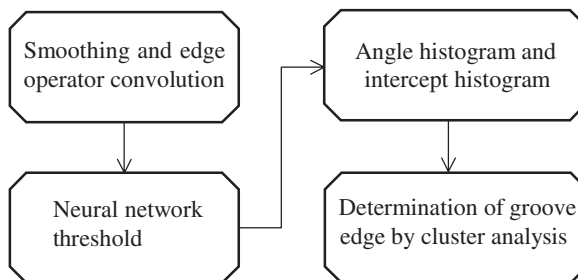
15.4 Flowchart for recognition of a groove by histogram statistics
