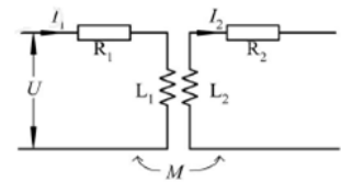
Fig. 2. Equivalent circuit of eddy current flowmeter sensor
