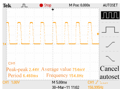
Fig. 9. Experimental results for DN4 mm with 40 L/h
