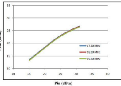
Fig. 10. Measurement results of power out versus power in from 1720 to 1920MHz for MMIC by long-gate-length method
