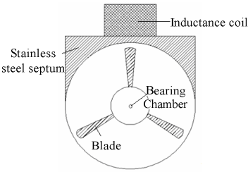
Fig. 1. Diagram of eddy current flowmeter sensor
