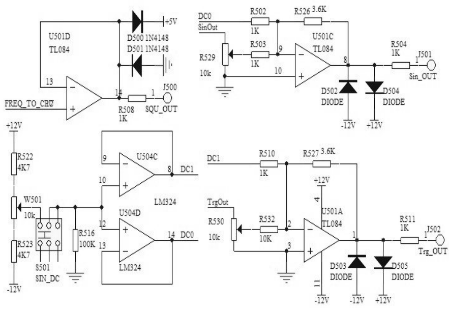
Fig. 6. Output Circuit of the Signal Generator
