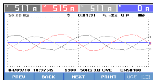
b. Source current waveform after compensation
