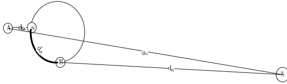
Fig. 2. IID estimate for a rigid spherical head
