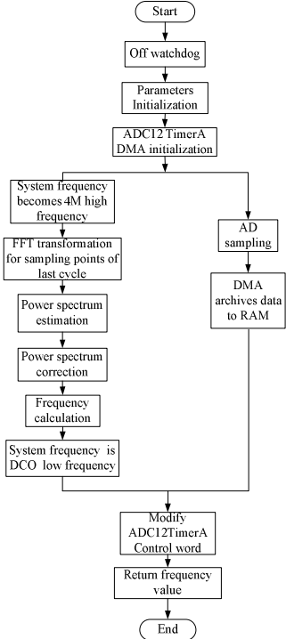
Fig. 8. FFT calculation
