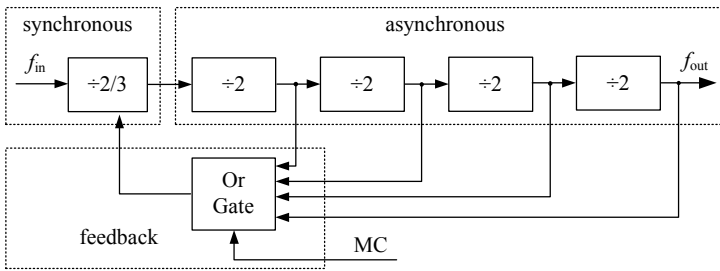
Fig. 1. Divide-by 32/33 dual-modulus prescaler
