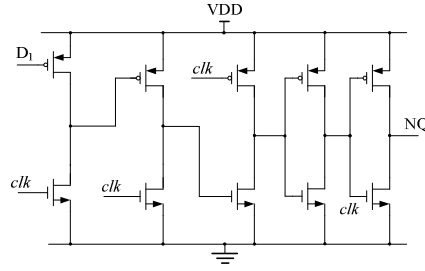
Fig. 7. Asynchronous divider
