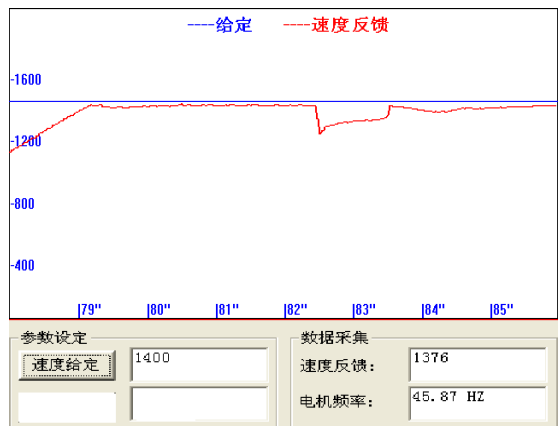
Fig. 5. Test curve of system interference
