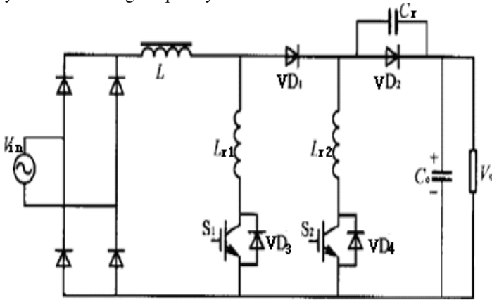
(a) circuit
