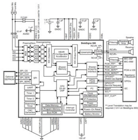
Fig. 3. The functional diagram of development tool BelaSigna 300
