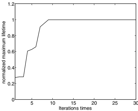
Fig. 1. Network lifetime convergence curve
