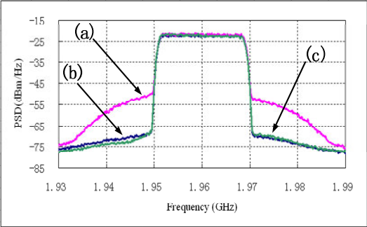
Fig. 4. Test results comparison between LUT DPD and memory polynomial DPD
