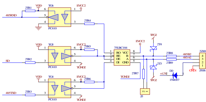
Fig. 3. Communications circuits
