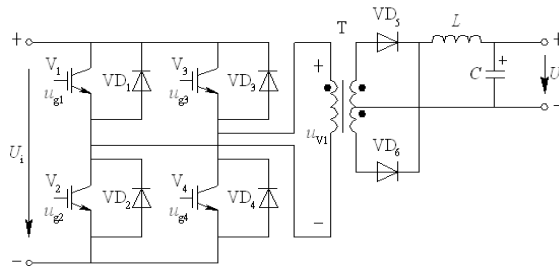
Fig. 5. The Full-Bridge conversion circuit
