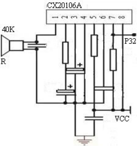
Fig. 4. Ultrasonic Receiving Circuit
