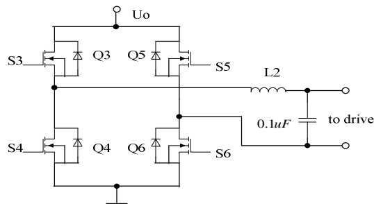
Fig. 4. The switching power amplifier’s main circuit
