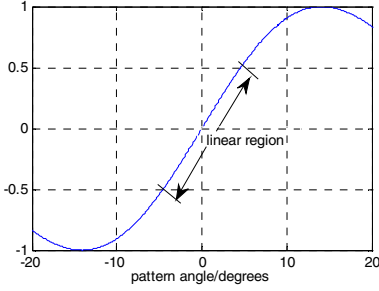
Fig. 1. The normalized \frac{\Delta}{\Sigma} vs. pattern angle
