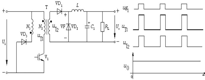
(a) schematic diagram (b) waveforms
