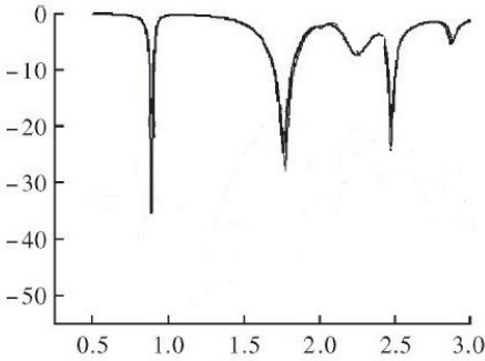
Fig. 3. The tri-band antenna return loss
