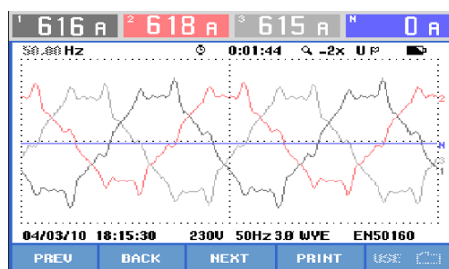
a. Source current waveform before compensation
