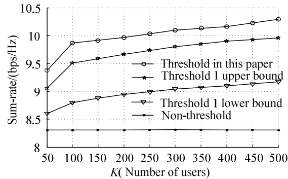
Fig. 2. Sum-rate versus the number of users for Z=100 bits
