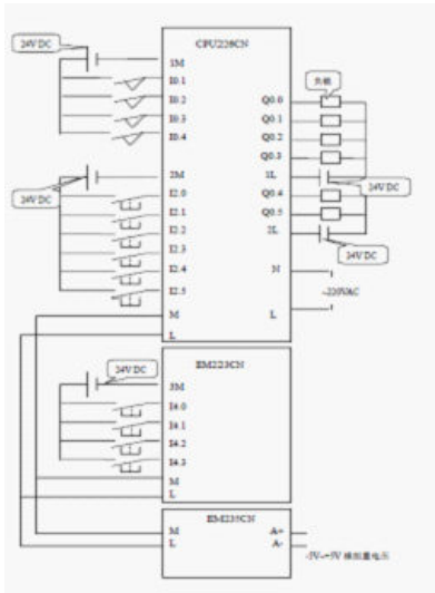
Fig. 3. PLC controlled robot I / O wiring diagram
