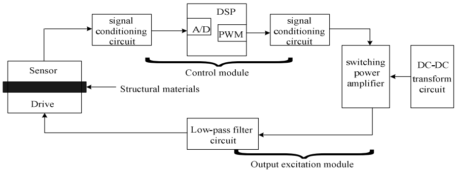
Fig. 1. Active vibration control system diagram
