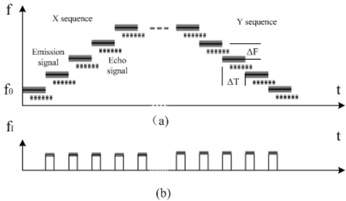
Fig. 6. The emission signal and echo signal
