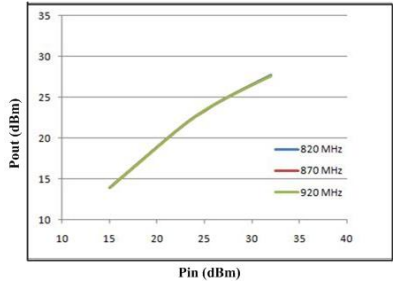
Fig. 9. Measurement results of power out versus power in from 820 to 920MHz for MMIC by long-gate-length method
