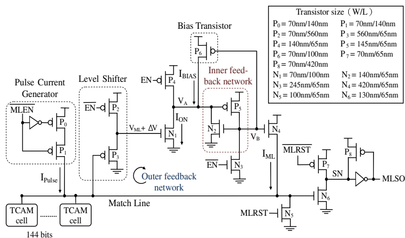
Fig. 3. Double-feedback match-line sense amplifier
