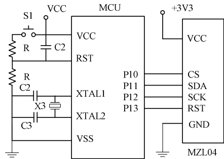
Fig. 5. Circuit of the data display
