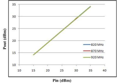
Fig. 7. Measurement results of power out versus power in from 820 to 920MHz for MMIC by three-gate-fingers method
