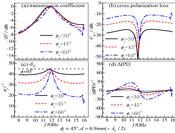
Fig. 5. Influence of incidence angle on the transmission characteristics of FSS in cross polarization
