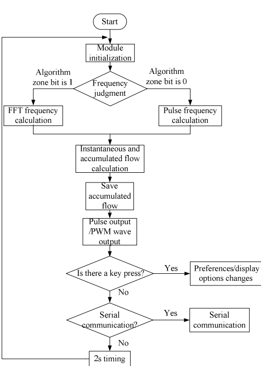
Fig. 7. Main flowchart
