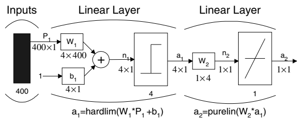
Fig. 2. Basic network to distinguish 15 faces
