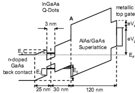
Fig. 1. Scheme of the energy band structure of the sample along the growth direction
